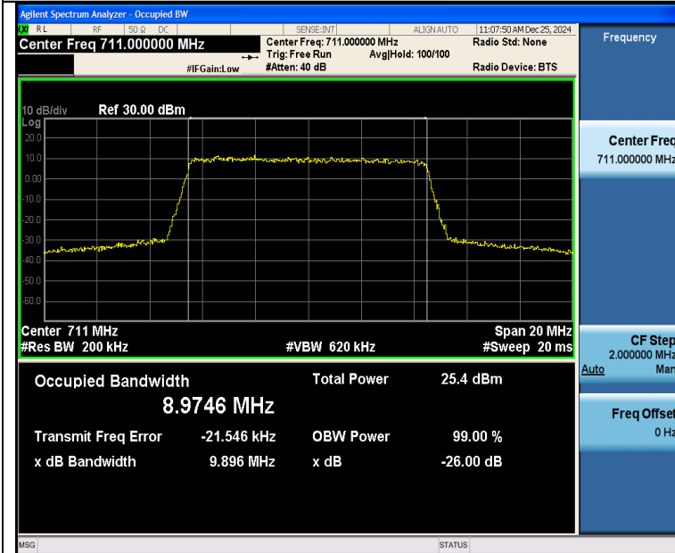
Band12-10MHz-QPSK-23130-50RB#0-PASS
