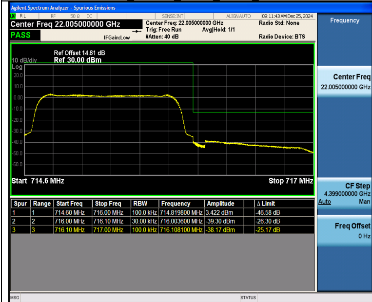
Band12 1.4MHz_QPSK_23173_6RB#0
