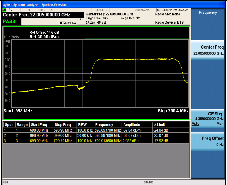
Band12 1.4MHz_16QAM_23017_6RB#0
