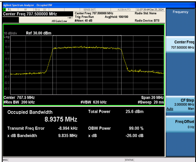
Band12-10MHz-QPSK-23095-50RB#0-PASS
