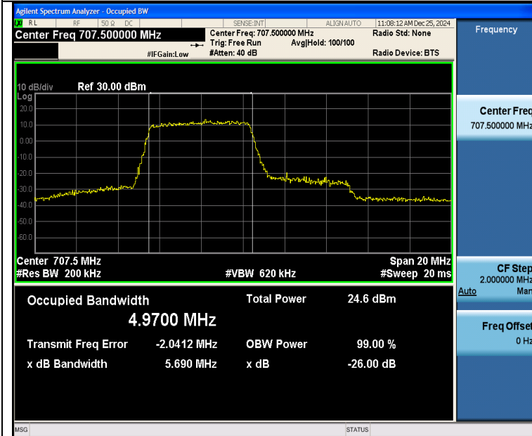
Band12-10MHz-16QAM-23095-27RB#0-PASS
