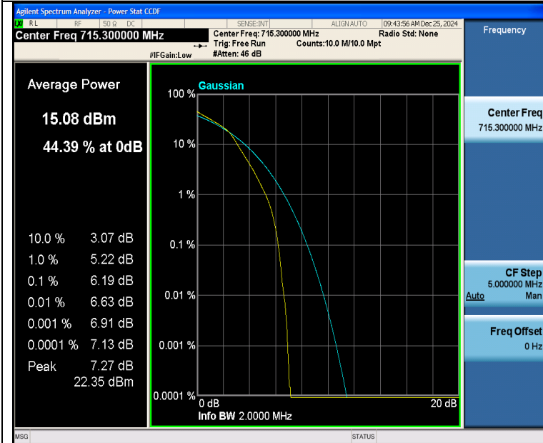
Band12-1.4MHz-16QAM-23173-6RB#0-PASS
