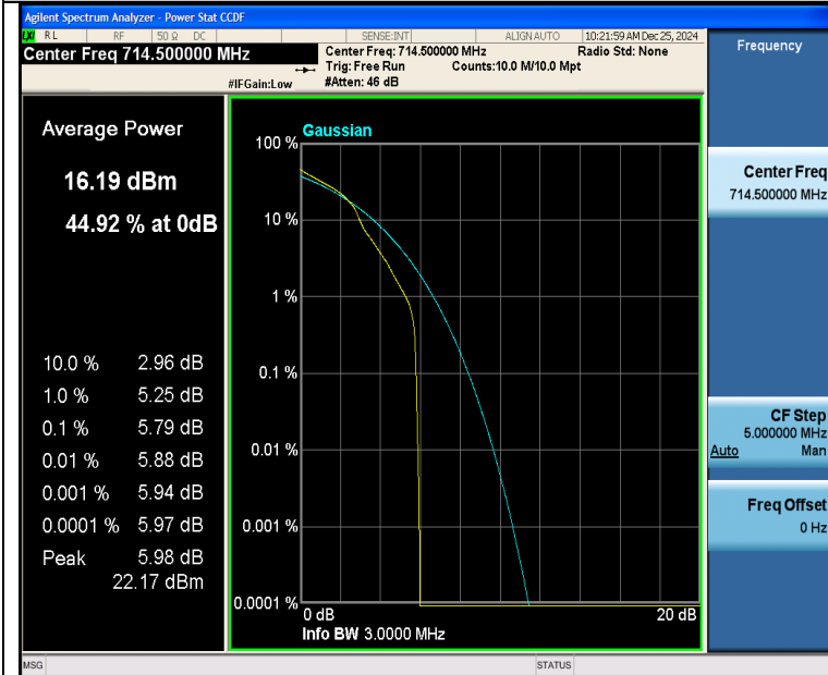
Band12-3MHz-16QAM-23165-1RB#0-PASS
