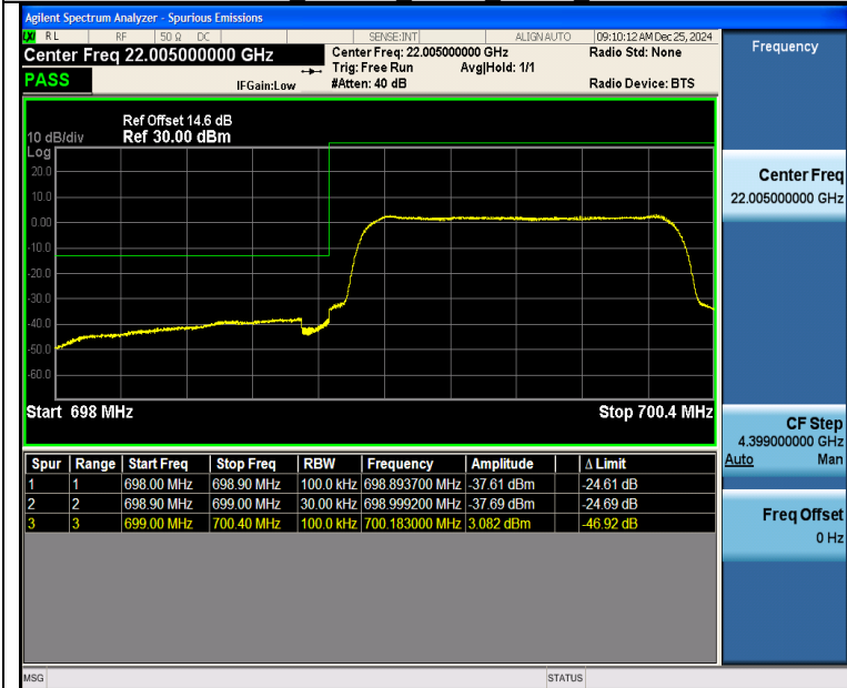
Band12 1.4MHz_QPSK_23017_6RB#0
