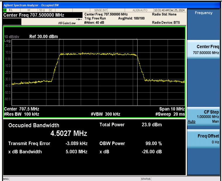
Band12-5MHz-16QAM-23095-25RB#0-PASS
