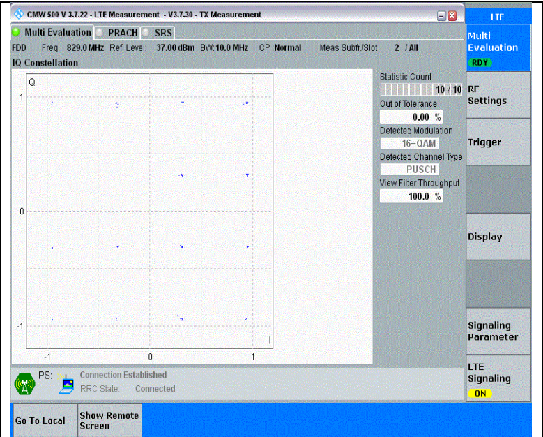
Band5-10MHz-16QAM-20450-1RB#0-PASS
