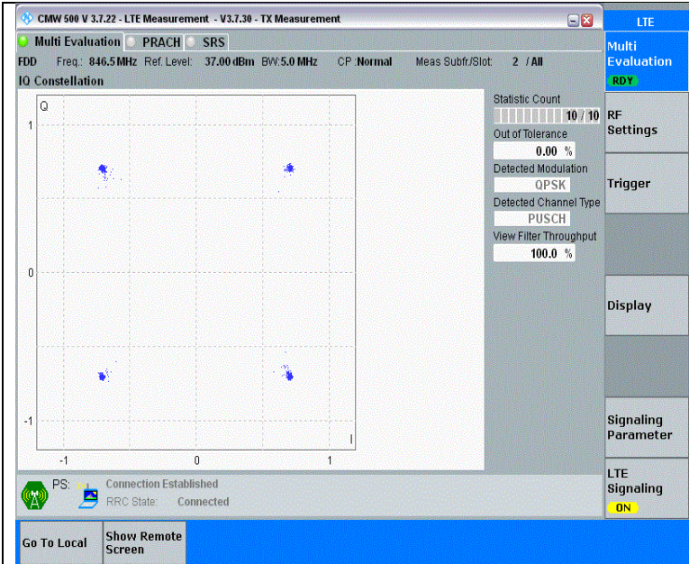
Band5-5MHz-QPSK-20625-25RB#0-PASS
