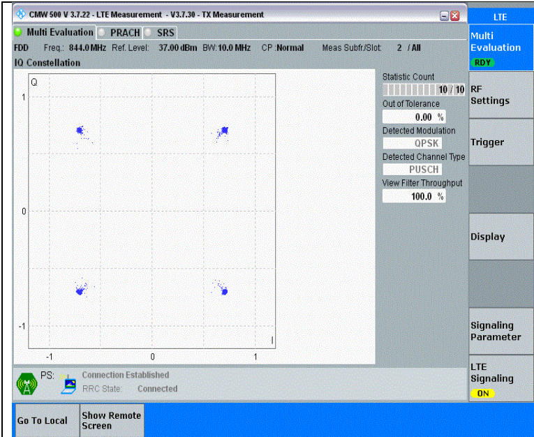
Band5-10MHz-QPSK-20600-50RB#0-PASS
