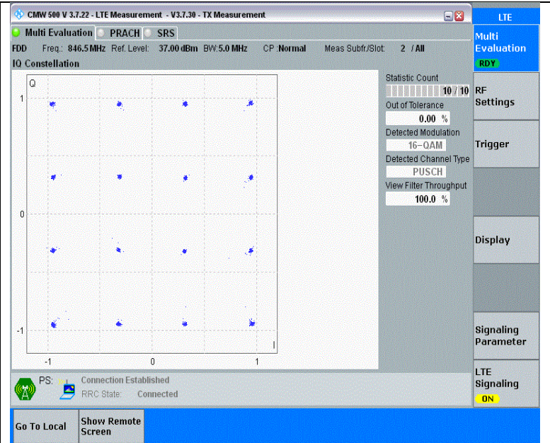
Band5-5MHz-16QAM-20625-25RB#0-PASS
