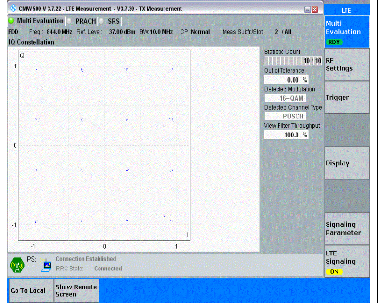
Band5-10MHz-16QAM-20600-1RB#0-PASS
