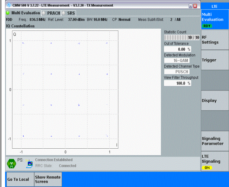
Band5-10MHz-16QAM-20525-1RB#0-PASS
