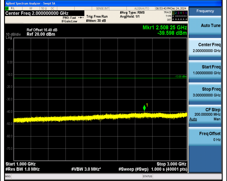
Band5_5MHz_QPSK_20425_25RB#0_1000~3000_1000~3000
