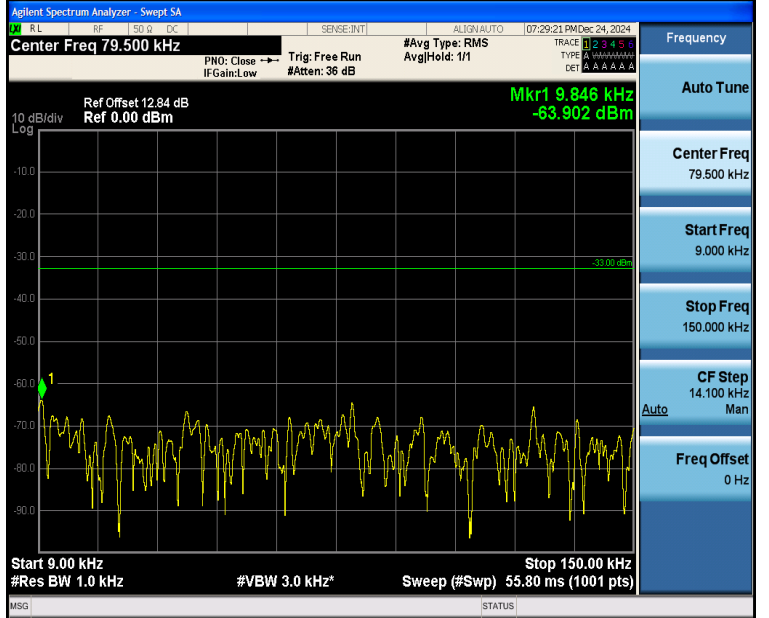
Band5_10MHz_16QAM_20525_1RB#0_0.009~0.15_0.009~0.15
