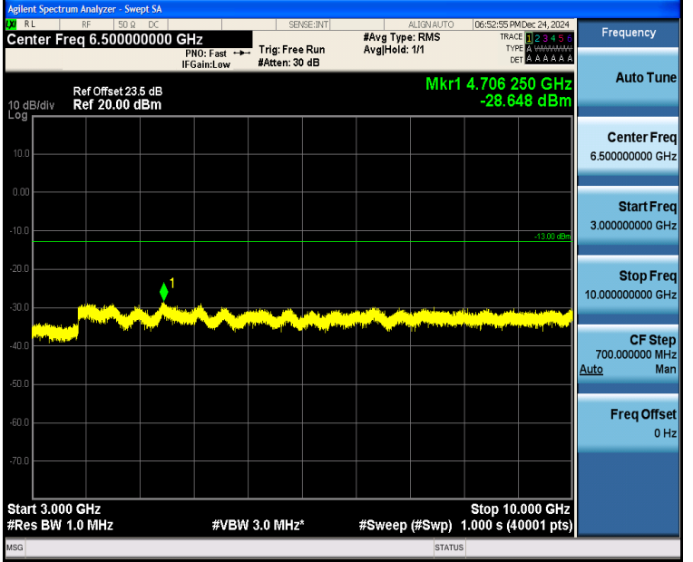
Band5_5MHz_16QAM_20425_1RB#24_3000~10000_3000~10000
