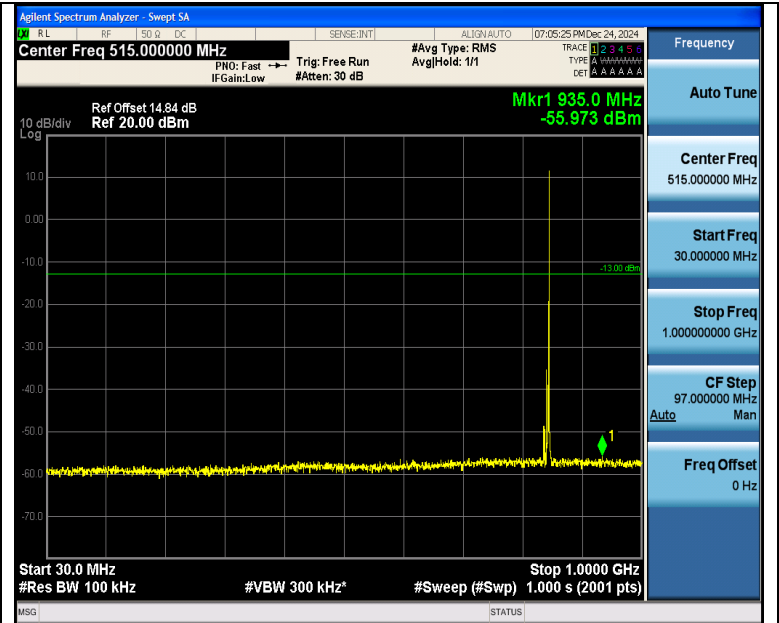
Band5_5MHz_16QAM_20625_1RB#24_30~1000_30~1000
