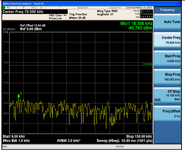
Band5_5MHz_16QAM_20425_25RB#0_0.009~0.15_0.009~0.15
