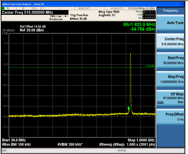
Band5_5MHz_16QAM_20525_25RB#0_30~1000_30~1000
