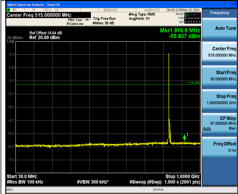
Band5_5MHz_QPSK_20525_1RB#0_30~1000_30~1000
