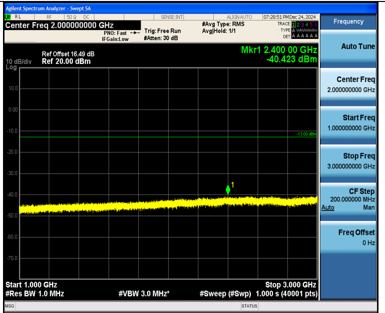
Band5_10MHz_QPSK_20525_1RB#0_1000~3000_1000~3000
