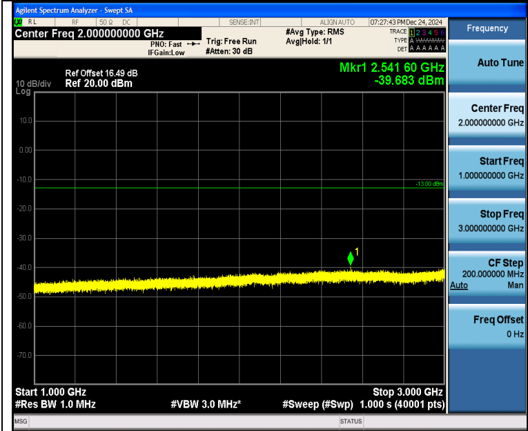
Band5_10MHz_16QAM_20450_1RB#49_1000~3000_1000~3000
