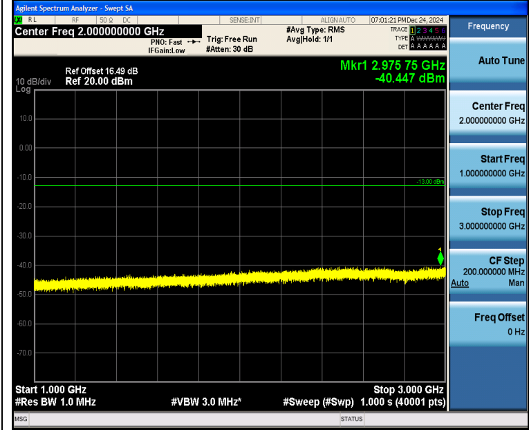
Band5_5MHz_16QAM_20525_25RB#0_1000~3000_1000~3000
