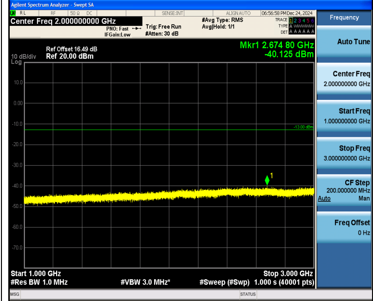
Band5_5MHz_16QAM_20525_1RB#0_1000~3000_1000~3000
