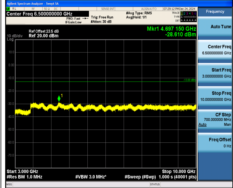
Band5_10MHz_QPSK_20525_1RB#0_3000~10000_3000~10000
