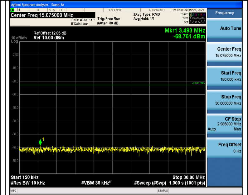
Band5_5MHz_QPSK_20625_1RB#0_0.15~30_0.15~30
