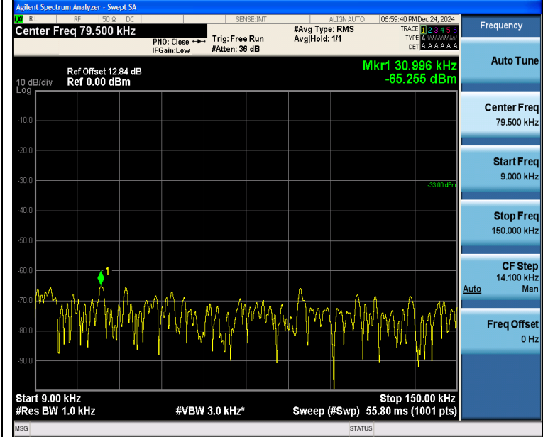
Band5_5MHz_QPSK_20525_25RB#0_0.009~0.15_0.009~0.15
