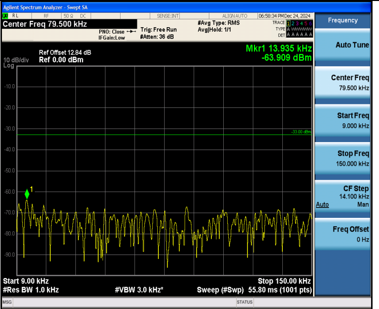
Band5_5MHz_16QAM_20525_1RB#24_0.009~0.15_0.009~0.15
