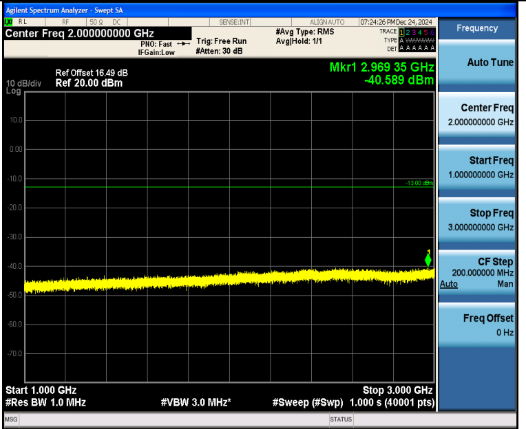
Band5_10MHz_QPSK_20450_1RB#0_1000~3000_1000~3000
