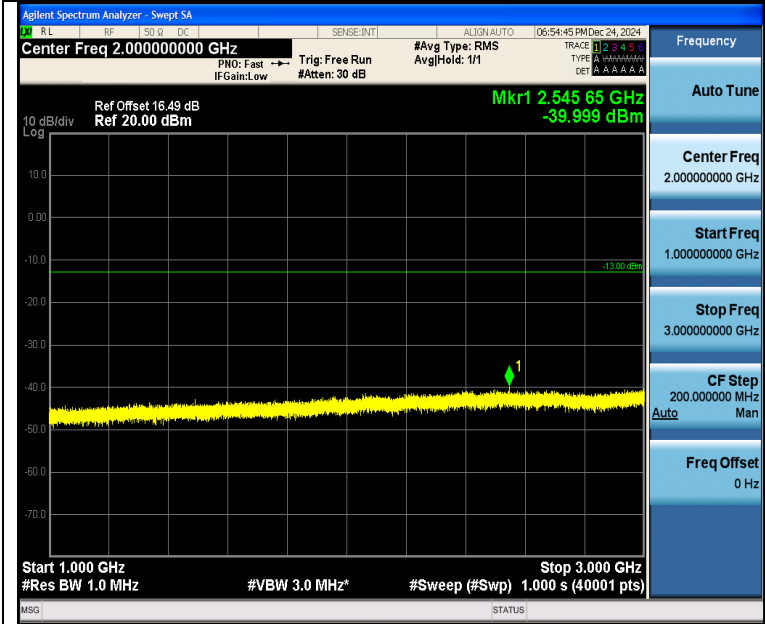
Band5_5MHz_16QAM_20425_25RB#0_1000~3000_1000~3000
