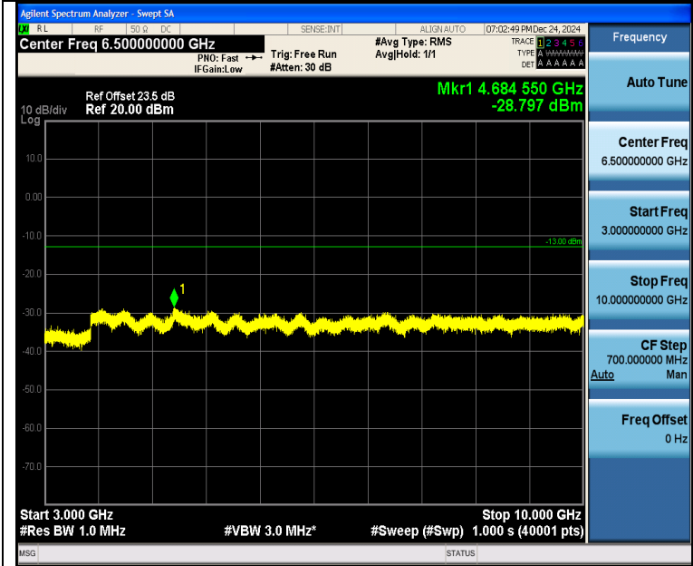
Band5_5MHz_QPSK_20625_1RB#0_3000~10000_3000~10000
