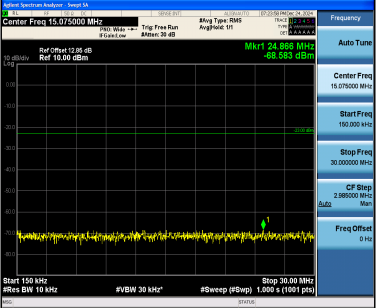
Band5_10MHz_QPSK_20450_1RB#0_0.15~30_0.15~30
