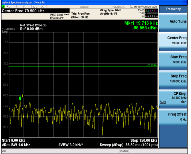
Band5_5MHz_16QAM_20525_25RB#0_0.009~0.15_0.009~0.15
