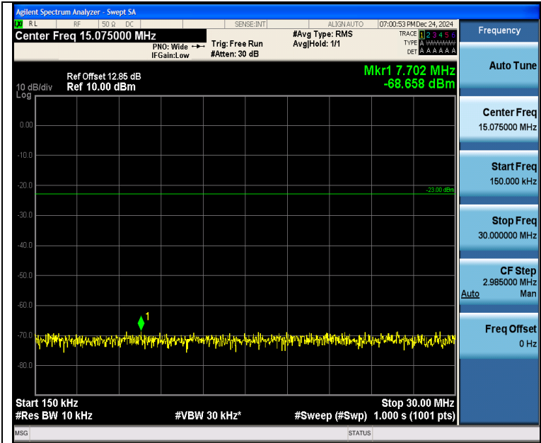
Band5_5MHz_16QAM_20525_25RB#0_0.15~30_0.15~30
