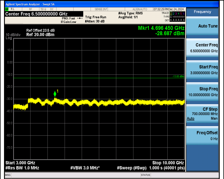
Band5_10MHz_16QAM_20525_1RB#49_3000~10000_3000~10000
