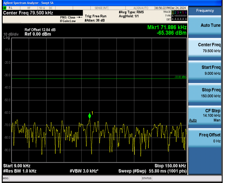
Band5_5MHz_16QAM_20525_1RB#0_0.009~0.15_0.009~0.15
