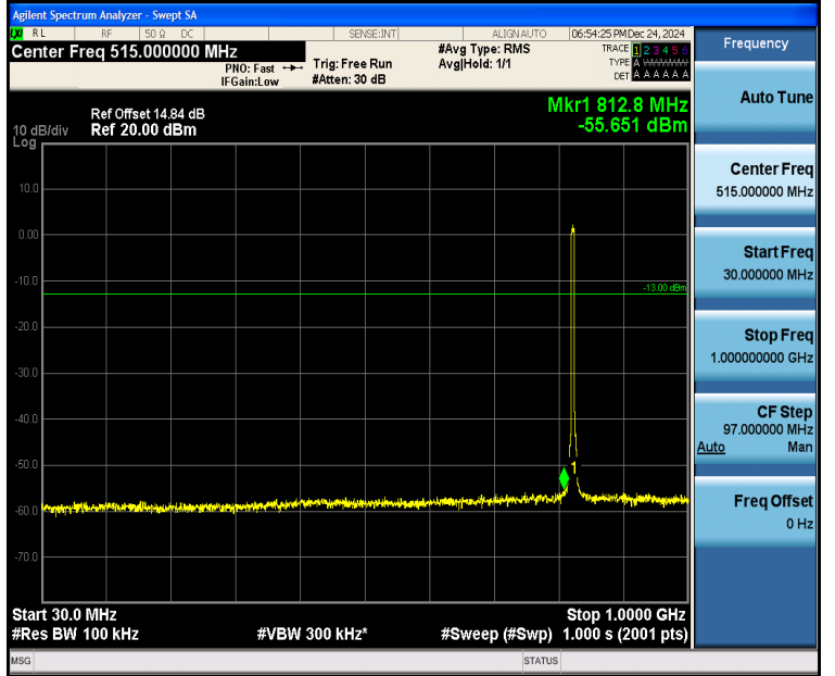
Band5_5MHz_16QAM_20425_25RB#0_30~1000_30~1000
