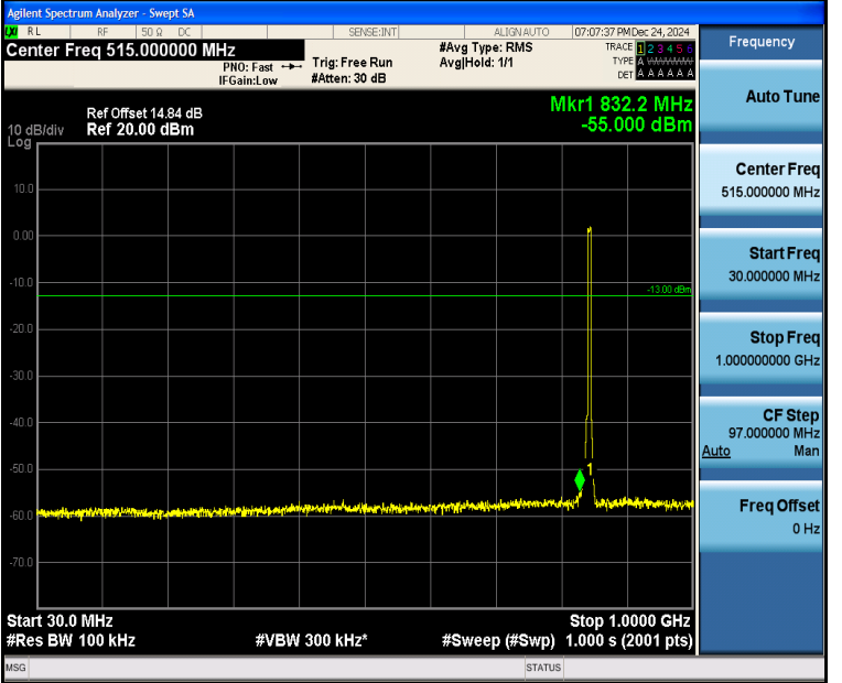
Band5_5MHz_16QAM_20625_25RB#0_30~1000_30~1000
