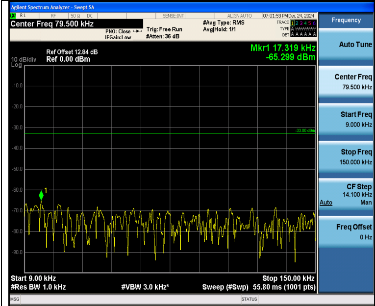
Band5_5MHz_QPSK_20625_1RB#0_0.009~0.15_0.009~0.15
