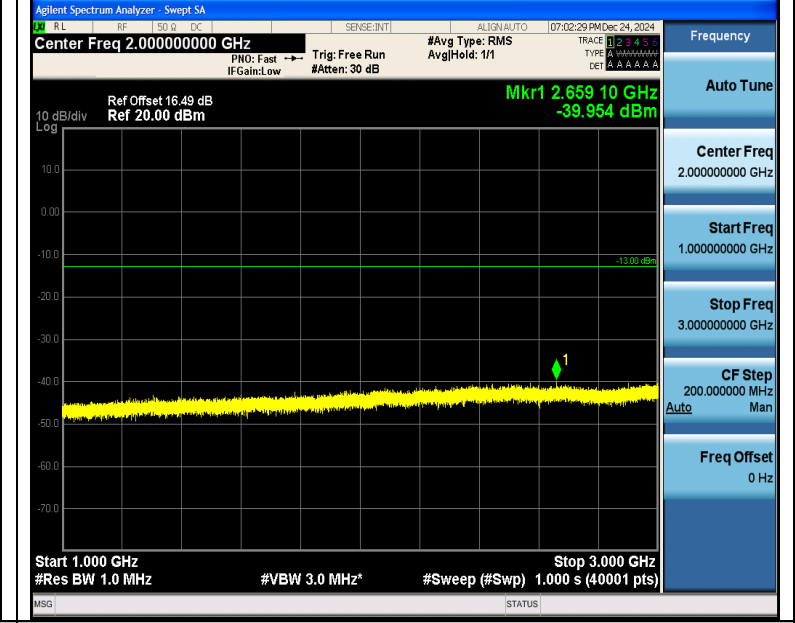
Band5_5MHz_QPSK_20625_1RB#0_1000~3000_1000~3000
