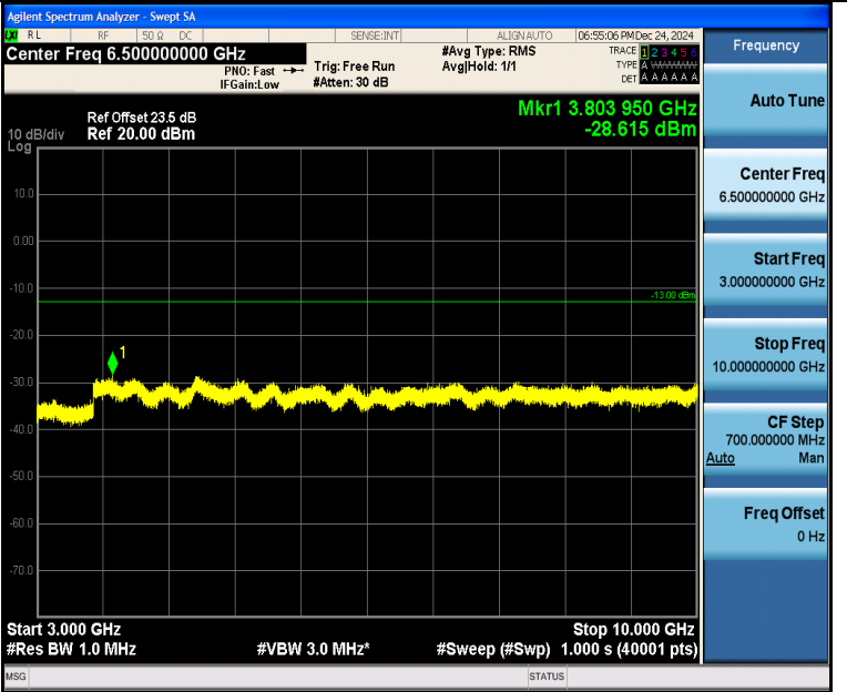
Band5_5MHz_16QAM_20425_25RB#0_3000~10000_3000~10000
