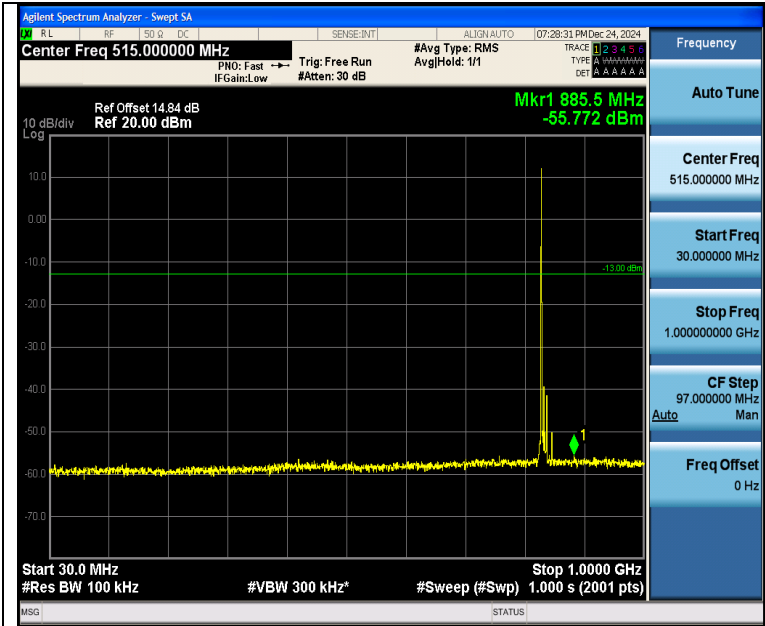
Band5_10MHz_QPSK_20525_1RB#0_30~1000_30~1000
