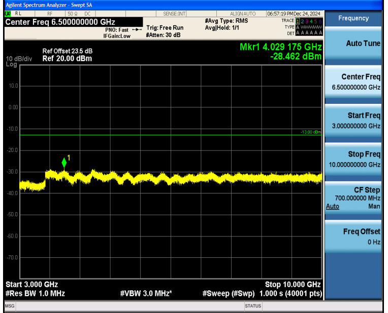
Band5_5MHz_16QAM_20525_1RB#0_3000~10000_3000~10000
