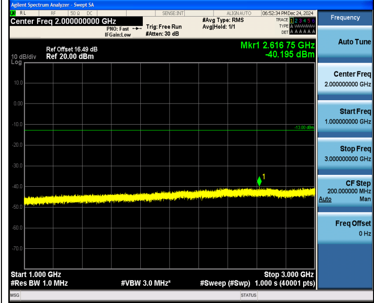
Band5_5MHz_16QAM_20425_1RB#24_1000~3000_1000~3000
