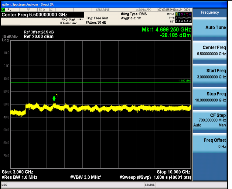
Band5_5MHz_16QAM_20625_1RB#0_3000~10000_3000~10000
