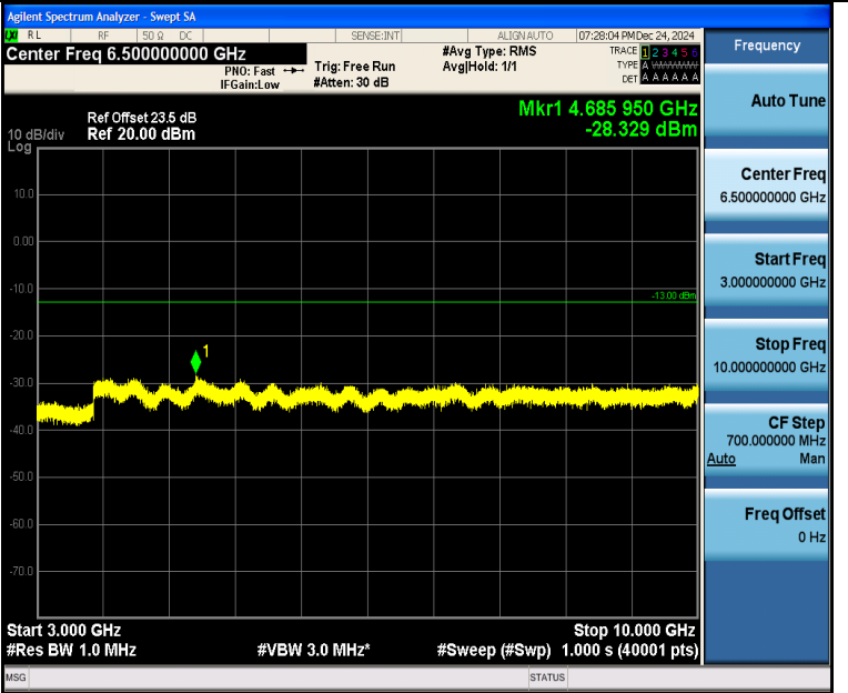
Band5_10MHz_16QAM_20450_1RB#49_3000~10000_3000~10000
