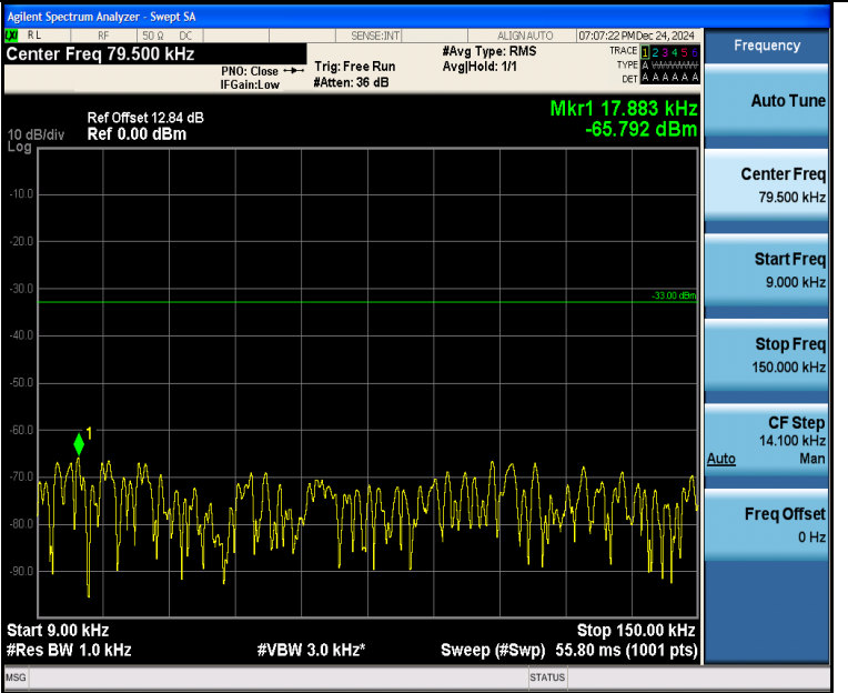
Band5_5MHz_16QAM_20625_25RB#0_0.009~0.15_0.009~0.15
