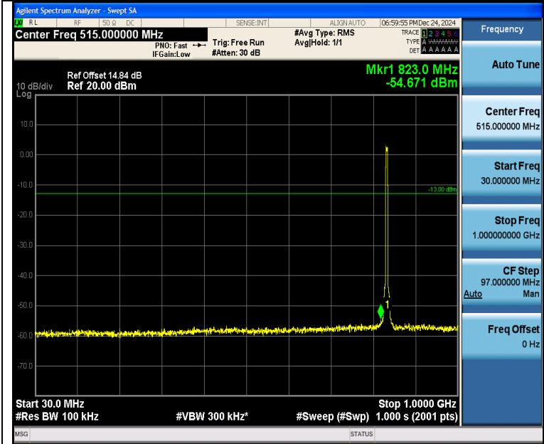
Band5_5MHz_QPSK_20525_25RB#0_30~1000_30~1000
