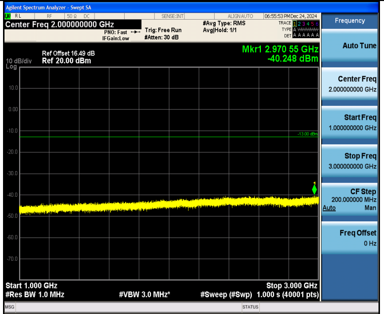
Band5_5MHz_QPSK_20525_1RB#0_1000~3000_1000~3000
