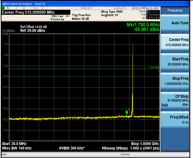
Band5_5MHz_16QAM_20425_1RB#24_30~1000_30~1000
