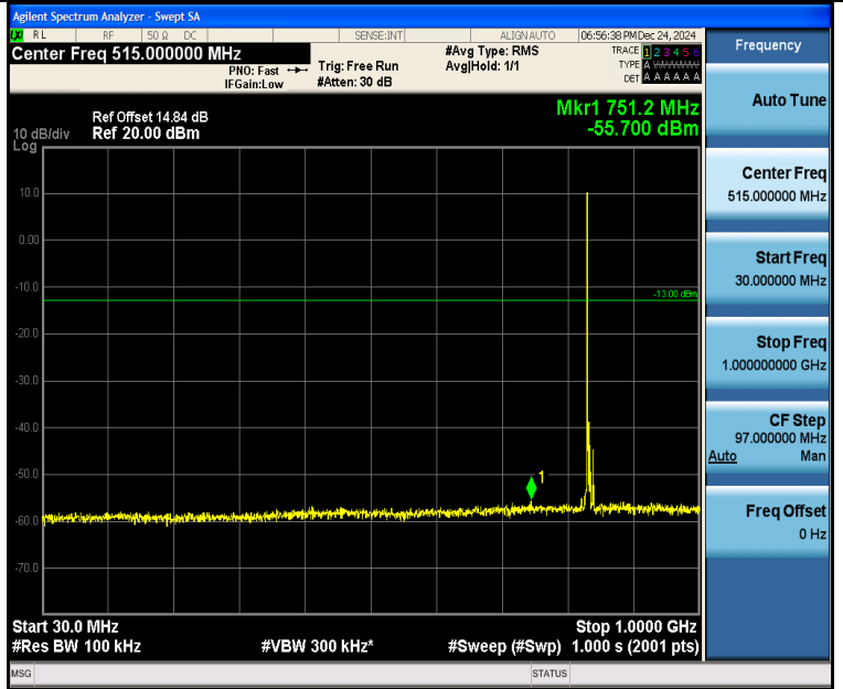
Band5_5MHz_16QAM_20525_1RB#0_30~1000_30~1000
