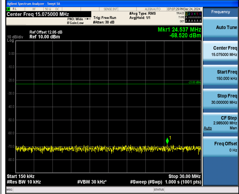
Band5_5MHz_16QAM_20625_25RB#0_0.15~30_0.15~30
