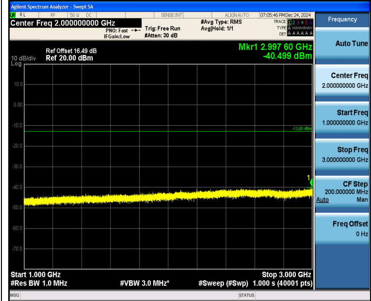
Band5_5MHz_16QAM_20625_1RB#24_1000~3000_1000~3000
