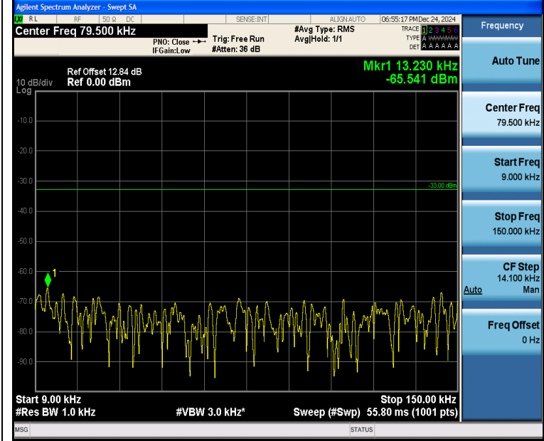
Band5_5MHz_QPSK_20525_1RB#0_0.009~0.15_0.009~0.15
