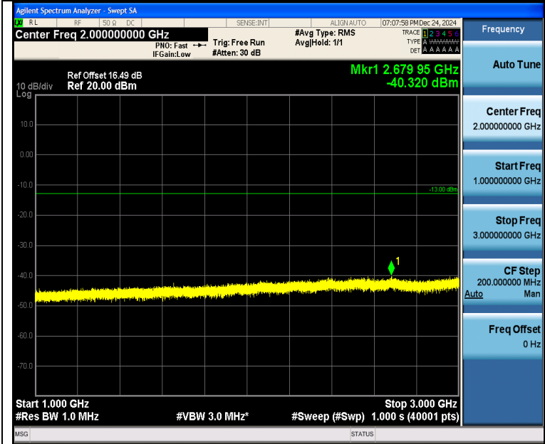
Band5_5MHz_16QAM_20625_25RB#0_1000~3000_1000~3000
