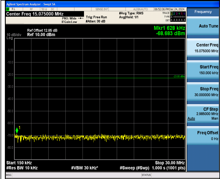
Band5_5MHz_16QAM_20425_1RB#24_0.15~30_0.15~30
