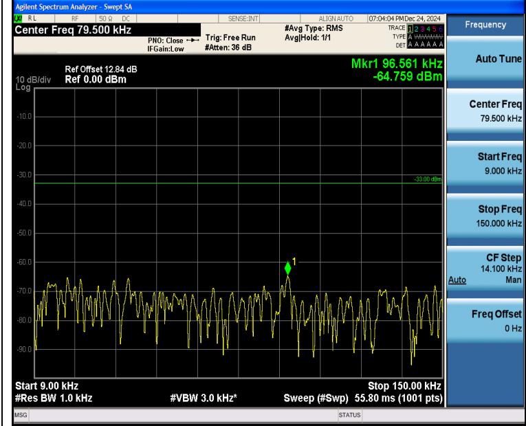
Band5_5MHz_QPSK_20625_1RB#24_0.009~0.15_0.009~0.15
