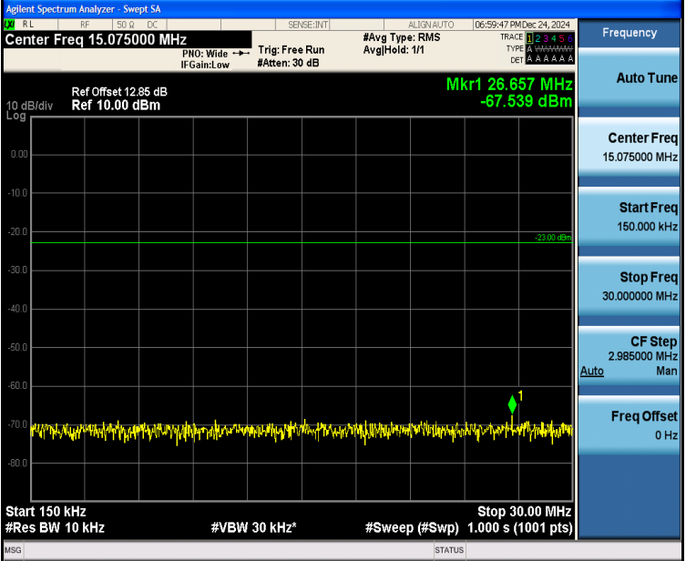
Band5_5MHz_QPSK_20525_25RB#0_0.15~30_0.15~30
