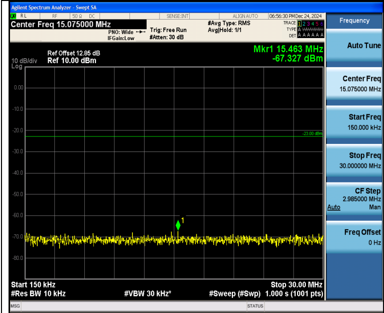
Band5_5MHz_16QAM_20525_1RB#0_0.15~30_0.15~30
