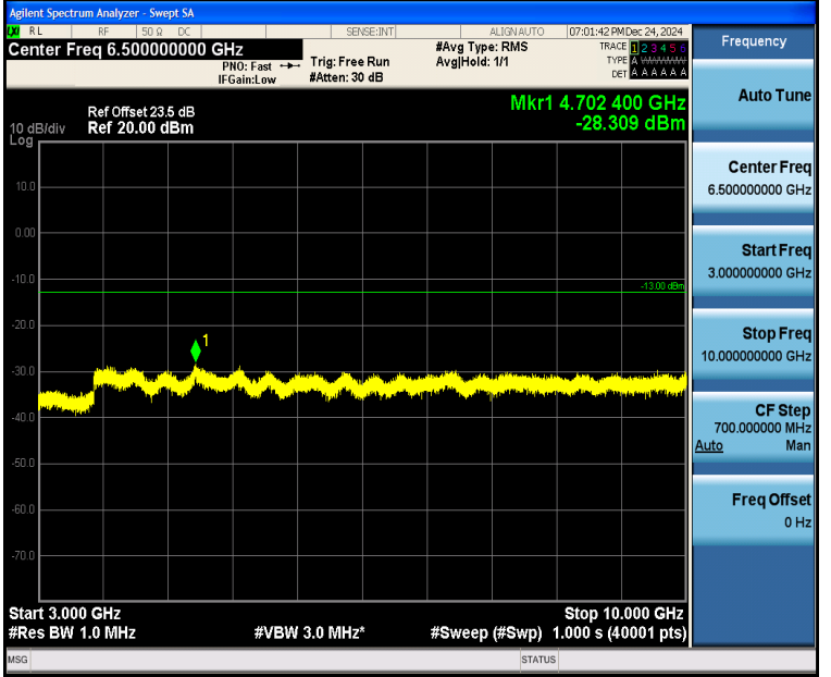
Band5_5MHz_16QAM_20525_25RB#0_3000~10000_3000~10000
