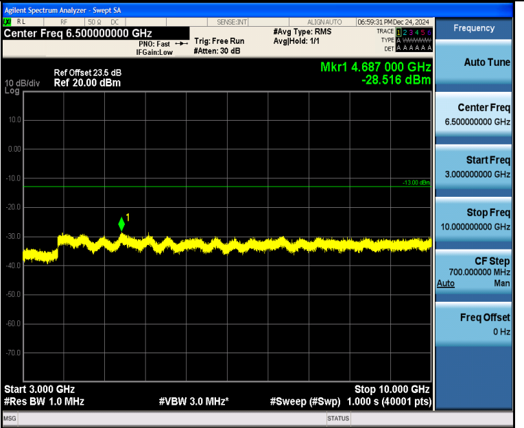
Band5_5MHz_16QAM_20525_1RB#24_3000~10000_3000~10000
