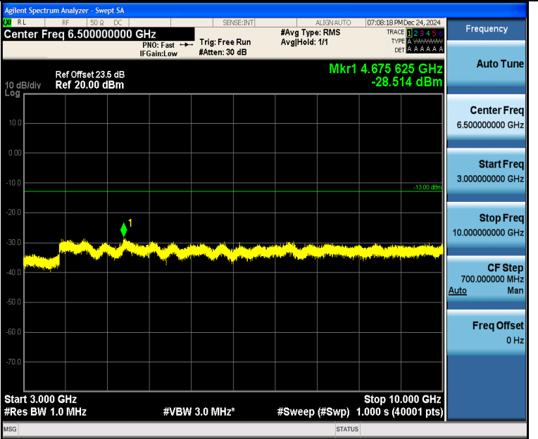
Band5_5MHz_16QAM_20625_25RB#0_3000~10000_3000~10000
