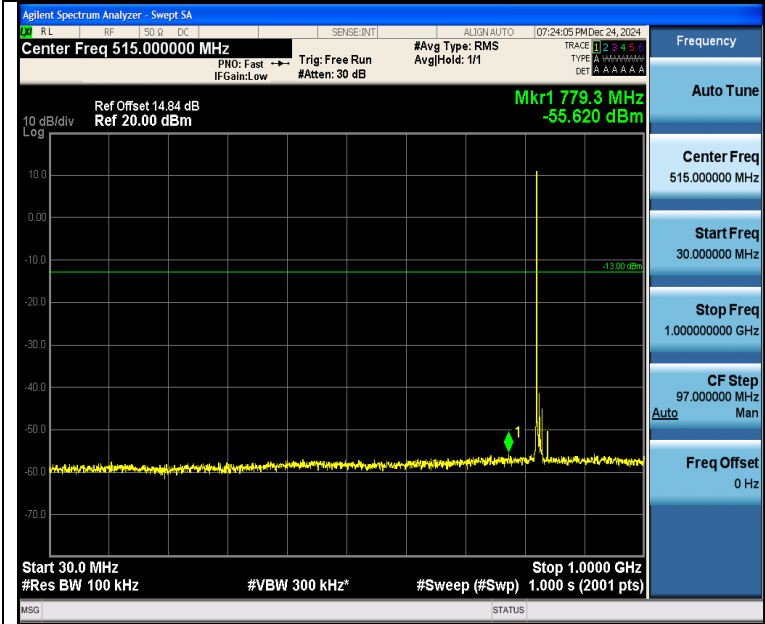
Band5_10MHz_QPSK_20450_1RB#0_30~1000_30~1000
