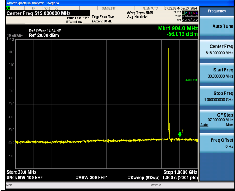
Band5_5MHz_QPSK_20625_1RB#0_30~1000_30~1000
