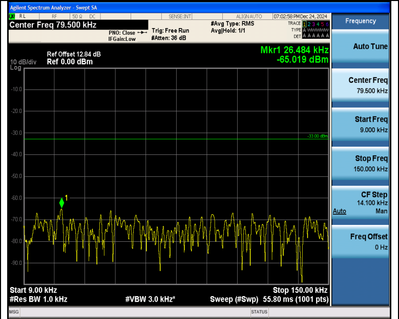
Band5_5MHz_16QAM_20625_1RB#0_0.009~0.15_0.009~0.15
