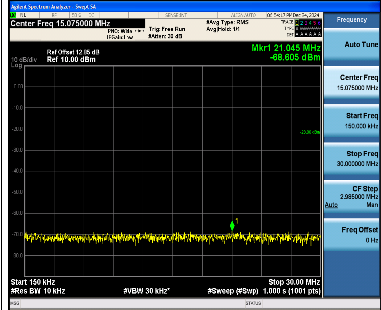
Band5_5MHz_16QAM_20425_25RB#0_0.15~30_0.15~30
