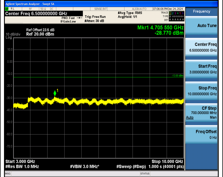
Band5_5MHz_16QAM_20625_1RB#24_3000~10000_3000~10000
