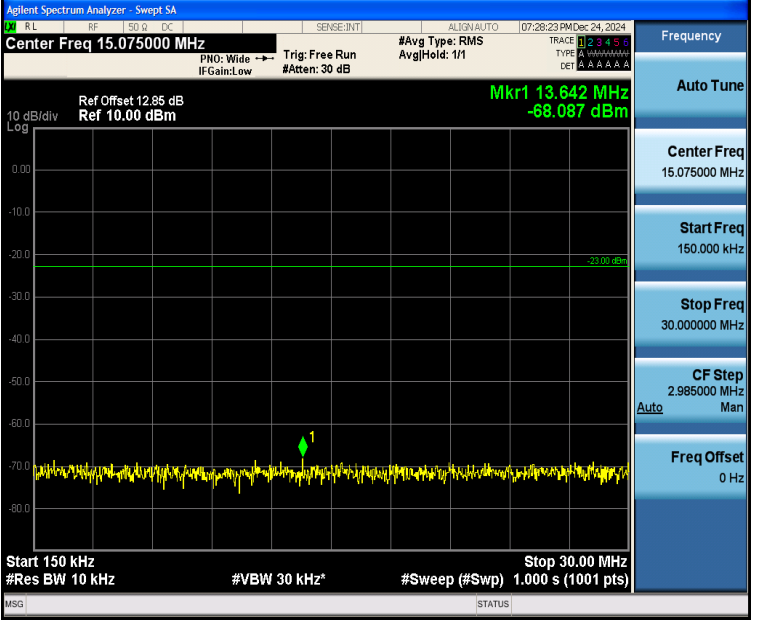
Band5_10MHz_QPSK_20525_1RB#0_0.15~30_0.15~30
