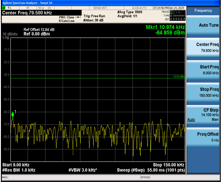
Band5_10MHz_16QAM_20450_1RB#0_0.009~0.15_0.009~0.15
