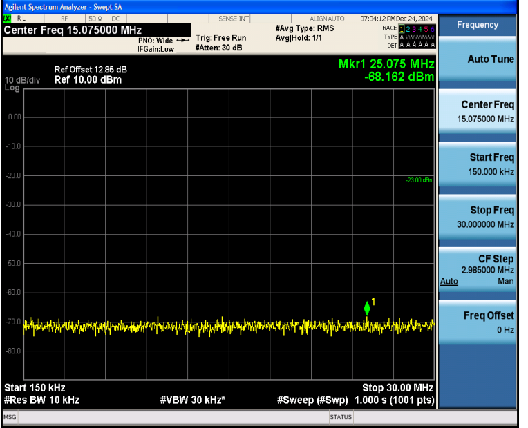
Band5_5MHz_QPSK_20625_1RB#24_0.15~30_0.15~30
