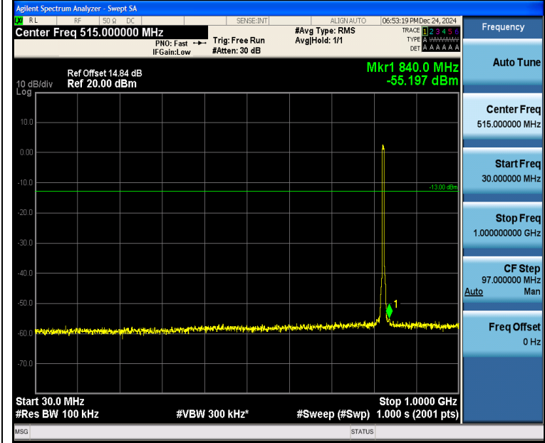
Band5_5MHz_QPSK_20425_25RB#0_30~1000_30~1000
