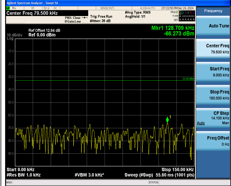
Band5_10MHz_QPSK_20450_1RB#0_0.009~0.15_0.009~0.15
