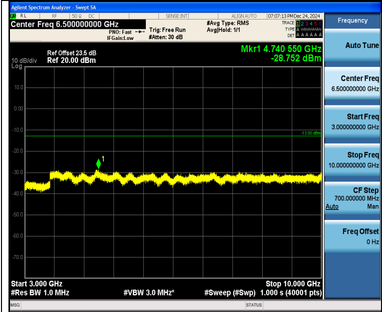
Band5_5MHz_QPSK_20625_25RB#0_3000~10000_3000~10000
