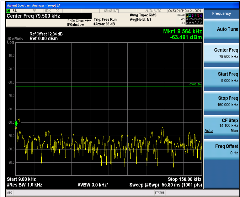
Band5_5MHz_QPSK_20425_25RB#0_0.009~0.15_0.009~0.15
