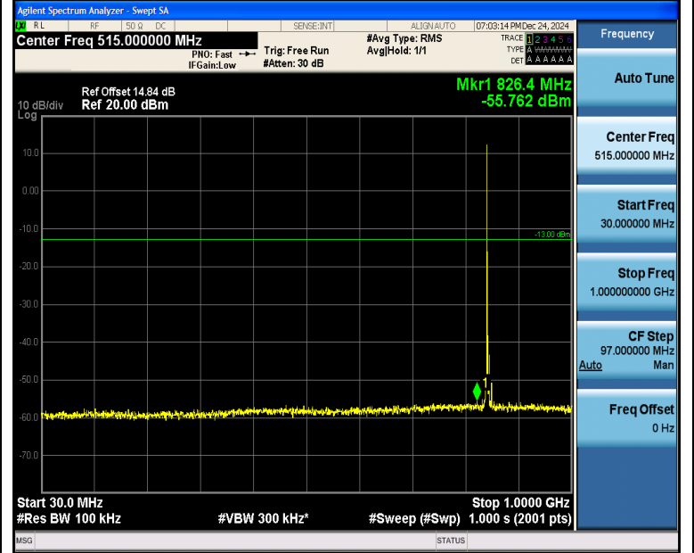
Band5_5MHz_16QAM_20625_1RB#0_30~1000_30~1000
