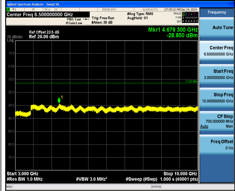
Band5_5MHz_QPSK_20625_1RB#24_3000~10000_3000~10000
