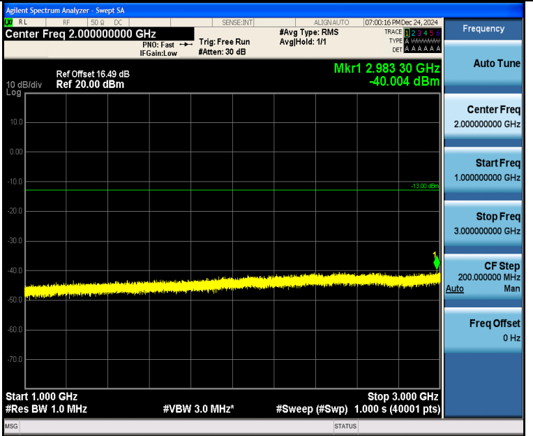
Band5_5MHz_QPSK_20525_25RB#0_1000~3000_1000~3000
