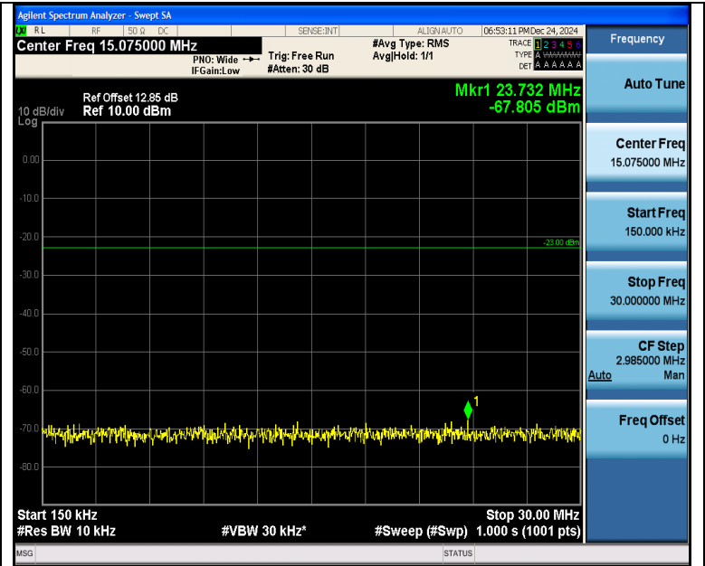
Band5_5MHz_QPSK_20425_25RB#0_0.15~30_0.15~30
