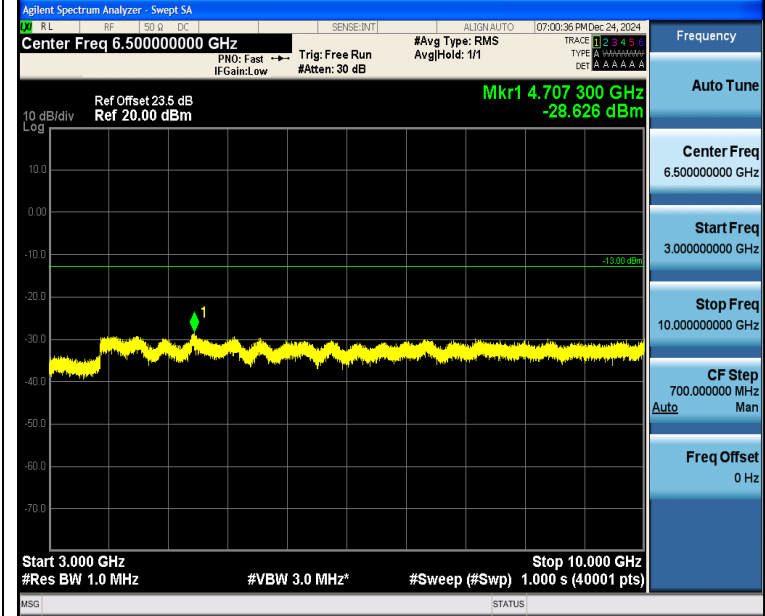
Band5_5MHz_QPSK_20525_25RB#0_3000~10000_3000~10000
