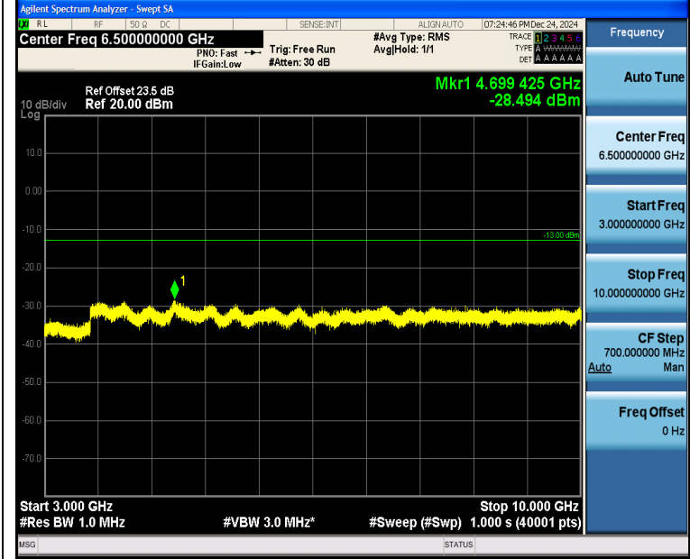
Band5_10MHz_QPSK_20450_1RB#0_3000~10000_3000~10000
