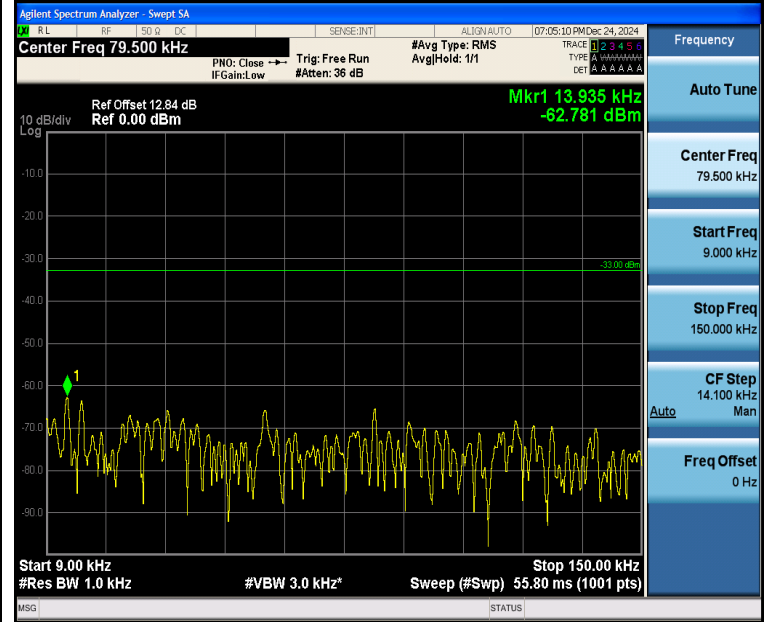
Band5_5MHz_16QAM_20625_1RB#24_0.009~0.15_0.009~0.15
