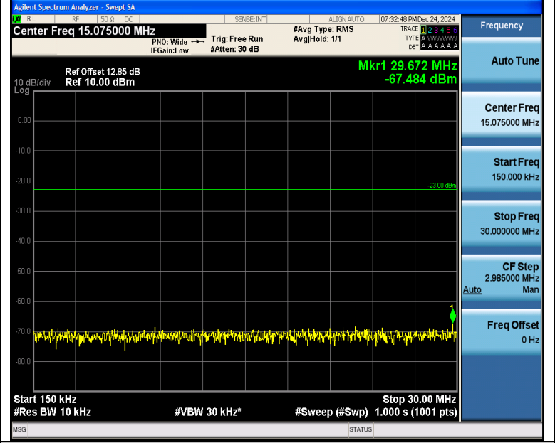
Band5_10MHz_QPSK_20600_1RB#0_0.15~30_0.15~30
