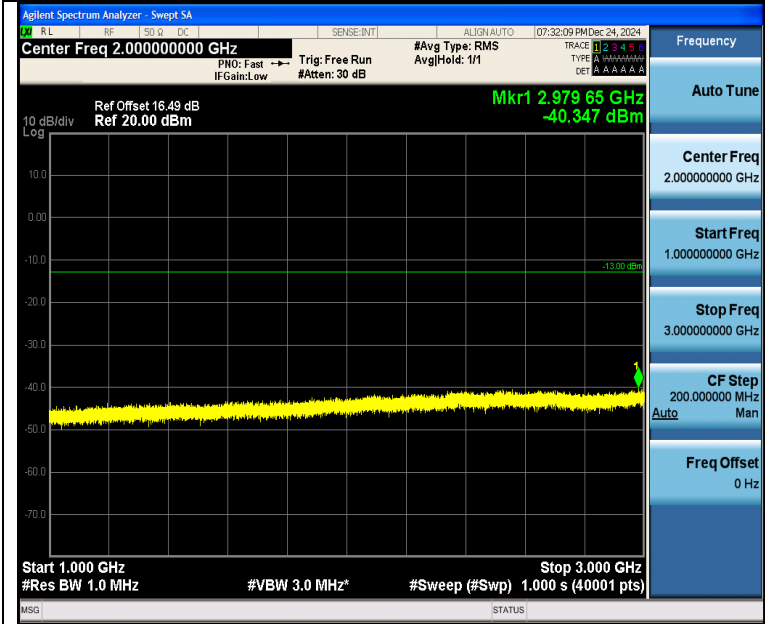
Band5_10MHz_16QAM_20525_1RB#49_1000~3000_1000~3000
