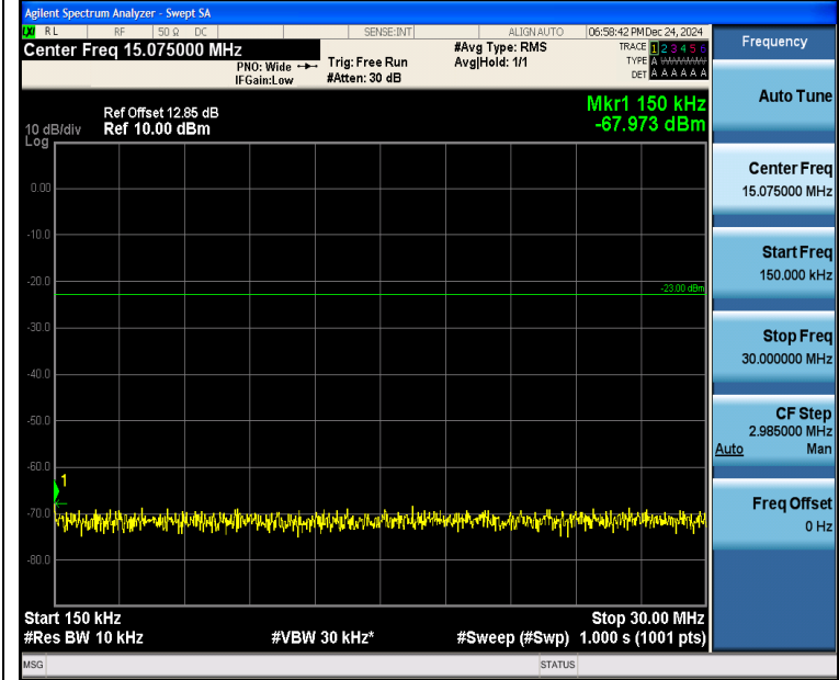
Band5_5MHz_16QAM_20525_1RB#24_0.15~30_0.15~30
