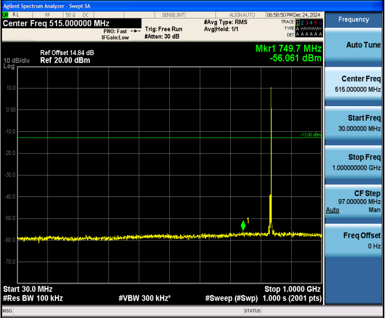
Band5_5MHz_16QAM_20525_1RB#24_30~1000_30~1000
