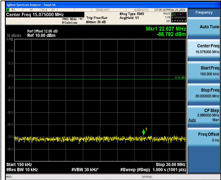
Band5_5MHz_16QAM_20625_1RB#24_0.15~30_0.15~30
