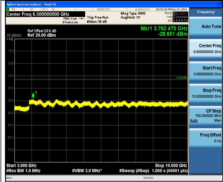
Band5_5MHz_QPSK_20425_25RB#0_3000~10000_3000~10000
