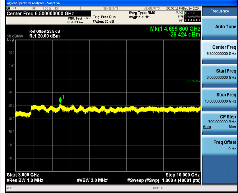
Band5_5MHz_QPSK_20525_1RB#0_3000~10000_3000~10000
