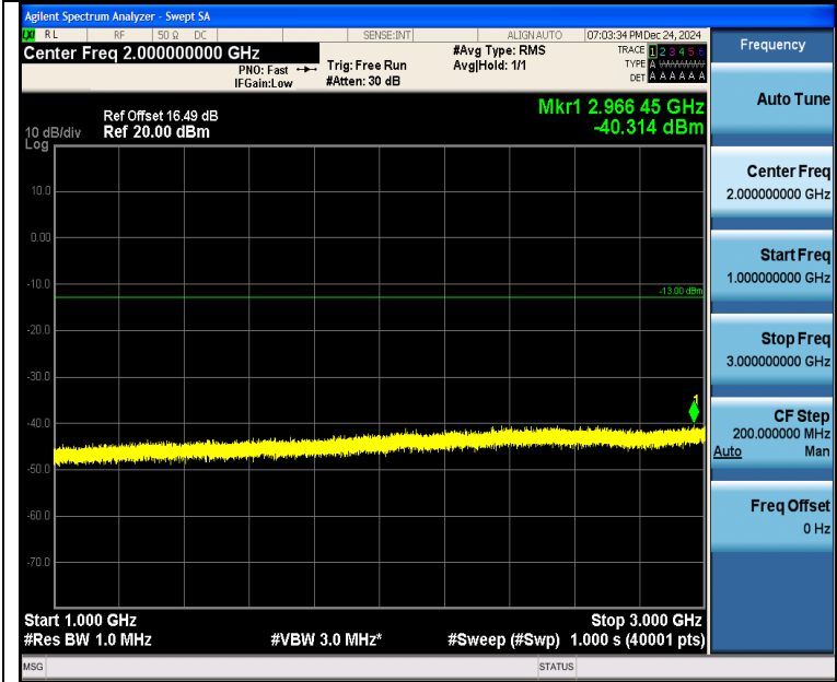
Band5_5MHz_16QAM_20625_1RB#0_1000~3000_1000~3000
