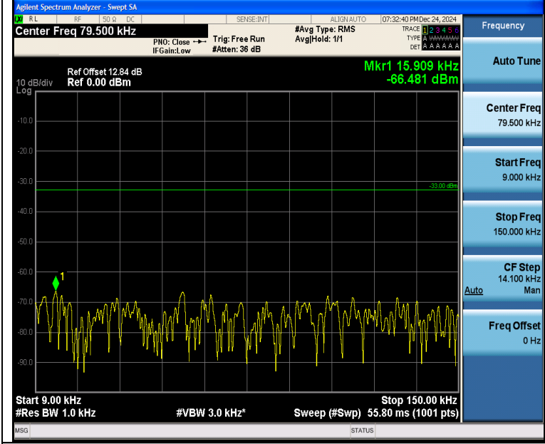
Band5_10MHz_QPSK_20600_1RB#0_0.009~0.15_0.009~0.15
