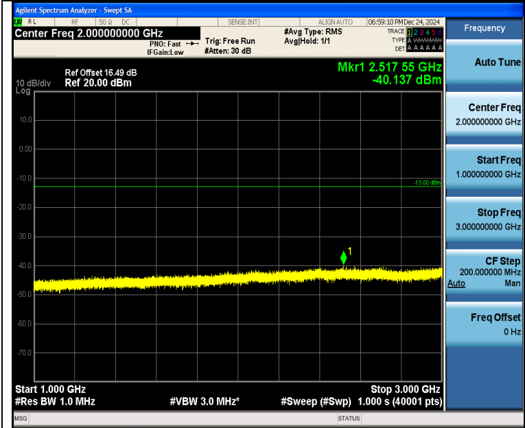
Band5_5MHz_16QAM_20525_1RB#24_1000~3000_1000~3000
