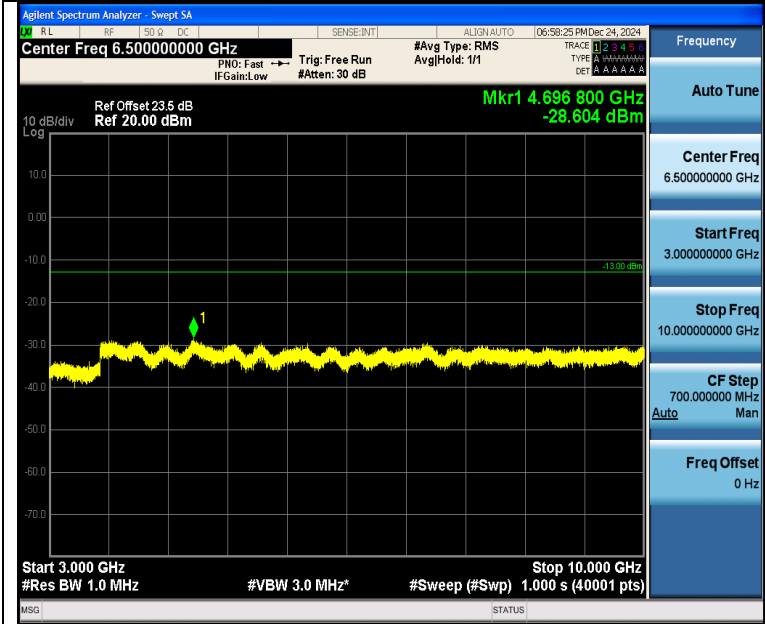
Band5_5MHz_QPSK_20525_1RB#24_3000~10000_3000~10000
