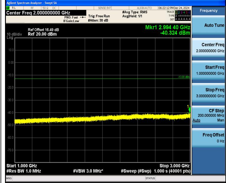
Band5_3MHz_16QAM_20525_1RB#14_1000~3000_1000~3000
