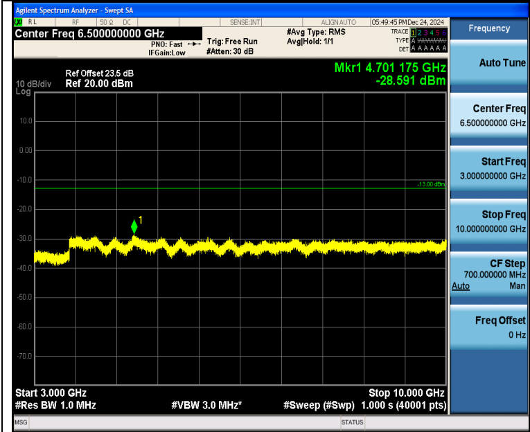
Band5_1.4MHz_QPSK_20643_6RB#0_3000~10000_3000~10000
