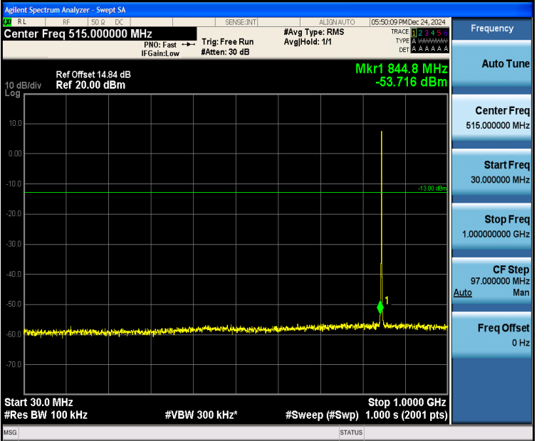
Band5_1.4MHz_16QAM_20643_6RB#0_30~1000_30~1000
