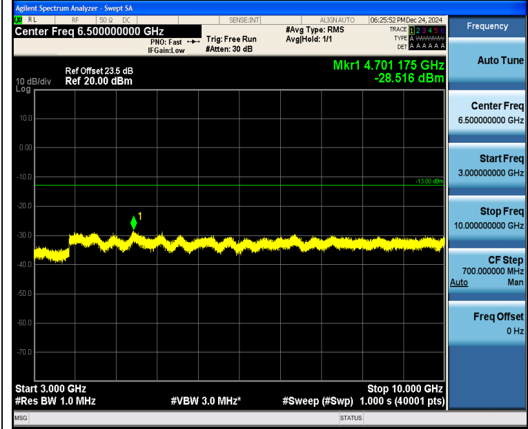
Band5_3MHz_QPSK_20635_1RB#0_3000~10000_3000~10000
