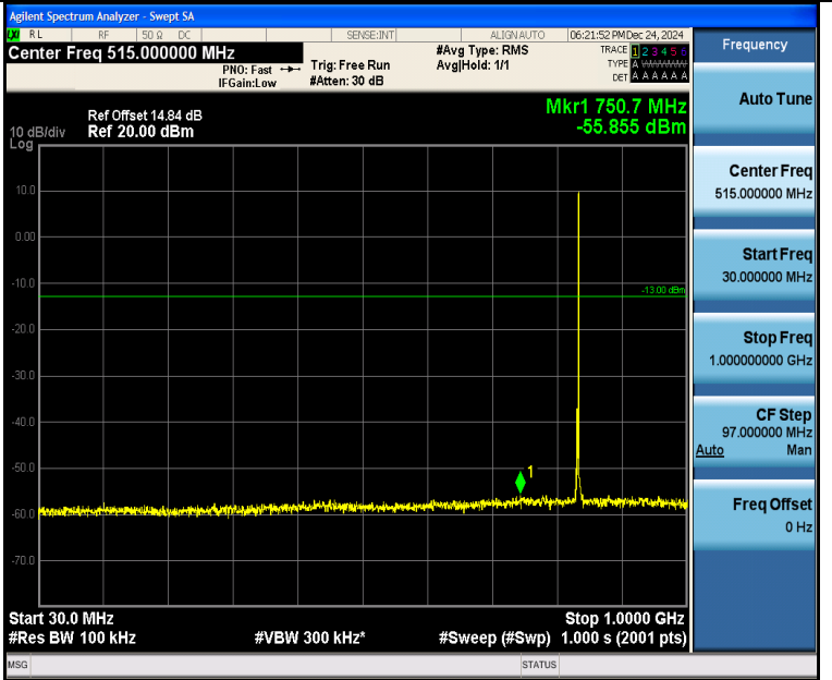
Band5_3MHz_16QAM_20525_1RB#14_30~1000_30~1000
