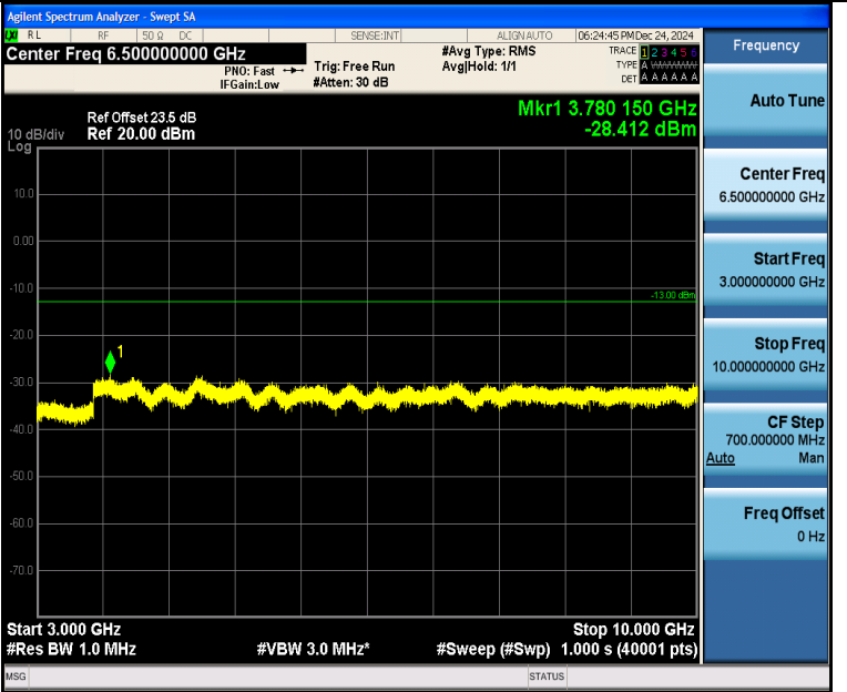
Band5_3MHz_16QAM_20525_15RB#0_3000~10000_3000~10000
