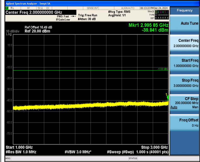
Band5_3MHz_16QAM_20415_1RB#0_1000~3000_1000~3000
