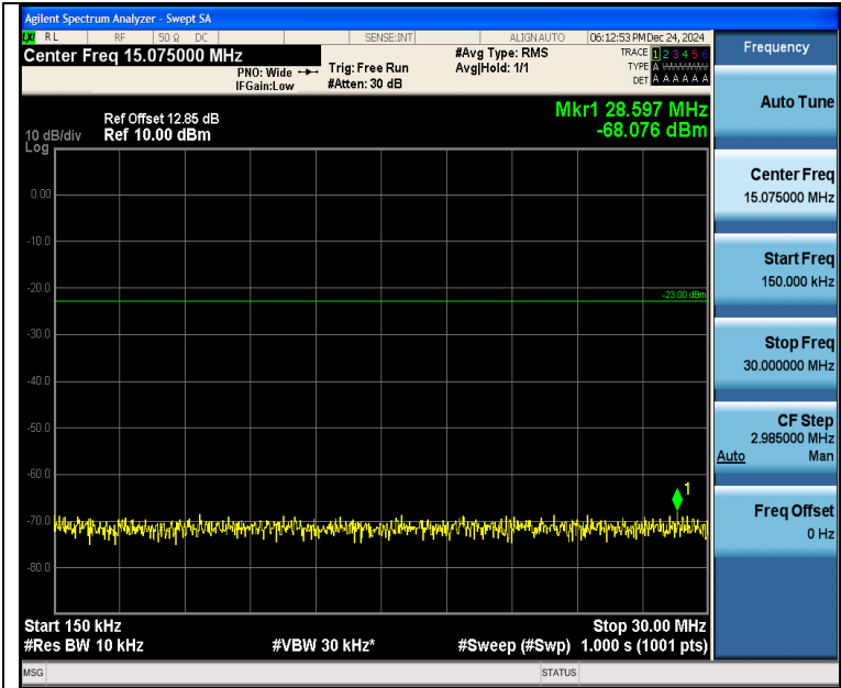
Band5_3MHz_16QAM_20415_1RB#0_0.15~30_0.15~30
