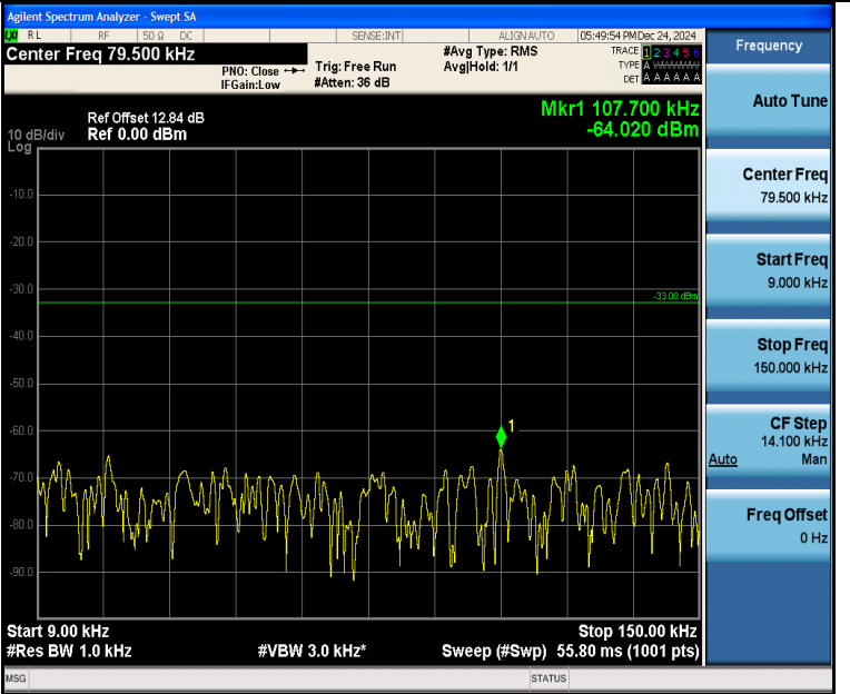
Band5_1.4MHz_16QAM_20643_6RB#0_0.009~0.15_0.009~0.15
