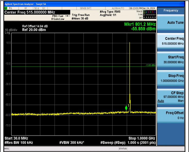
Band5_3MHz_16QAM_20415_1RB#0_30~1000_30~1000
