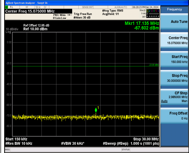
Band5_3MHz_16QAM_20635_1RB#14_0.15~30_0.15~30
