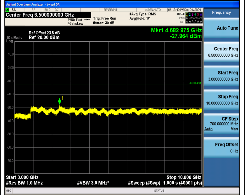
Band5_3MHz_16QAM_20415_1RB#0_3000~10000_3000~10000
