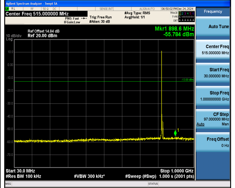
Band5_5MHz_16QAM_20425_1RB#0_30~1000_30~1000
