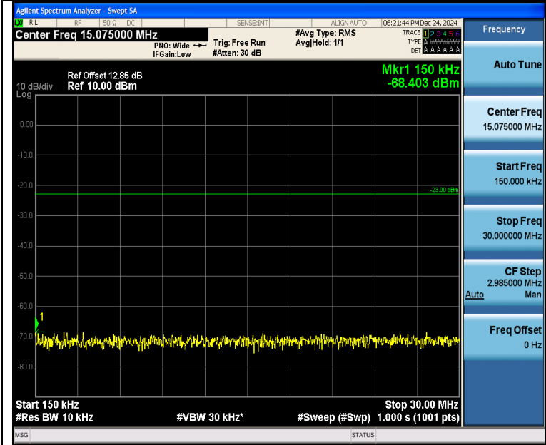
Band5_3MHz_16QAM_20525_1RB#14_0.15~30_0.15~30
