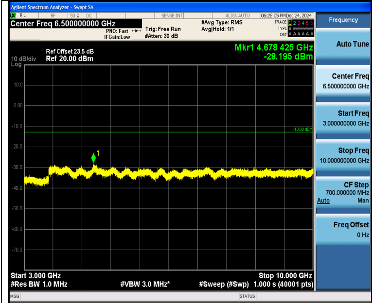
Band5_3MHz_QPSK_20635_1RB#14_3000~10000_3000~10000
