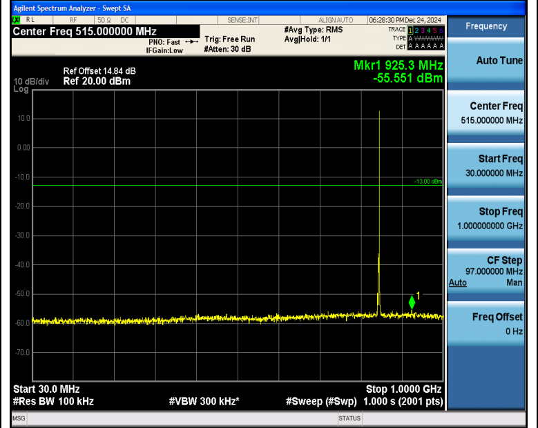
Band5_3MHz_16QAM_20635_1RB#14_30~1000_30~1000
