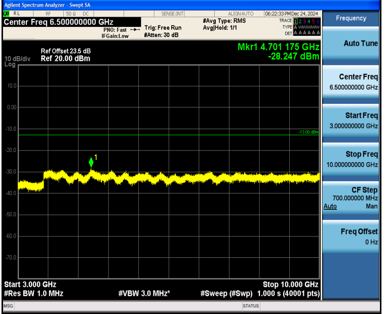
Band5_3MHz_16QAM_20525_1RB#14_3000~10000_3000~10000
