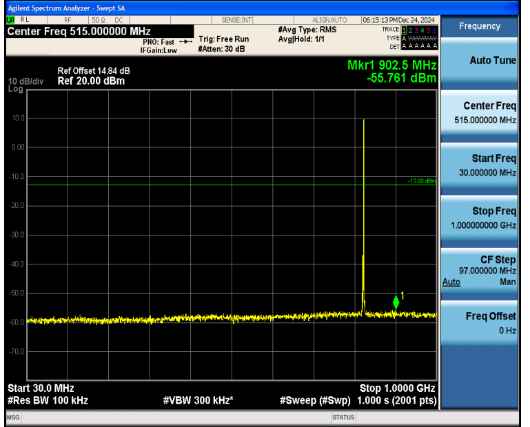
Band5_3MHz_16QAM_20415_1RB#14_30~1000_30~1000
