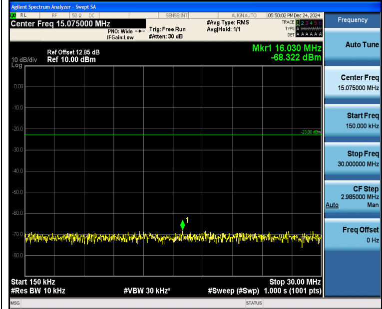
Band5_1.4MHz_16QAM_20643_6RB#0_0.15~30_0.15~30
