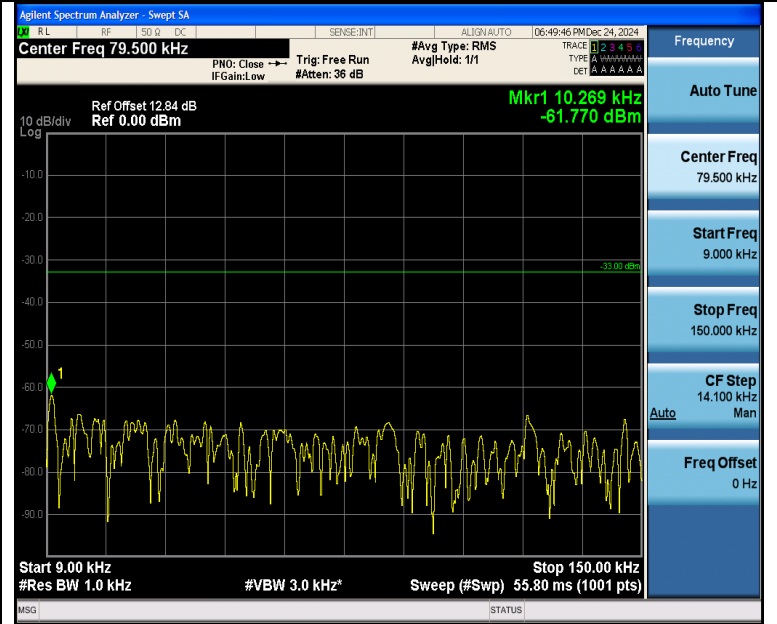
Band5_5MHz_16QAM_20425_1RB#0_0.009~0.15_0.009~0.15
