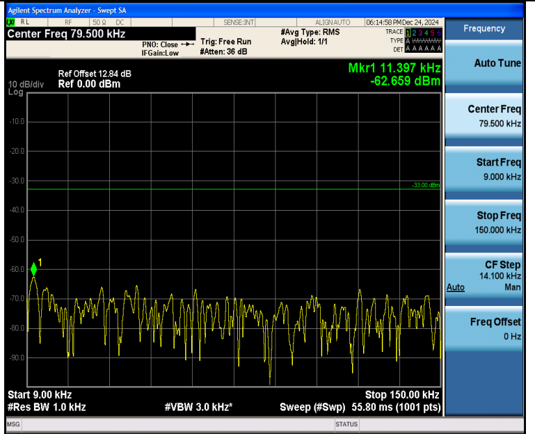
Band5_3MHz_16QAM_20415_1RB#14_0.009~0.15_0.009~0.15
