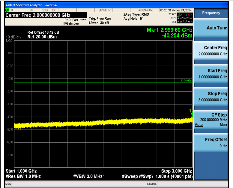
Band5_3MHz_QPSK_20635_1RB#0_1000~3000_1000~3000
