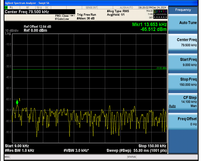
Band5_3MHz_16QAM_20635_1RB#0_0.009~0.15_0.009~0.15
