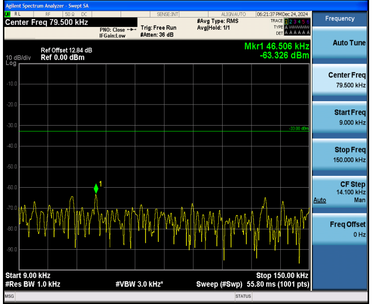
Band5_3MHz_16QAM_20525_1RB#14_0.009~0.15_0.009~0.15
