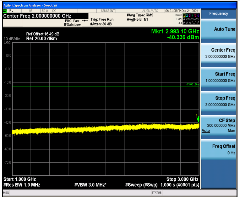
Band5_3MHz_QPSK_20525_1RB#14_1000~3000_1000~3000
