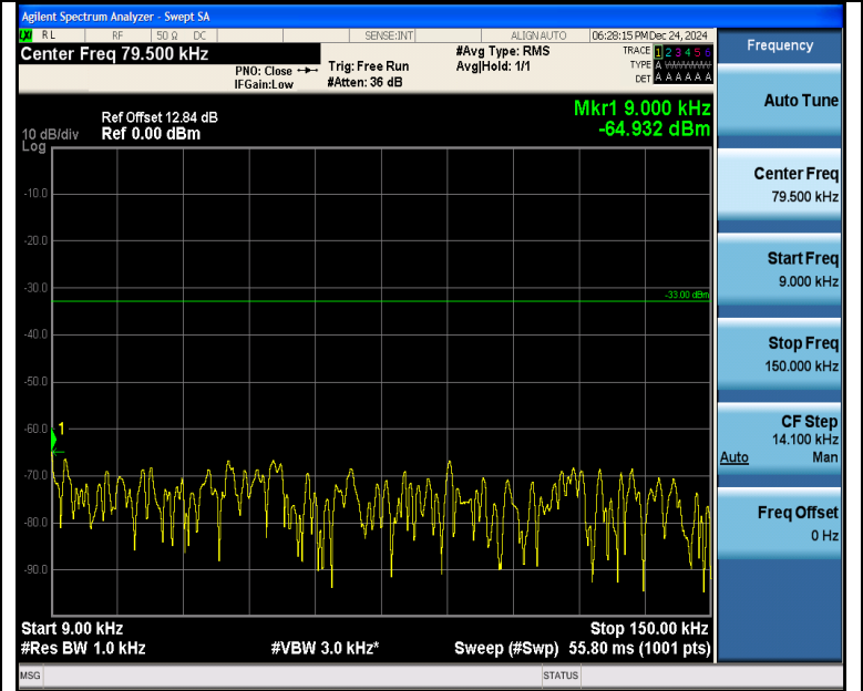
Band5_3MHz_16QAM_20635_1RB#14_0.009~0.15_0.009~0.15
