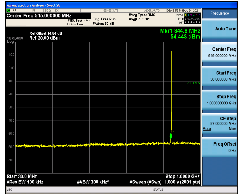
Band5_1.4MHz_QPSK_20643_1RB#5_30~1000_30~1000
