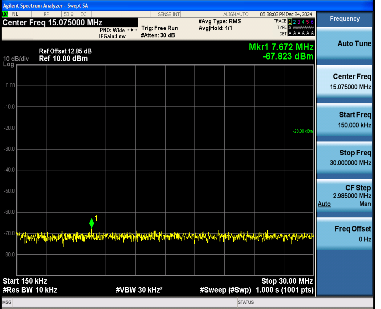
Band5_1.4MHz_QPSK_20525_1RB#0_0.15~30_0.15~30
