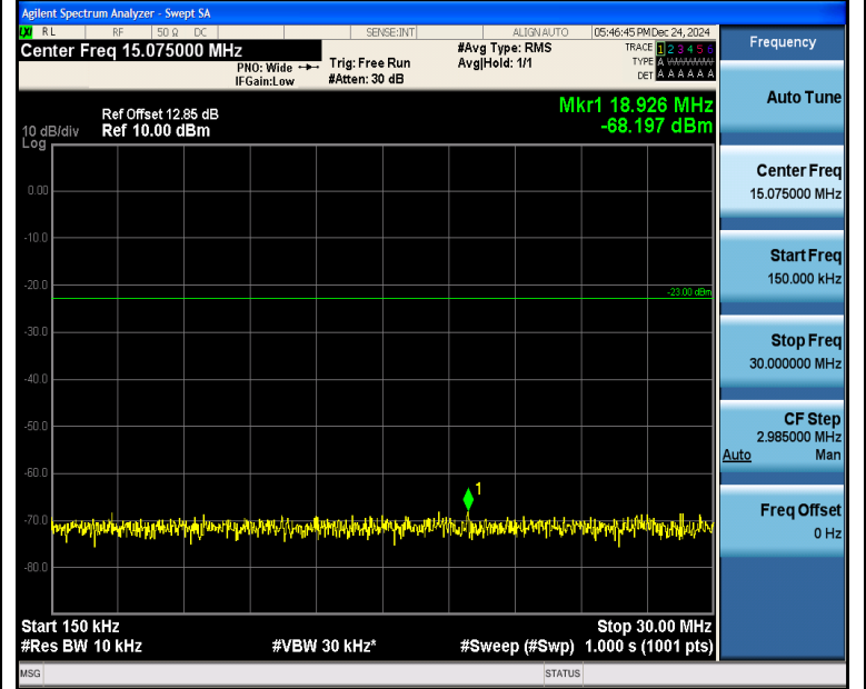
Band5_1.4MHz_QPSK_20643_1RB#5_0.15~30_0.15~30
