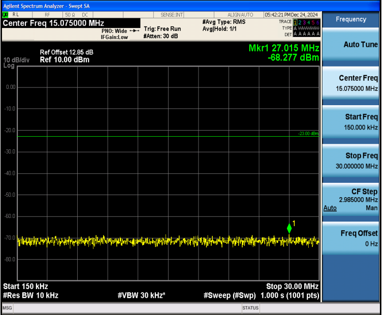
Band5_1.4MHz_QPSK_20525_6RB#0_0.15~30_0.15~30
