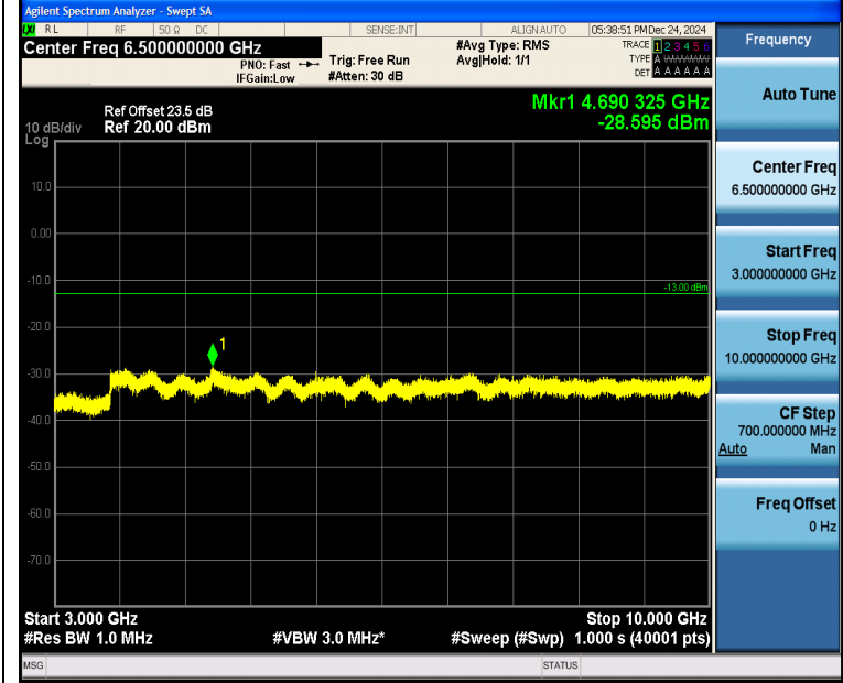
Band5_1.4MHz_QPSK_20525_1RB#0_3000~10000_3000~10000
