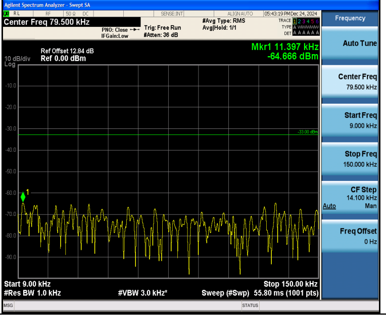
Band5_1.4MHz_16QAM_20525_6RB#0_0.009~0.15_0.009~0.15
