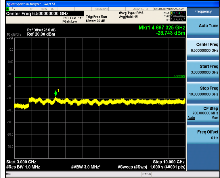
Band5_1.4MHz_QPSK_20407_1RB#5_3000~10000_3000~10000
