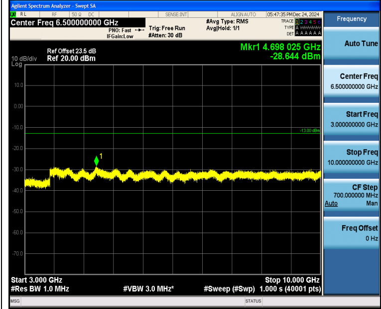
Band5_1.4MHz_QPSK_20643_1RB#5_3000~10000_3000~10000
