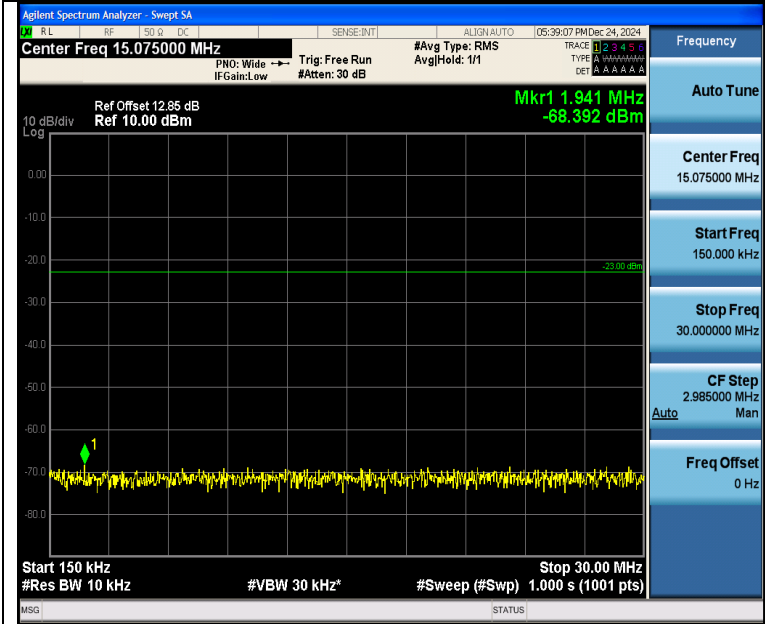
Band5_1.4MHz_16QAM_20525_1RB#0_0.15~30_0.15~30
