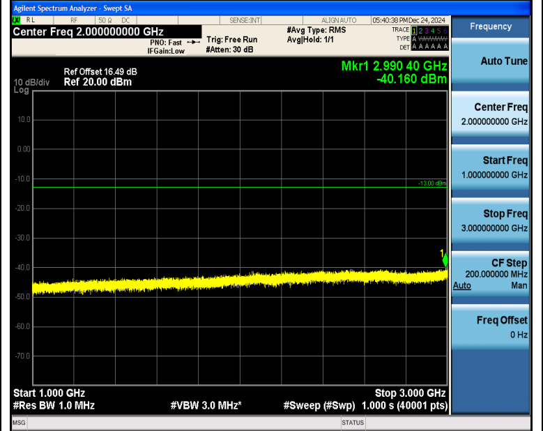
Band5_1.4MHz_QPSK_20525_1RB#5_1000~3000_1000~3000
