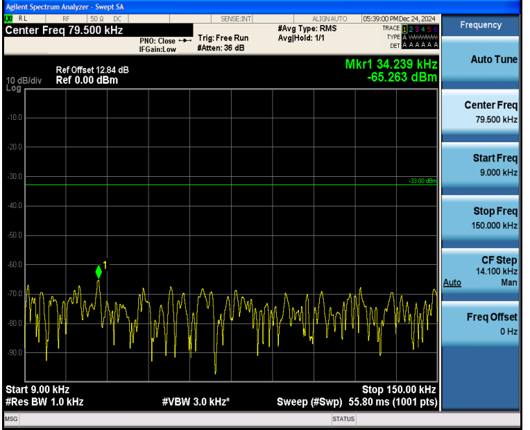
Band5_1.4MHz_16QAM_20525_1RB#0_0.009~0.15_0.009~0.15
