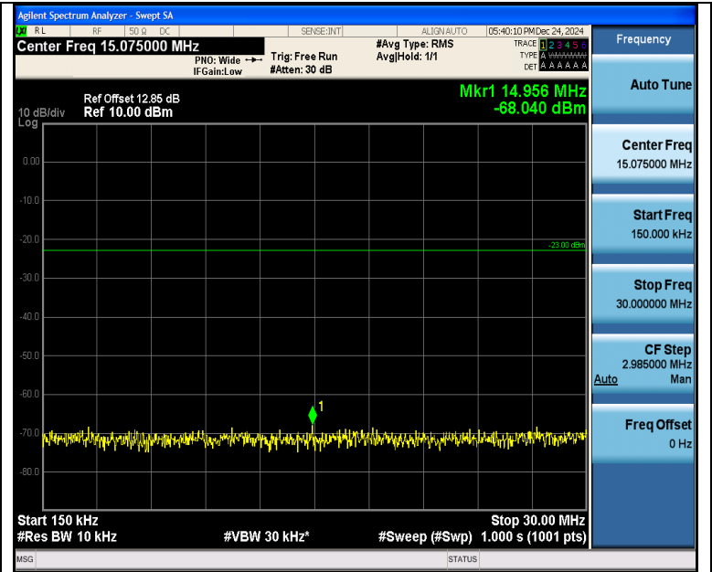
Band5_1.4MHz_QPSK_20525_1RB#5_0.15~30_0.15~30
