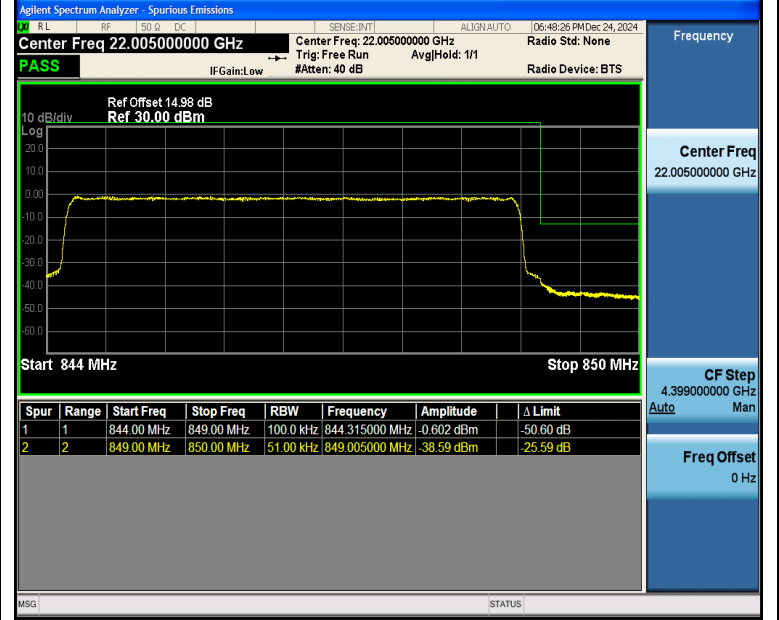
Band5_5MHz_16QAM_20625_25RB#0
