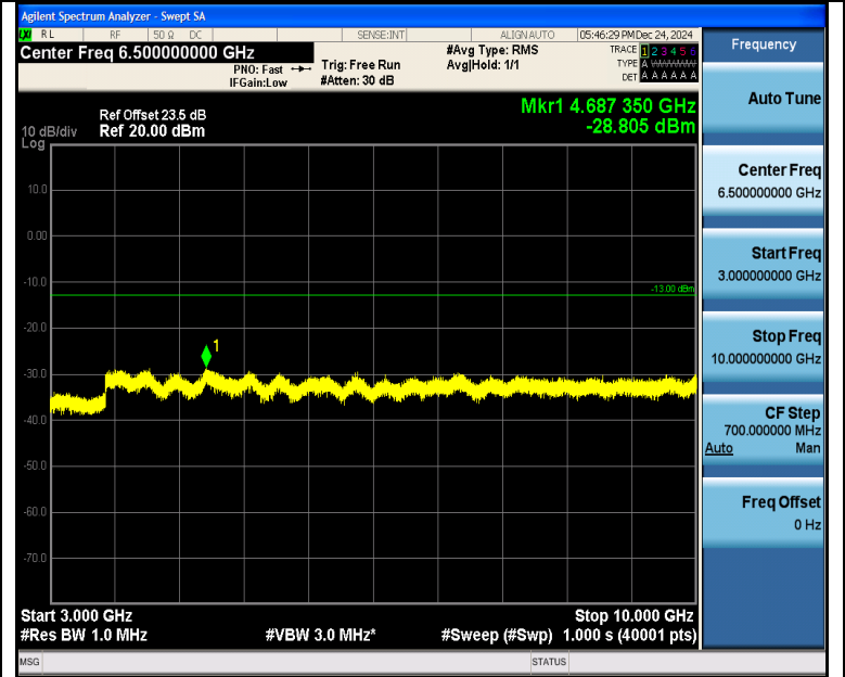
Band5_1.4MHz_16QAM_20643_1RB#0_3000~10000_3000~10000
