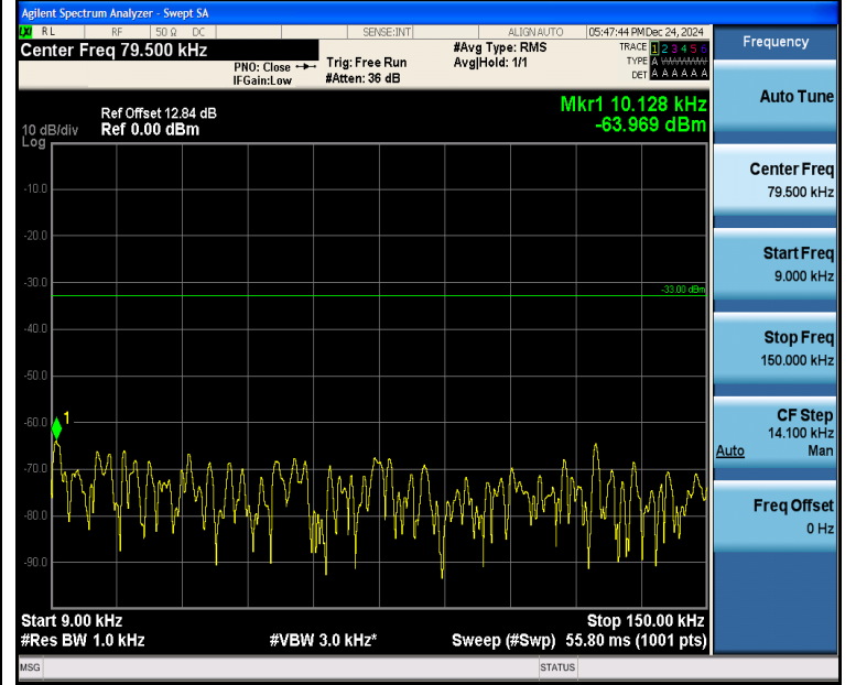
Band5_1.4MHz_16QAM_20643_1RB#5_0.009~0.15_0.009~0.15
