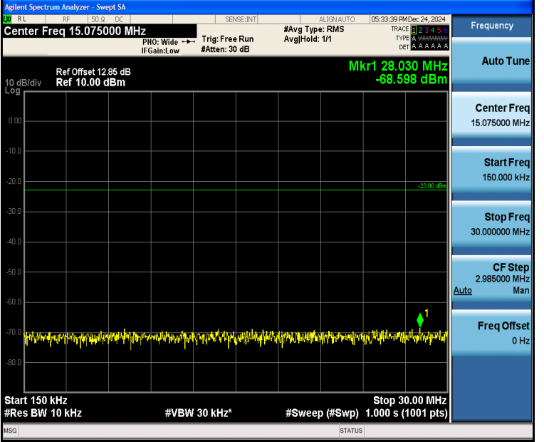
Band5_1.4MHz_QPSK_20407_1RB#5_0.15~30_0.15~30
