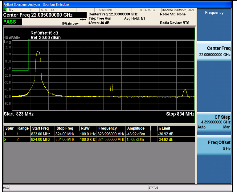
Band5_10MHz_16QAM_20450_1RB#0
