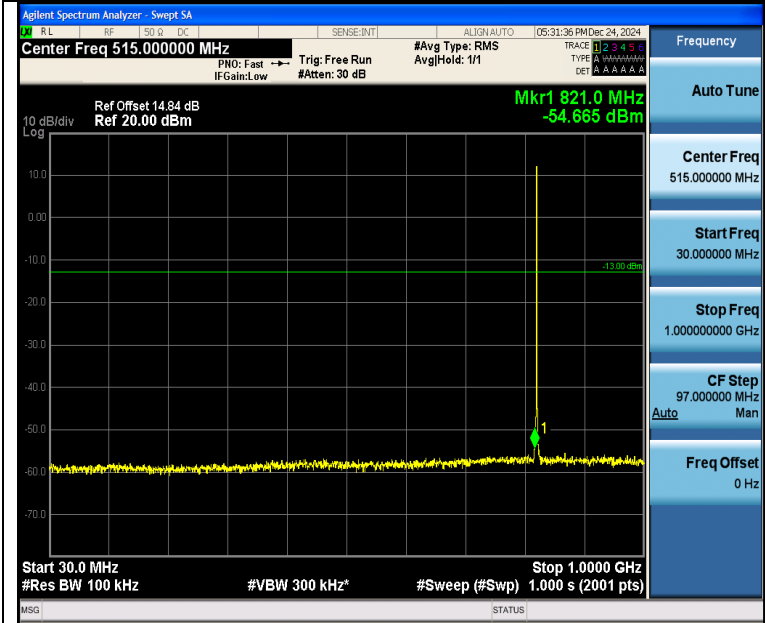
Band5_1.4MHz_QPSK_20407_1RB#0_30~1000_30~1000
