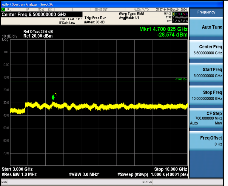
Band5_1.4MHz_16QAM_20407_6RB#0_3000~10000_3000~10000
