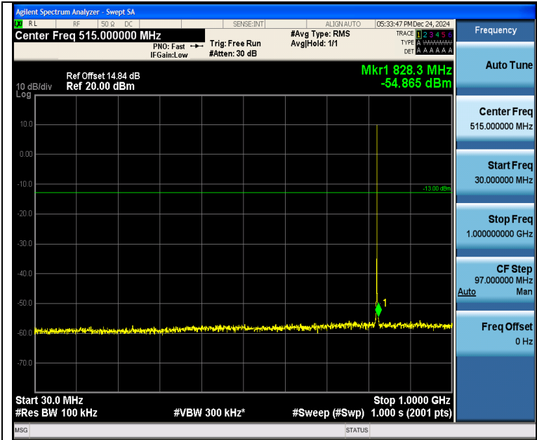
Band5_1.4MHz_QPSK_20407_1RB#5_30~1000_30~1000
