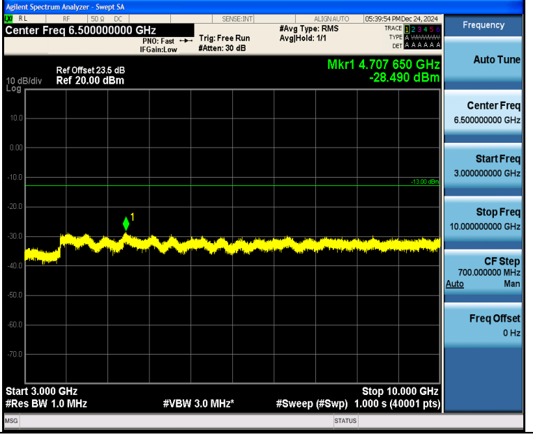
Band5_1.4MHz_16QAM_20525_1RB#0_3000~10000_3000~10000
