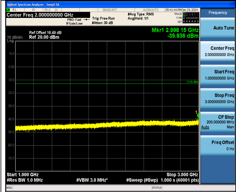
Band5_1.4MHz_16QAM_20525_1RB#5_1000~3000_1000~3000
