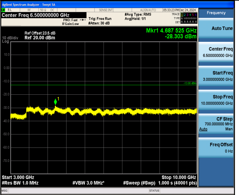
Band5_1.4MHz_16QAM_20407_1RB#0_3000~10000_3000~10000
