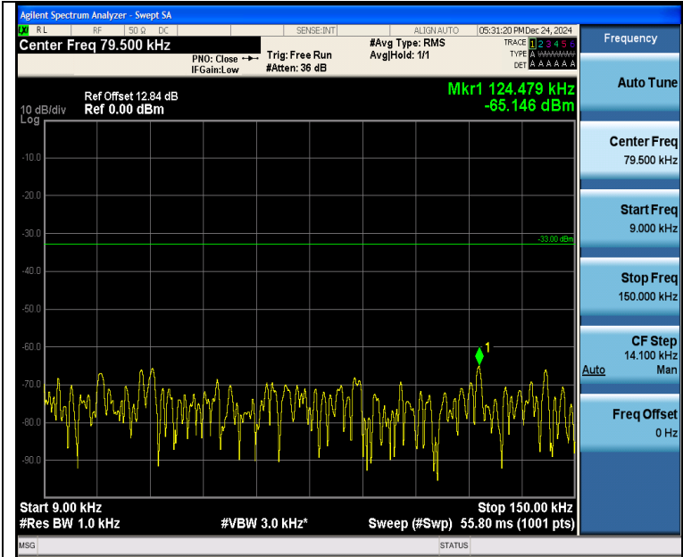
Band5_1.4MHz_QPSK_20407_1RB#0_0.009~0.15_0.009~0.15
