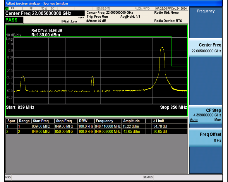
Band5_10MHz_16QAM_20600_1RB#49
