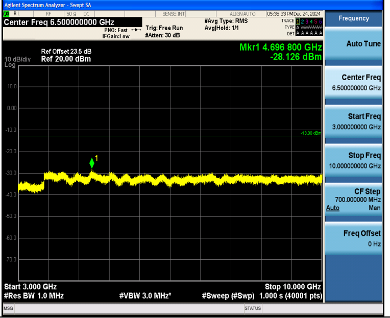
Band5_1.4MHz_16QAM_20407_1RB#5_3000~10000_3000~10000
