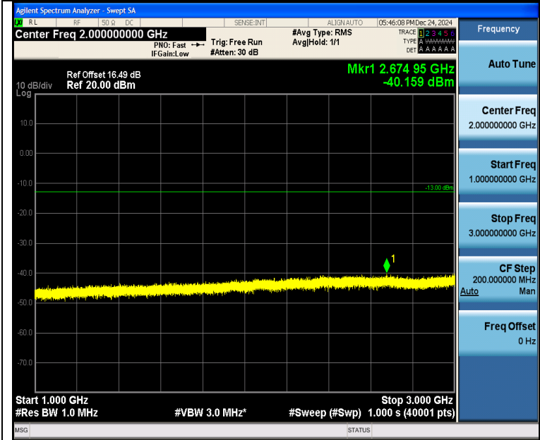
Band5_1.4MHz_16QAM_20643_1RB#0_1000~3000_1000~3000
