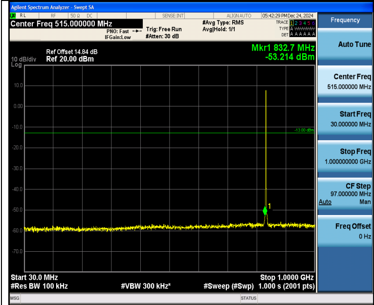
Band5_1.4MHz_QPSK_20525_6RB#0_30~1000_30~1000
