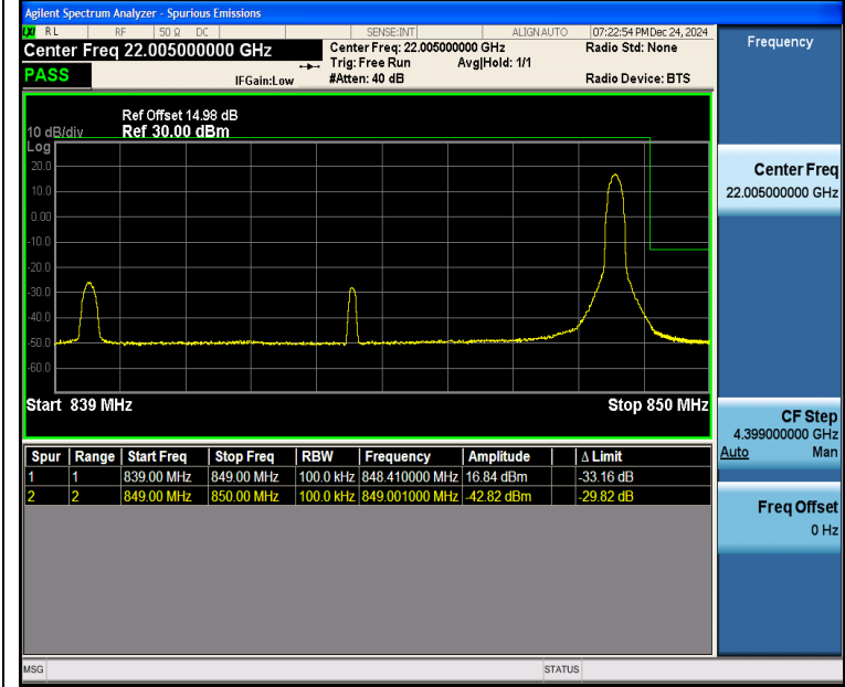
Band5_10MHz_QPSK_20600_1RB#49
