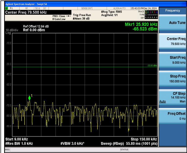
Band5_1.4MHz_QPSK_20525_1RB#5_0.009~0.15_0.009~0.15
