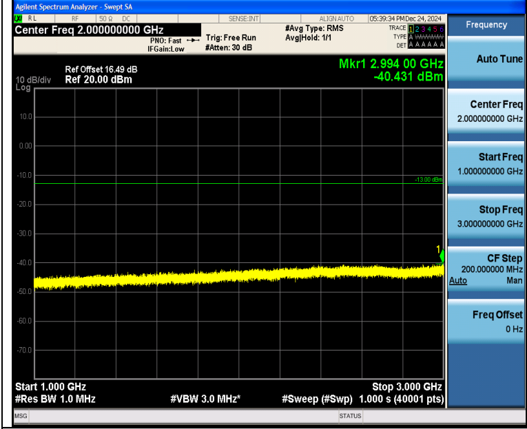
Band5_1.4MHz_16QAM_20525_1RB#0_1000~3000_1000~3000
