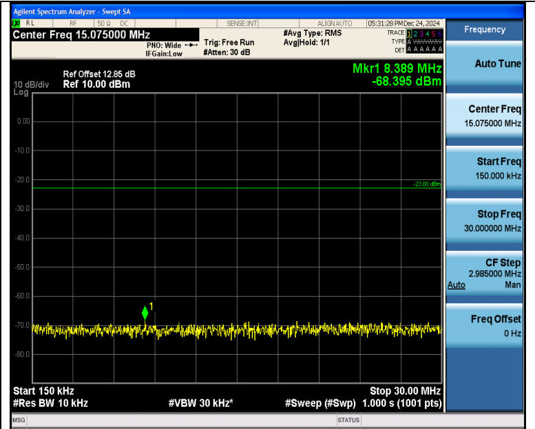
Band5_1.4MHz_QPSK_20407_1RB#0_0.15~30_0.15~30
