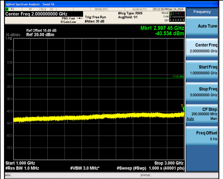
Band5_1.4MHz_QPSK_20407_1RB#0_1000~3000_1000~3000
