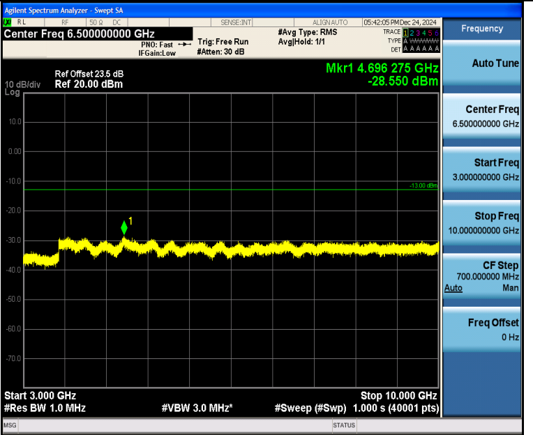
Band5_1.4MHz_16QAM_20525_1RB#5_3000~10000_3000~10000
