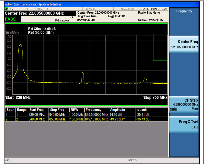
Band5_10MHz_16QAM_20600_1RB#0
