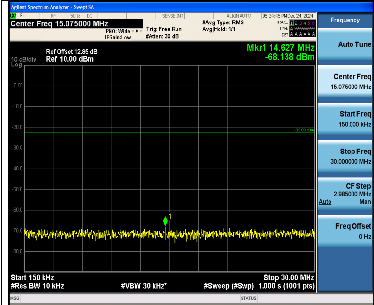
Band5_1.4MHz_16QAM_20407_1RB#5_0.15~30_0.15~30
