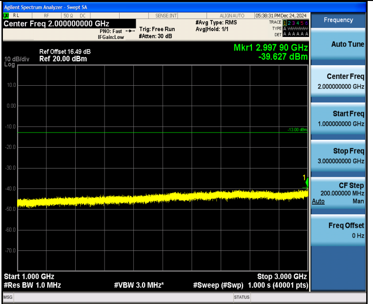
Band5_1.4MHz_QPSK_20525_1RB#0_1000~3000_1000~3000
