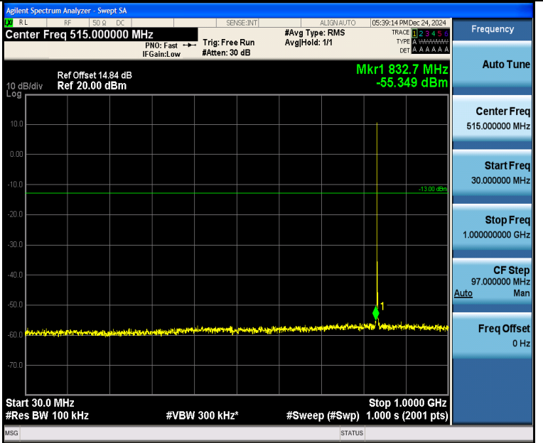
Band5_1.4MHz_16QAM_20525_1RB#0_30~1000_30~1000
