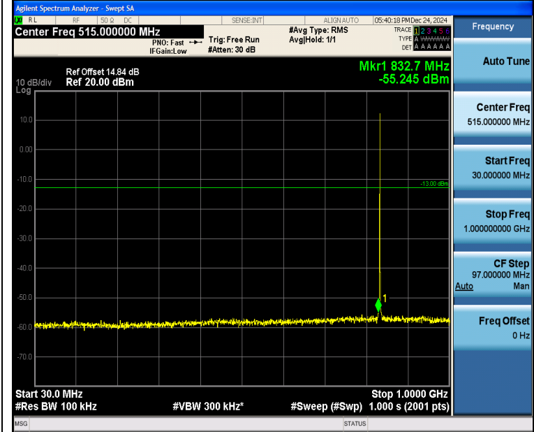
Band5_1.4MHz_QPSK_20525_1RB#5_30~1000_30~1000
