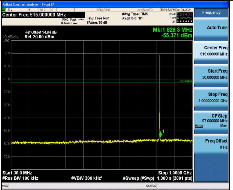
Band5_1.4MHz_16QAM_20407_1RB#5_30~1000_30~1000
