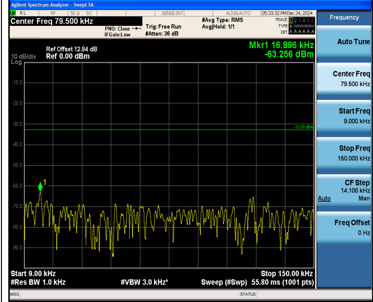
Band5_1.4MHz_QPSK_20407_1RB#5_0.009~0.15_0.009~0.15
