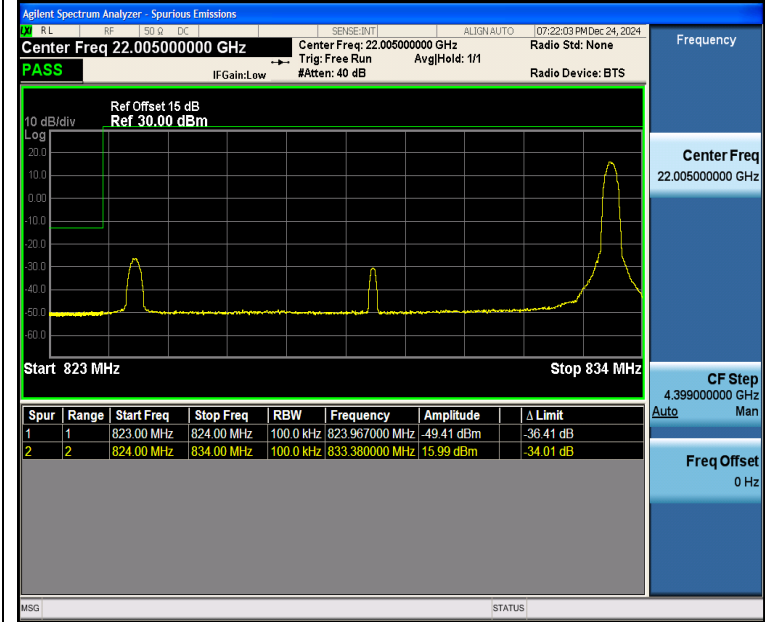
Band5_10MHz_QPSK_20450_1RB#49
