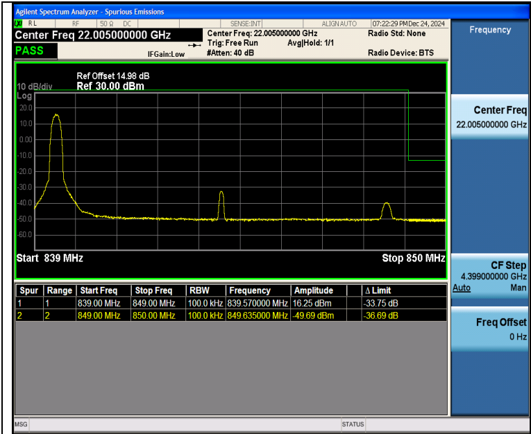
Band5_10MHz_QPSK_20600_1RB#0
