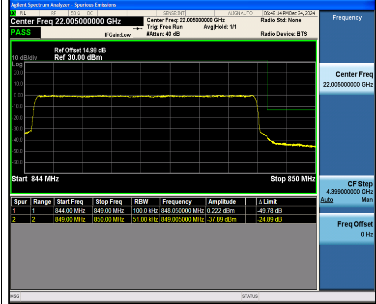
Band5_5MHz_QPSK_20625_25RB#0
