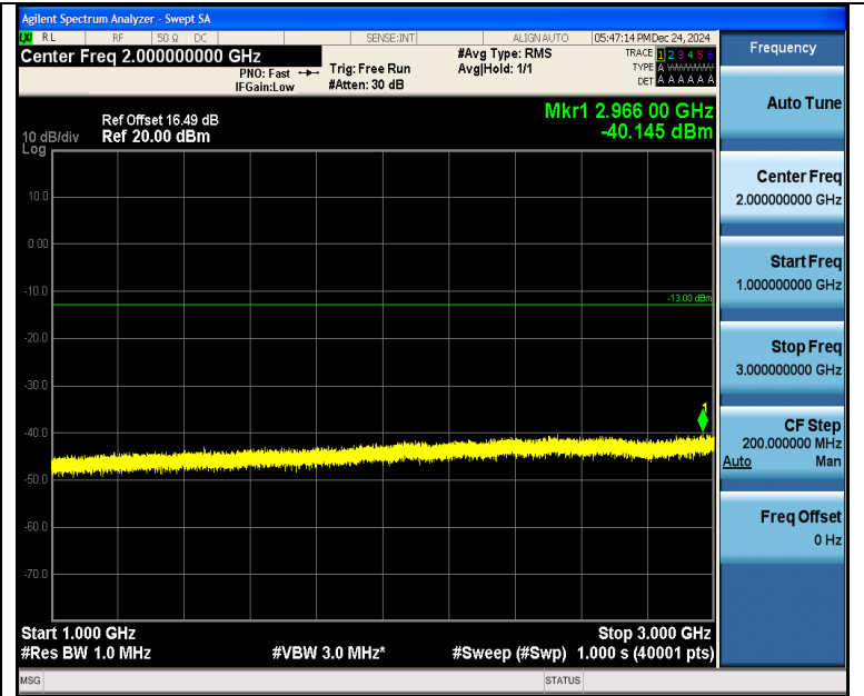
Band5_1.4MHz_QPSK_20643_1RB#5_1000~3000_1000~3000
