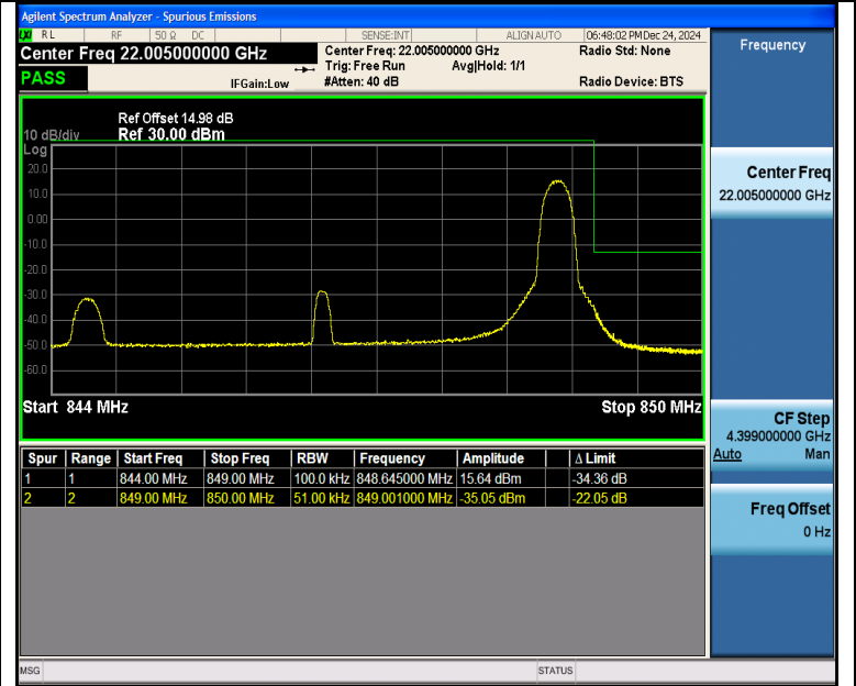
Band5_5MHz_16QAM_20625_1RB#24
