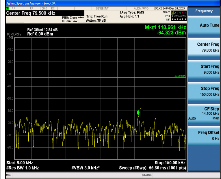
Band5_1.4MHz_QPSK_20525_6RB#0_0.009~0.15_0.009~0.15
