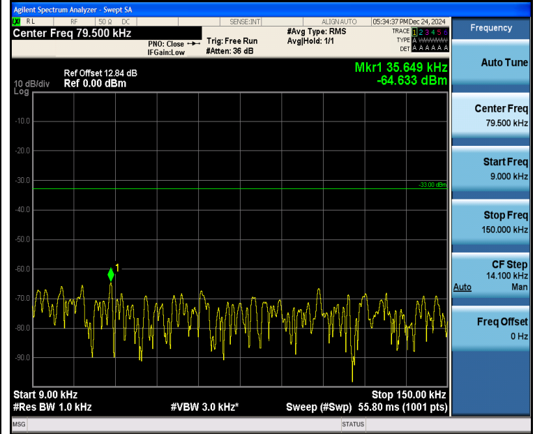
Band5_1.4MHz_16QAM_20407_1RB#5_0.009~0.15_0.009~0.15
