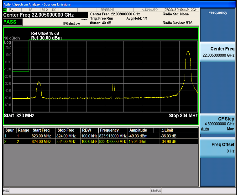
Band5_10MHz_16QAM_20450_1RB#49
