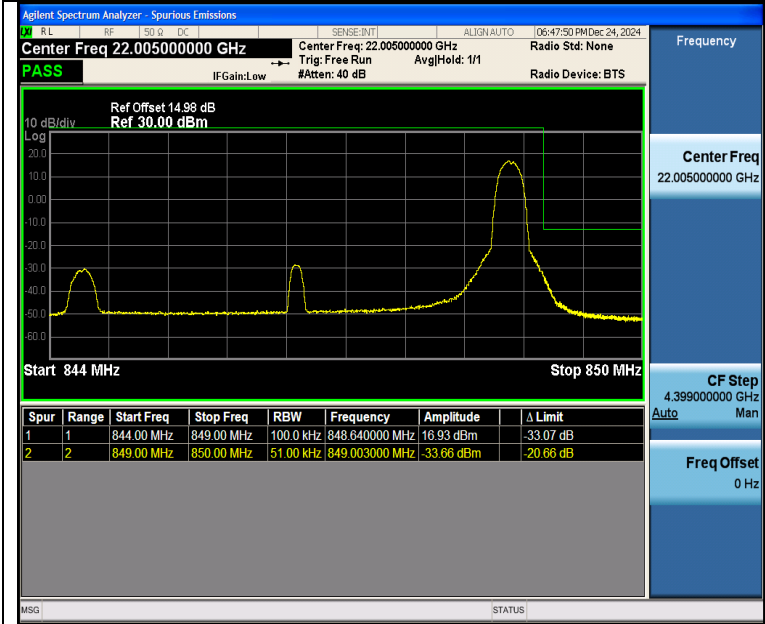
Band5_5MHz_QPSK_20625_1RB#24
