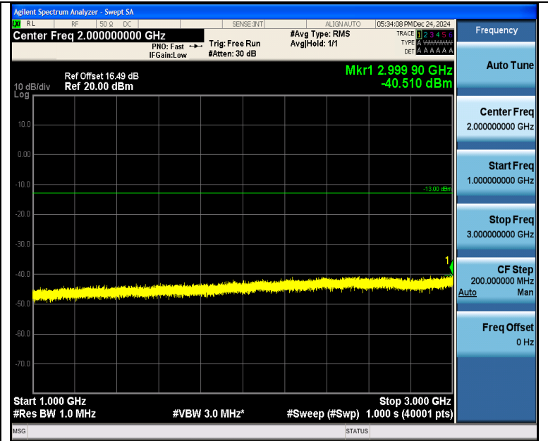
Band5_1.4MHz_QPSK_20407_1RB#5_1000~3000_1000~3000
