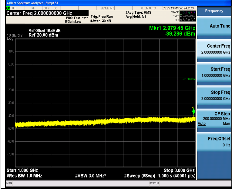
Band5_1.4MHz_16QAM_20407_1RB#5_1000~3000_1000~3000
