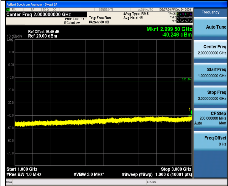
Band5_1.4MHz_16QAM_20407_6RB#0_1000~3000_1000~3000
