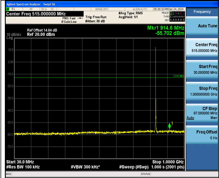
Band5_1.4MHz_QPSK_20525_1RB#0_30~1000_30~1000
