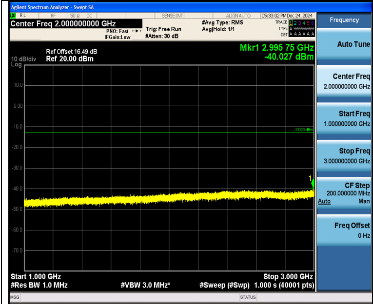
Band5_1.4MHz_16QAM_20407_1RB#0_1000~3000_1000~3000
