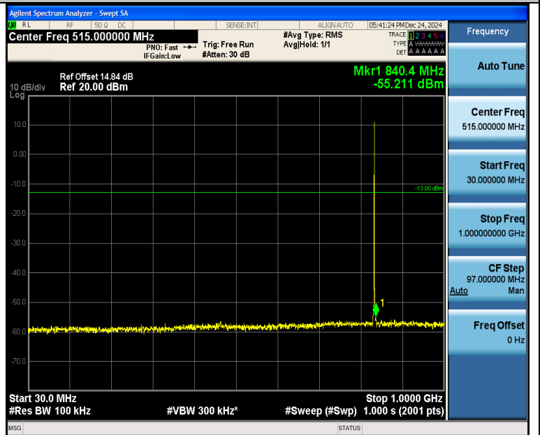
Band5 1.4MHz 16QAM 20525 1RB#5 30~1000 30~1000
