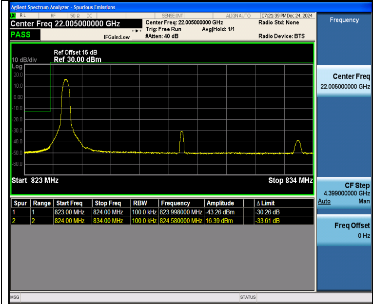
Band5_10MHz_QPSK_20450_1RB#0
