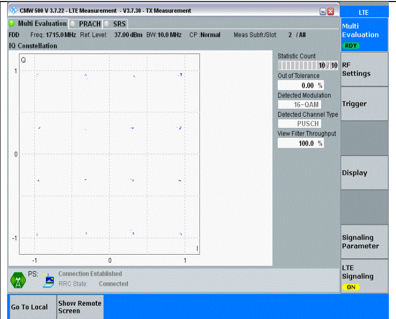
Band4-10MHz-16QAM-20000-1RB#0-PASS
