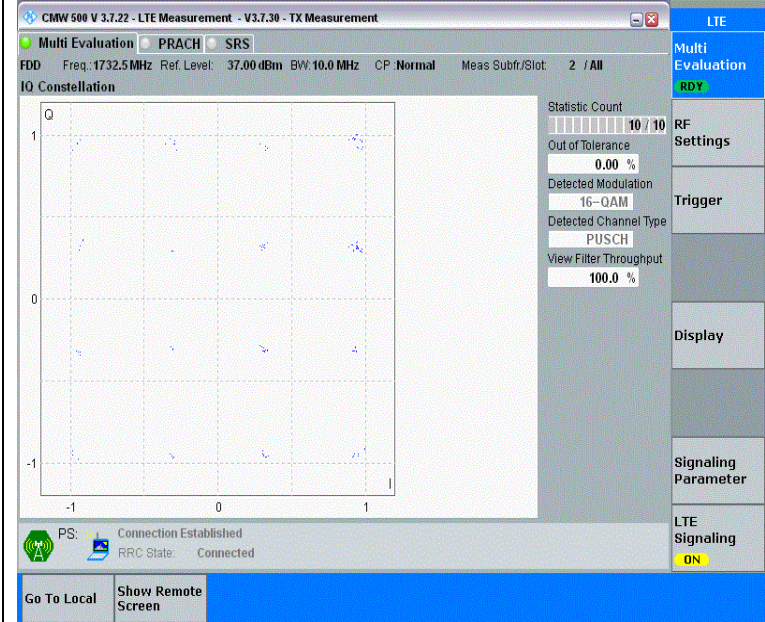
Band4-10MHz-16QAM-20175-1RB#0-PASS
