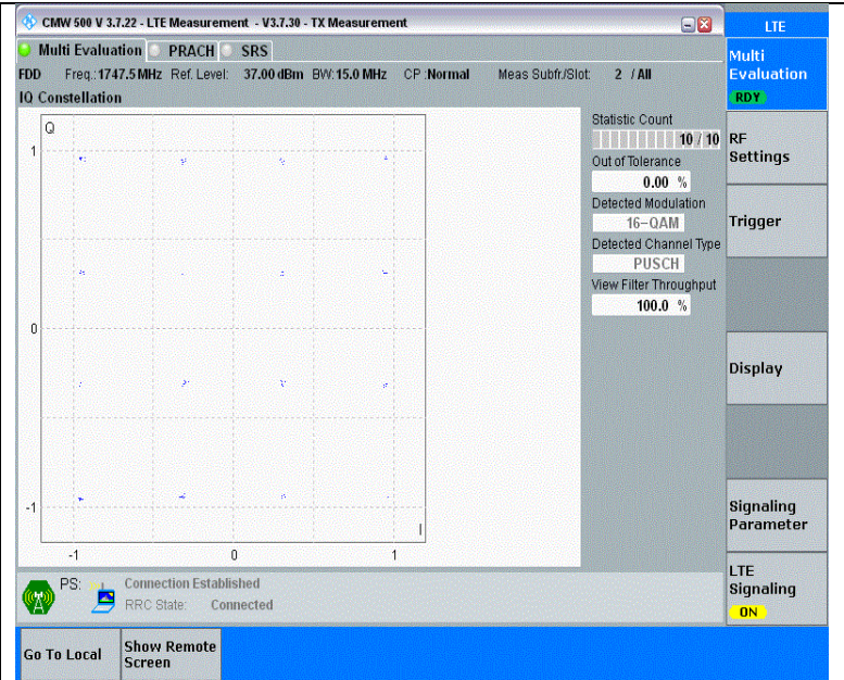
Band4-15MHz-16QAM-20325-1RB#0-PASS
