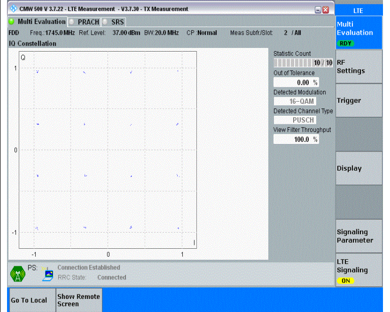
Band4-20MHz-16QAM-20300-1RB#0-PASS
