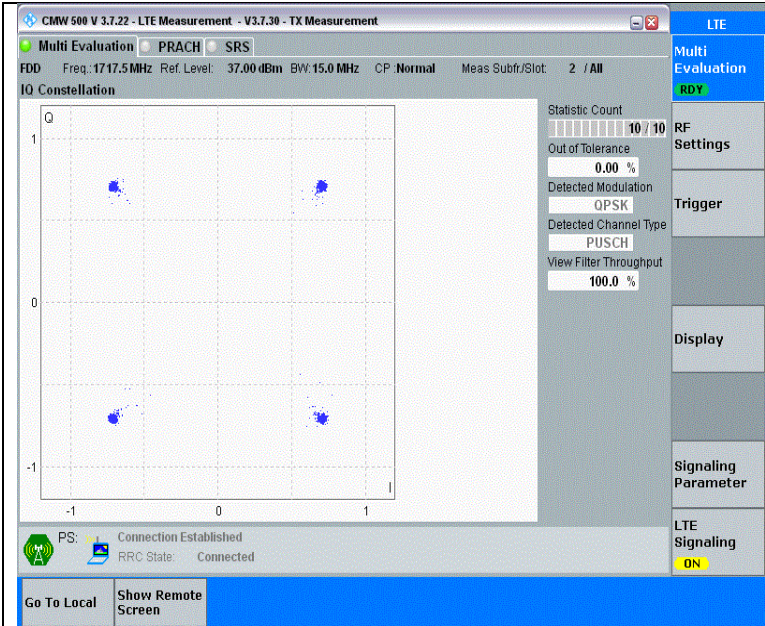
Band4-15MHz-QPSK-20025-75RB#0-PASS
