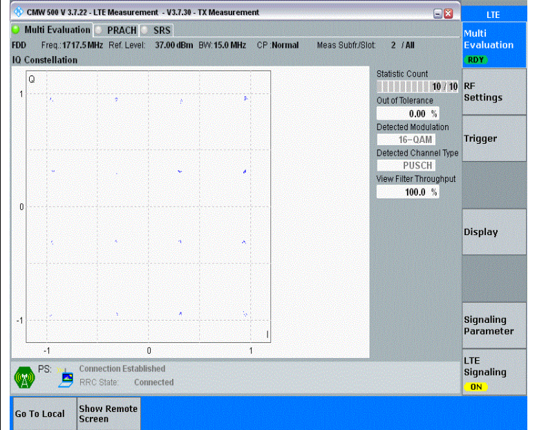
Band4-15MHz-16QAM-20025-1RB#0-PASS
