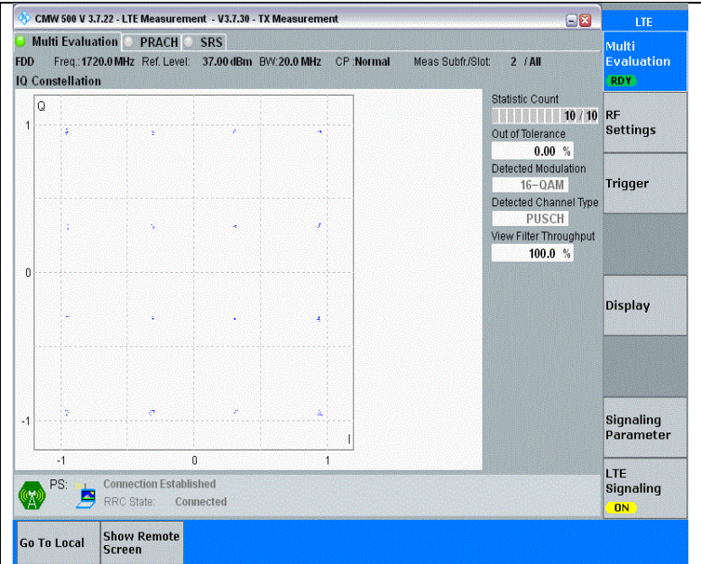
Band4-20MHz-16QAM-20050-1RB#0-PASS
