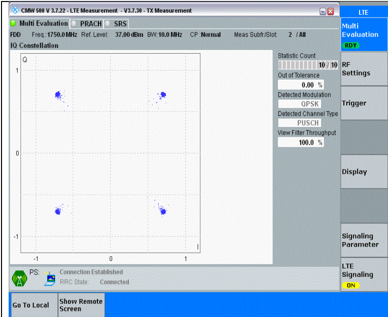
Band4-10MHz-QPSK-20350-50RB#0-PASS
