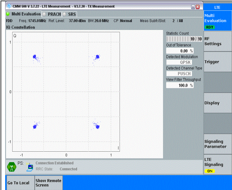
Band4-20MHz-QPSK-20300-100RB#0-PASS
