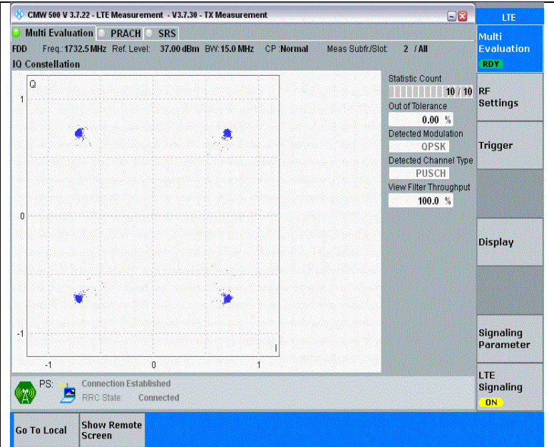
Band4-15MHz-QPSK-20175-75RB#0-PASS
