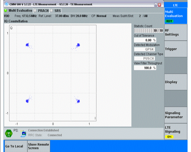
Band4-20MHz-QPSK-20175-100RB#0-PASS
