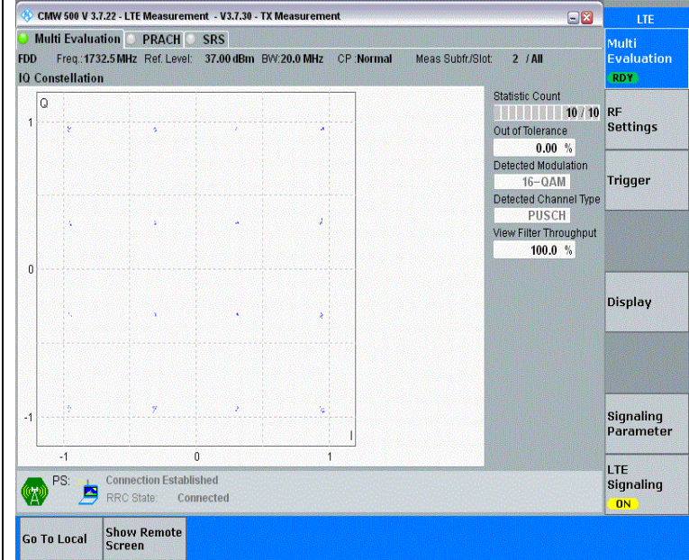
Band4-20MHz-16QAM-20175-1RB#0-PASS
