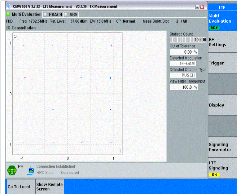
Band4-15MHz-16QAM-20175-1RB#0-PASS
