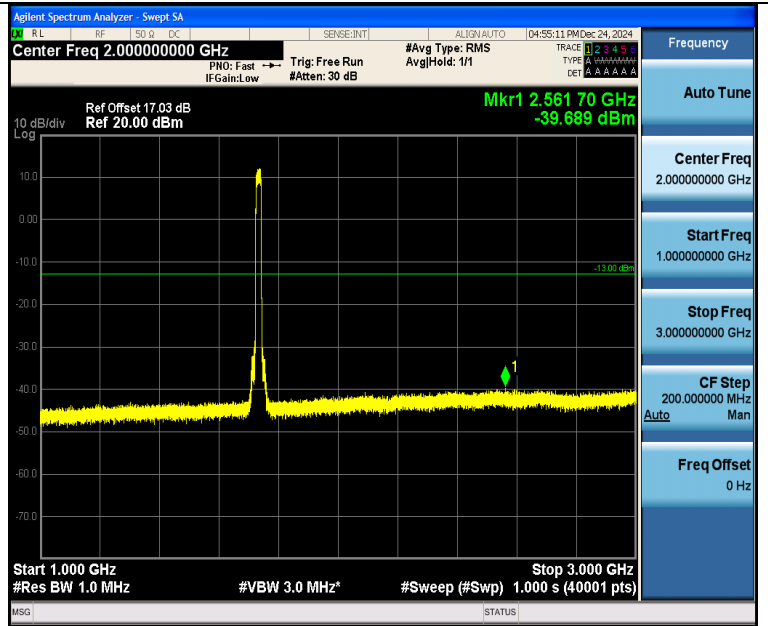
Band4_20MHz_QPSK_20175_100RB#0_1000~3000_1000~3000
