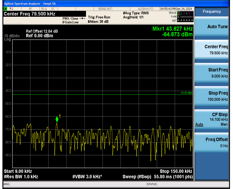
Band4_20MHz_QPSK_20300_100RB#0_0.009~0.15_0.009~0.15
