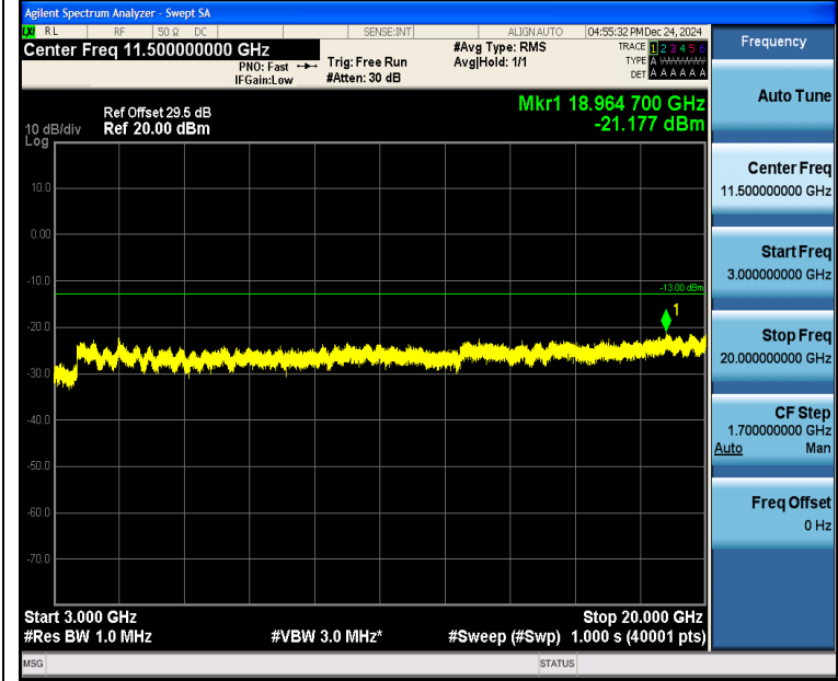
Band4_20MHz_QPSK_20175_100RB#0_3000~20000_3000~20000
