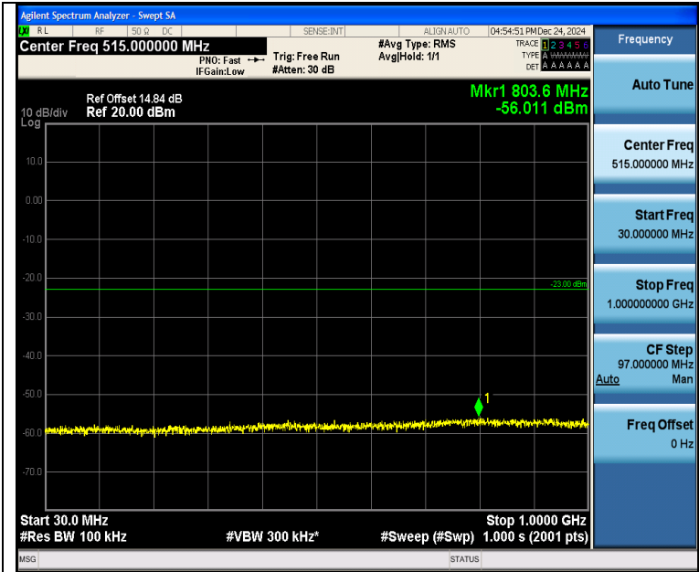
Band4_20MHz_QPSK_20175_100RB#0_30~1000_30~1000
