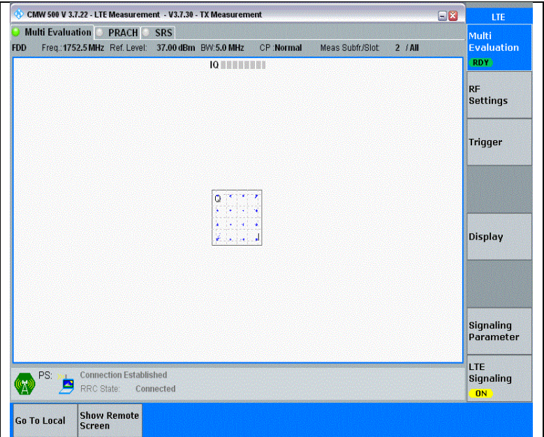
Band4-5MHz-16QAM-20375-25RB#0-PASS
