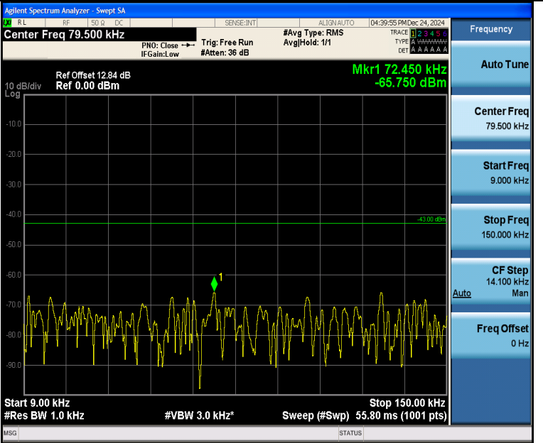
Band4_20MHz_QPSK_20050_1RB#0_0.009~0.15_0.009~0.15
