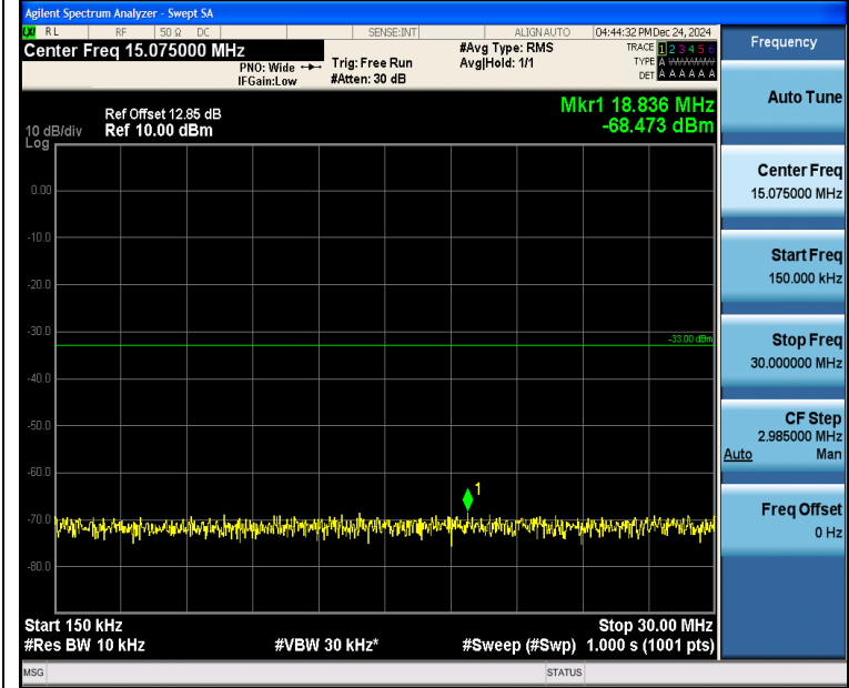
Band4_20MHz_QPSK_20175_1RB#0_0.15~30_0.15~30
