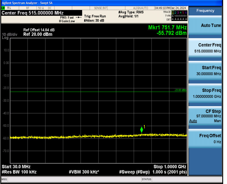
Band4_20MHz_QPSK_20300_1RB#0_30~1000_30~1000
