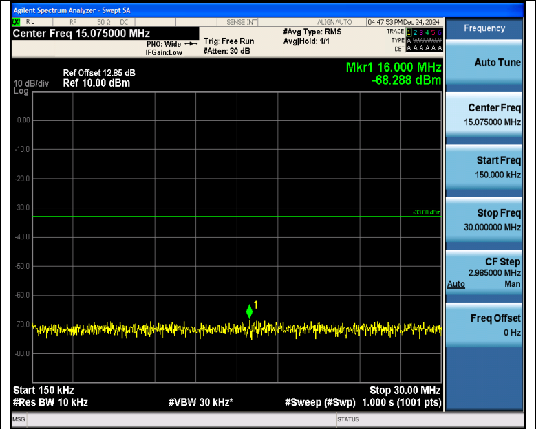
Band4_20MHz_16QAM_20175_1RB#99_0.15~30_0.15~30
