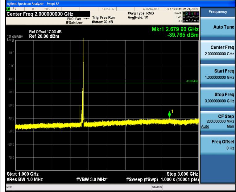
Band4_20MHz_QPSK_20175_1RB#99_1000~3000_1000~3000
