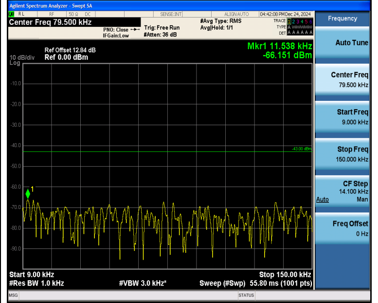
Band4_20MHz_QPSK_20050_1RB#99_0.009~0.15_0.009~0.15
