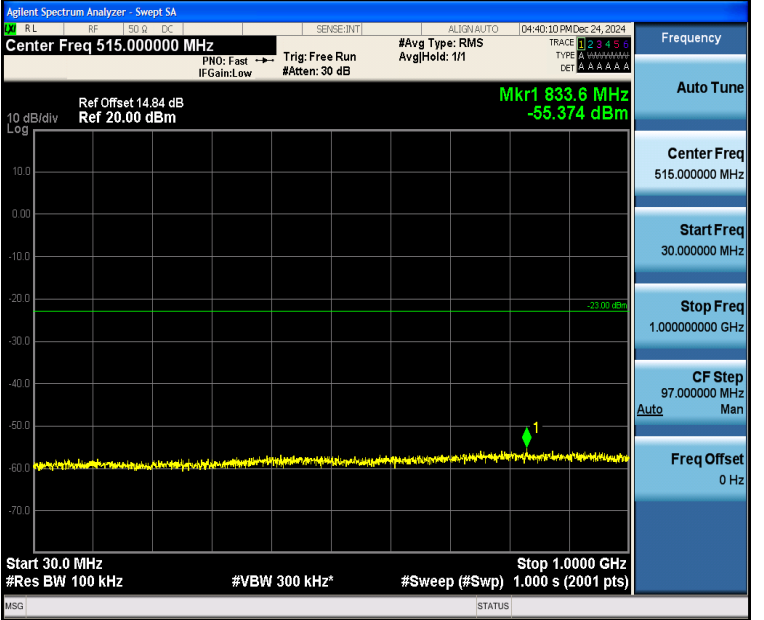
Band4_20MHz_QPSK_20050_1RB#0_30~1000_30~1000
