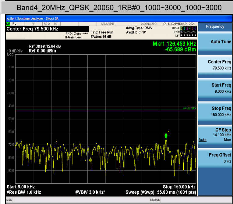
Band4_20MHz_QPSK_20050_1RB#0_1000~3000_1000~3000
