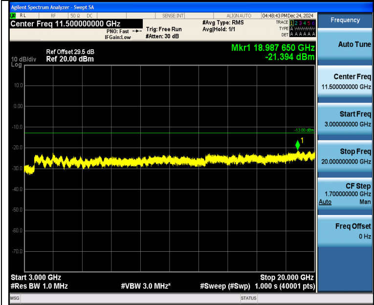
Band4_20MHz_16QAM_20175_1RB#99_3000~20000_3000~20000
