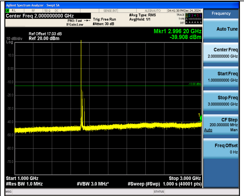
Band4_20MHz_16QAM_20050_1RB#0_1000~3000_1000~3000
