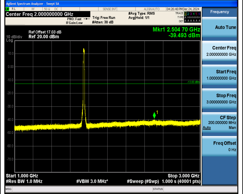
Band4_15MHz_QPSK_20325_75RB#0_1000~3000_1000~3000
