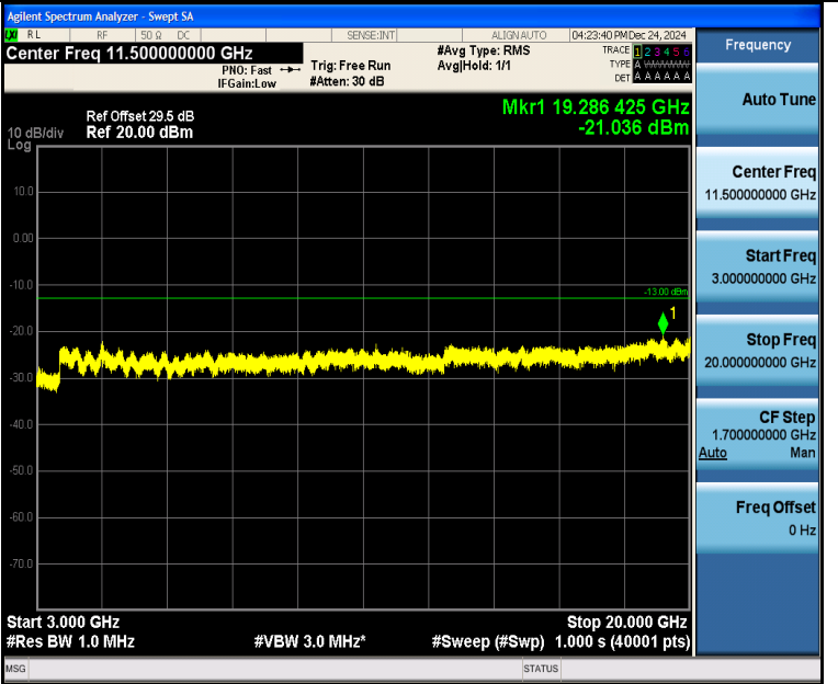
Band4_15MHz_16QAM_20325_1RB#74_3000~20000_3000~20000
