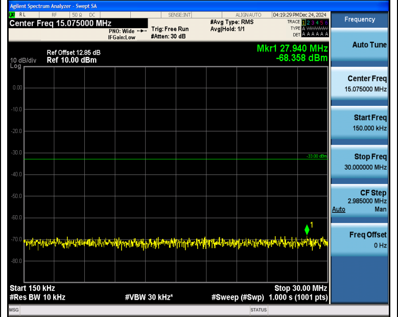
Band4_15MHz_QPSK_20325_1RB#0_0.15~30_0.15~30
