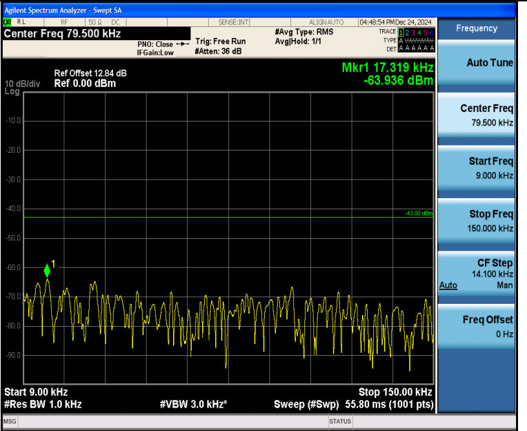
Band4_20MHz_QPSK_20300_1RB#0_0.009~0.15_0.009~0.15
