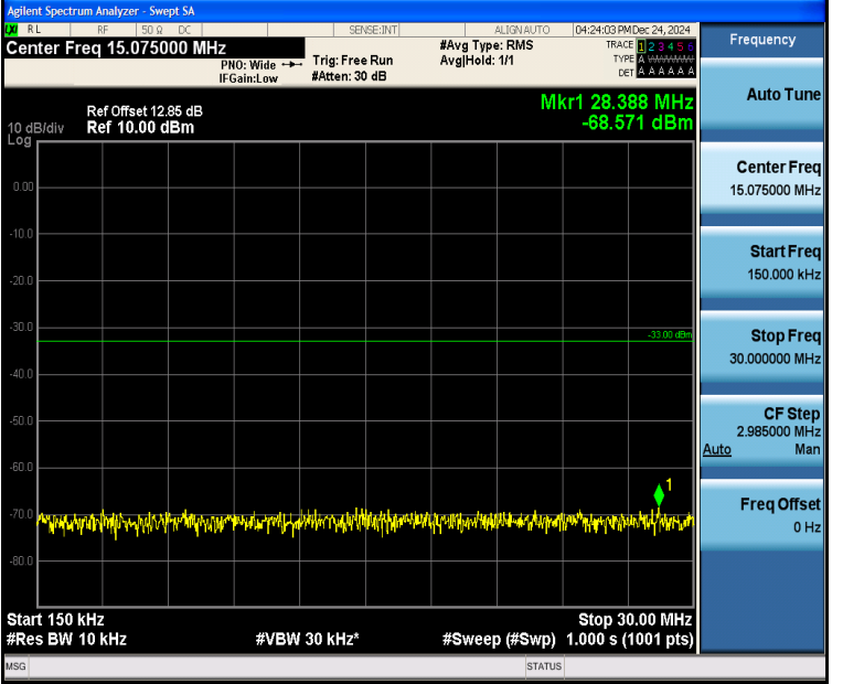
Band4_15MHz_QPSK_20025_75RB#0_0.15~30_0.15~30
