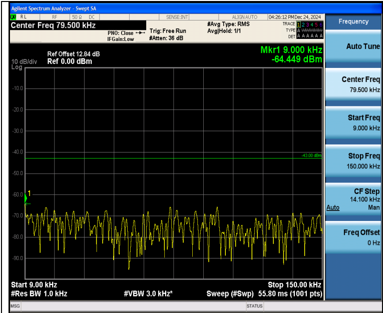
Band4_15MHz_QPSK_20325_75RB#0_0.009~0.15_0.009~0.15
