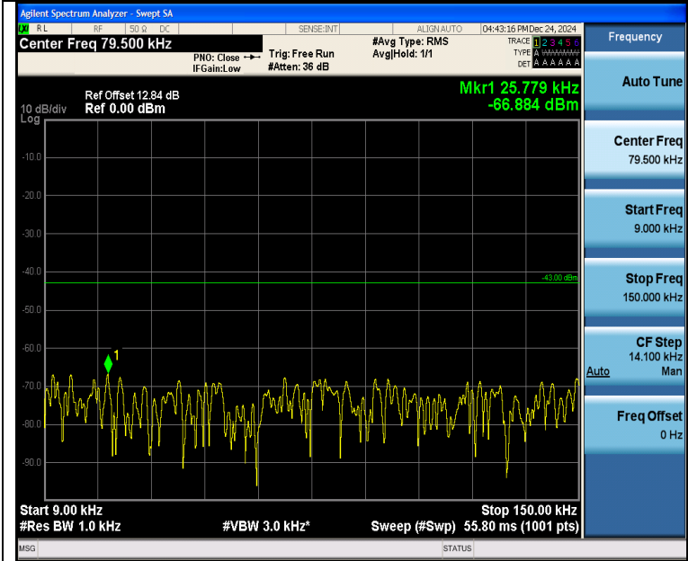
Band4_20MHz_16QAM_20050_1RB#99_0.009~0.15_0.009~0.15
