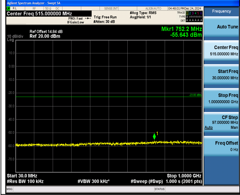
Band4_20MHz_16QAM_20175_1RB#99_30~1000_30~1000
