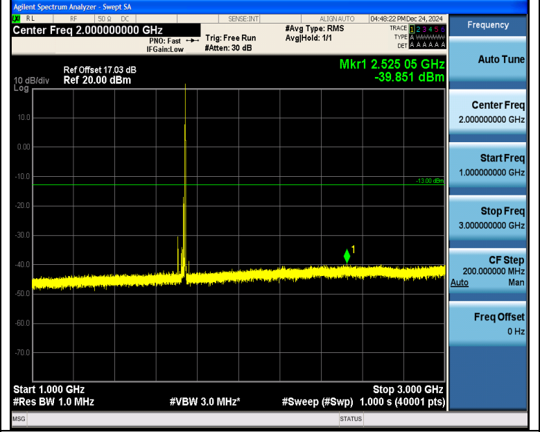
Band4_20MHz_16QAM_20175_1RB#99_1000~3000_1000~3000
