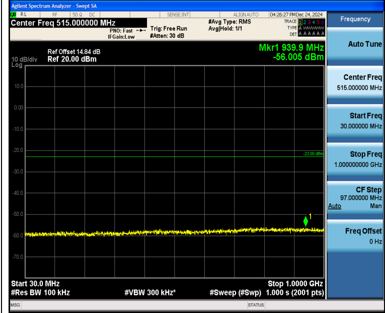
Band4_15MHz_QPSK_20325_75RB#0_30~1000_30~1000
