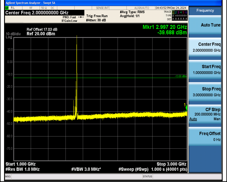
Band4_20MHz_16QAM_20050_1RB#99_1000~3000_1000~3000
