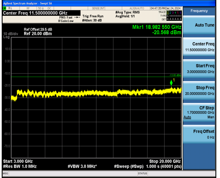
Band4_20MHz_QPSK_20175_1RB#99_3000~20000_3000~20000
