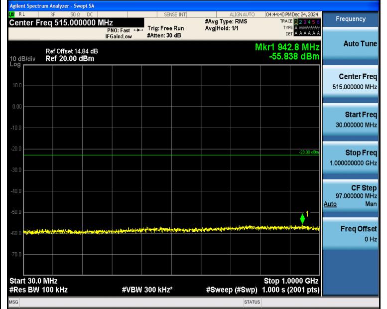
Band4_20MHz_QPSK_20175_1RB#0_30~1000_30~1000
