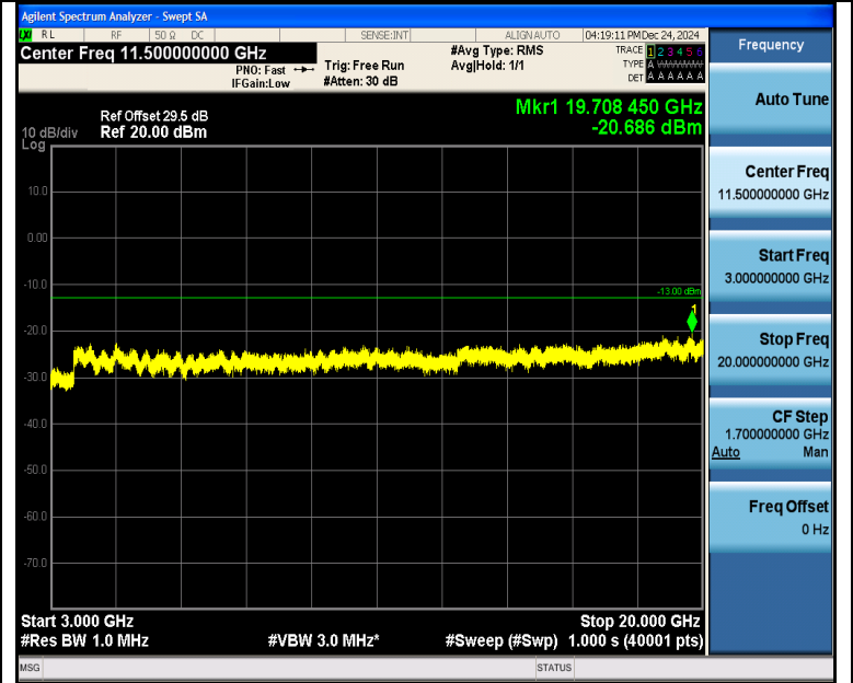
Band4_15MHz_16QAM_20175_1RB#74_3000~20000_3000~20000
