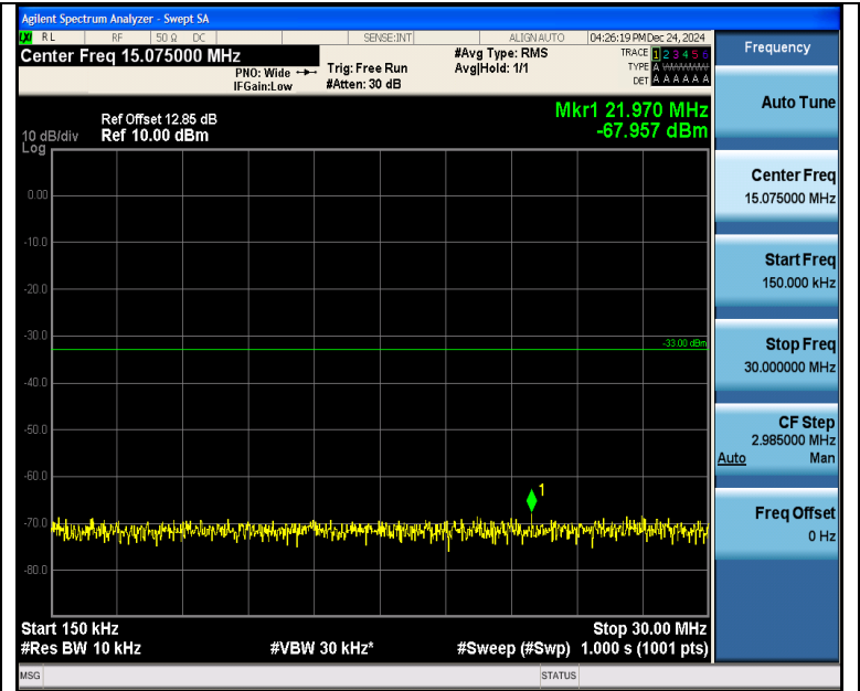
Band4_15MHz_QPSK_20325_75RB#0_0.15~30_0.15~30
