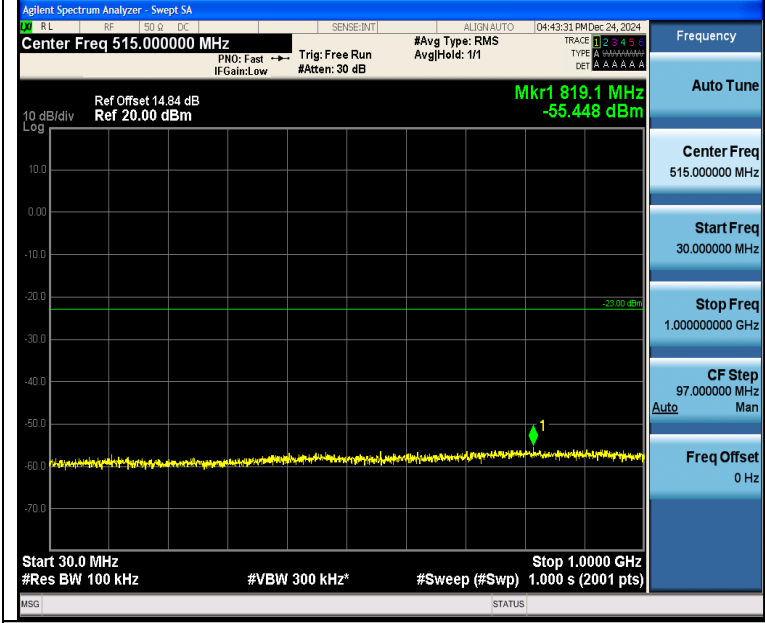
Band4_20MHz_16QAM_20050_1RB#99_30~1000_30~1000
