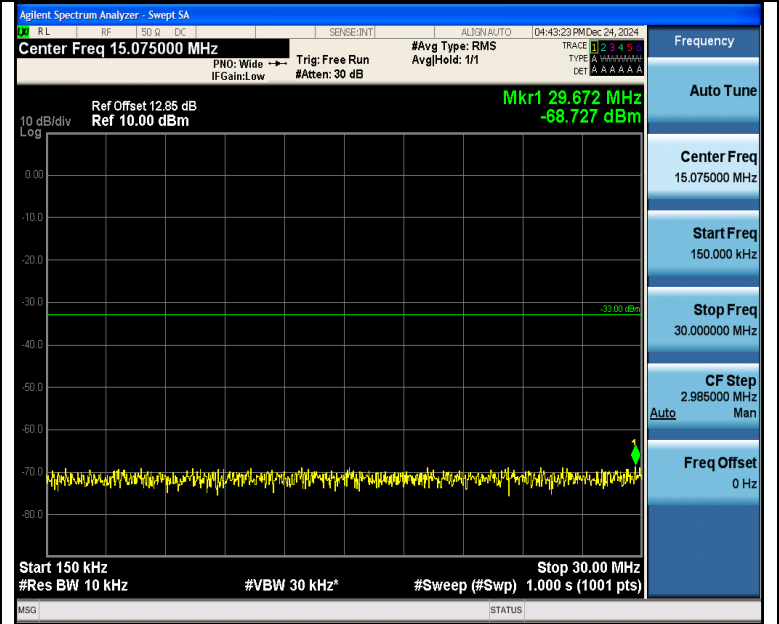
Band4_20MHz_16QAM_20050_1RB#99_0.15~30_0.15~30
