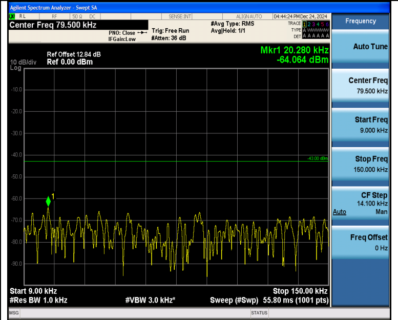
Band4_20MHz_QPSK_20175_1RB#0_0.009~0.15_0.009~0.15
