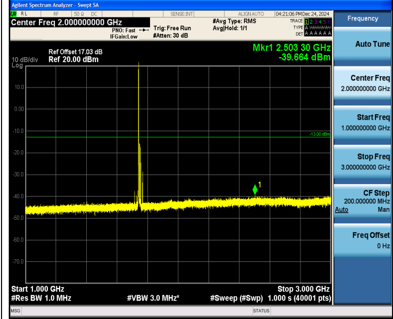
Band4_15MHz_16QAM_20325_1RB#0_1000~3000_1000~3000
