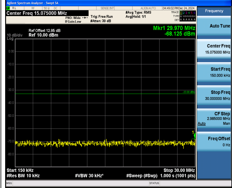
Band4_20MHz_QPSK_20300_1RB#0_0.15~30_0.15~30
