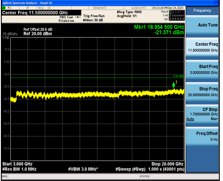
Band4_15MHz_16QAM_20325_1RB#0_3000~20000_3000~20000
