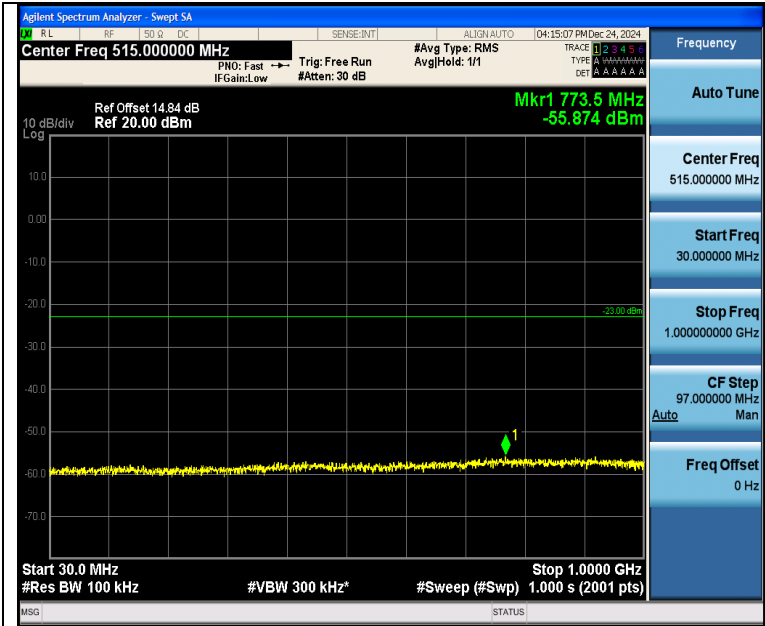
Band4_15MHz_QPSK_20175_1RB#0_30~1000_30~1000
