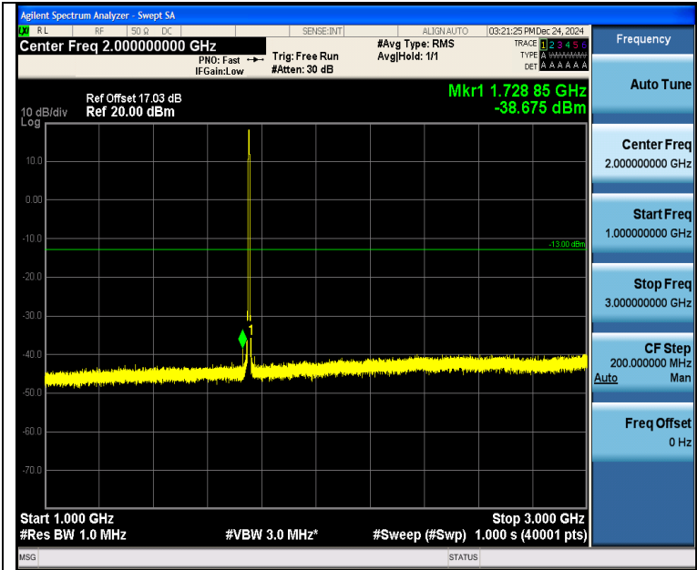
Band4_5MHz_QPSK_20375_25RB#0_1000~3000_1000~3000
