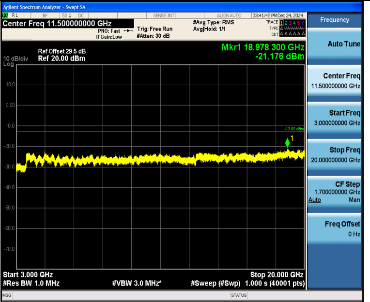
Band4_10MHz_QPSK_20000_1RB#49_3000~20000_3000~20000
