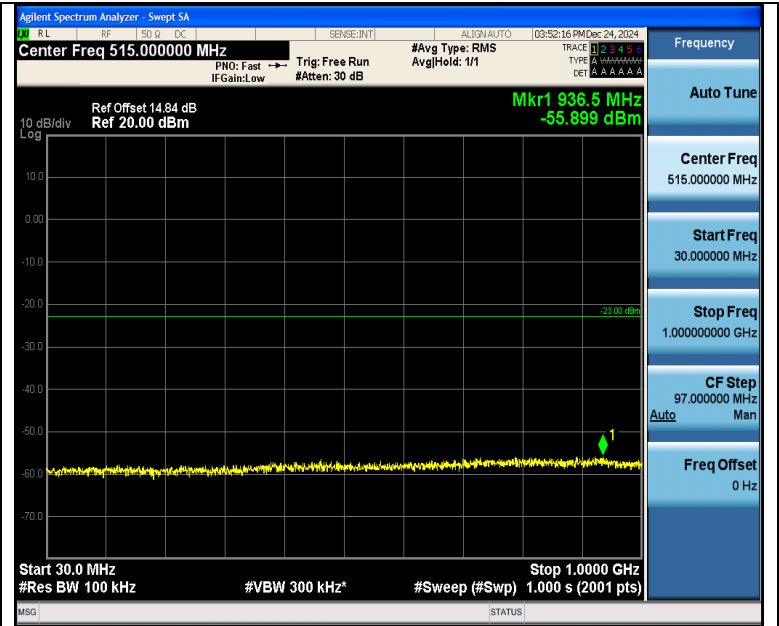
Band4_10MHz_QPSK_20000_50RB#0_30~1000_30~1000
