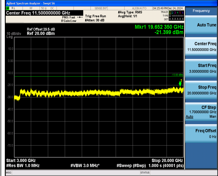
Band4_15MHz_QPSK_20175_1RB#0_3000~20000_3000~20000
