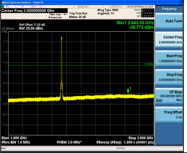
Band4_10MHz_QPSK_20175_50RB#0_1000~3000_1000~3000
