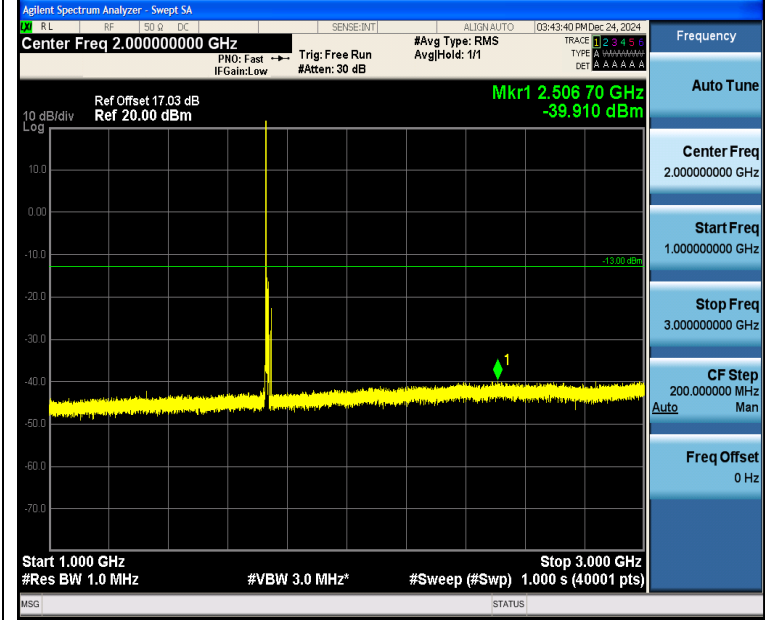
Band4_10MHz_QPSK_20175_1RB#0_1000~3000_1000~3000
