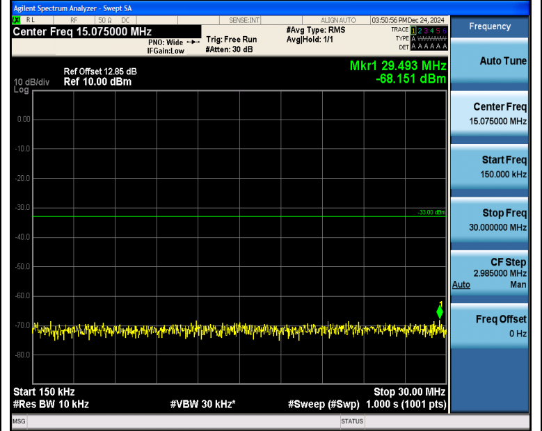
Band4_10MHz_16QAM_20350_1RB#49_0.15~30_0.15~30
