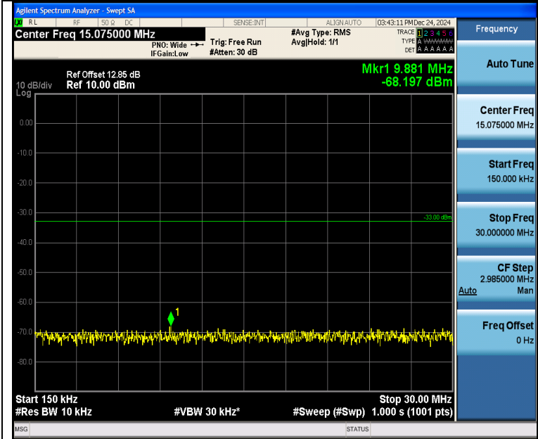
Band4_10MHz_QPSK_20175_1RB#0_0.15~30_0.15~30
