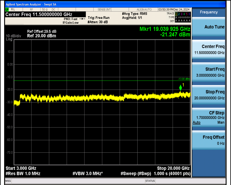
Band4_10MHz_QPSK_20350_1RB#49_3000~20000_3000~20000
