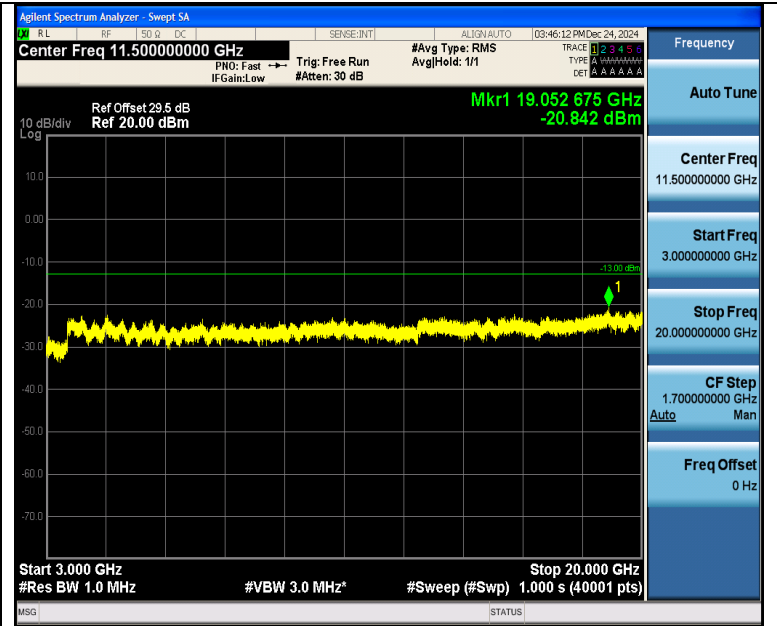
Band4_10MHz_QPSK_20175_1RB#49_3000~20000_3000~20000
