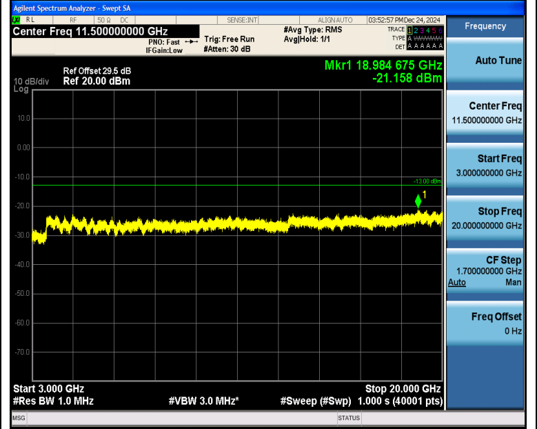
Band4_10MHz_QPSK_20000_50RB#0_3000~20000_3000~20000
