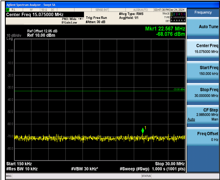
Band4_10MHz_QPSK_20350_1RB#0_0.15~30_0.15~30
