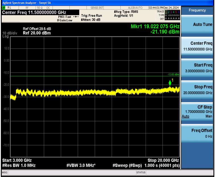
Band4_10MHz_QPSK_20175_1RB#0_3000~20000_3000~20000
