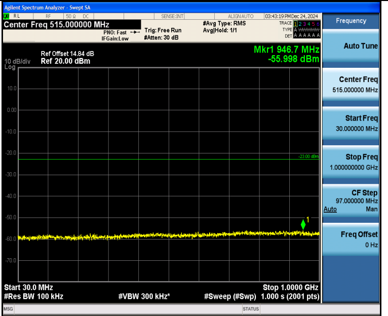
Band4_10MHz_QPSK_20175_1RB#0_30~1000_30~1000
