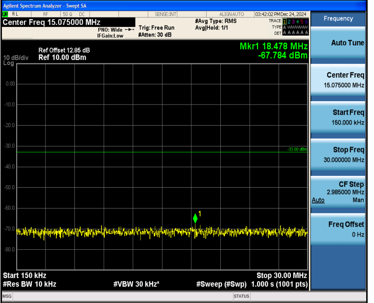
Band4_10MHz_16QAM_20000_1RB#49_0.15~30_0.15~30
