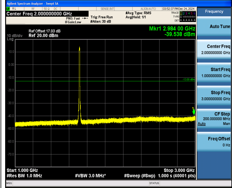
Band4_10MHz_QPSK_20000_50RB#0_1000~3000_1000~3000
