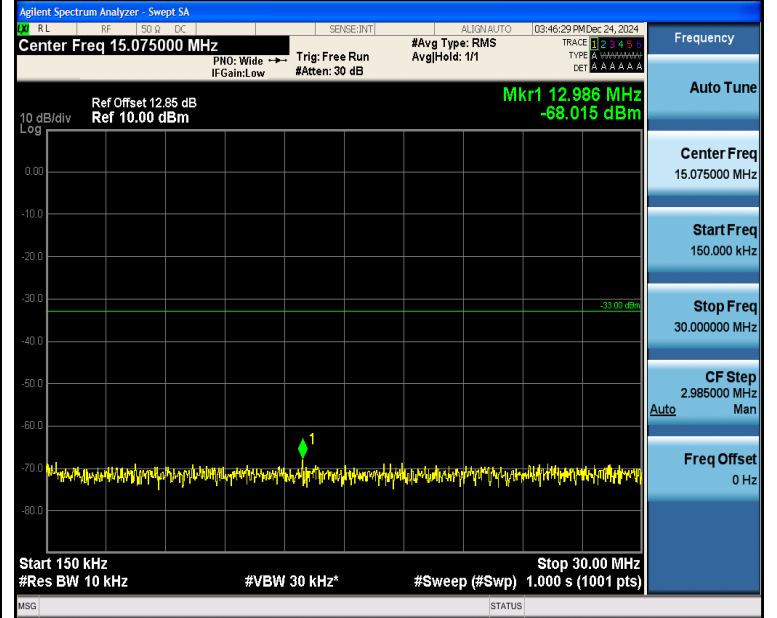
Band4_10MHz_16QAM_20175_1RB#49_0.15~30_0.15~30
