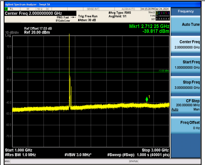
Band4_15MHz_QPSK_20175_1RB#0_1000~3000_1000~3000
