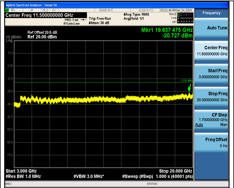
Band4_5MHz_QPSK_20375_25RB#0_3000~20000_3000~20000
