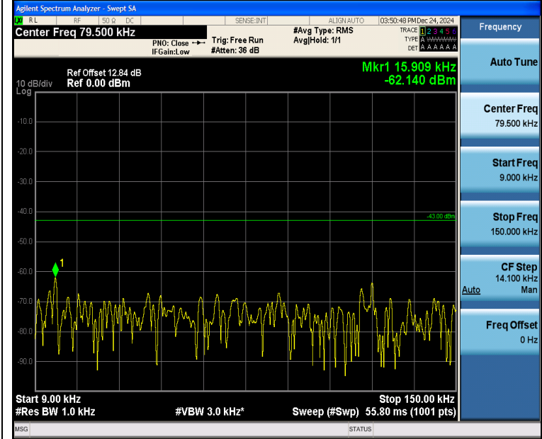
Band4_10MHz_16QAM_20350_1RB#49_0.009~0.15_0.009~0.15
