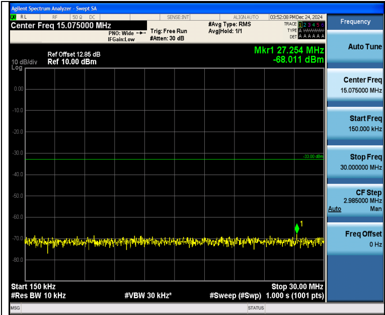
Band4_10MHz_QPSK_20000_50RB#0_0.15~30_0.15~30
