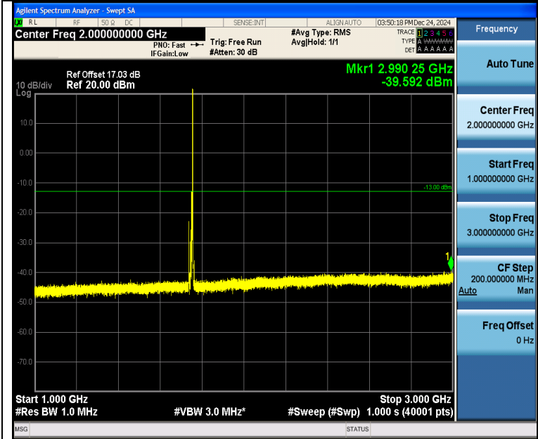
Band4_10MHz_QPSK_20350_1RB#49_1000~3000_1000~3000
