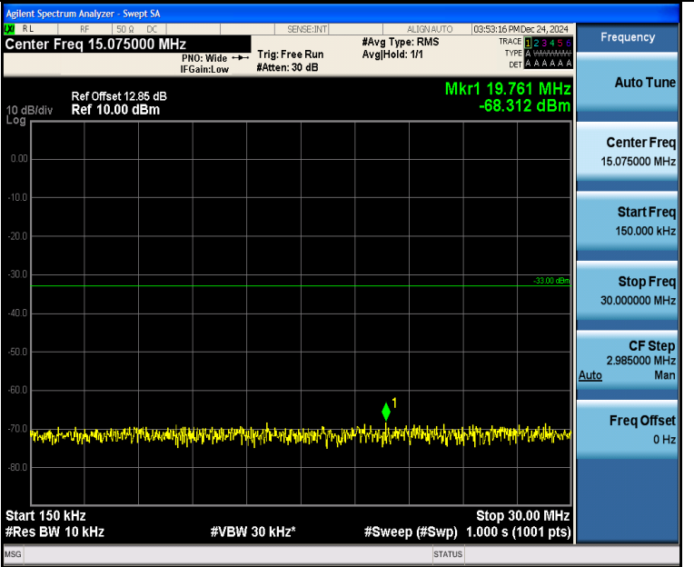
Band4_10MHz_QPSK_20175_50RB#0_0.15~30_0.15~30
