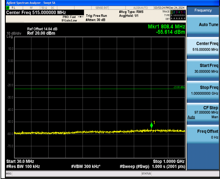
Band4_10MHz_QPSK_20175_50RB#0_30~1000_30~1000
