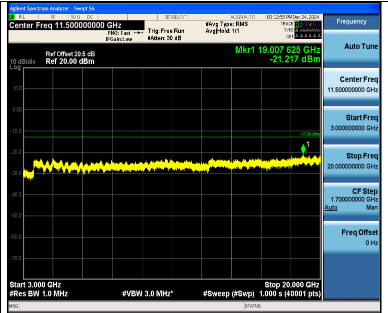
Band4_5MHz_QPSK_20175_1RB#24_3000~20000_3000~20000
