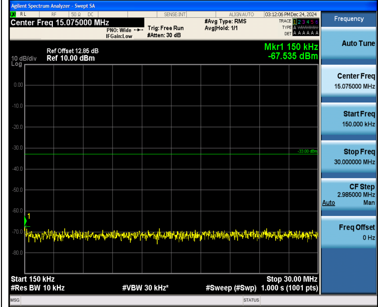
Band4_5MHz_QPSK_20175_1RB#24_0.15~30_0.15~30
