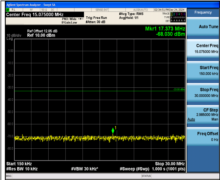
Band4_3MHz_QPSK_20175_1RB#14_0.15~30_0.15~30
