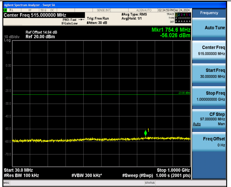
Band4_3MHz_QPSK_20175_1RB#14_30~1000_30~1000
