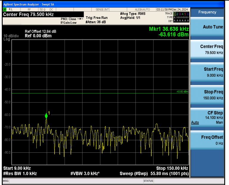
Band4_5MHz_QPSK_20175_1RB#24_0.009~0.15_0.009~0.15
