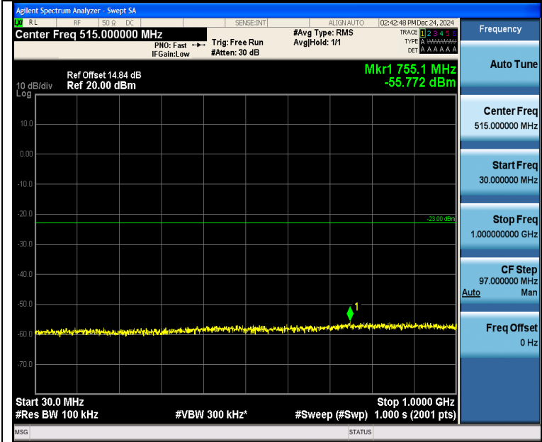
Band4_3MHz_16QAM_20385_1RB#14_30~1000_30~1000
