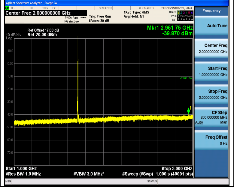
Band4_5MHz_16QAM_19975_1RB#24_1000~3000_1000~3000
