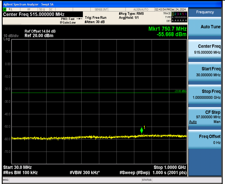
Band4_3MHz_QPSK_20385_15RB#0_30~1000_30~1000
