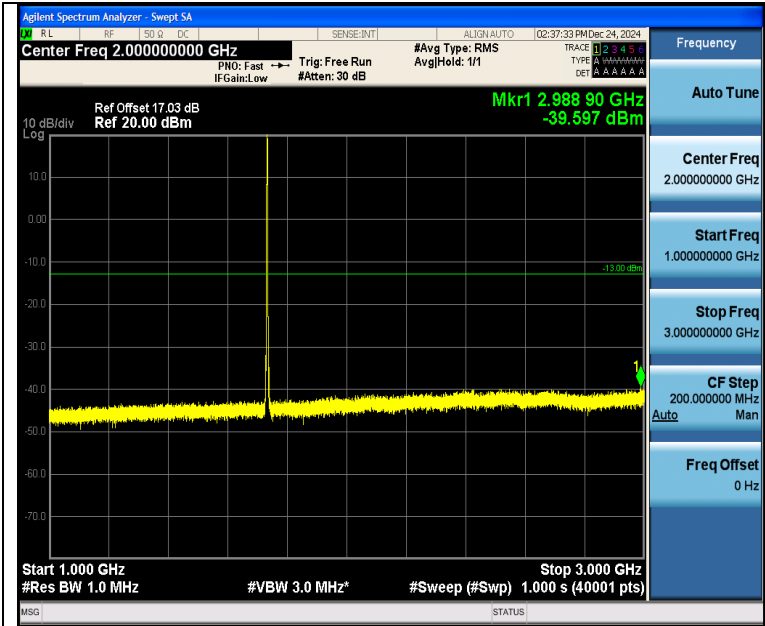
Band4_3MHz_QPSK_20175_15RB#0_1000~3000_1000~3000
