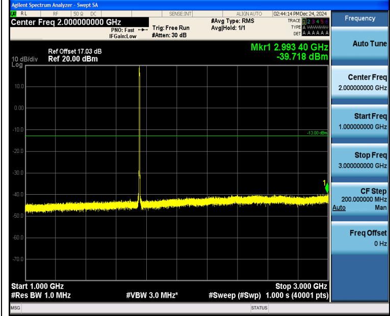
Band4_3MHz_QPSK_20385_15RB#0_1000~3000_1000~3000
