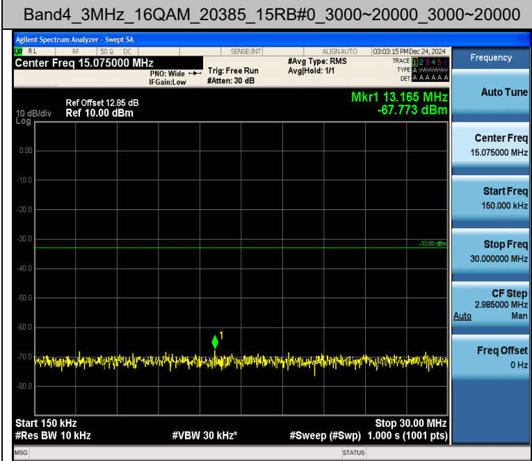
Band4_3MHz_16QAM_20385_15RB#0_3000~20000_3000~20000
