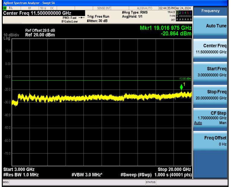
Band4_3MHz_QPSK_20385_15RB#0_3000~20000_3000~20000
