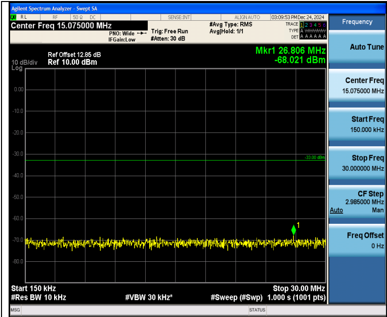
Band4_5MHz_QPSK_20175_1RB#0_0.15~30_0.15~30
