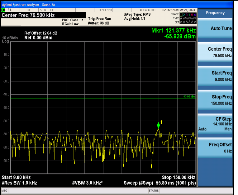
Band4_3MHz_QPSK_20175_15RB#0_0.009~0.15_0.009~0.15
