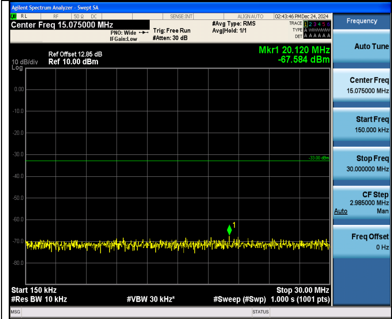
Band4_3MHz_QPSK_20385_15RB#0_0.15~30_0.15~30
