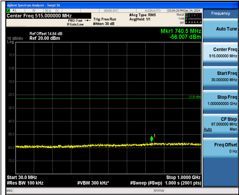
Band4_5MHz_16QAM_19975_1RB#0_30~1000_30~1000
