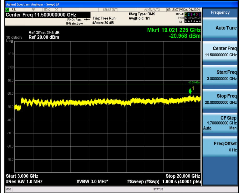
Band4_5MHz_QPSK_20175_25RB#0_3000~20000_3000~20000
