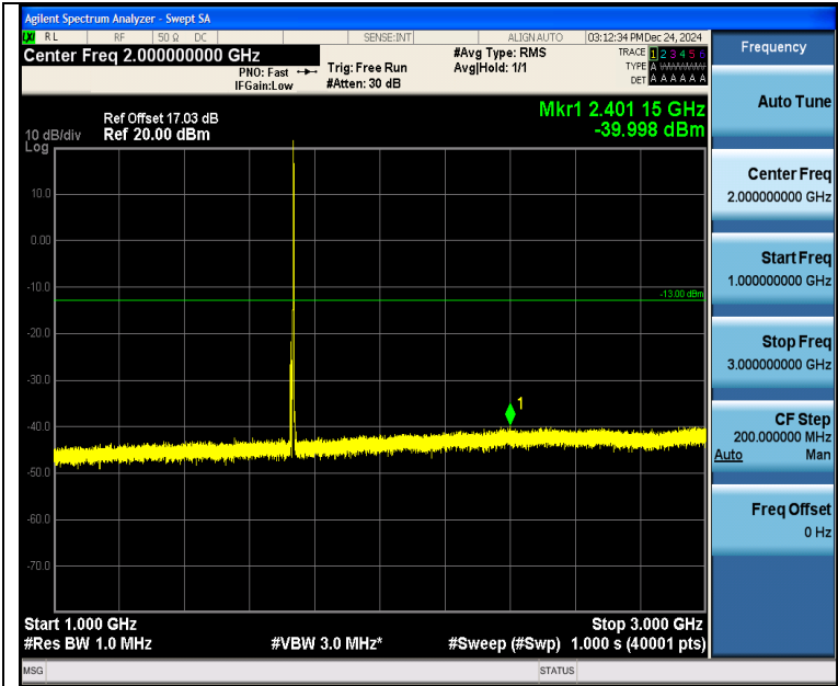
Band4_5MHz_QPSK_20175_1RB#24_1000~3000_1000~3000
