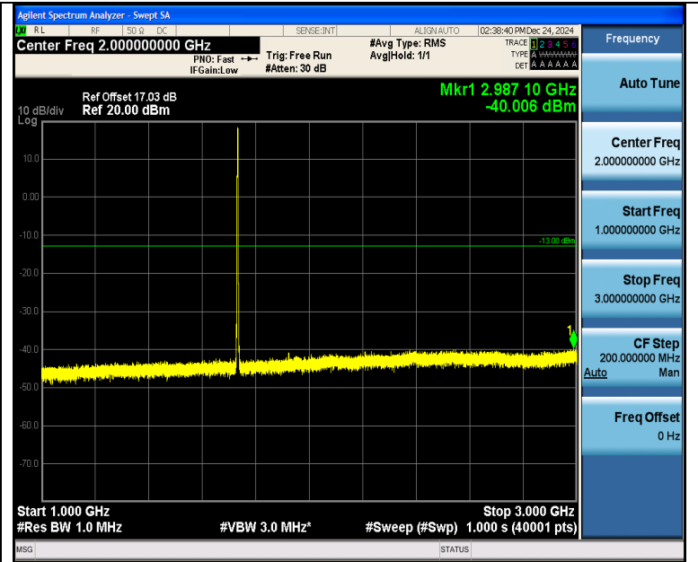
Band4_3MHz_16QAM_20175_15RB#0_1000~3000_1000~3000
