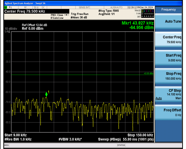
Band4_3MHz_QPSK_20385_1RB#0_0.009~0.15_0.009~0.15
