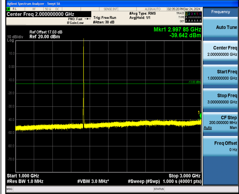
Band4_3MHz_QPSK_20175_1RB#14_1000~3000_1000~3000
