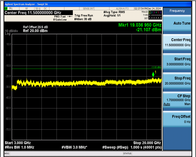
Band4_3MHz_QPSK_20175_15RB#0_3000~20000_3000~20000
