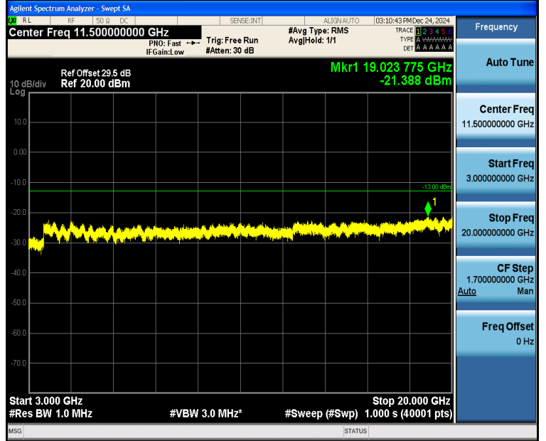
Band4_5MHz_QPSK_20175_1RB#0_3000~20000_3000~20000
