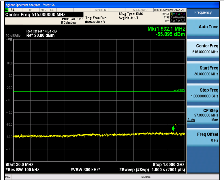
Band4_5MHz_QPSK_20175_25RB#0_30~1000_30~1000
