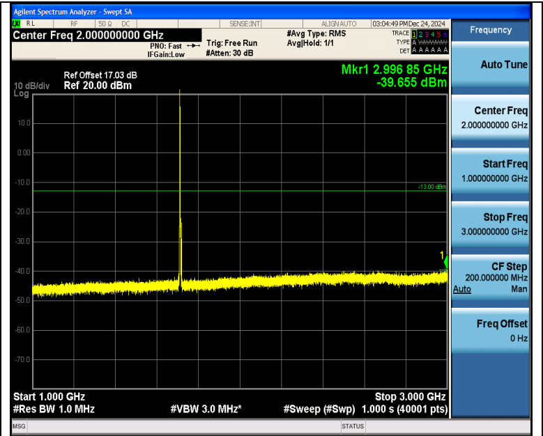
Band4_5MHz_16QAM_19975_1RB#0_1000~3000_1000~3000
