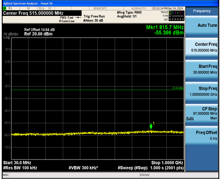
Band4_5MHz_QPSK_20175_1RB#24_30~1000_30~1000
