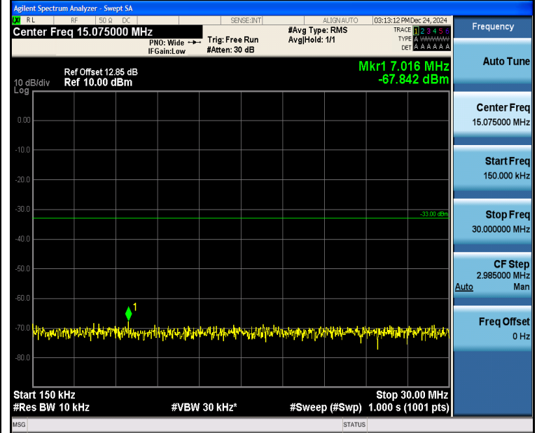
Band4_5MHz_16QAM_20175_1RB#24_0.15~30_0.15~30
