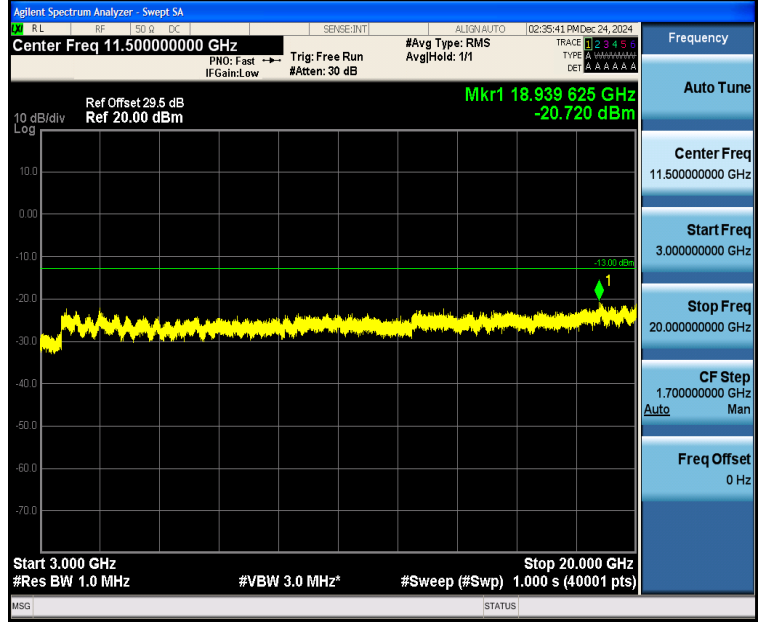
Band4_3MHz_QPSK_20175_1RB#14_3000~20000_3000~20000
