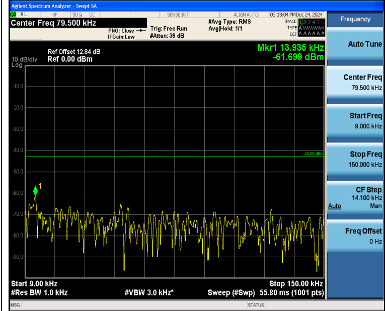
Band4_5MHz_16QAM_20175_1RB#24_0.009~0.15_0.009~0.15
