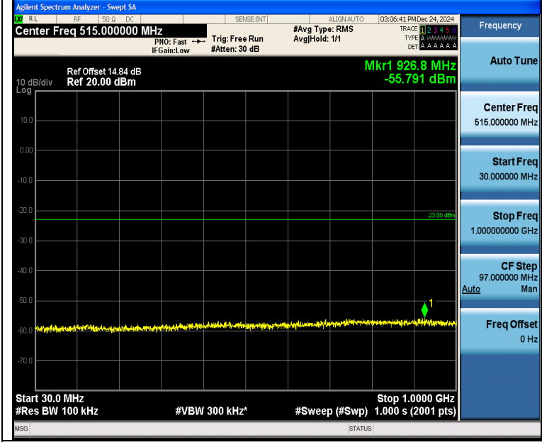
Band4_5MHz_16QAM_19975_1RB#24_30~1000_30~1000
