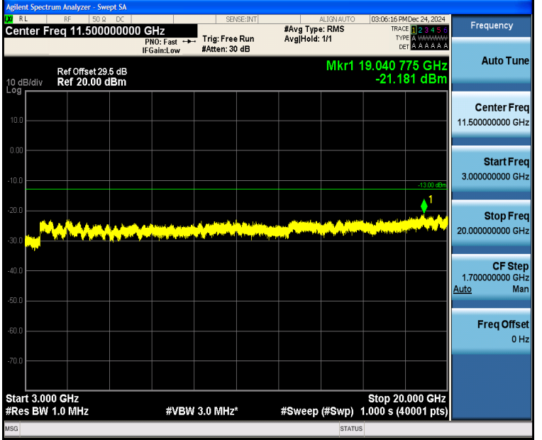
Band4_5MHz_QPSK_19975_1RB#24_3000~20000_3000~20000
