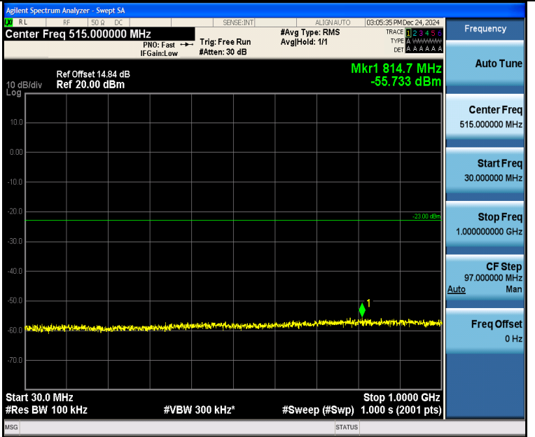
Band4_5MHz_QPSK_19975_1RB#24_30~1000_30~1000
