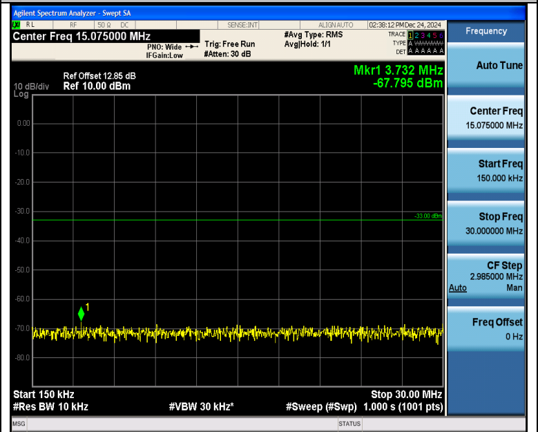
Band4_3MHz_16QAM_20175_15RB#0_0.15~30_0.15~30
