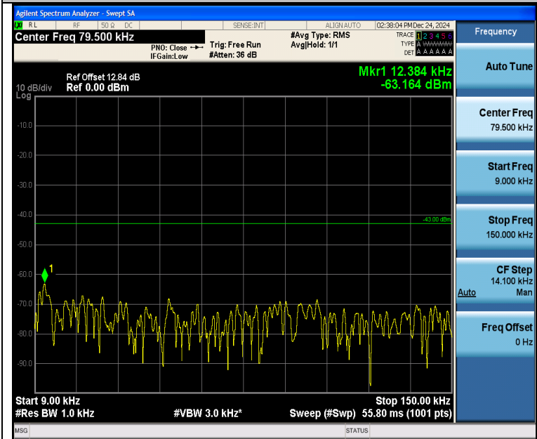
Band4_3MHz_16QAM_20175_15RB#0_0.009~0.15_0.009~0.15
