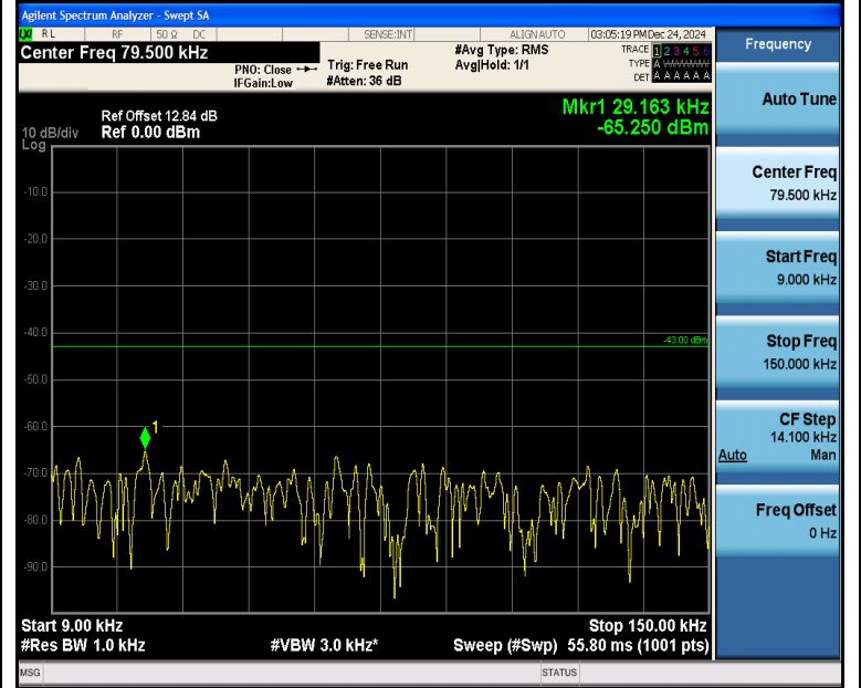
Band4_5MHz_QPSK_19975_1RB#24_0.009~0.15_0.009~0.15
