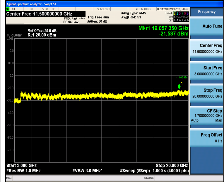
Band4_5MHz_16QAM_19975_1RB#0_3000~20000_3000~20000
