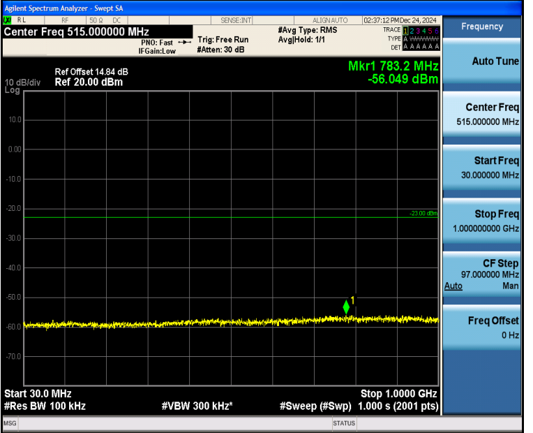
Band4_3MHz_QPSK_20175_15RB#0_30~1000_30~1000
