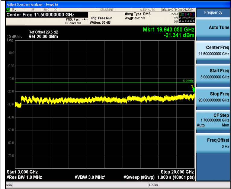
Band4_5MHz_16QAM_20175_1RB#0_3000~20000_3000~20000
