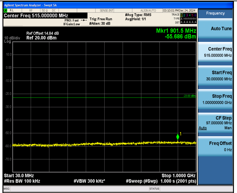
Band4_5MHz_QPSK_20175_1RB#0_30~1000_30~1000
