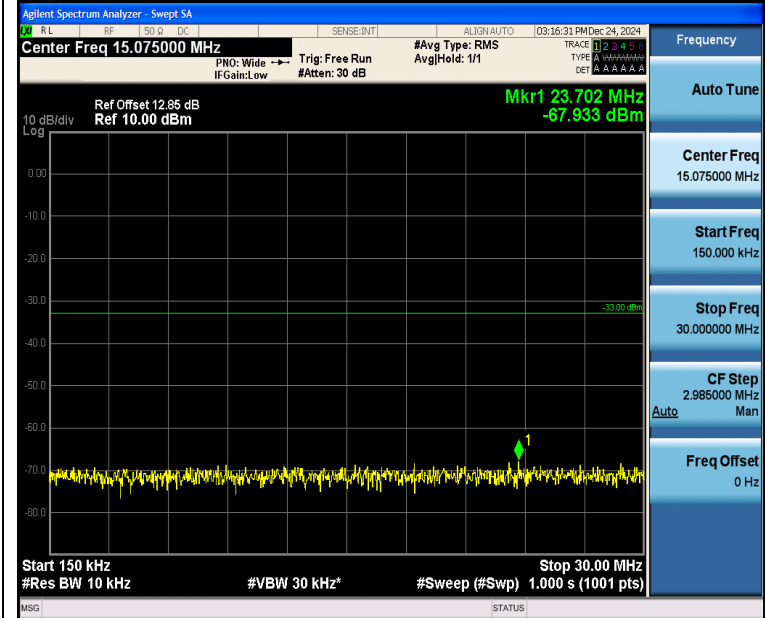
Band4_5MHz_QPSK_20375_1RB#0_0.15~30_0.15~30
