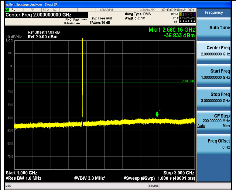
Band4_3MHz_16QAM_20385_1RB#14_1000~3000_1000~3000
