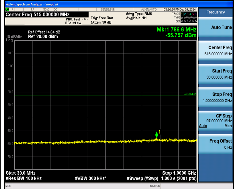
Band4_5MHz_QPSK_20375_1RB#0_30~1000_30~1000
