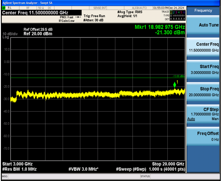
Band4_1.4MHz_QPSK_20175_6RB#0_3000~20000_3000~20000
