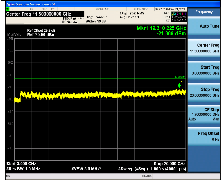
Band4_3MHz_16QAM_19965_1RB#0_3000~20000_3000~20000
