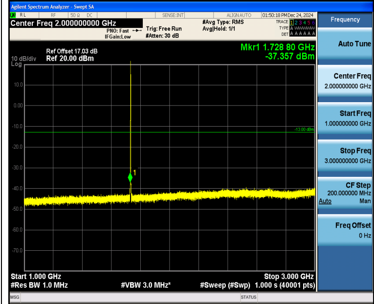
Band4_1.4MHz_QPSK_20175_1RB#0_1000~3000_1000~3000
