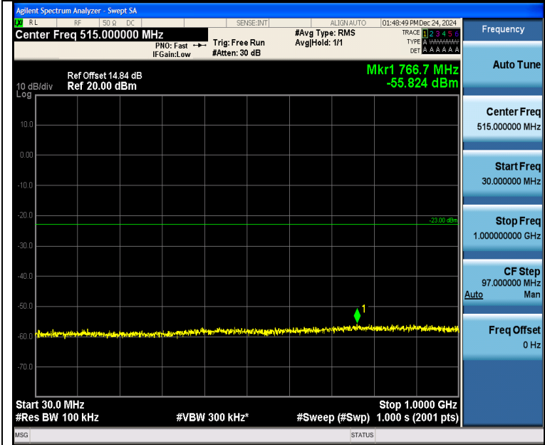
Band4_1.4MHz_16QAM_19957_6RB#0_30~1000_30~1000
