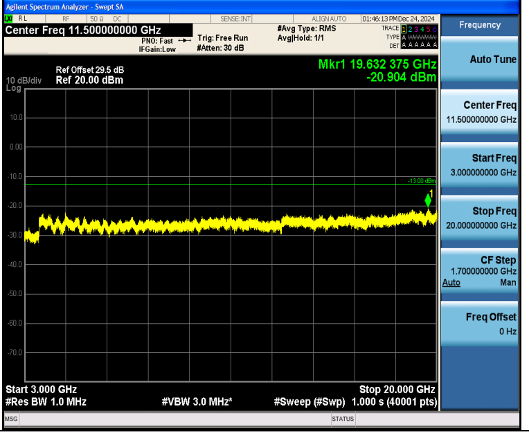
Band4_1.4MHz_QPSK_19957_1RB#5_3000~20000_3000~20000
