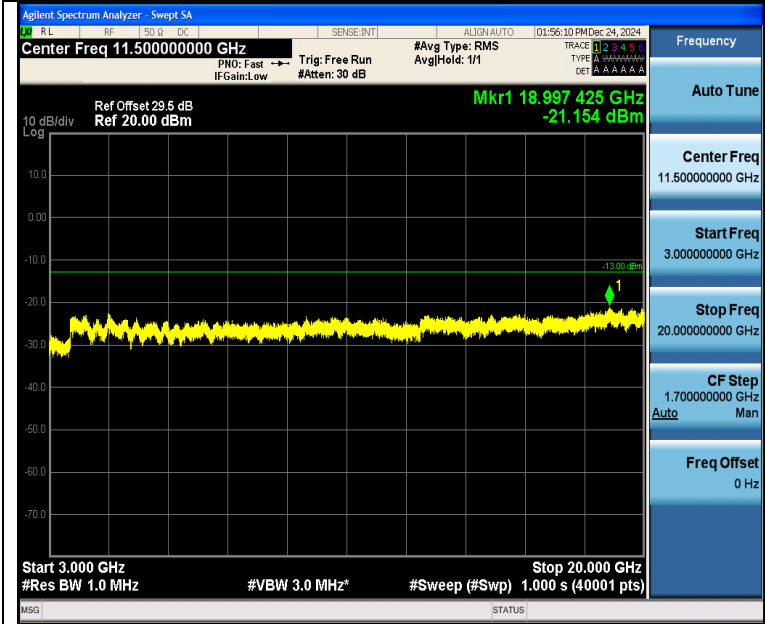
Band4_1.4MHz_16QAM_20175_6RB#0_3000~20000_3000~20000
