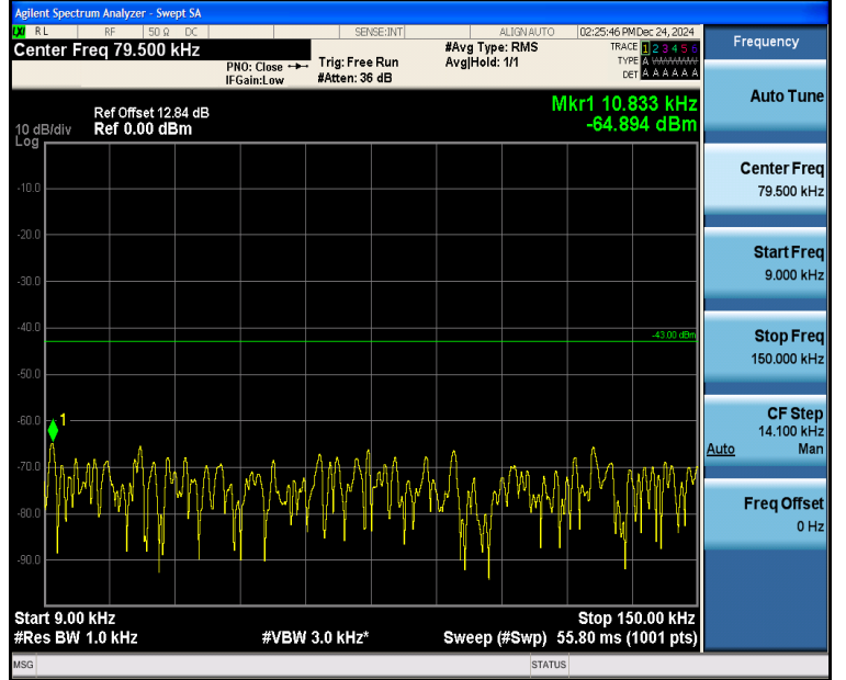
Band4_3MHz_QPSK_19965_1RB#0_0.009~0.15_0.009~0.15
