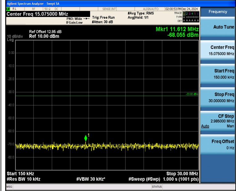
Band4_1.4MHz_QPSK_20393_6RB#0_0.15~30_0.15~30
