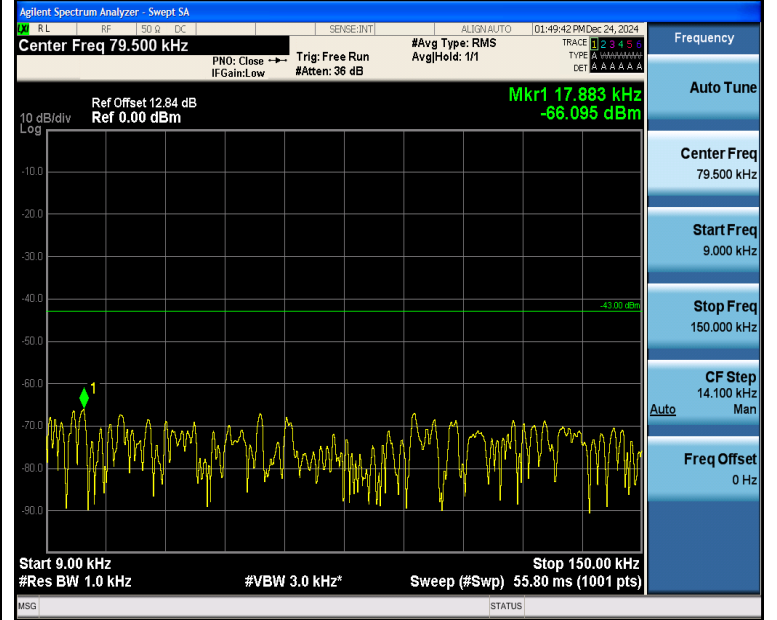
Band4_1.4MHz_QPSK_20175_1RB#0_0.009~0.15_0.009~0.15
