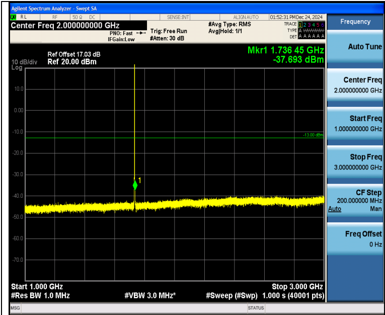
Band4_1.4MHz_QPSK_20175_1RB#5_1000~3000_1000~3000
