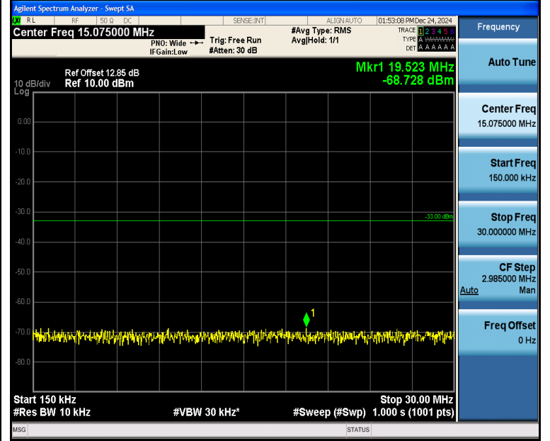
Band4_1.4MHz_16QAM_20175_1RB#5_0.15~30_0.15~30
