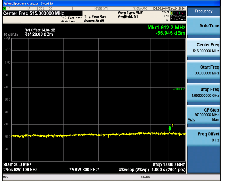
Band4_3MHz_QPSK_19965_1RB#14_30~1000_30~1000
