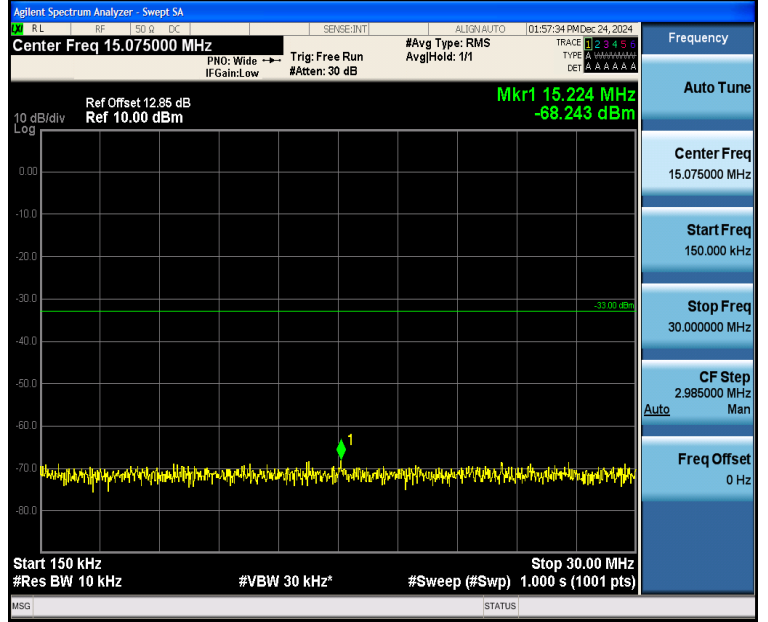
Band4_1.4MHz_16QAM_20393_1RB#0_0.15~30_0.15~30
