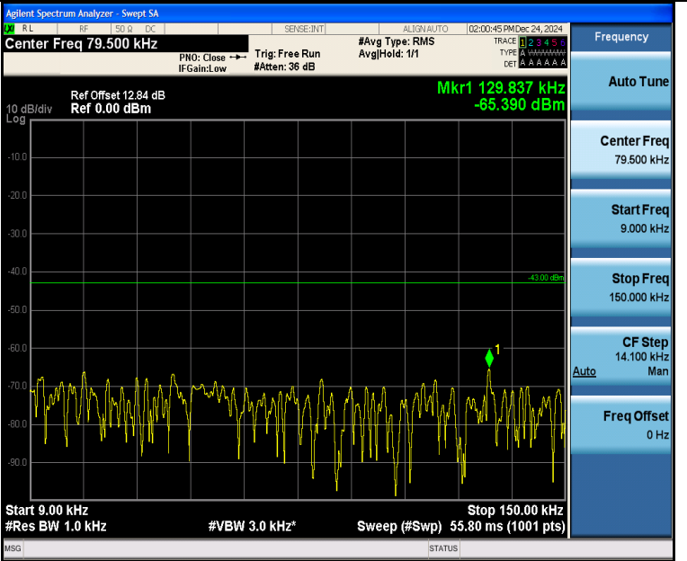
Band4_1.4MHz_QPSK_20393_6RB#0_0.009~0.15_0.009~0.15
