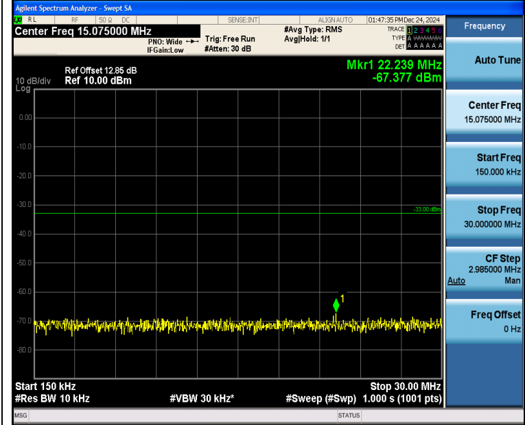
Band4_1.4MHz_QPSK_19957_6RB#0_0.15~30_0.15~30
