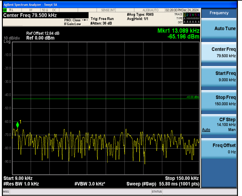
Band4_3MHz_QPSK_19965_1RB#14_0.009~0.15_0.009~0.15
