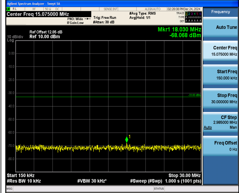
Band4_3MHz_QPSK_19965_1RB#14_0.15~30_0.15~30
