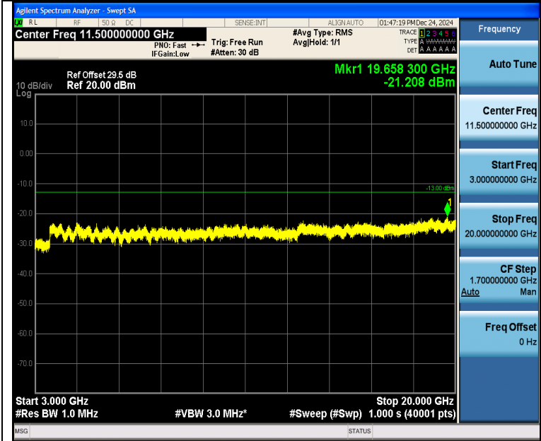
Band4_1.4MHz_16QAM_19957_1RB#5_3000~20000_3000~20000
