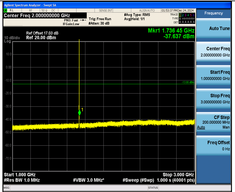
Band4_1.4MHz_16QAM_20175_1RB#5_1000~3000_1000~3000
