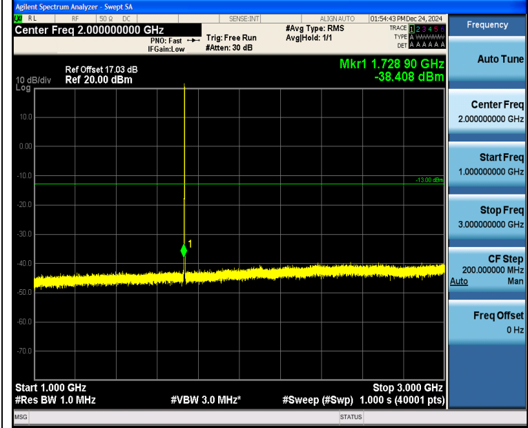
Band4_1.4MHz_QPSK_20175_6RB#0_1000~3000_1000~3000
