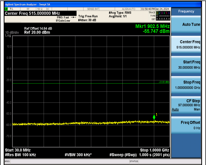
Band4_1.4MHz_QPSK_20393_1RB#5_30~1000_30~1000
