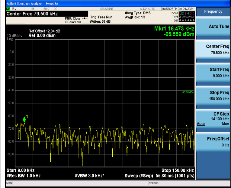
Band4_1.4MHz_16QAM_20393_1RB#0_0.009~0.15_0.009~0.15
