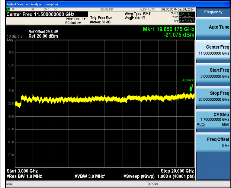
Band4_3MHz_16QAM_19965_1RB#14_3000~20000_3000~20000
