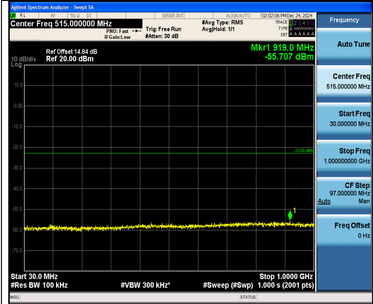
Band4_1.4MHz_16QAM_20393_6RB#0_30~1000_30~1000
