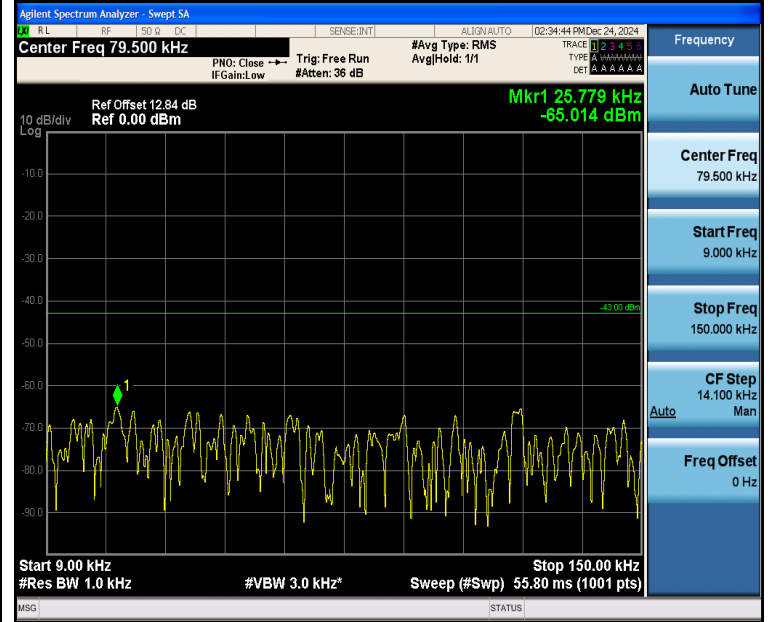
Band4_3MHz_QPSK_20175_1RB#14_0.009~0.15_0.009~0.15
