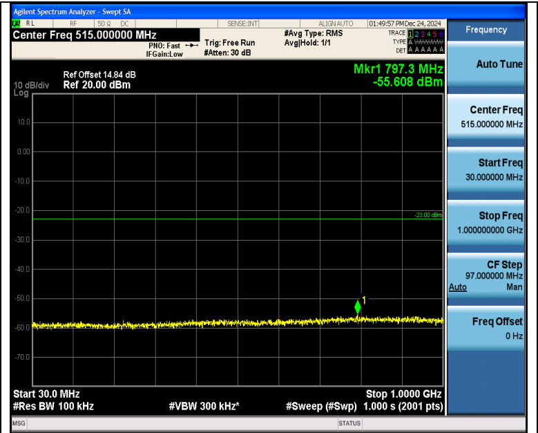
Band4_1.4MHz_QPSK_20175_1RB#0_30~1000_30~1000
