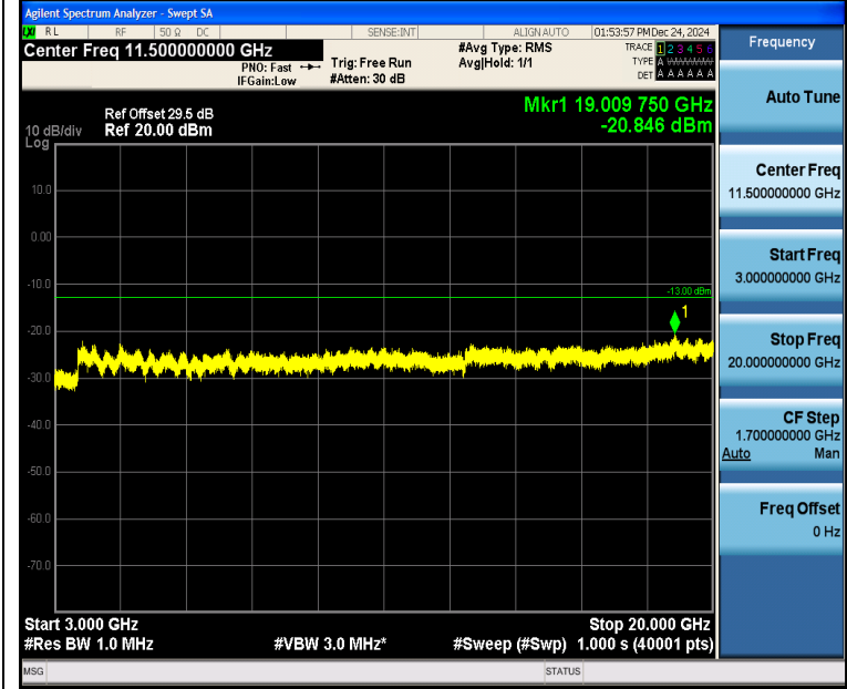
Band4_1.4MHz_16QAM_20175_1RB#5_3000~20000_3000~20000
