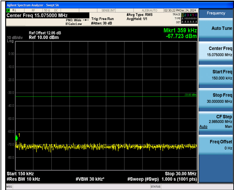
Band4_3MHz_QPSK_19965_15RB#0_0.15~30_0.15~30
