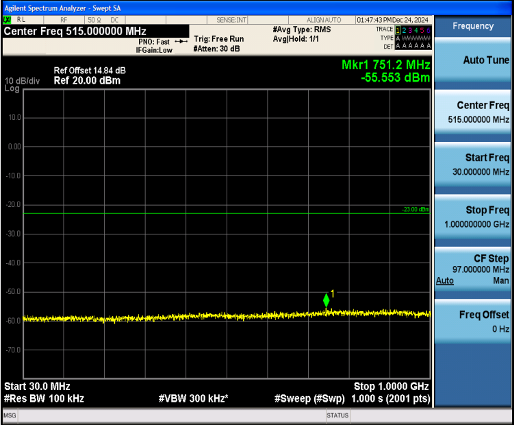
Band4_1.4MHz_QPSK_19957_6RB#0_30~1000_30~1000
