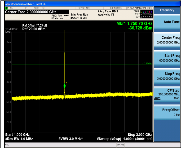
Band4_1.4MHz_QPSK_20393_1RB#0_1000~3000_1000~3000
