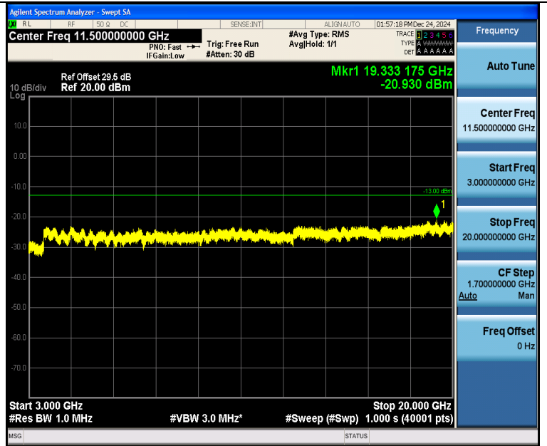
Band4_1.4MHz_QPSK_20393_1RB#0_3000~20000_3000~20000
