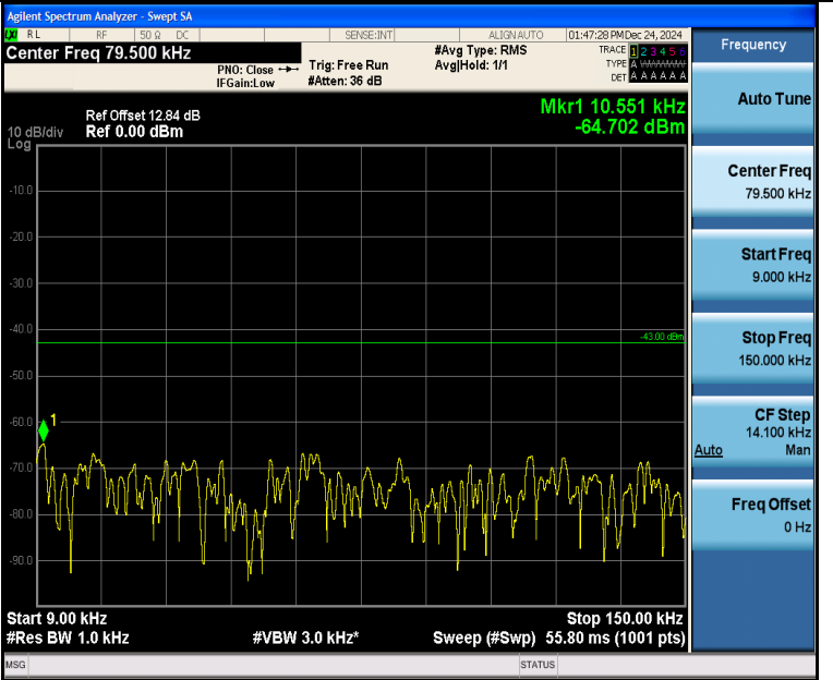
Band4_1.4MHz_QPSK_19957_6RB#0_0.009~0.15_0.009~0.15
