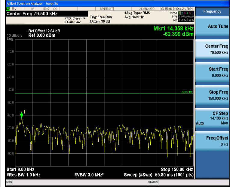
Band4_1.4MHz_16QAM_20175_1RB#5_0.009~0.15_0.009~0.15
