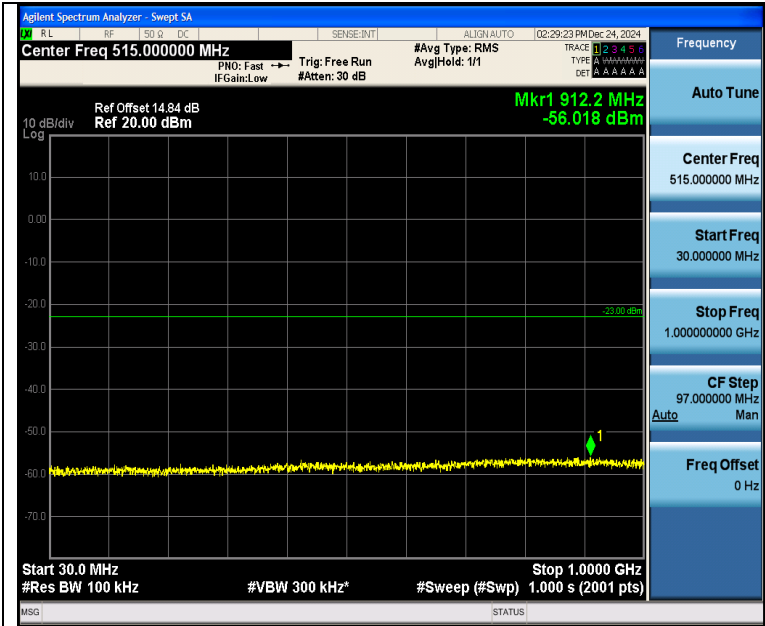
Band4_3MHz_16QAM_19965_1RB#14_30~1000_30~1000
