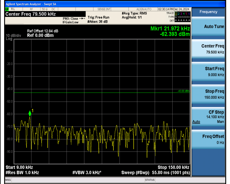
Band4_3MHz_QPSK_19965_15RB#0_0.009~0.15_0.009~0.15
