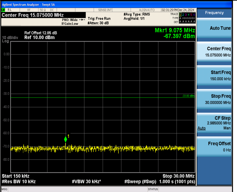
Band4_3MHz_16QAM_19965_15RB#0_0.15~30_0.15~30
