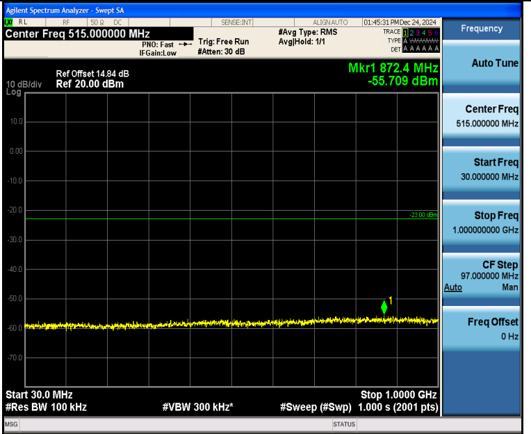
Band4_1.4MHz_QPSK_19957_1RB#5_30~1000_30~1000
