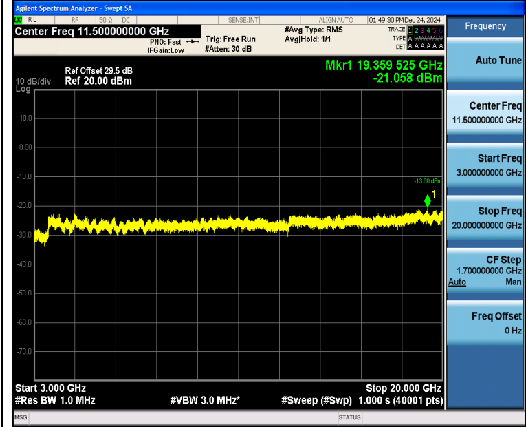
Band4_1.4MHz_16QAM_19957_6RB#0_3000~20000_3000~20000
