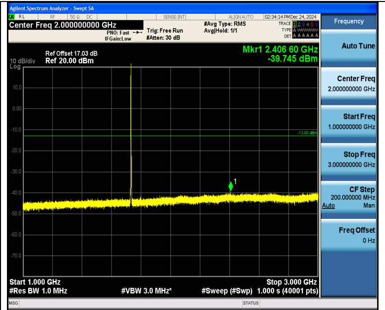
Band4_3MHz_16QAM_20175_1RB#0_1000~3000_1000~3000
