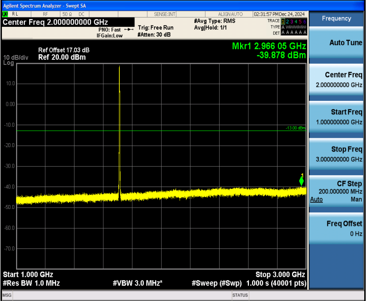
Band4_3MHz_16QAM_19965_15RB#0_1000~3000_1000~3000
