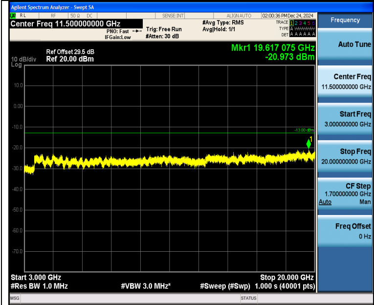
Band4_1.4MHz_16QAM_20393_1RB#5_3000~20000_3000~20000
