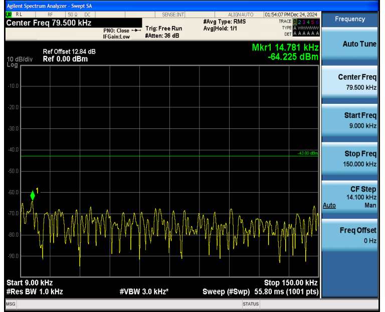
Band4_1.4MHz_QPSK_20175_6RB#0_0.009~0.15_0.009~0.15
