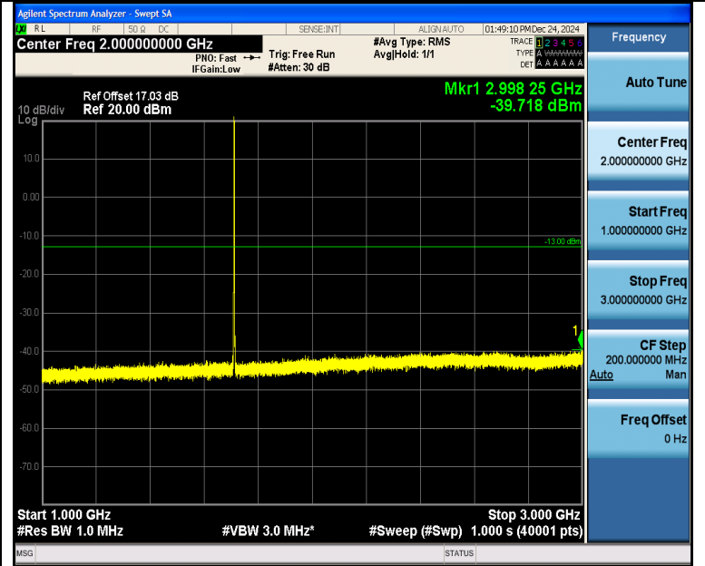
Band4_1.4MHz_16QAM_19957_6RB#0_1000~3000_1000~3000
