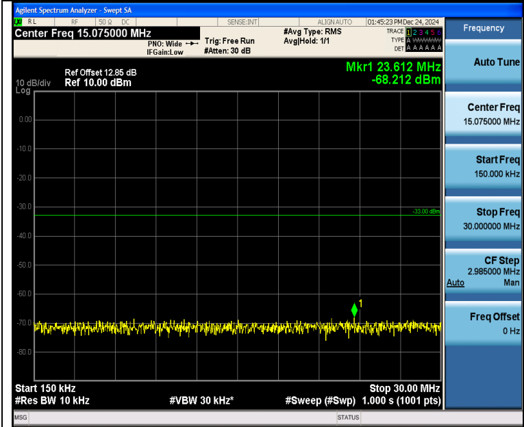
Band4_1.4MHz_QPSK_19957_1RB#5_0.15~30_0.15~30
