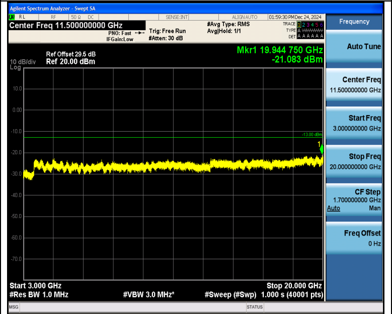
Band4_1.4MHz_QPSK_20393_1RB#5_3000~20000_3000~20000
