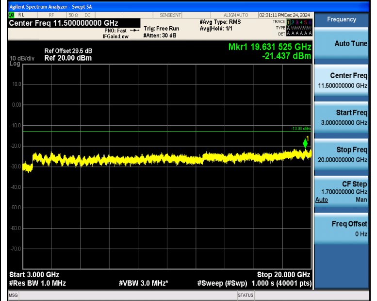
Band4_3MHz_QPSK_19965_15RB#0_3000~20000_3000~20000
