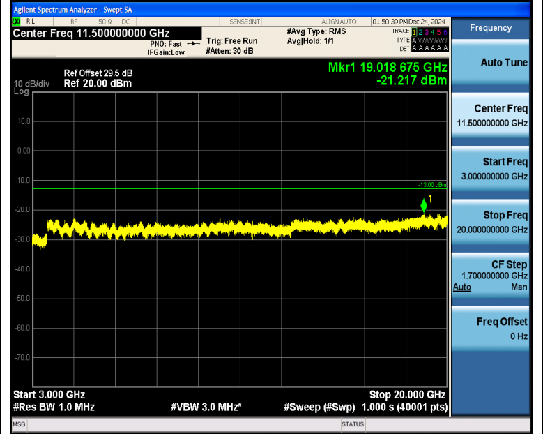
Band4_1.4MHz_QPSK_20175_1RB#0_3000~20000_3000~20000
