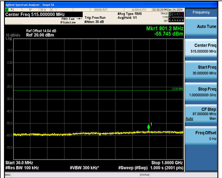
Band4_3MHz_QPSK_19965_15RB#0_30~1000_30~1000
