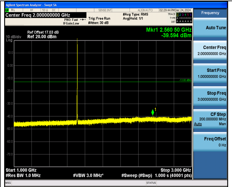
Band4_3MHz_16QAM_19965_1RB#14_1000~3000_1000~3000
