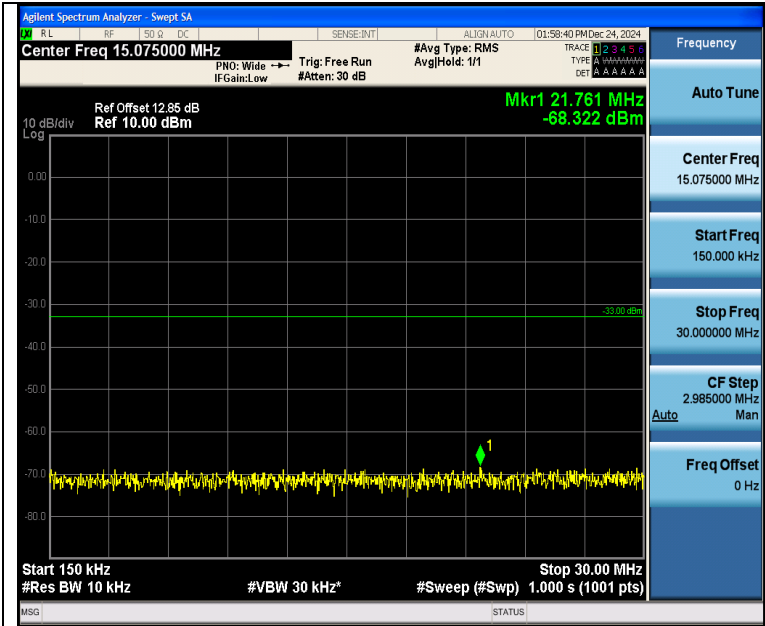
Band4_1.4MHz_QPSK_20393_1RB#5_0.15~30_0.15~30
