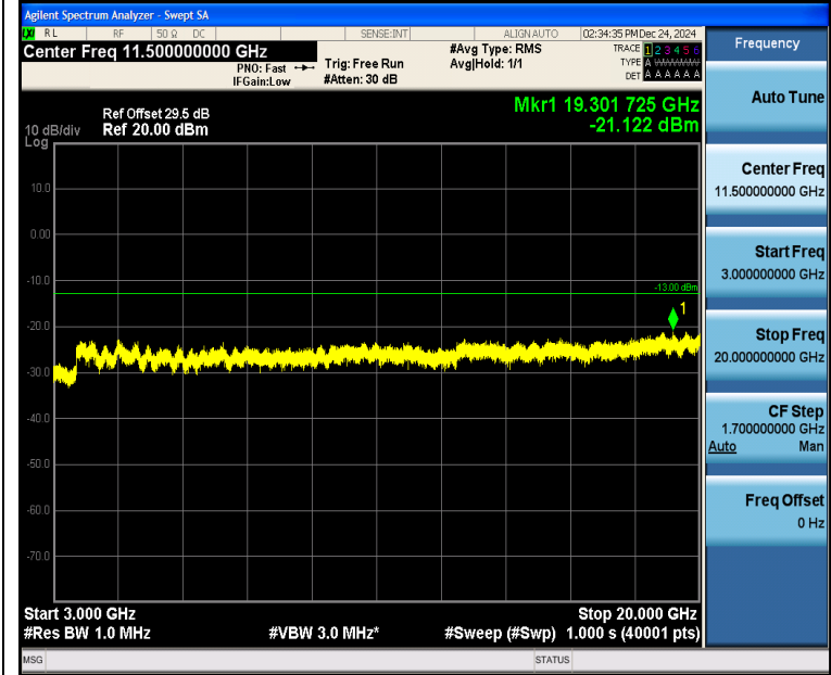
Band4_3MHz_16QAM_20175_1RB#0_3000~20000_3000~20000
