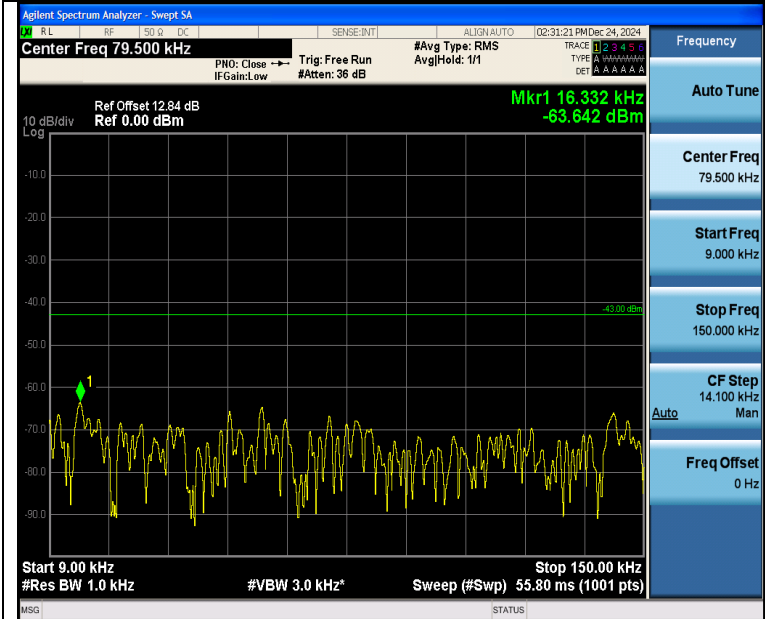
Band4_3MHz_16QAM_19965_15RB#0_0.009~0.15_0.009~0.15
