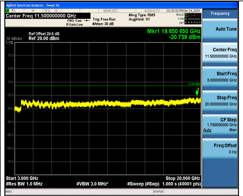
Band4_1.4MHz_QPSK_20175_1RB#5_3000~20000_3000~20000
