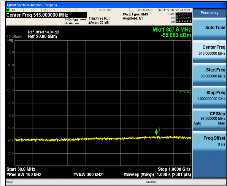
Band4_3MHz_16QAM_20175_1RB#0_30~1000_30~1000
