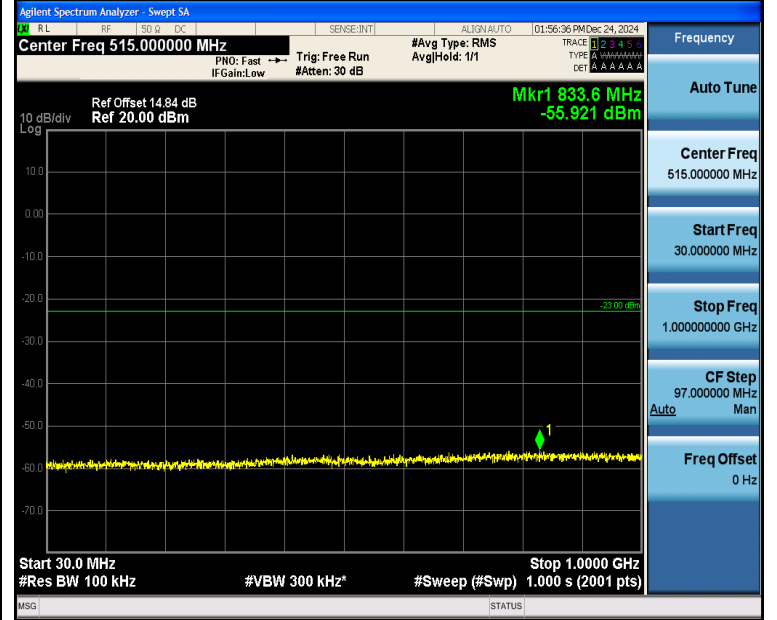
Band4_1.4MHz_QPSK_20393_1RB#0_30~1000_30~1000
