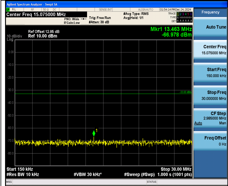
Band4_1.4MHz_QPSK_20175_6RB#0_0.15~30_0.15~30
