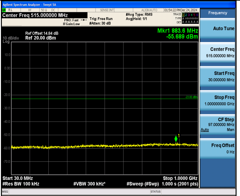
Band4_1.4MHz_QPSK_20175_6RB#0_30~1000_30~1000
