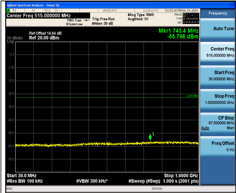
Band4_1.4MHz_16QAM_20175_1RB#5_30~1000_30~1000
