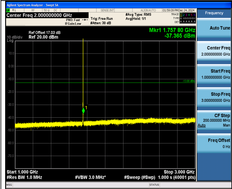
Band4_1.4MHz_QPSK_20393_1RB#5_1000~3000_1000~3000
