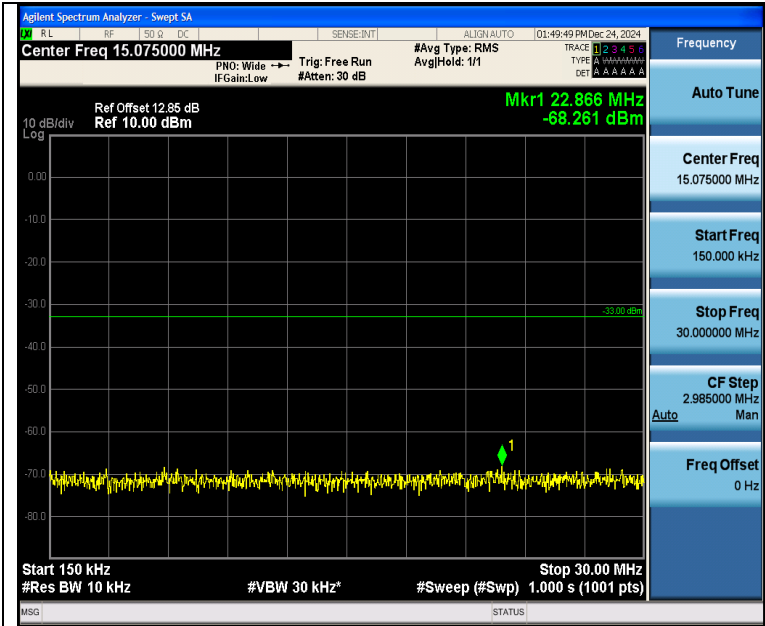
Band4_1.4MHz_QPSK_20175_1RB#0_0.15~30_0.15~30
