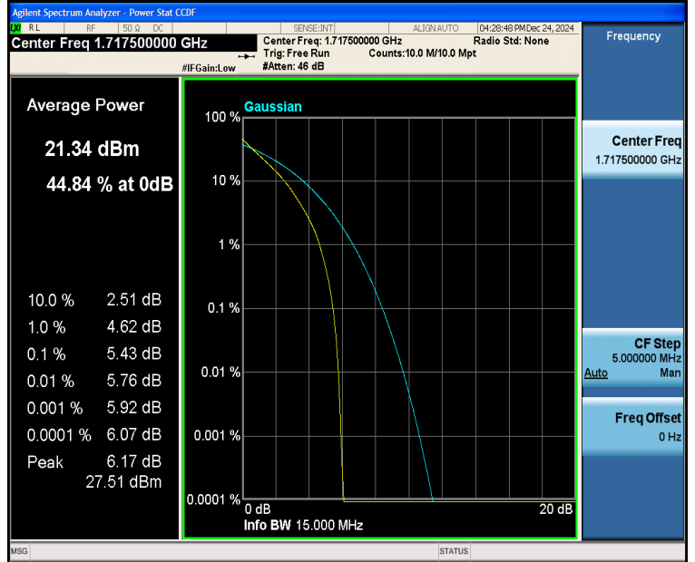
Band4-15MHz-QPSK-20025-75RB#0-PASS
