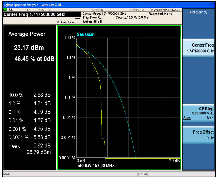
Band4-15MHz-QPSK-20325-1RB#0-PASS
