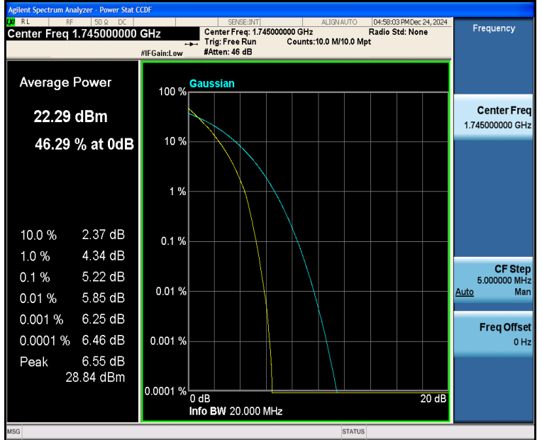
Band4-20MHz-QPSK-20300-100RB#0-PASS
