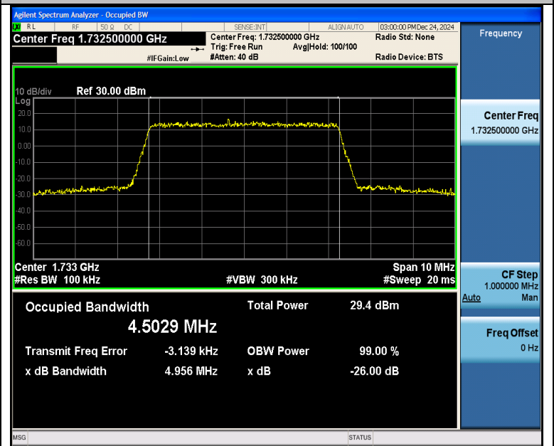
Band4-5MHz-16QAM-20175-25RB#0-PASS
