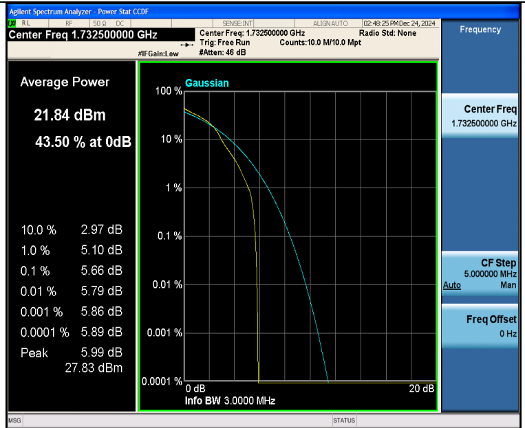
Band4-3MHz-16QAM-20175-1RB#0-PASS
