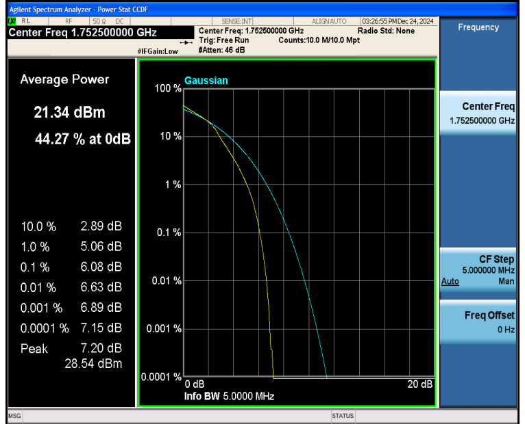
Band4-5MHz-16QAM-20375-25RB#0-PASS
