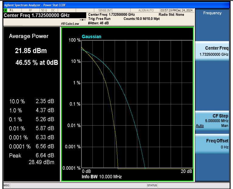
Band4-10MHz-QPSK-20175-50RB#0-PASS
