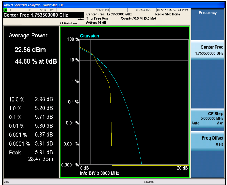
Band4-3MHz-16QAM-20385-1RB#0-PASS
