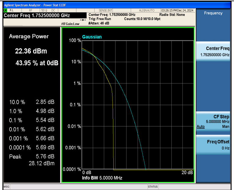
Band4-5MHz-16QAM-20375-1RB#0-PASS
