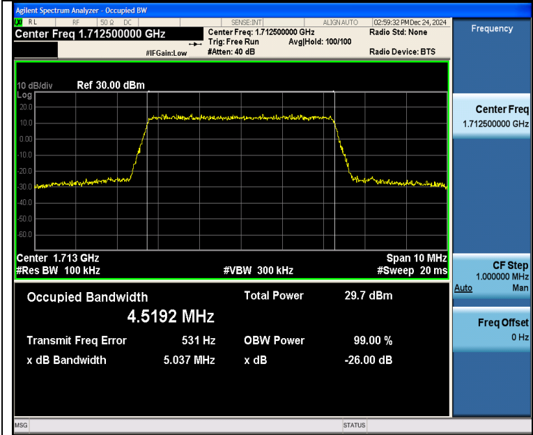
Band4-5MHz-QPSK-19975-25RB#0-PASS
