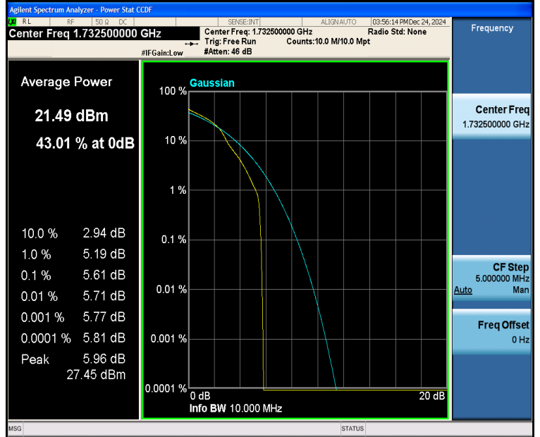
Band4-10MHz-16QAM-20175-1RB#0-PASS
