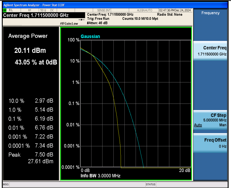
Band4-3MHz-16QAM-19965-15RB#0-PASS
