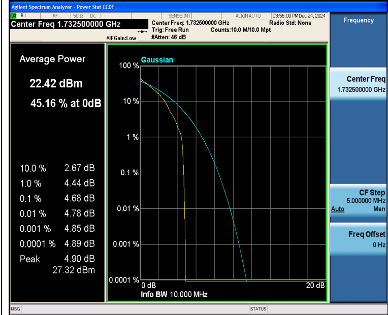
Band4-10MHz-QPSK-20175-1RB#0-PASS
