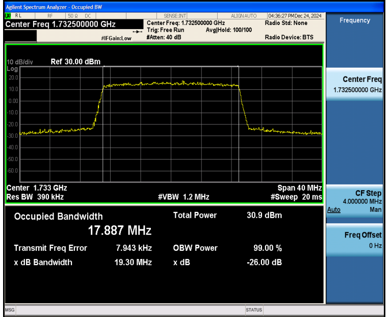
Band4-20MHz-QPSK-20175-100RB#0-PASS
