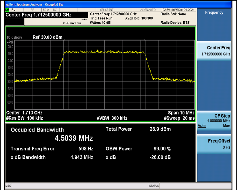
Band4-5MHz-16QAM-19975-25RB#0-PASS
