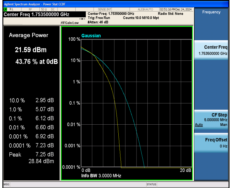
Band4-3MHz-16QAM-20385-15RB#0-PASS
