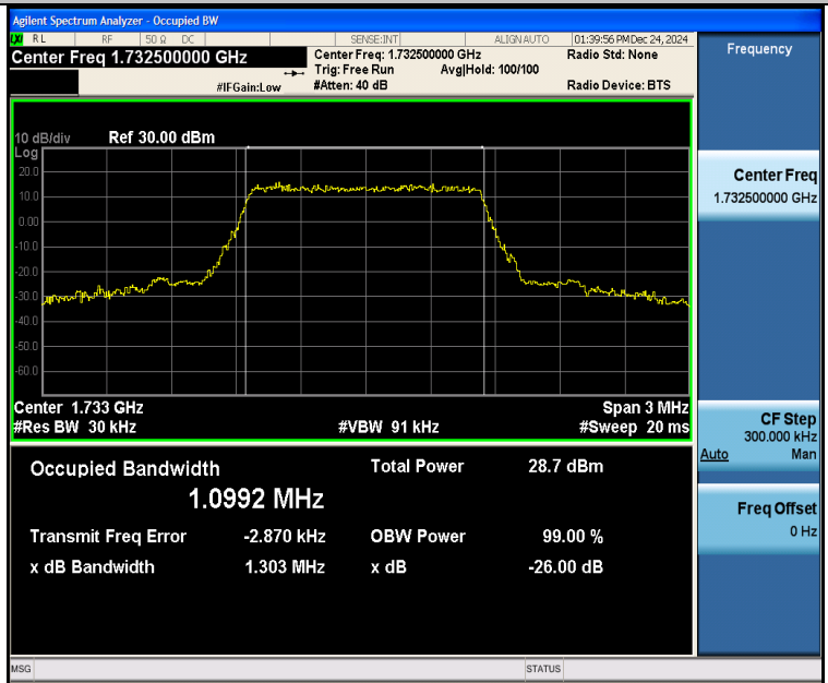
Band4-1.4MHz-16QAM-20175-6RB#0-PASS
