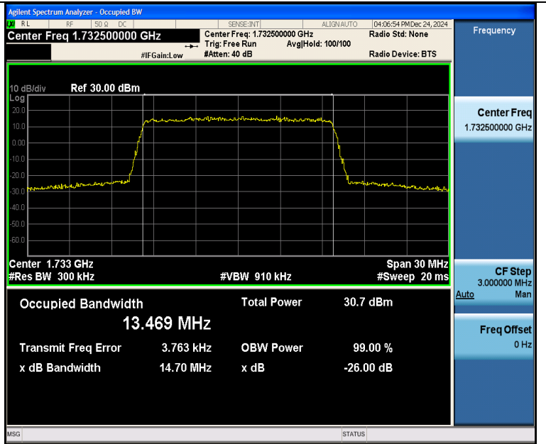
Band4-15MHz-QPSK-20175-75RB#0-PASS
