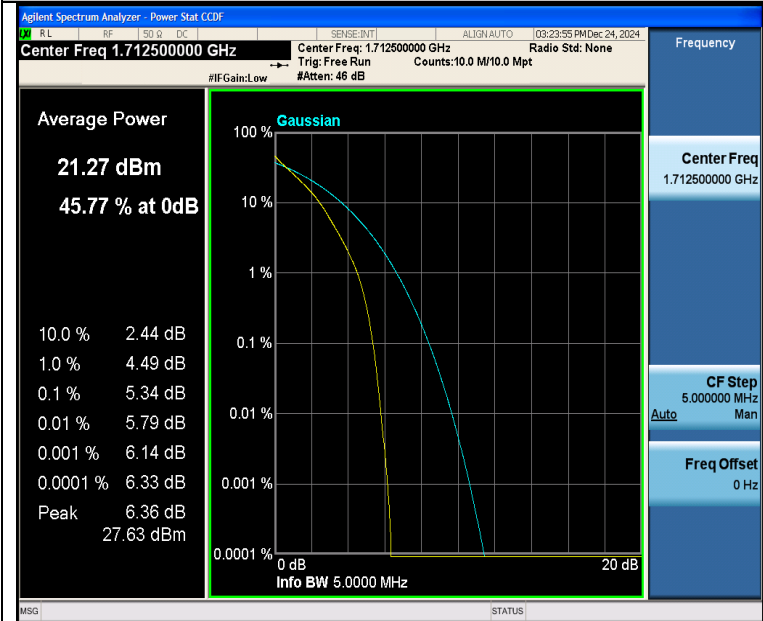
Band4-5MHz-QPSK-19975-25RB#0-PASS
