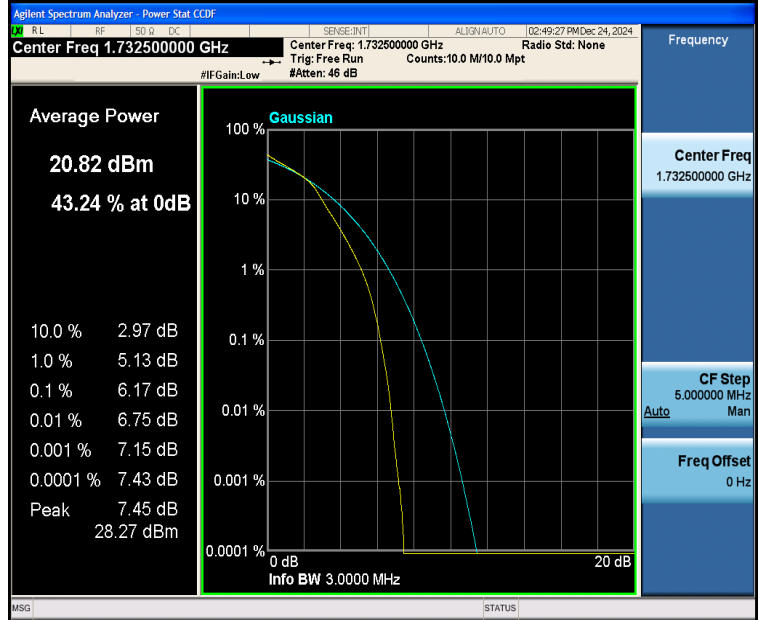
Band4-3MHz-16QAM-20175-15RB#0-PASS
