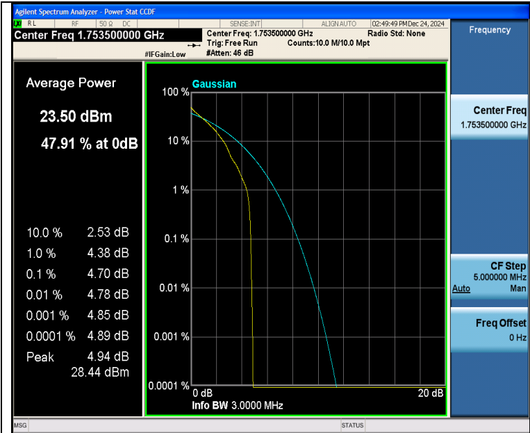
Band4-3MHz-QPSK-20385-1RB#0-PASS
