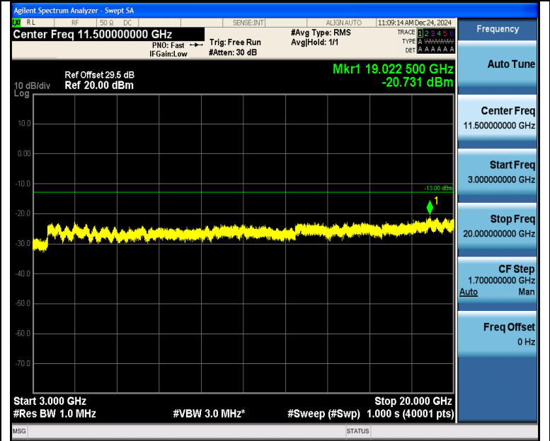
Band2_20MHz_16QAM_19100_1RB#0_3000~20000_3000~20000
