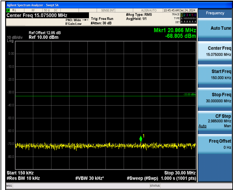
Band2_15MHz_QPSK_18900_1RB#74_0.15~30_0.15~30
