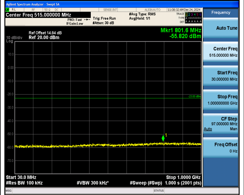
Band2_20MHz_16QAM_19100_1RB#0_30~1000_30~1000
