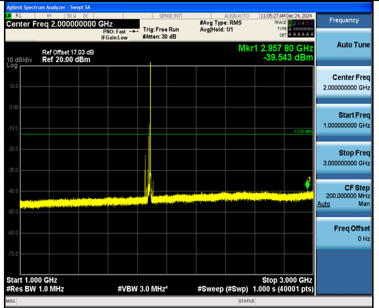
Band2_20MHz_QPSK_18900_1RB#99_1000~3000_1000~3000
