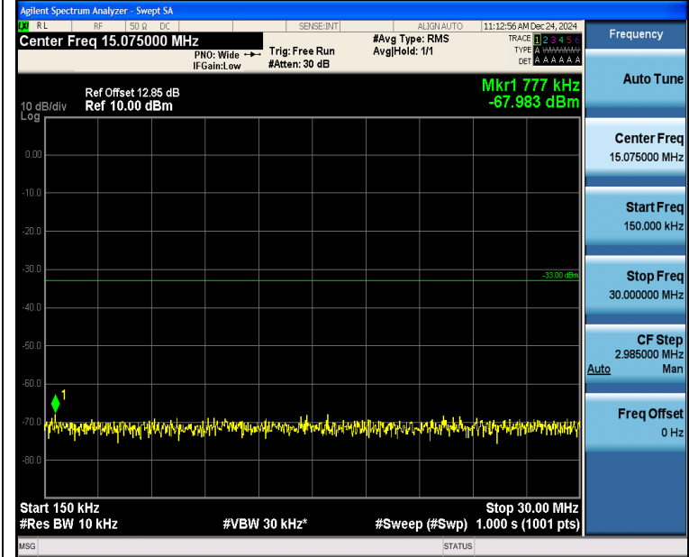
Band2_20MHz_QPSK_18900_100RB#0_0.15~30_0.15~30
