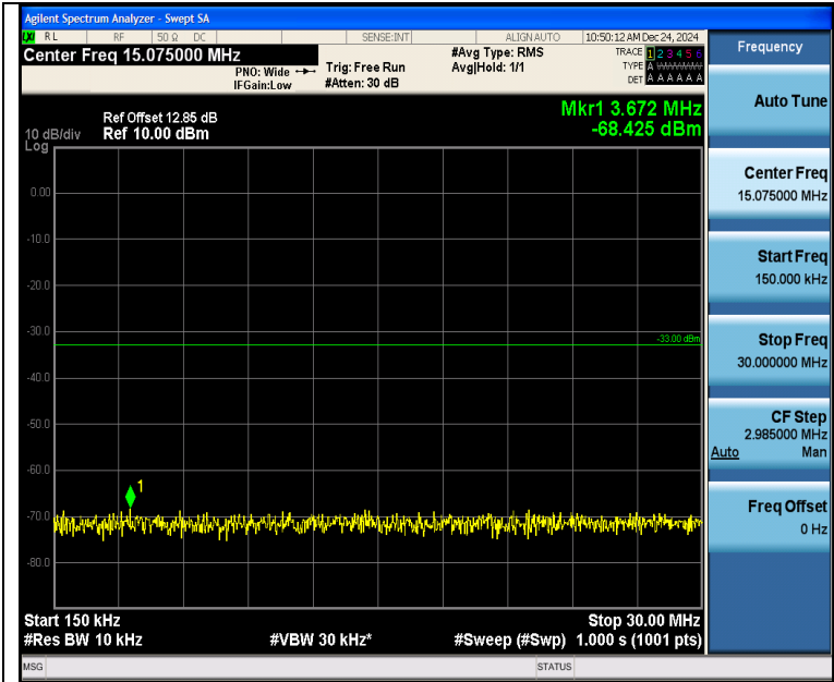
Band2_15MHz_QPSK_19125_1RB#74_0.15~30_0.15~30
