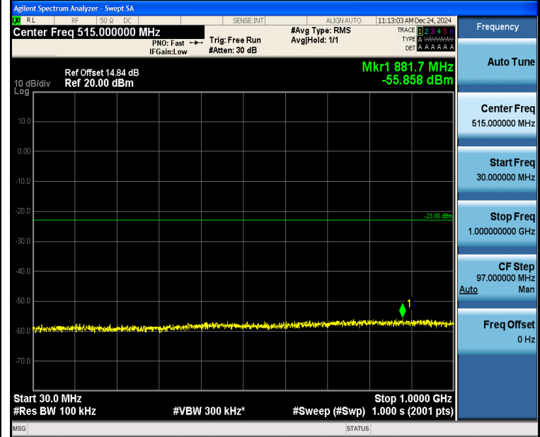
Band2_20MHz_QPSK_18900_100RB#0_30~1000_30~1000
