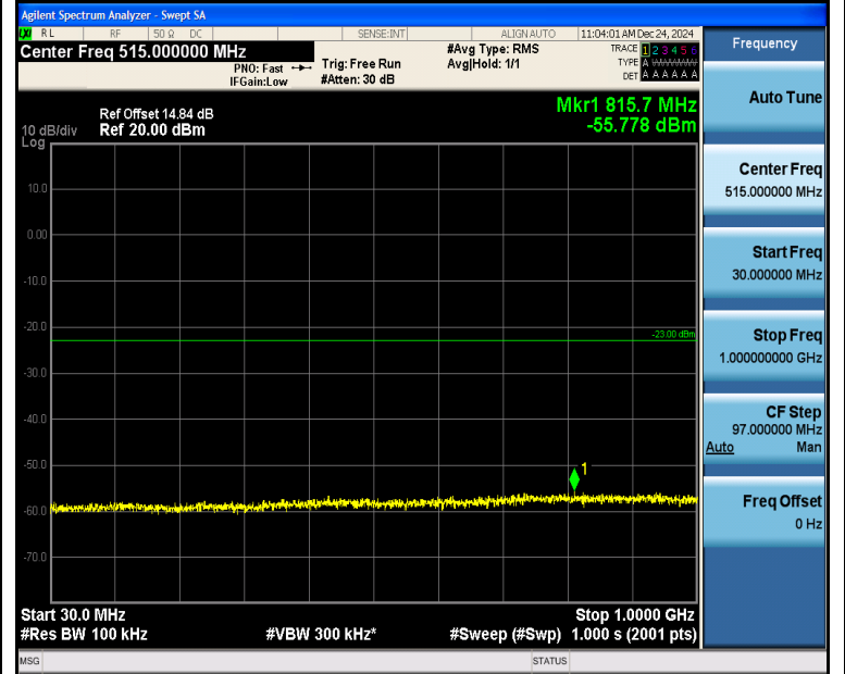
Band2_20MHz_16QAM_18900_1RB#0_30~1000_30~1000
