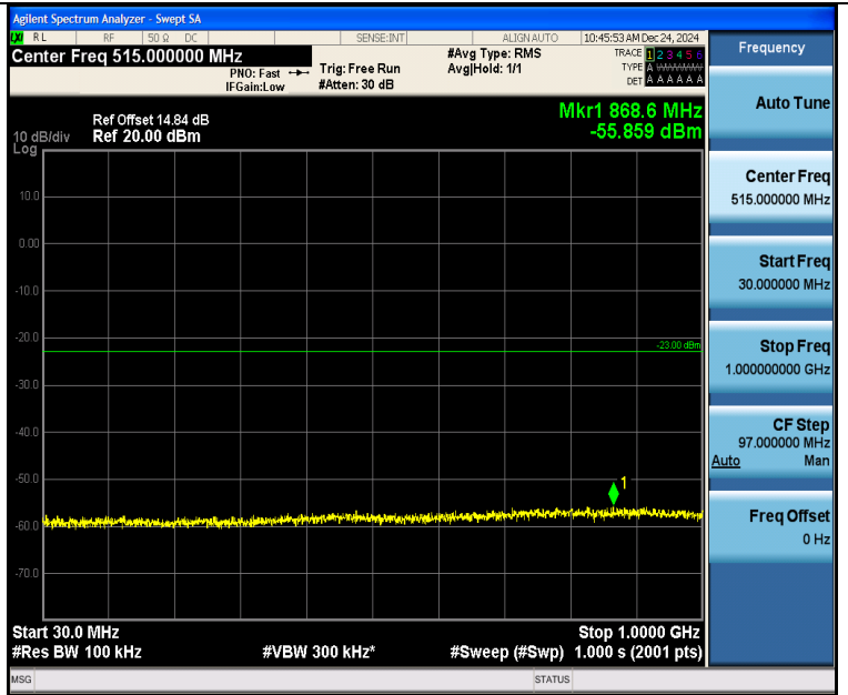
Band2_15MHz_QPSK_18900_1RB#74_30~1000_30~1000
