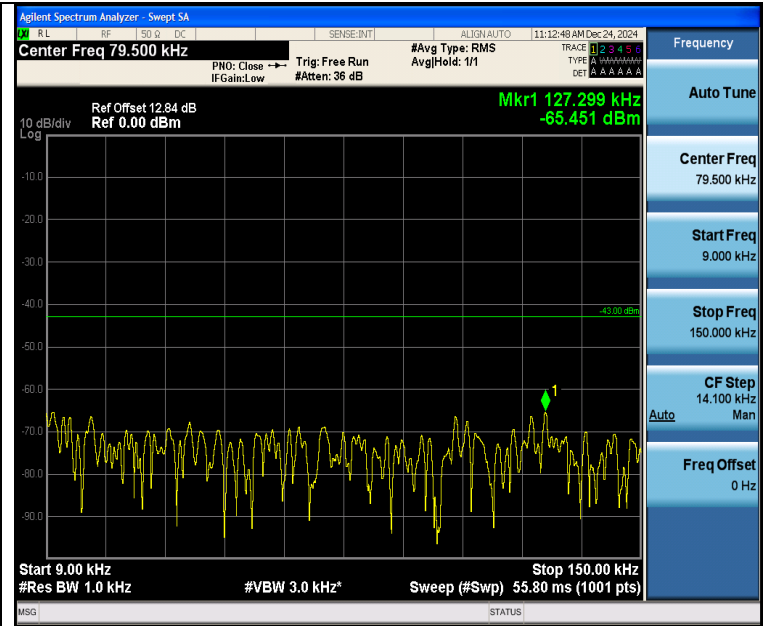
Band2_20MHz_QPSK_18900_100RB#0_0.009~0.15_0.009~0.15
