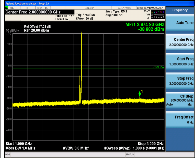
Band2_15MHz_QPSK_19125_1RB#74_1000~3000_1000~3000
