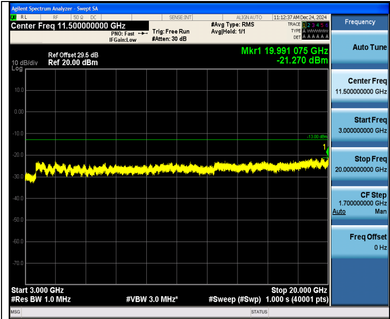
Band2_20MHz_QPSK_18700_100RB#0_3000~20000_3000~20000
