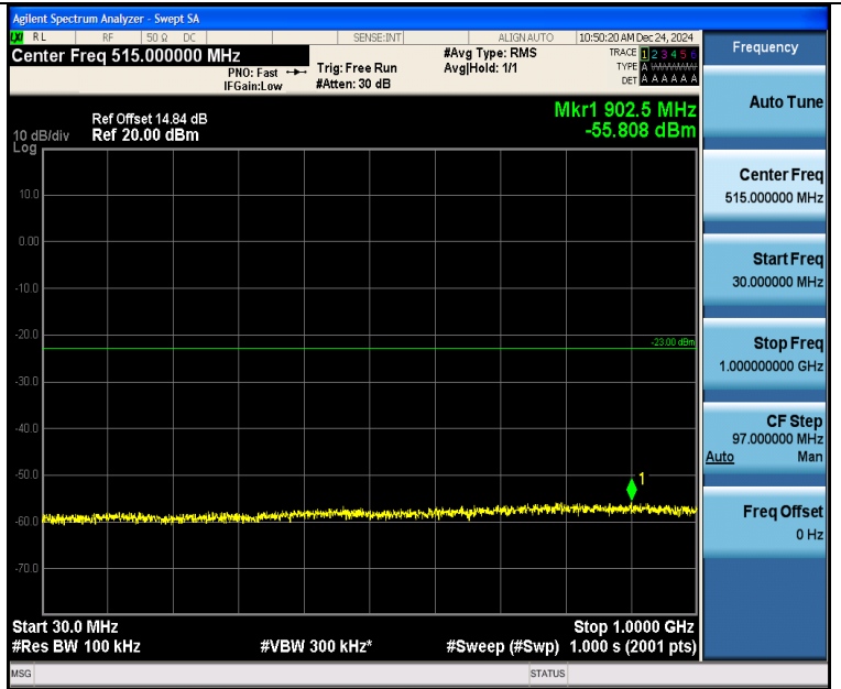
Band2_15MHz_QPSK_19125_1RB#74_30~1000_30~1000
