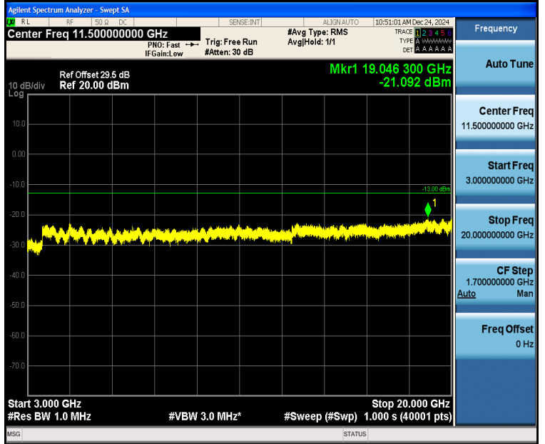
Band2_15MHz_QPSK_19125_1RB#74_3000~20000_3000~20000
