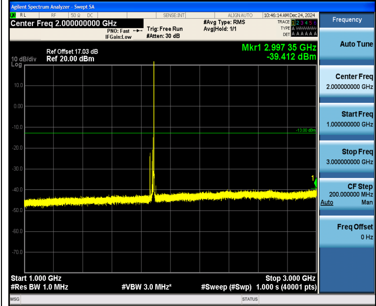
Band2_15MHz_QPSK_18900_1RB#74_1000~3000_1000~3000
