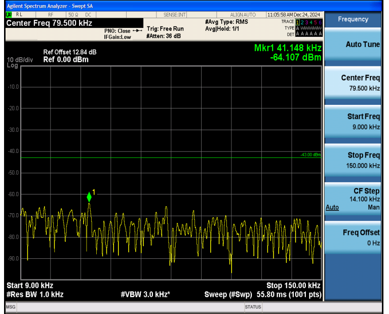
Band2_20MHz_16QAM_18900_1RB#99_0.009~0.15_0.009~0.15
