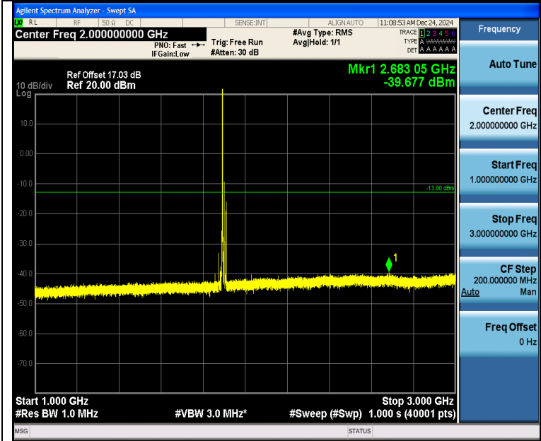
Band2_20MHz_16QAM_19100_1RB#0_1000~3000_1000~3000
