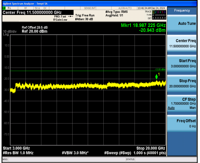
Band2_15MHz_QPSK_18900_1RB#74_3000~20000_3000~20000
