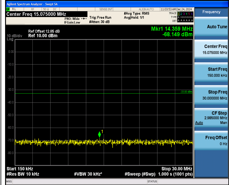
Band2_20MHz_16QAM_18900_1RB#0_0.15~30_0.15~30
