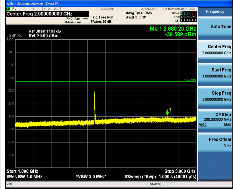
Band2_3MHz_16QAM_18900_1RB#14_1000~3000_1000~3000
