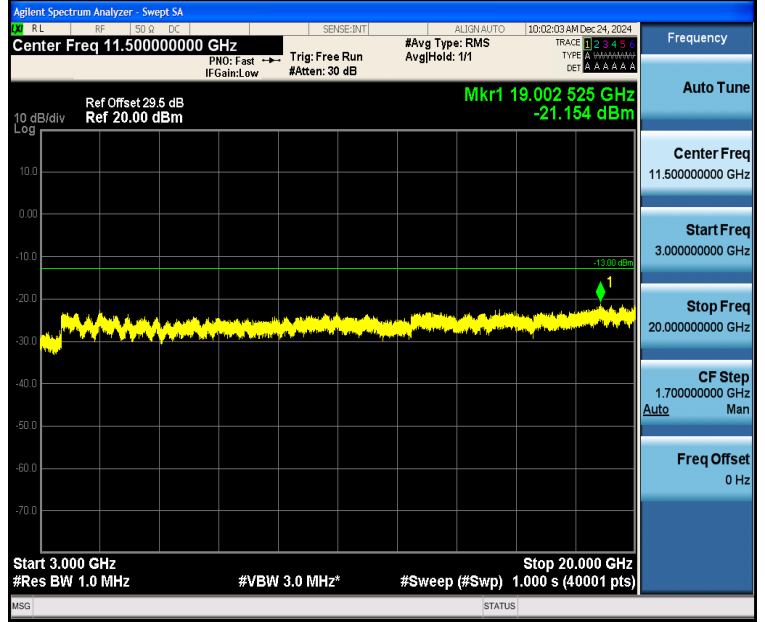
Band2_5MHz_16QAM_18625_1RB#24_3000~20000_3000~20000
