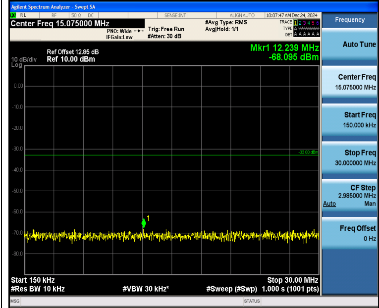
Band2_5MHz_16QAM_18900_1RB#24_0.15~30_0.15~30
