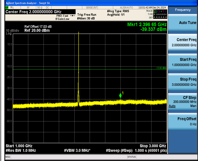
Band2_5MHz_16QAM_18625_1RB#24_1000~3000_1000~3000
