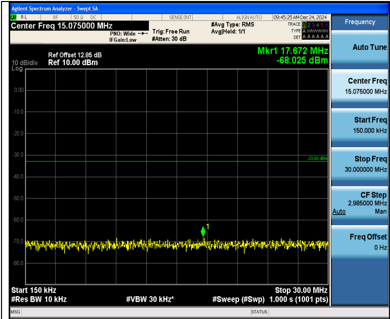
Band2_3MHz_16QAM_18900_1RB#14_0.15~30_0.15~30
