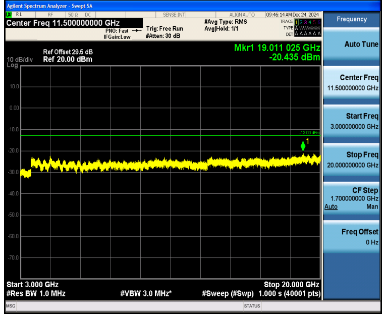
Band2_3MHz_16QAM_18900_1RB#14_3000~20000_3000~20000
