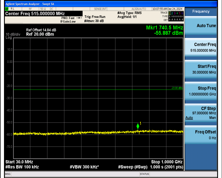
Band2_5MHz_16QAM_18900_1RB#24_30~1000_30~1000
