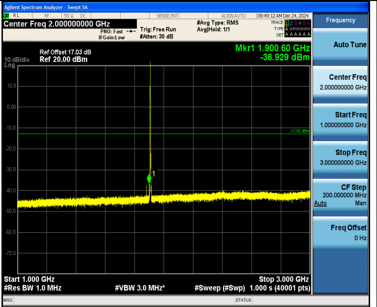
Band2_3MHz_QPSK_19185_1RB#0_1000~3000_1000~3000
