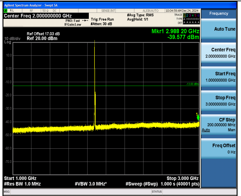
Band2_5MHz_QPSK_18900_1RB#0_1000~3000_1000~3000
