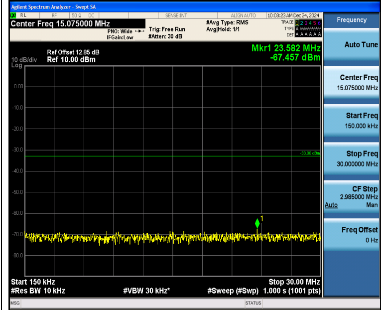
Band2_5MHz_16QAM_18625_25RB#0_0.15~30_0.15~30
