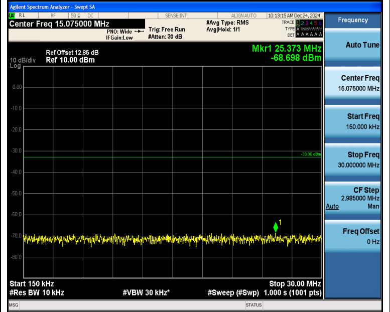
Band2_5MHz_QPSK_19175_1RB#24_0.15~30_0.15~30
