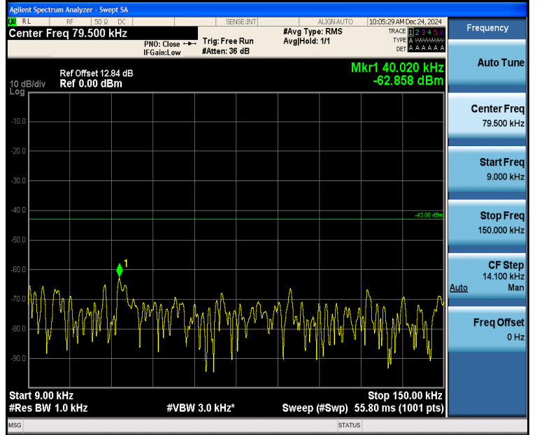
Band2_5MHz_16QAM_18900_1RB#0_0.009~0.15_0.009~0.15
