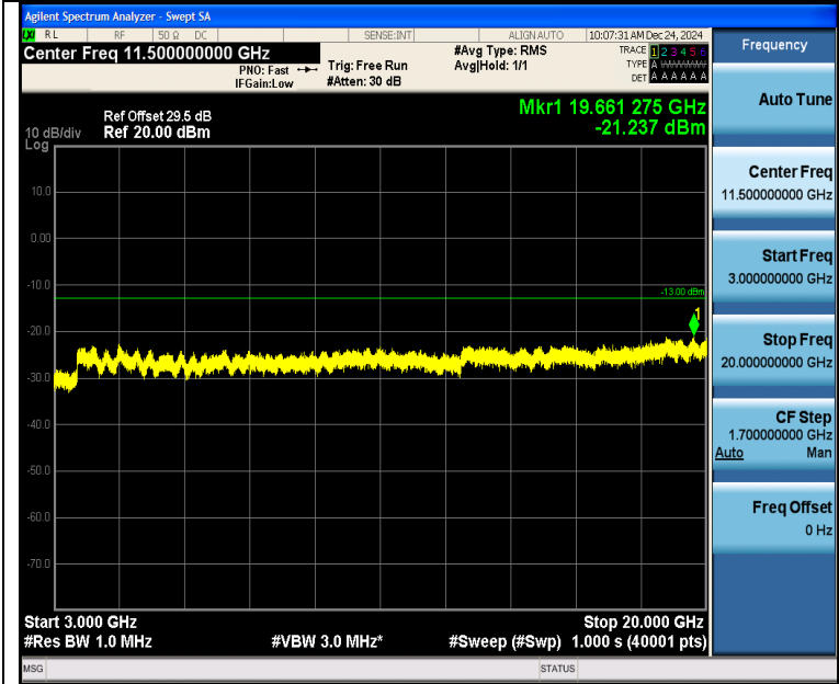
Band2_5MHz_QPSK_18900_1RB#24_3000~20000_3000~20000
