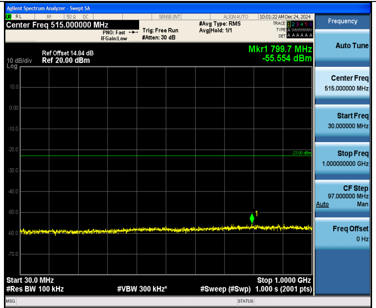
Band2_5MHz_16QAM_18625_1RB#24_30~1000_30~1000
