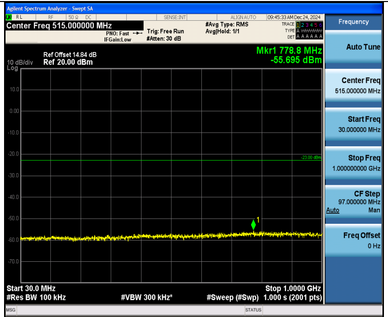
Band2_3MHz_16QAM_18900_1RB#14_30~1000_30~1000
