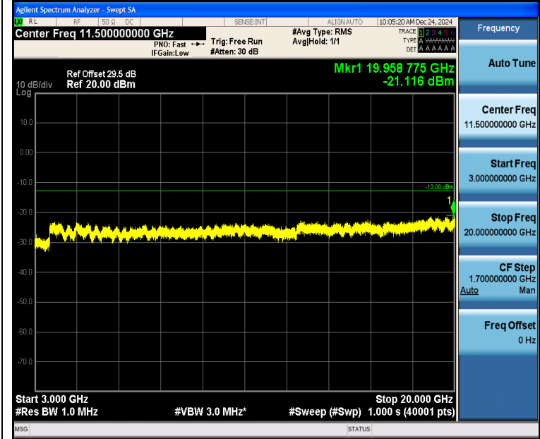
Band2_5MHz_QPSK_18900_1RB#0_3000~20000_3000~20000
