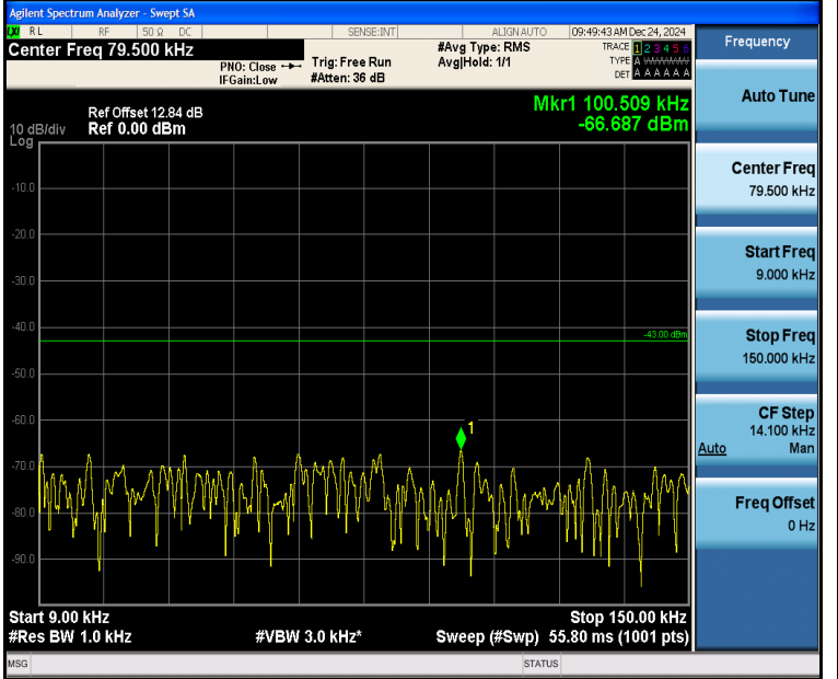
Band2_3MHz_16QAM_19185_1RB#0_0.009~0.15_0.009~0.15
