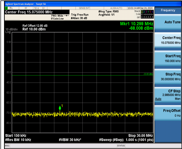
Band2_5MHz_16QAM_18625_1RB#24_0.15~30_0.15~30
