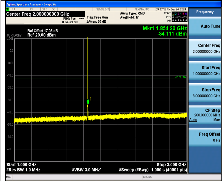
Band2_1.4MHz_16QAM_18607_6RB#0_1000~3000_1000~3000
