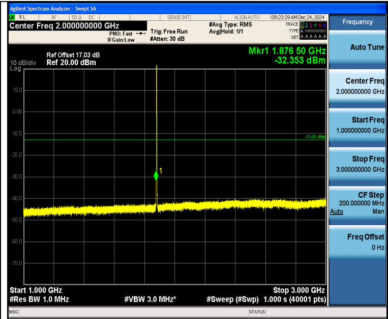
Band2_1.4MHz_QPSK_18900_6RB#0_1000~3000_1000~3000
