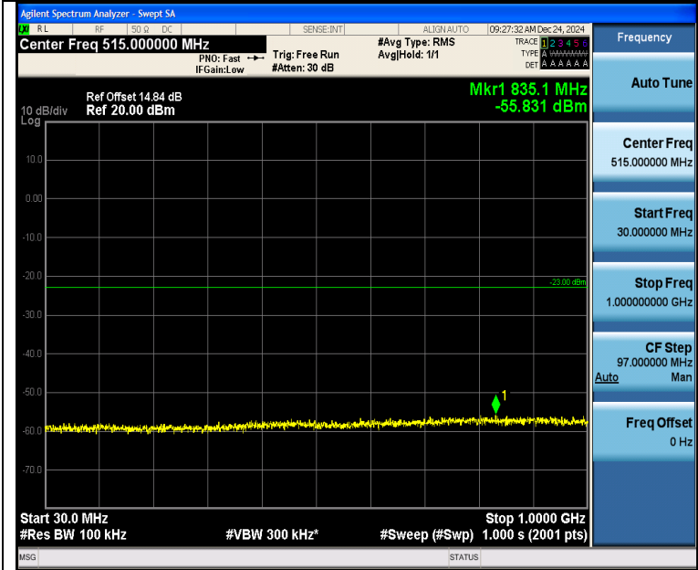
Band2_1.4MHz_QPSK_19193_1RB#5_30~1000_30~1000
