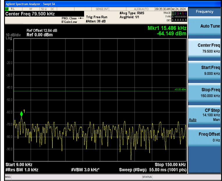
Band2_3MHz_16QAM_18615_1RB#0_0.009~0.15_0.009~0.15
