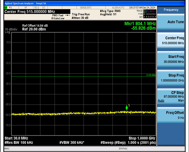
Band2_3MHz_16QAM_18615_1RB#14_30~1000_30~1000
