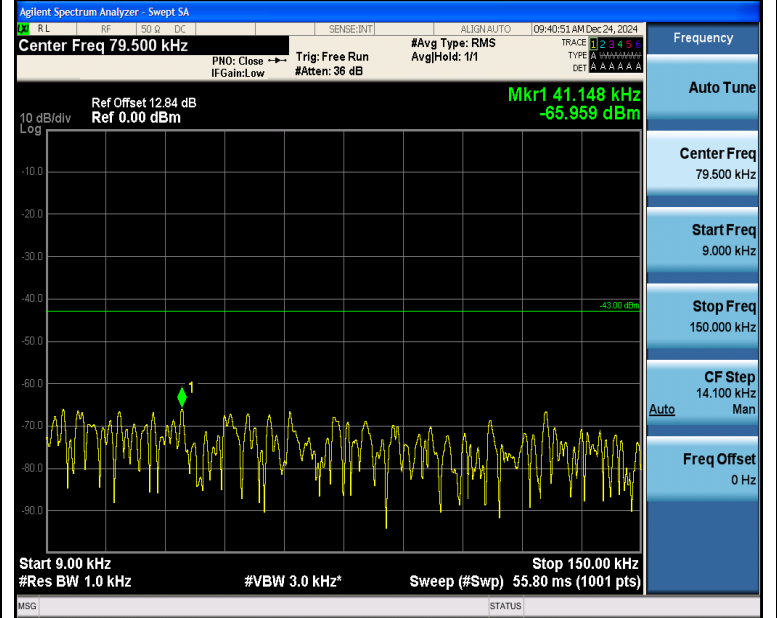
Band2_3MHz_16QAM_18615_15RB#0_0.009~0.15_0.009~0.15
