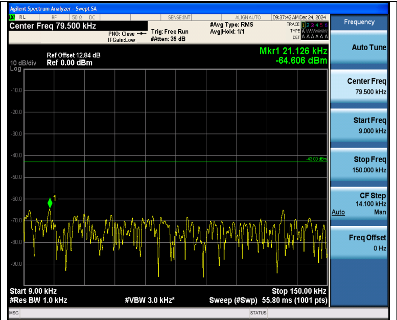
Band2_3MHz_16QAM_18615_1RB#14_0.009~0.15_0.009~0.15
