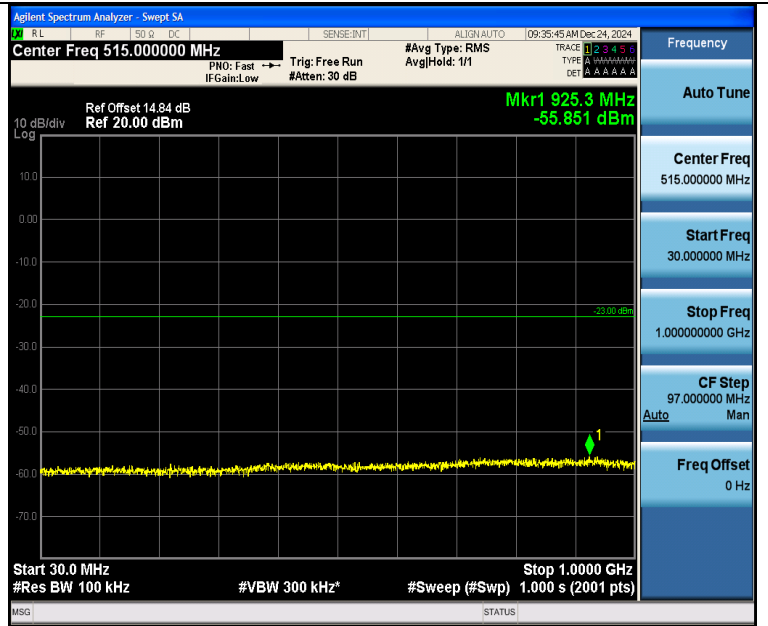
Band2_3MHz_16QAM_18615_1RB#0_30~1000_30~1000
