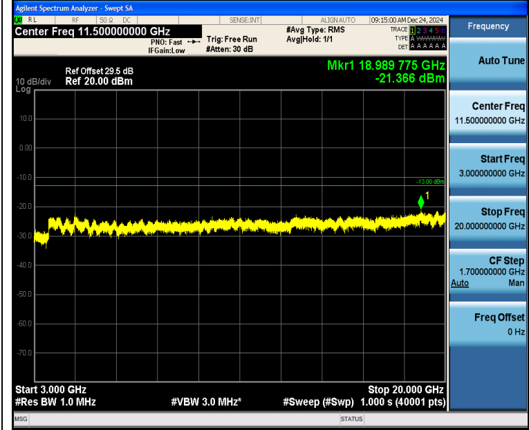
Band2_1.4MHz_QPSK_18607_1RB#5_3000~20000_3000~20000
