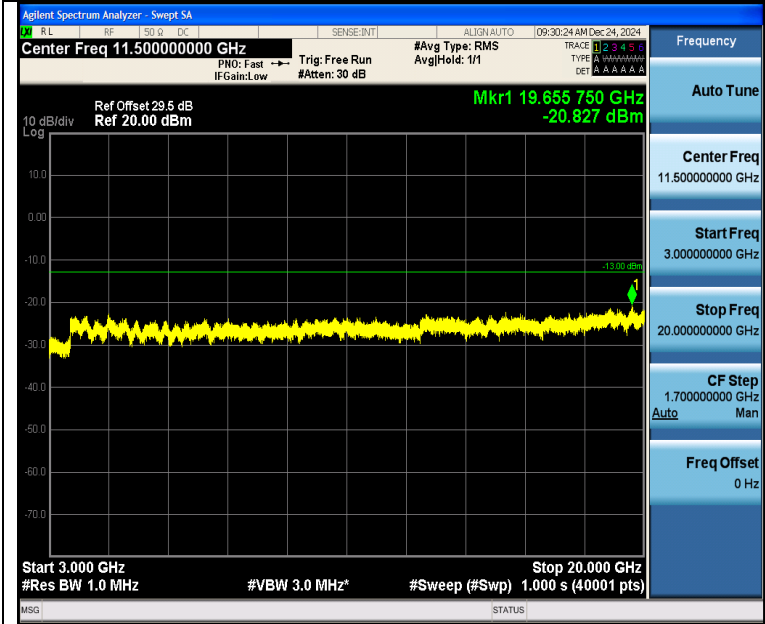
Band2_1.4MHz_QPSK_19193_6RB#0_3000~20000_3000~20000
