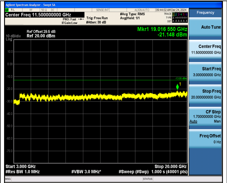
Band2_3MHz_16QAM_18900_1RB#0_3000~20000_3000~20000
