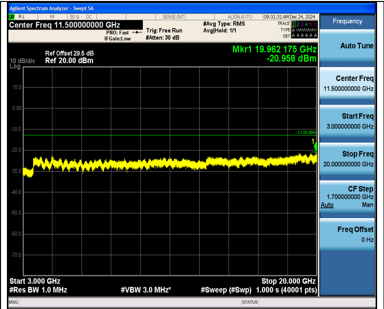
Band2_1.4MHz_16QAM_19193_6RB#0_3000~20000_3000~20000
