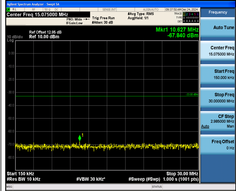
Band2_3MHz_16QAM_18615_1RB#14_0.15~30_0.15~30
