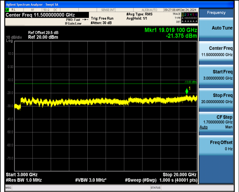
Band2_1.4MHz_16QAM_19193_1RB#0_3000~20000_3000~20000
