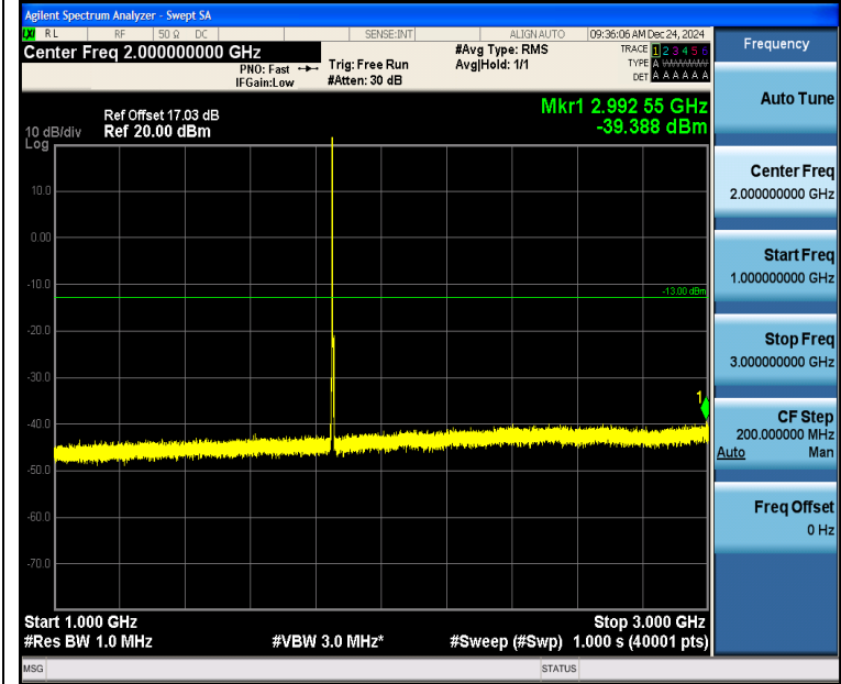
Band2_3MHz_16QAM_18615_1RB#0_1000~3000_1000~3000
