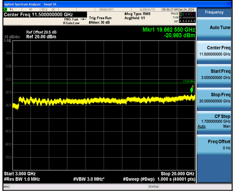
Band2_3MHz_16QAM_18615_1RB#0_3000~20000_3000~20000
