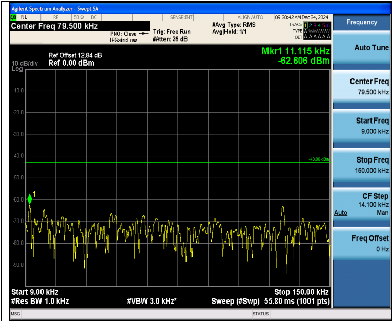
Band2_1.4MHz_QPSK_18900_1RB#5_0.009~0.15_0.009~0.15
