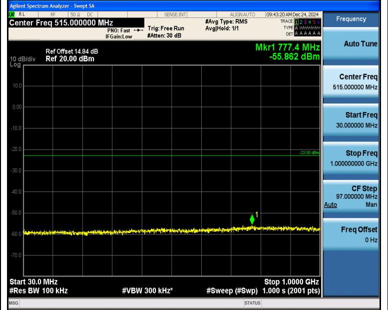
Band2_3MHz_16QAM_18900_1RB#0_30~1000_30~1000
