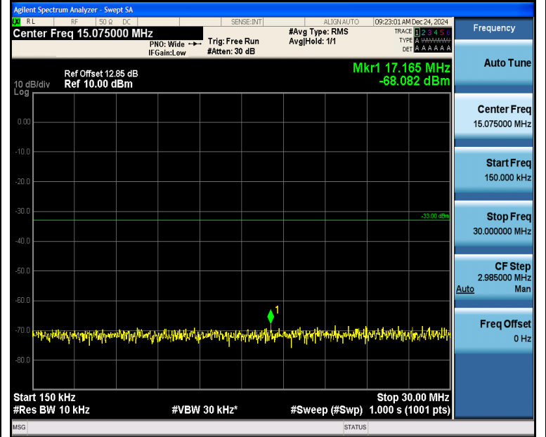
Band2_1.4MHz_QPSK_18900_6RB#0_0.15~30_0.15~30
