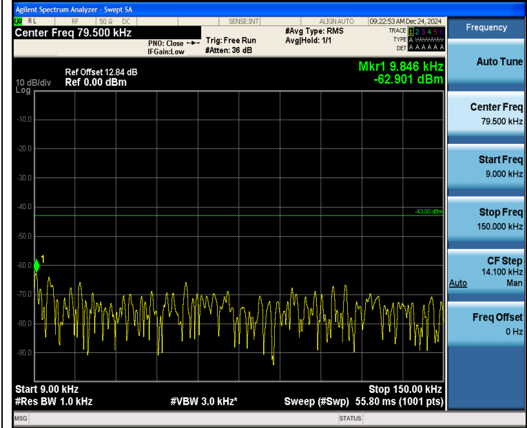
Band2_1.4MHz_QPSK_18900_6RB#0_0.009~0.15_0.009~0.15
