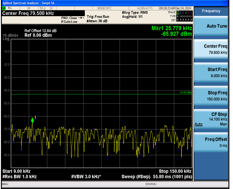
Band2_1.4MHz_16QAM_19193_1RB#5_0.009~0.15_0.009~0.15
