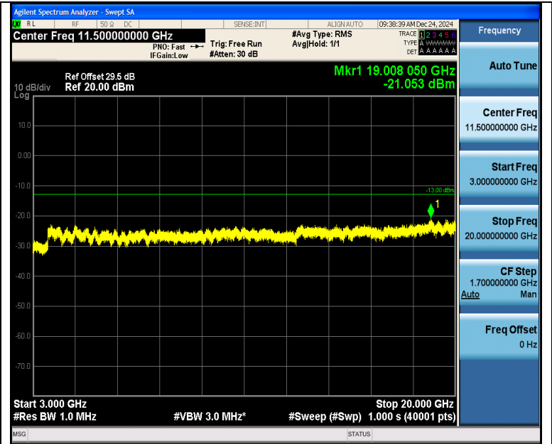
Band2_3MHz_16QAM_18615_1RB#14_3000~20000_3000~20000
