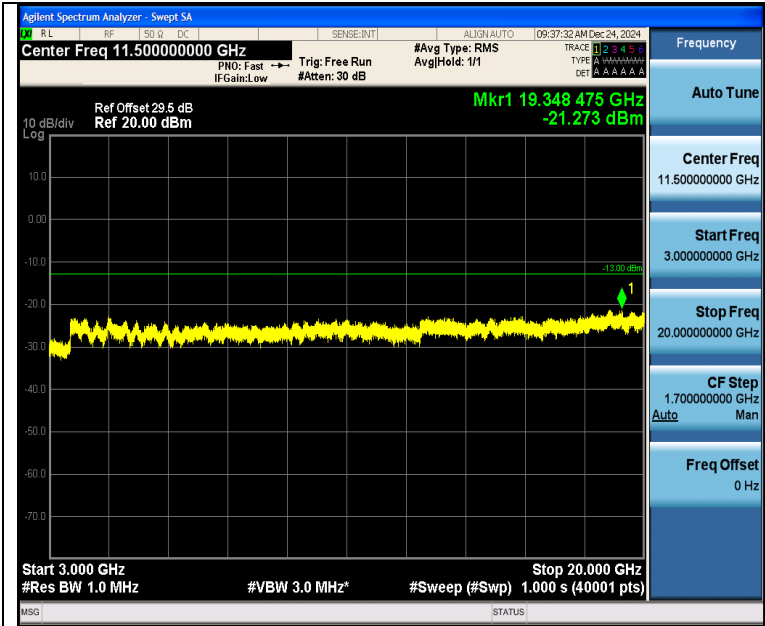
Band2_3MHz_QPSK_18615_1RB#14_3000~20000_3000~20000
