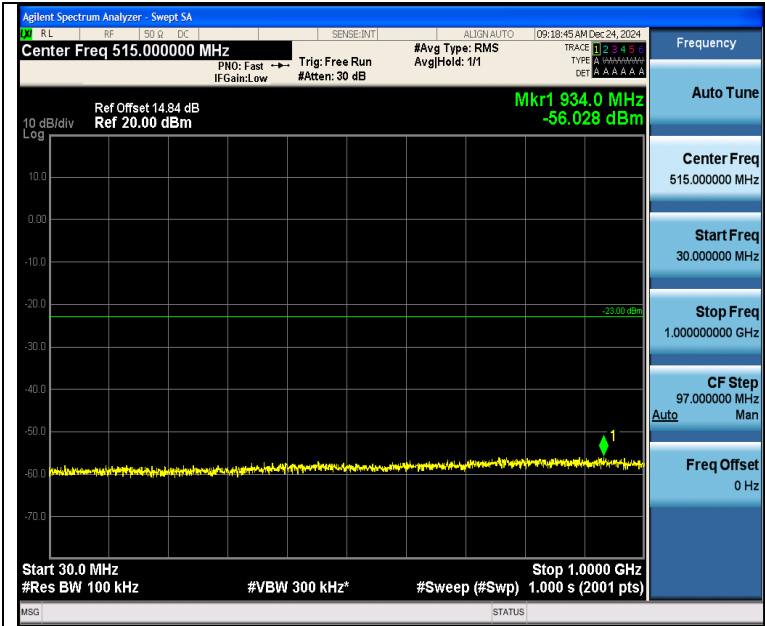
Band2_1.4MHz_QPSK_18900_1RB#0_30~1000_30~1000
