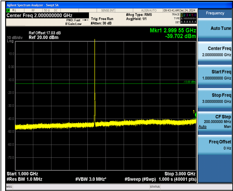
Band2_3MHz_16QAM_18900_1RB#0_1000~3000_1000~3000
