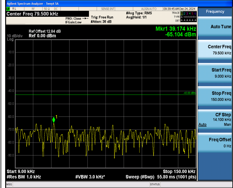
Band2_3MHz_QPSK_18615_15RB#0_0.009~0.15_0.009~0.15
