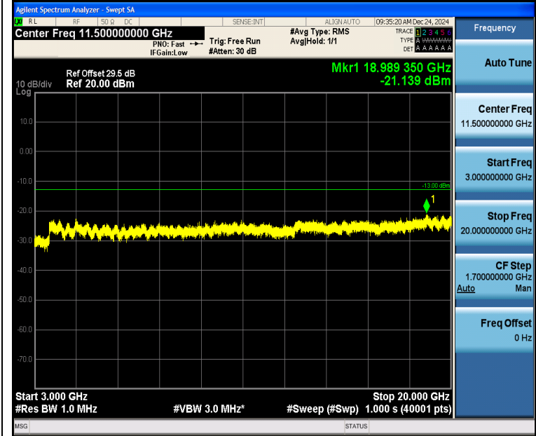
Band2_3MHz_QPSK_18615_1RB#0_3000~20000_3000~20000
