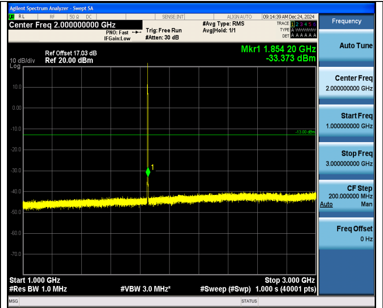
Band2_1.4MHz_QPSK_18607_1RB#5_1000~3000_1000~3000
