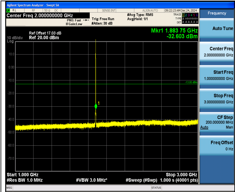
Band2_1.4MHz_16QAM_18900_1RB#5_1000~3000_1000~3000
