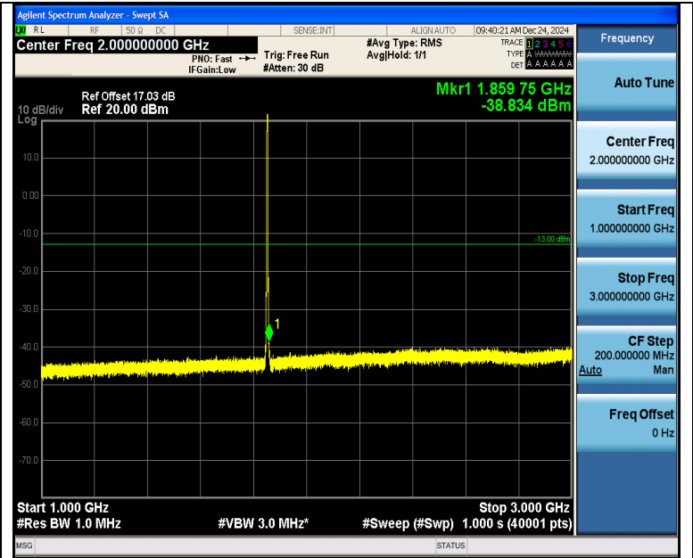
Band2_3MHz_QPSK_18615_15RB#0_1000~3000_1000~3000
