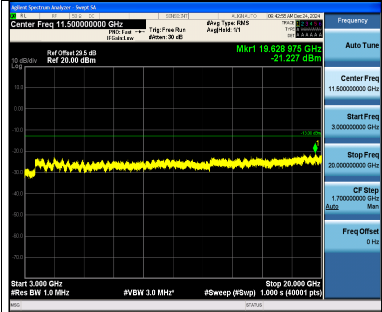
Band2_3MHz_QPSK_18900_1RB#0_3000~20000_3000~20000
