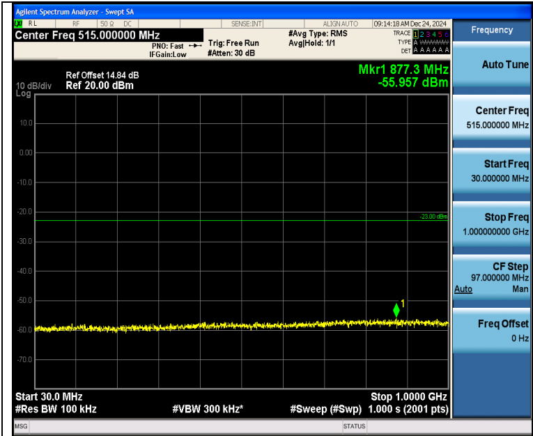
Band2_1.4MHz_QPSK_18607_1RB#5_30~1000_30~1000
