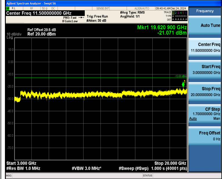
Band2_3MHz_QPSK_18615_15RB#0_3000~20000_3000~20000
