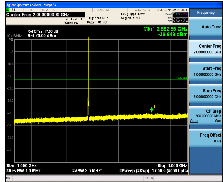
Band2_3MHz_16QAM_18615_1RB#14_1000~3000_1000~3000
