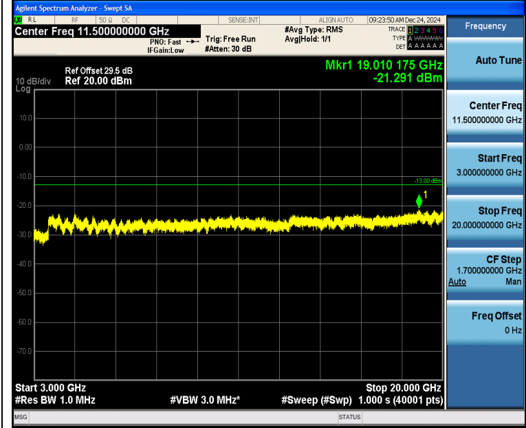
Band2_1.4MHz_QPSK_18900_6RB#0_3000~20000_3000~20000
