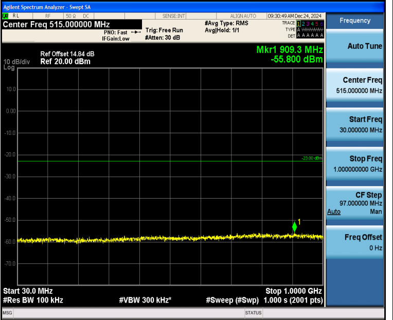
Band2_1.4MHz_16QAM_19193_6RB#0_30~1000_30~1000
