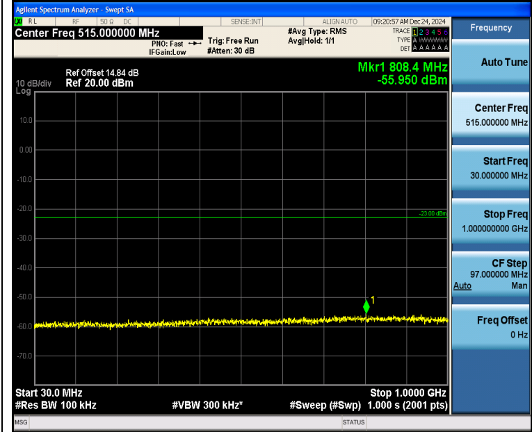
Band2_1.4MHz_QPSK_18900_1RB#5_30~1000_30~1000
