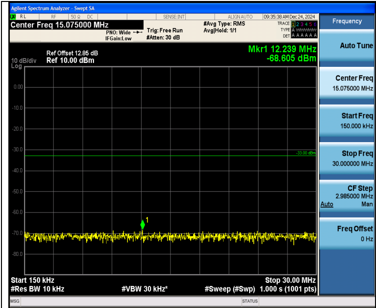
Band2_3MHz_16QAM_18615_1RB#0_0.15~30_0.15~30
