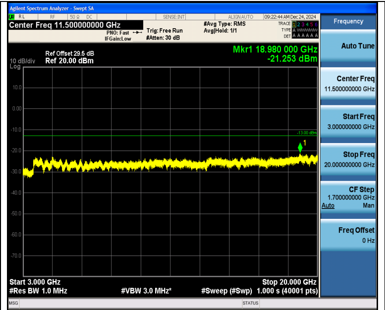
Band2_1.4MHz_16QAM_18900_1RB#5_3000~20000_3000~20000
