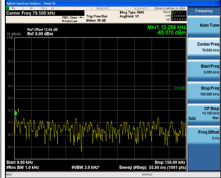
Band2_3MHz_QPSK_18900_1RB#14_0.009~0.15_0.009~0.15
