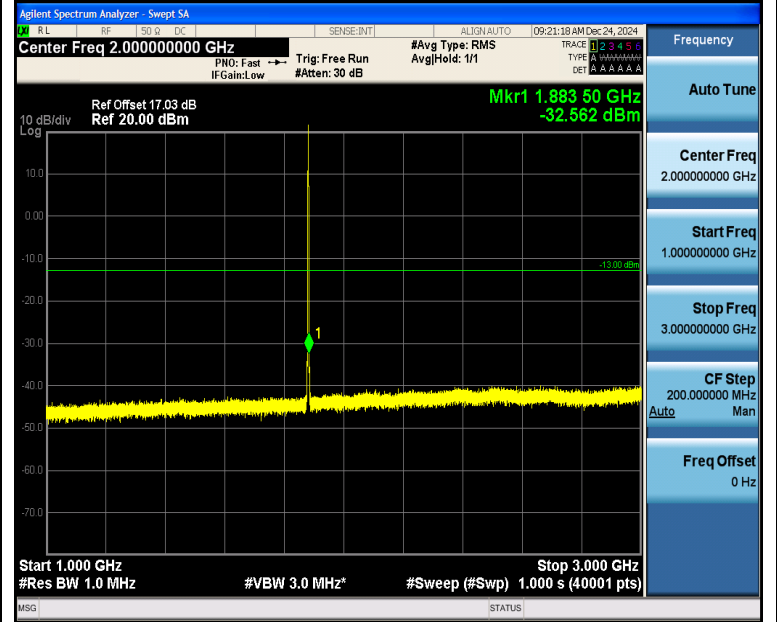
Band2_1.4MHz_QPSK_18900_1RB#5_1000~3000_1000~3000
