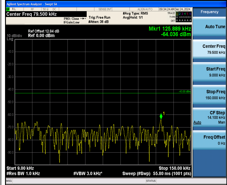
Band2_3MHz_QPSK_18615_1RB#0_0.009~0.15_0.009~0.15
