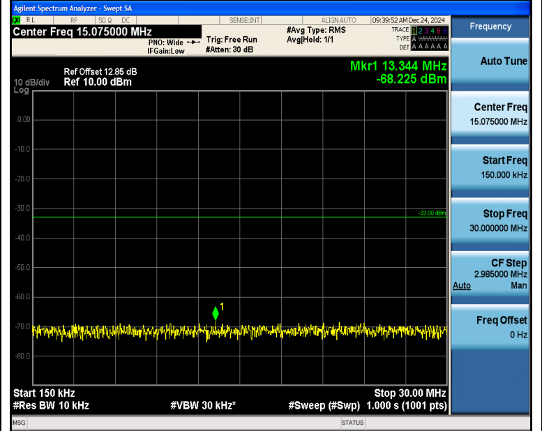
Band2_3MHz_QPSK_18615_15RB#0_0.15~30_0.15~30
