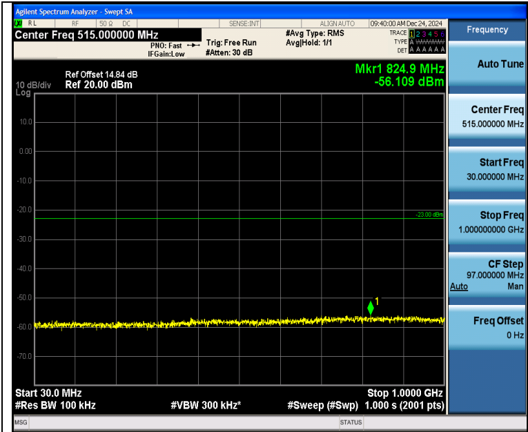
Band2_3MHz_QPSK_18615_15RB#0_30~1000_30~1000
