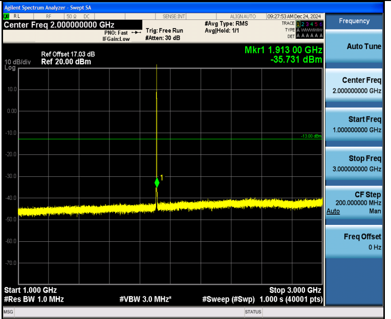
Band2_1.4MHz_QPSK_19193_1RB#5_1000~3000_1000~3000
