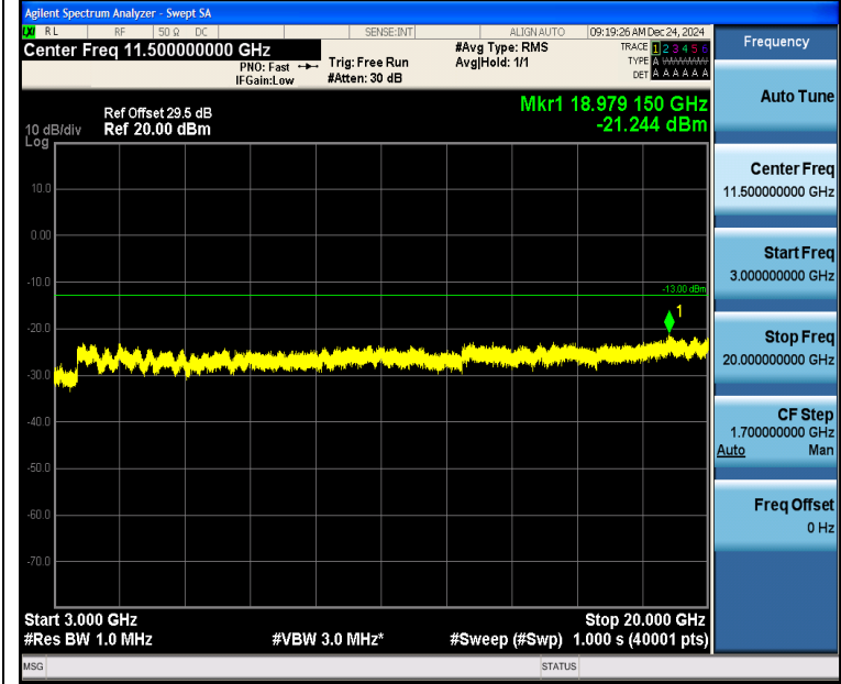
Band2_1.4MHz_QPSK_18900_1RB#0_3000~20000_3000~20000
