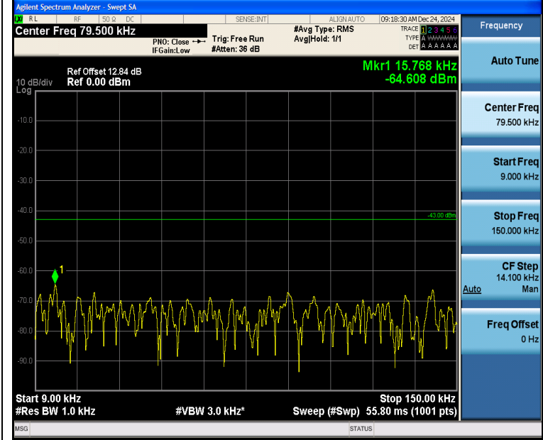
Band2_1.4MHz_QPSK_18900_1RB#0_0.009~0.15_0.009~0.15
