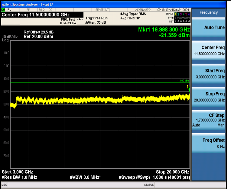
Band2_1.4MHz_16QAM_18607_6RB#0_3000~20000_3000~20000
