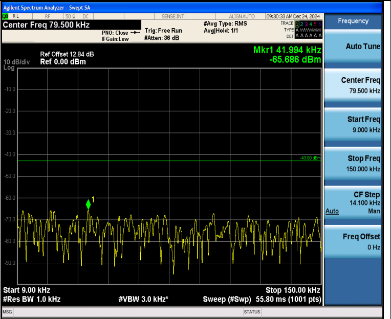
Band2_1.4MHz_16QAM_19193_6RB#0_0.009~0.15_0.009~0.15
