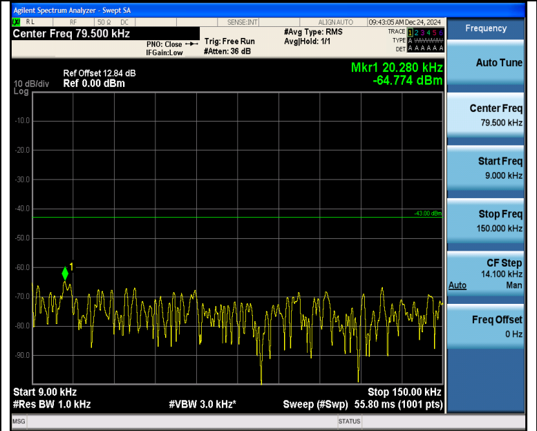
Band2_3MHz_16QAM_18900_1RB#0_0.009~0.15_0.009~0.15
