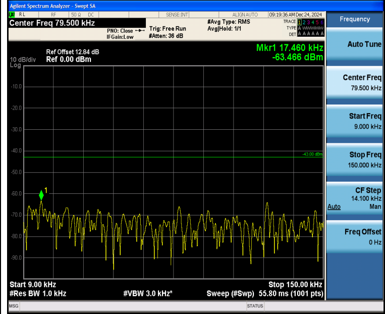
Band2_1.4MHz_16QAM_18900_1RB#0_0.009~0.15_0.009~0.15
