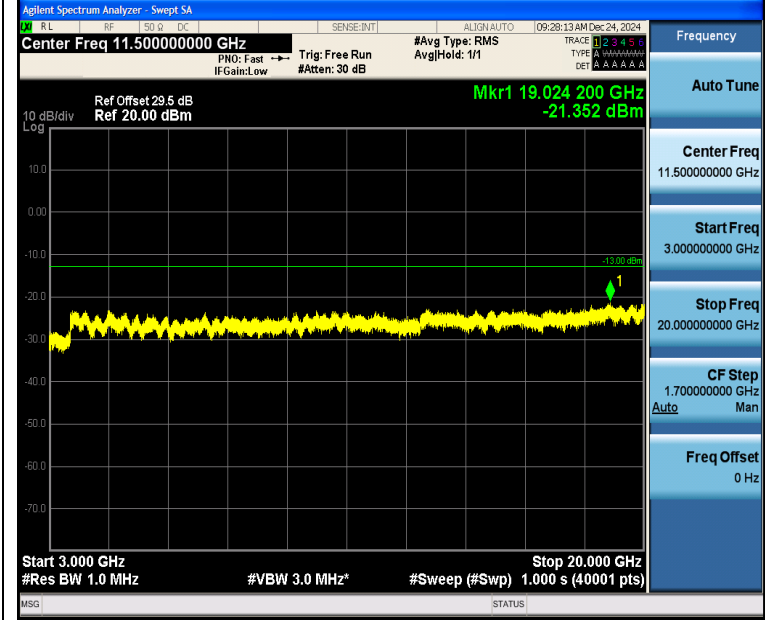
Band2_1.4MHz_QPSK_19193_1RB#5_3000~20000_3000~20000
