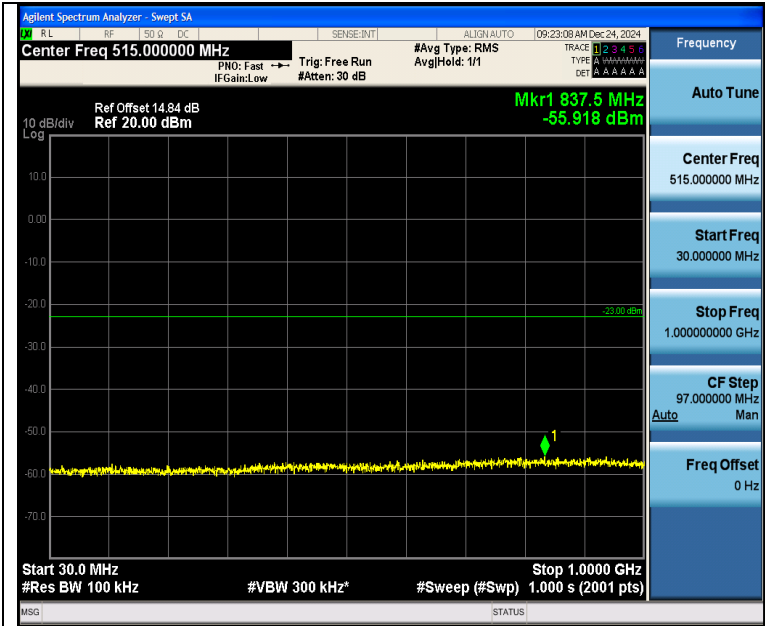
Band2_1.4MHz_QPSK_18900_6RB#0_30~1000_30~1000
