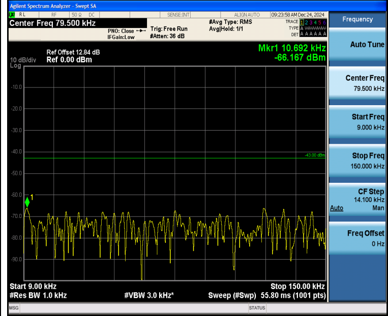
Band2_1.4MHz_16QAM_18900_6RB#0_0.009~0.15_0.009~0.15
