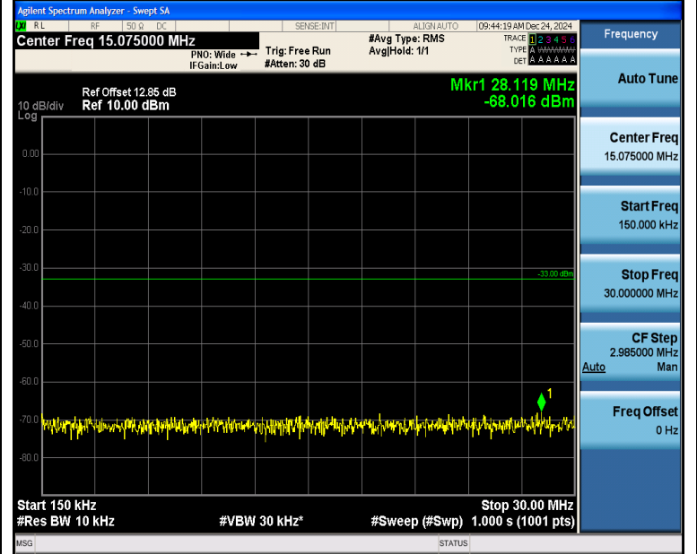
Band2_3MHz_QPSK_18900_1RB#14_0.15~30_0.15~30
