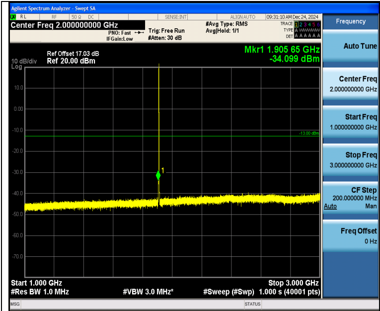
Band2_1.4MHz_16QAM_19193_6RB#0_1000~3000_1000~3000
