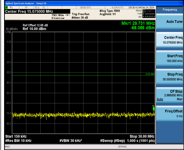
Band2_1.4MHz_16QAM_19193_6RB#0_0.15~30_0.15~30
