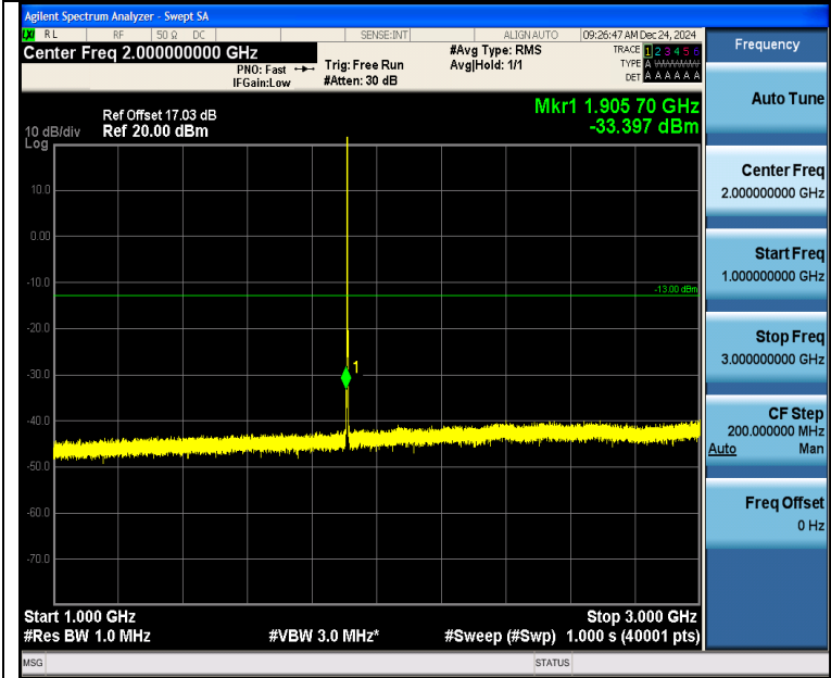
Band2_1.4MHz_16QAM_19193_1RB#0_1000~3000_1000~3000
