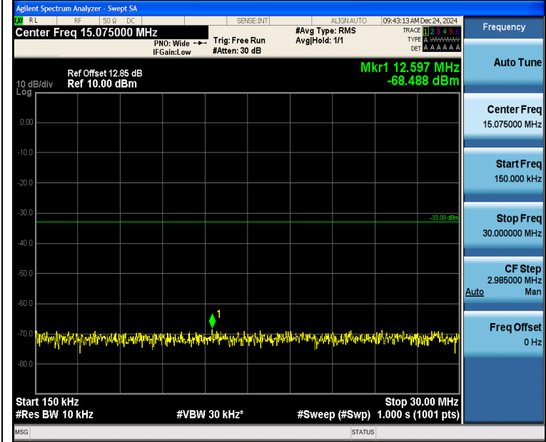
Band2_3MHz_16QAM_18900_1RB#0_0.15~30_0.15~30
