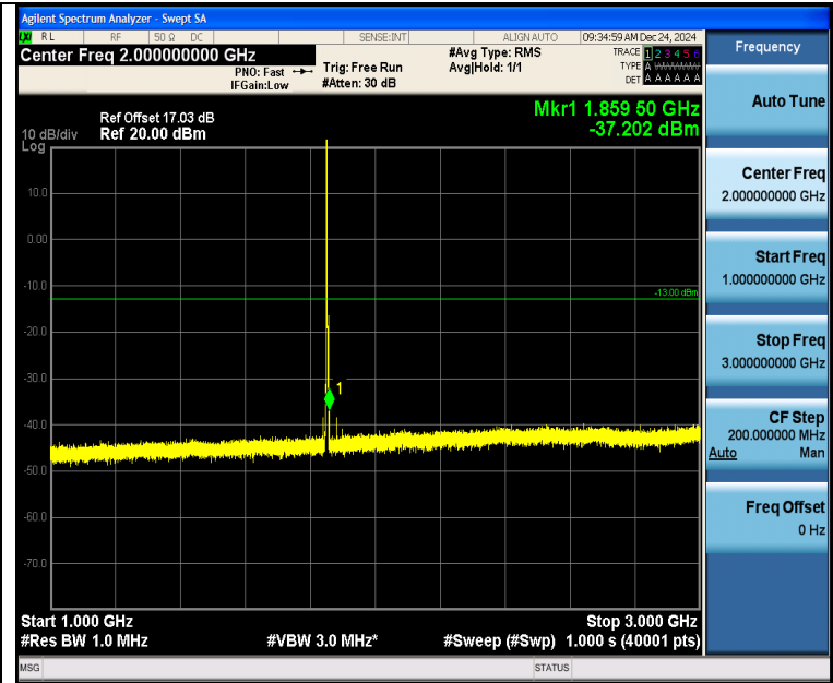
Band2_3MHz_QPSK_18615_1RB#0_1000~3000_1000~3000
