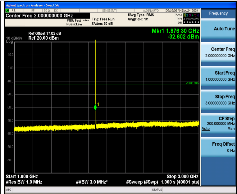
Band2_1.4MHz_QPSK_18900_1RB#0_1000~3000_1000~3000
