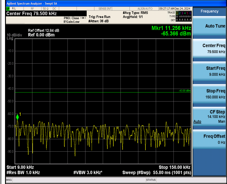
Band2_1.4MHz_QPSK_19193_1RB#5_0.009~0.15_0.009~0.15
