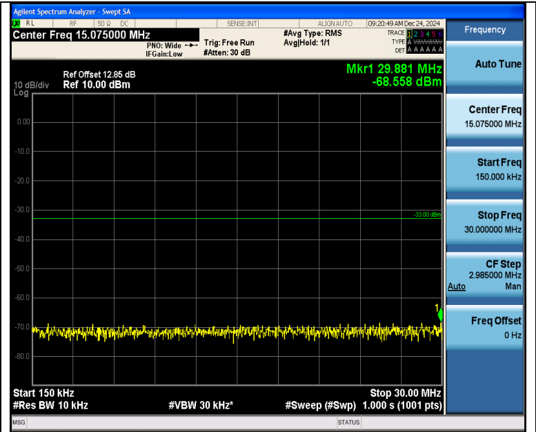
Band2_1.4MHz_QPSK_18900_1RB#5_0.15~30_0.15~30
