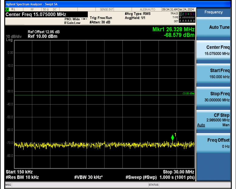
Band2_3MHz_QPSK_18615_1RB#0_0.15~30_0.15~30
