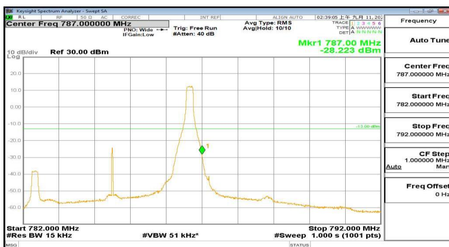
782MHz-792MHz_FreqHigh_BW(5MHz)_RB(1@24)_QPSK_Band13
