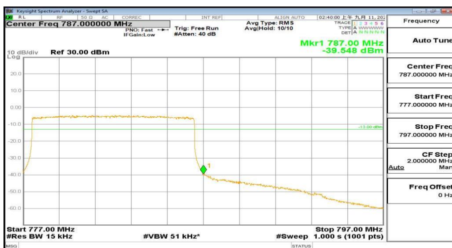
777MHz-797MHz_FreqHigh_BW(_10MHz)_RB(50@49)_QPSK_Band13
