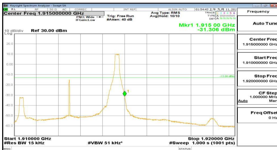
1910MHz-1920MHz_FreqHigh_BW(_5MHz)_RB(1@24)_QPSK_Band25
