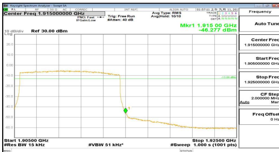
1905MHz-1925MHz_FreqHigh_BW(10MHz)_RB(50@49)_QPSK_Band25
