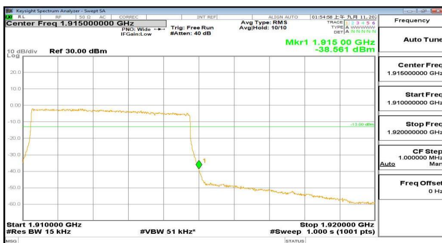
1910MHz-1920MHz_FreqHigh_BW(_5MHz)_RB(25@24)_QPSK_Band25
