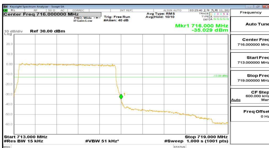
713MHz-719MHz_FreqHigh_BW(_3MHz)_RB(15@14)_QPSK_Band12
