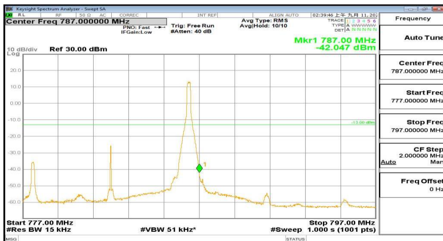
777MHz-797MHz_FreqHigh_BW(_10MHz)_RB(1@49)_QPSK_Band13
