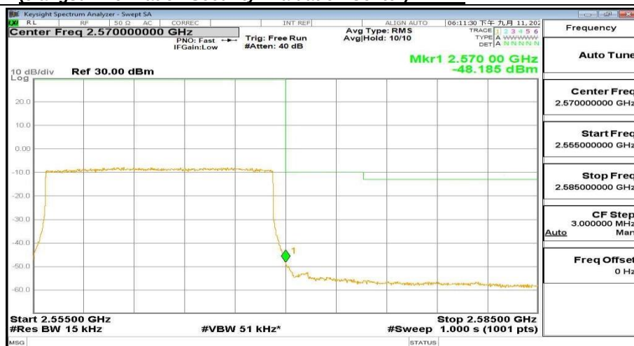
2555MHz-2585MHz_FreqHigh_BW(_15MHz)_RB(75@74)_QPSK_Band7
