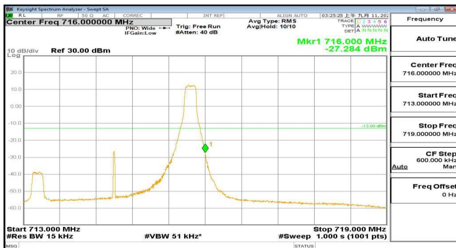
713MHz-719MHz_FreqHigh_BW(_3MHz)_RB(1@14)_QPSK_Band12
