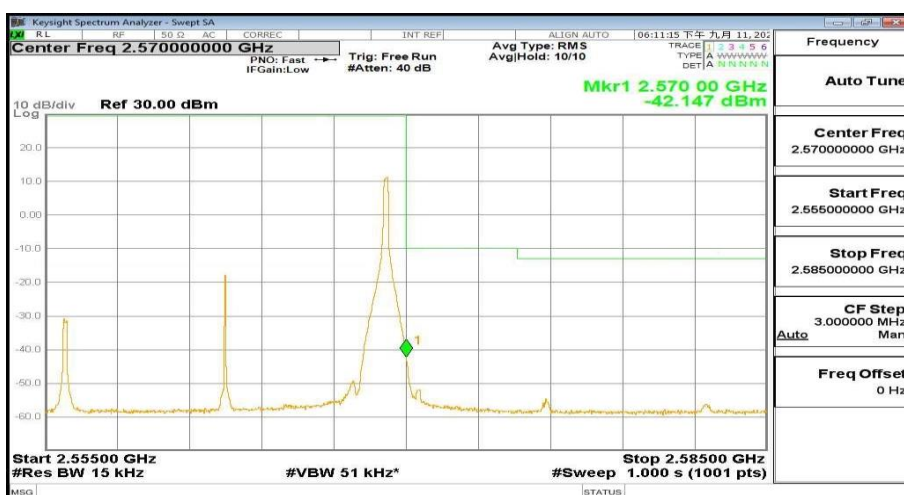
2555MHz-2585MHz_FreqHigh_BW(_15MHz)_RB(1@74)_QPSK_Band7
