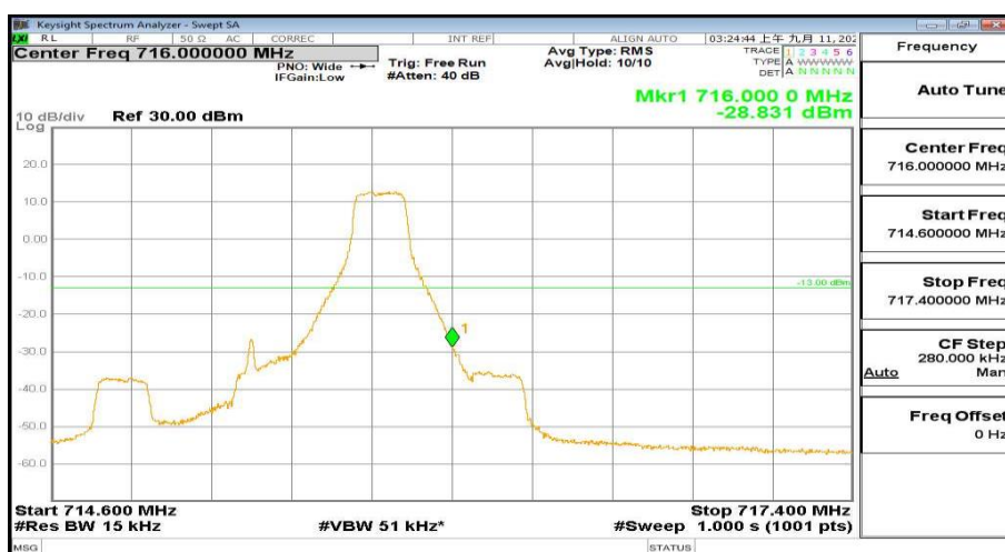
714.6MHz-717.4MHz_FreqHigh_BW(1D4MHz)_RB(1@5)_QPSK_Band12
