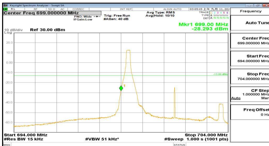
694MHz-704MHz_FreqLow_BW(5MHz)_RB(1@0)_QPSK_Band12
