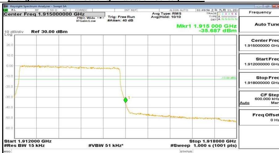
1912MHz-1918MHz_FreqHigh_BW(_3MHz)_RB(15@14)_QPSK_Band25
