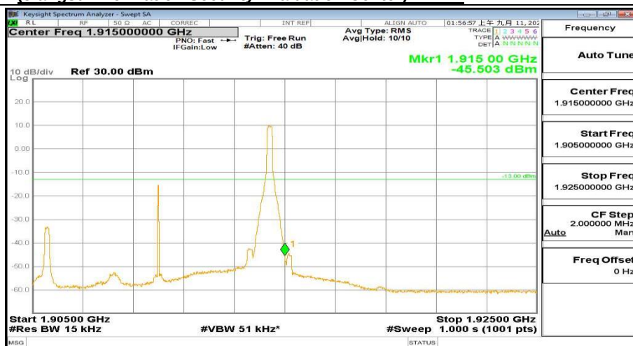
1905MHz-1925MHz_FreqHigh_BW(10MHz)_RB(1@49)_QPSK_Band25
