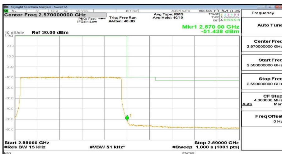
2550MHz-2590MHz_FreqHigh_BW(_20MHz)_RB(100@99)_QPSK_Band7
