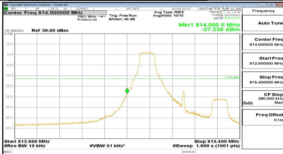
812.6MHz-815.4MHz_FreqLow_BW(1D4MHz)_RB(1@0)_QPSK_Band26
