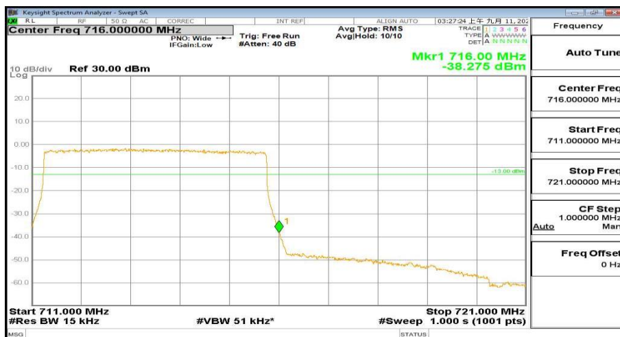
711MHz-721MHz_FreqHigh_BW(_5MHz)_RB(25@24)_QPSK_Band12
