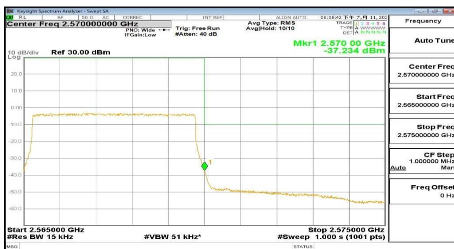
2565MHz-2575MHz_FreqHigh_BW(_5MHz)_RB(25@24)_QPSK_Band7
