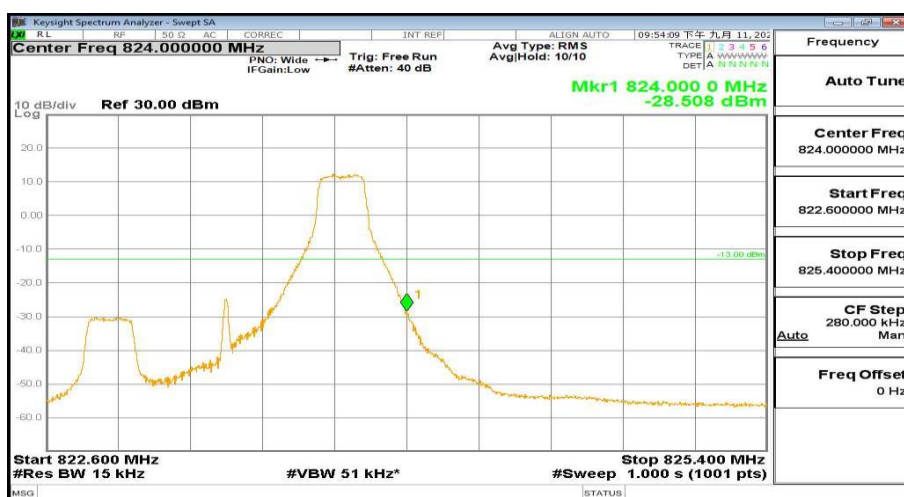
822.6MHz-825.4MHz_FreqHigh_BW(1D4MHz)_RB(1@5)_QPSK_Band26
