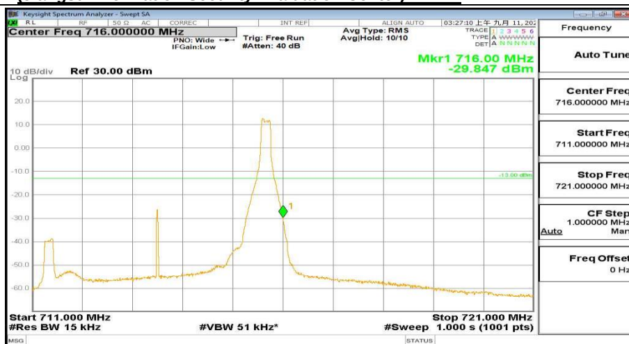
711MHz-721MHz_FreqHigh_BW(_5MHz)_RB(1@24)_QPSK_Band12
