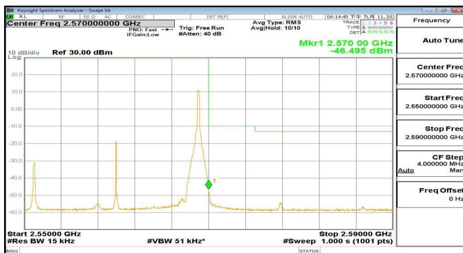
2550MHz-2590MHz_FreqHigh_BW(_20MHz)_RB(1@99)_QPSK_Band7
