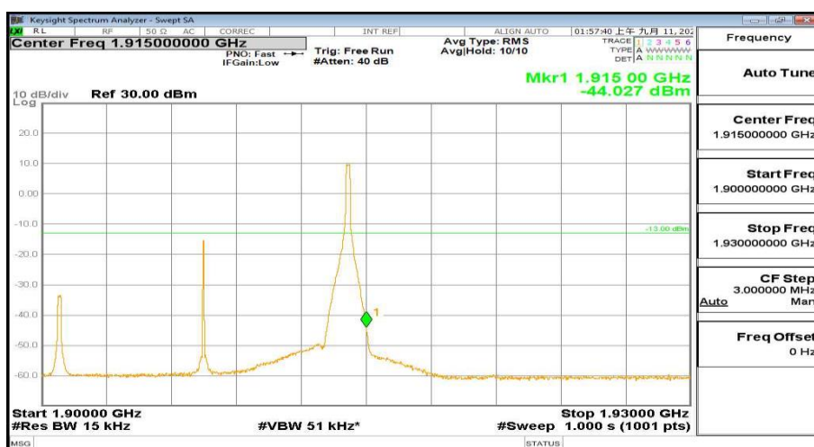
1900MHz-1930MHz_FreqHigh_BW(15MHz)_RB(1@74)_QPSK_Band25
