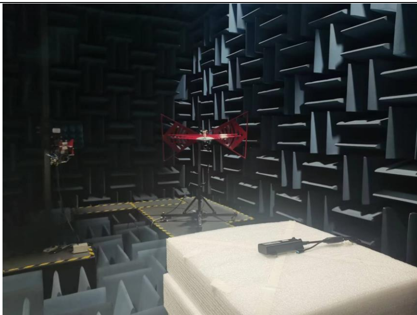
Radiated Spurious Emissions Test setup Internal Figure 1
