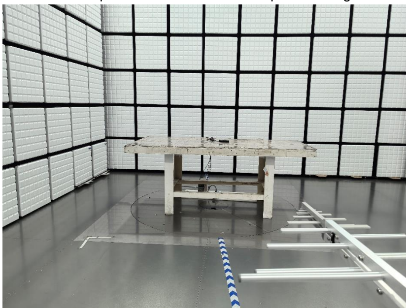
Radiated Spurious Emissions Test setup Internal Figure 2
