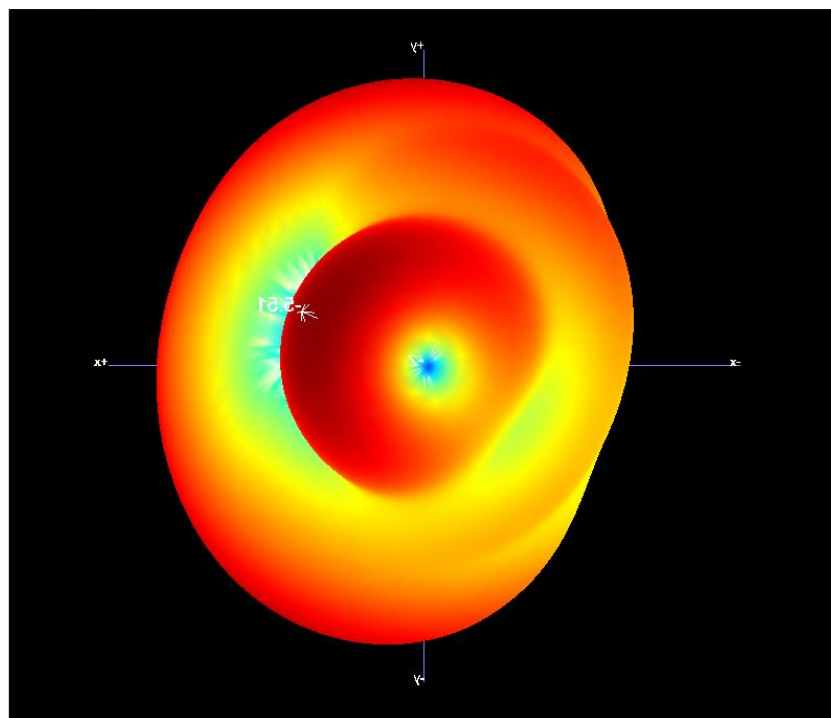
B1.2 3D Pattern for 2441MHz
