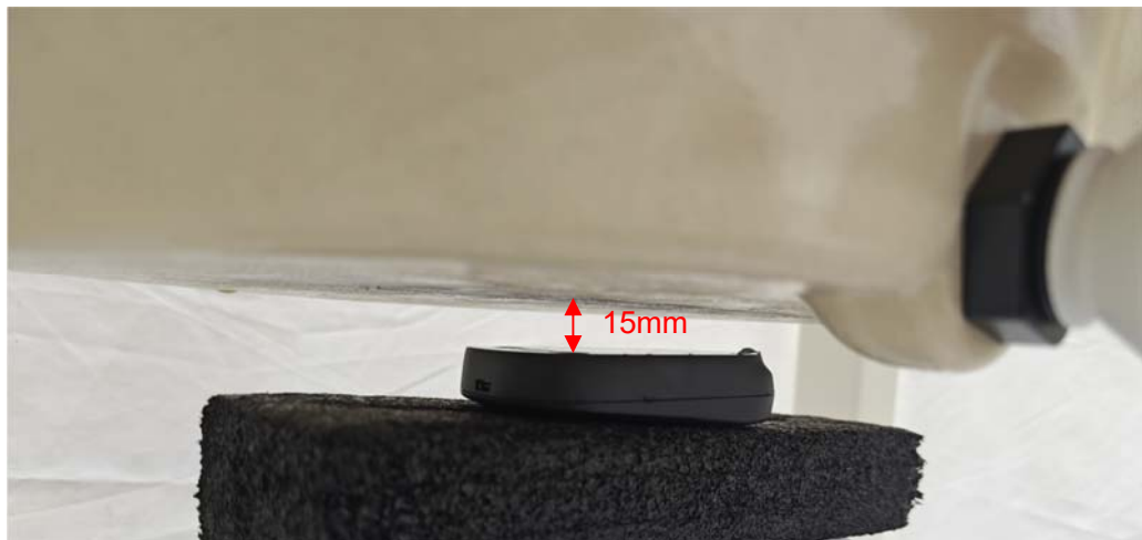
Picture 2: Front Side, the distance from handset to the bottom of the Phantom is 15mm
