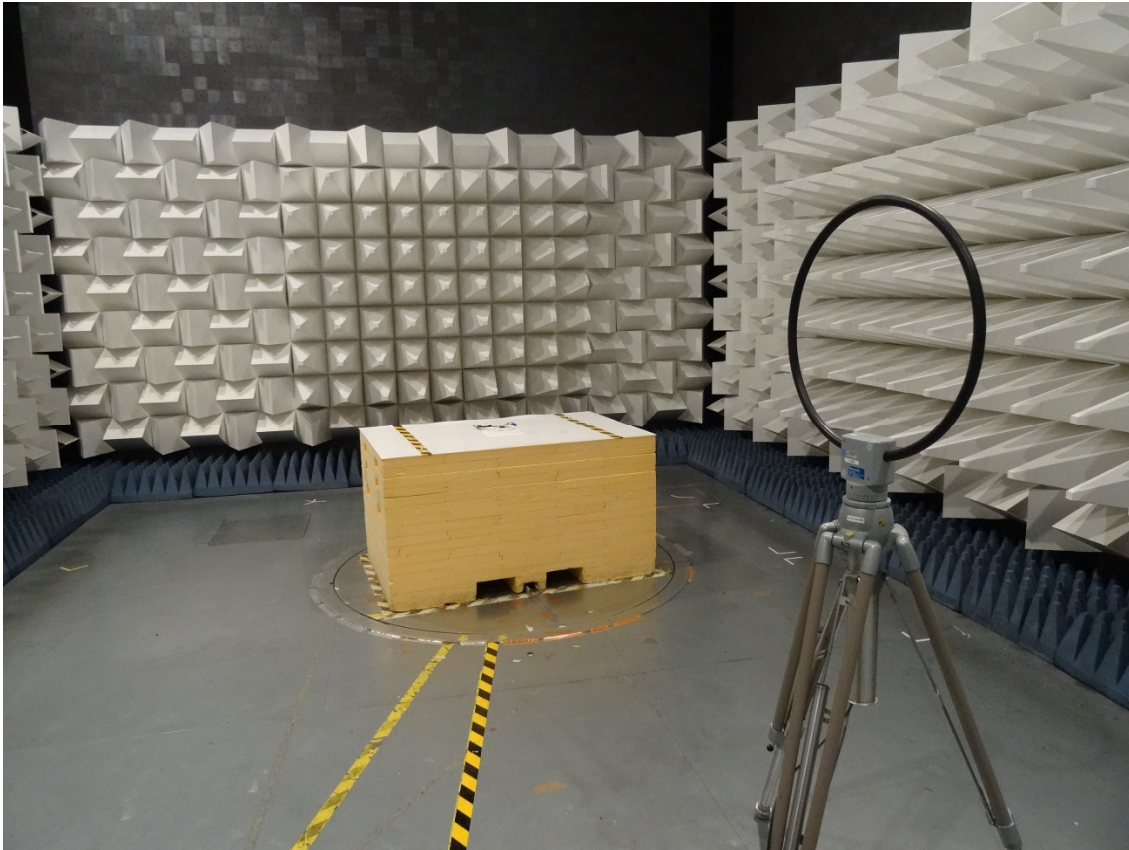
Radiated < 30MHz
