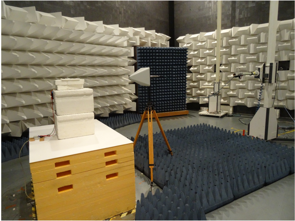
Radiated emission (pre-scan) 10GHz - 18 GHz
