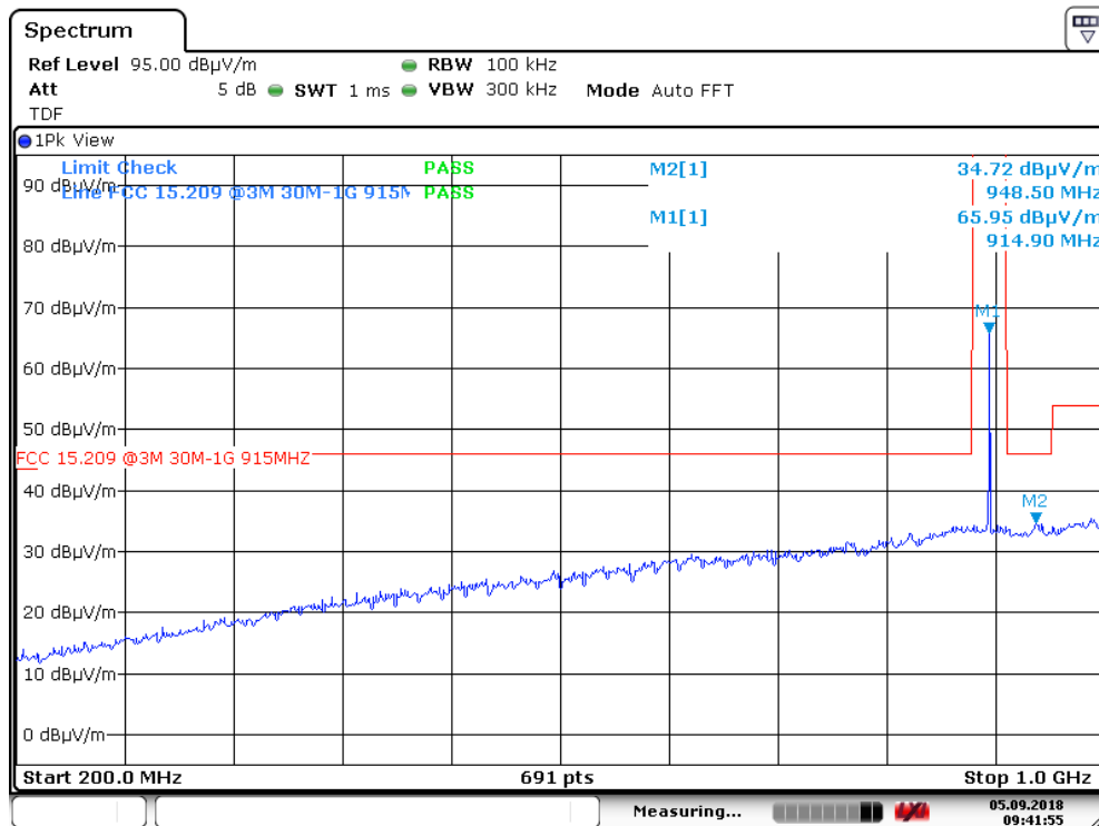
Radiated Emissions, 200 – 1000 MHz, HP, @3m, PK scan ch50 (Air modem)
