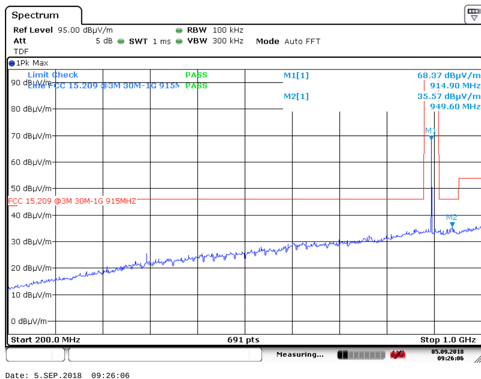
Radiated Emissions, 200 – 1000 MHz, VP, @3m, PK scan ch50 (Air modem)
