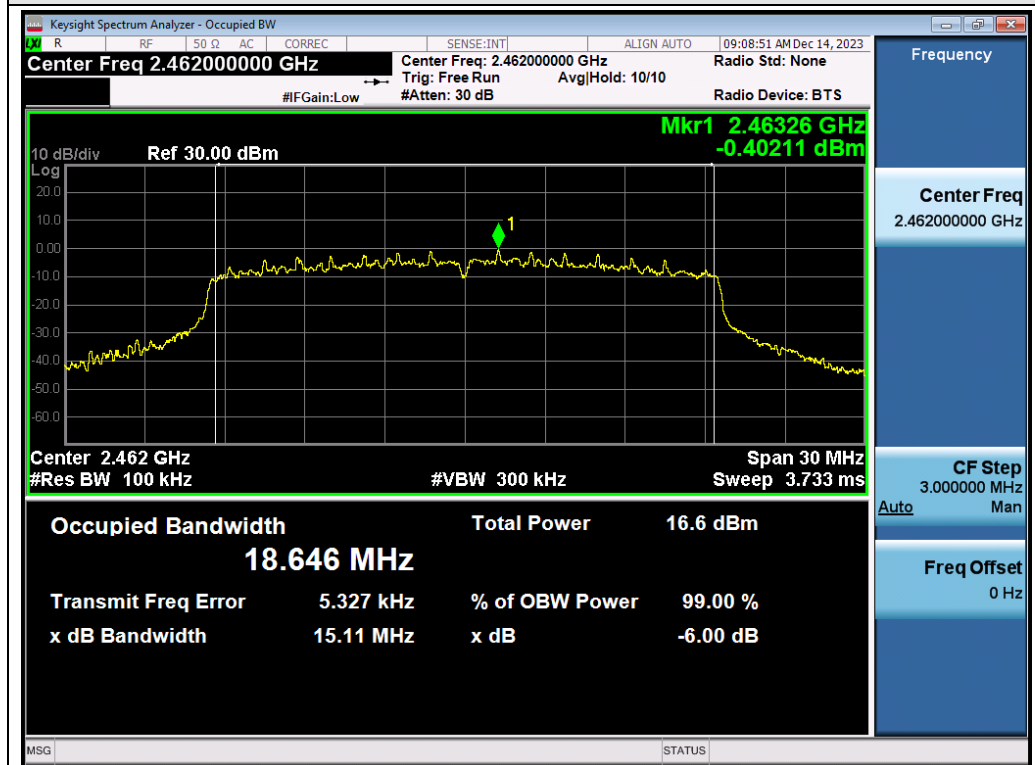
Test_Graph_802.11ax20_ANT1_2462_MCS0_DTSBW
