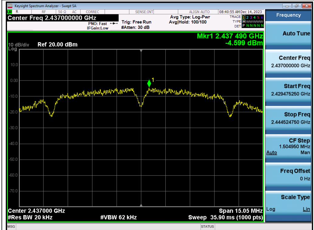
Test_Graph_802.11b_ANT1_2437_1Mbps_PSD
