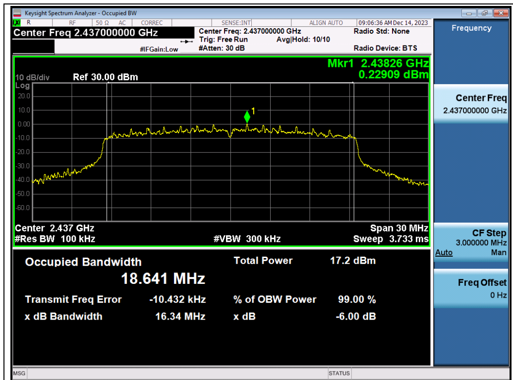
Test_Graph_802.11ax20_ANT1_2437_MCS0_DTSBW
