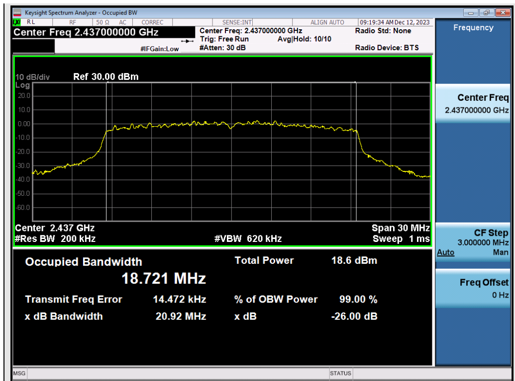
Test_Graph_802.11ax20_ANT1_2437_MCS0_OBW
