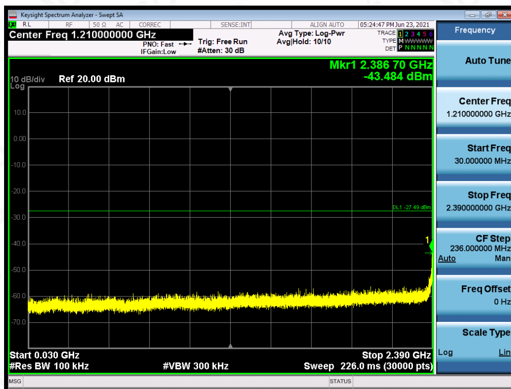
Test_Graph_802.11n40_ANT1_2422_MCS0_Lower Band Emissions
