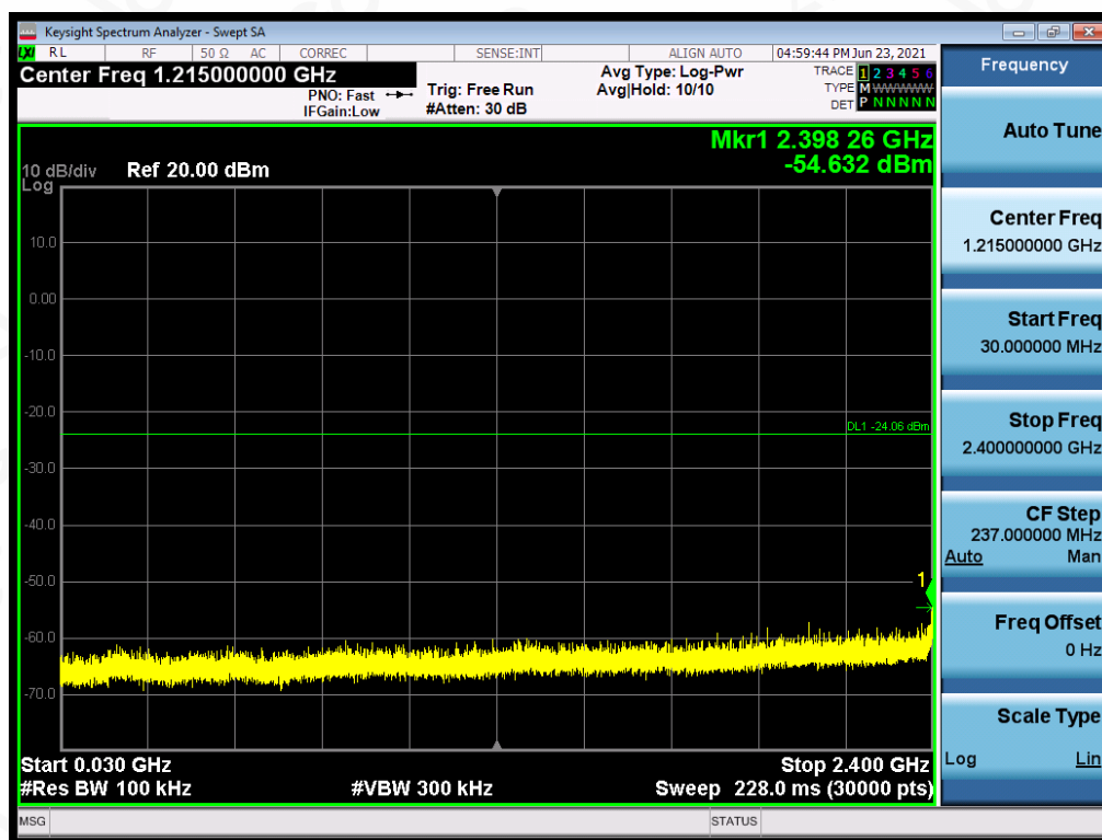
Test_Graph_802.11g_ANT1_2437_6Mbps_Lower Band Emissions
