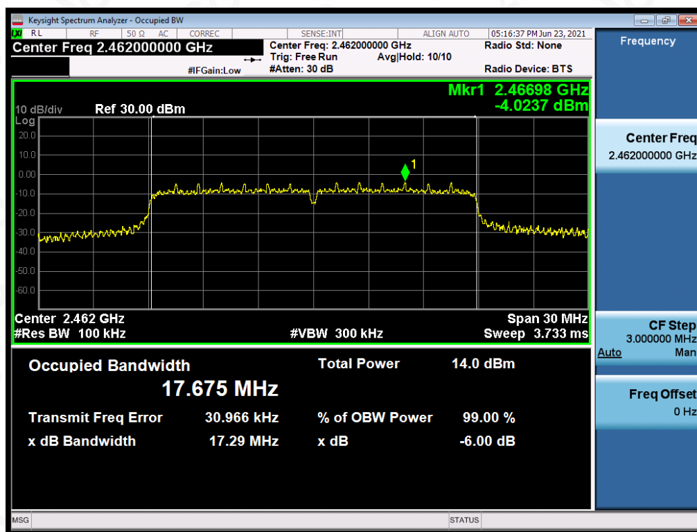
Test_Graph_802.11n20_ANT1_2462_MCS0_DTSBW
