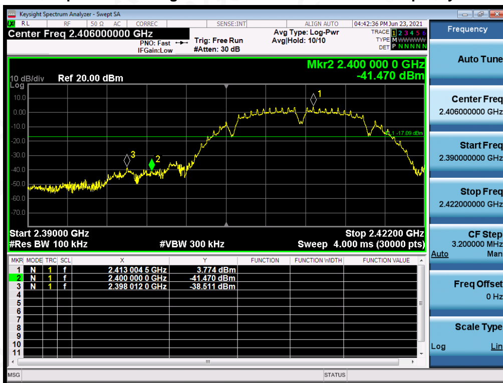
Test_Graph_802.11b_ANT1_2412_1Mbps_Lower Band Edge Emissions
