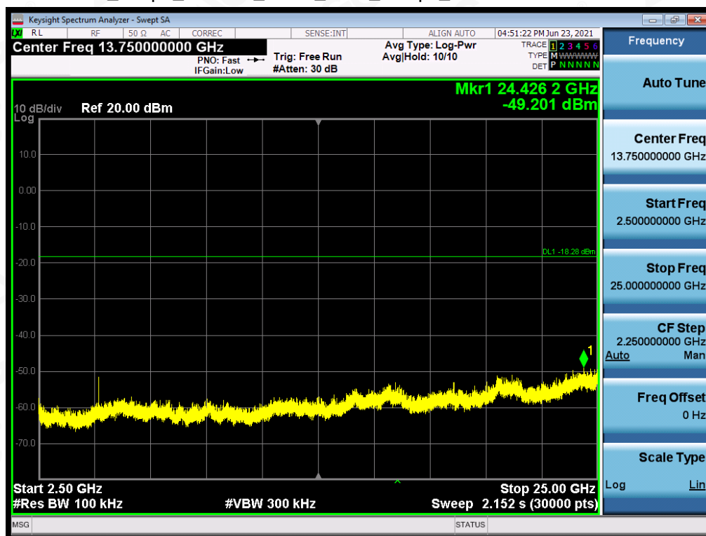
Test_Graph_802.11b_ANT1_2462_1Mbps_Higher Band Emissions
