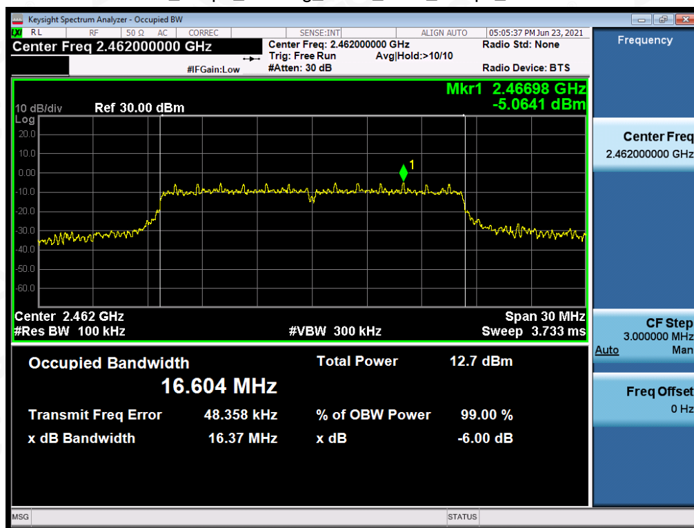
Test_Graph_802.11g_ANT1_2462_6Mbps_DTSBW
