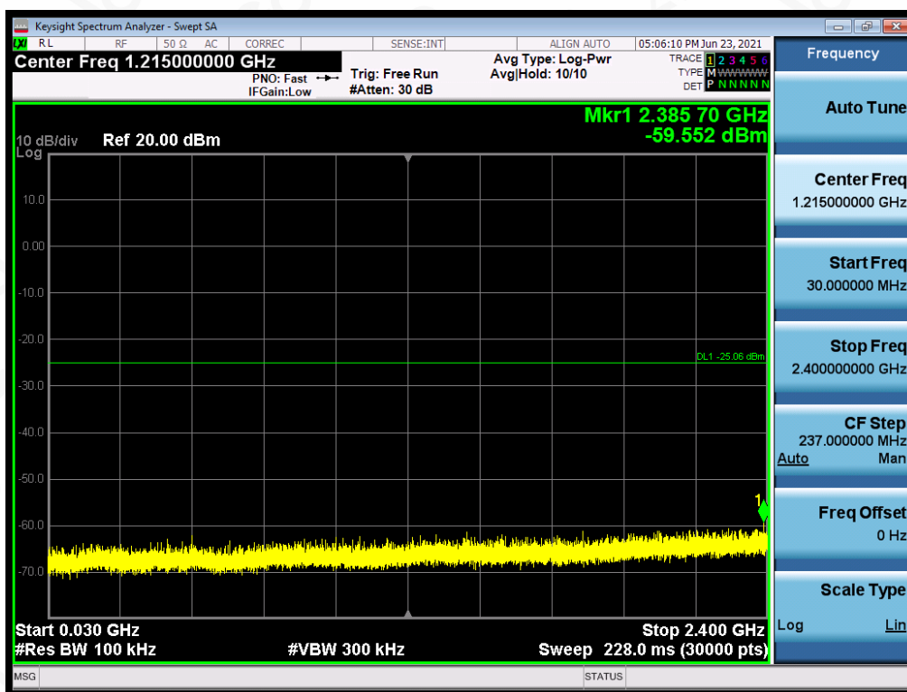
Test_Graph_802.11g_ANT1_2462_6Mbps_Lower Band Emissions
