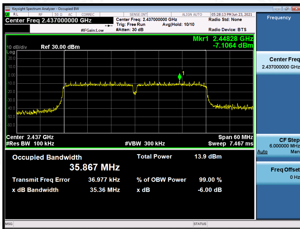
Test_Graph_802.11n40_ANT1_2437_MCS0_DTSBW
