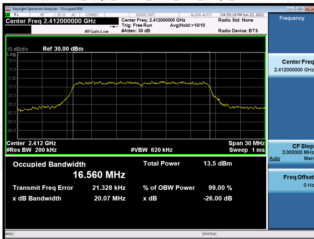
Test_Graph_802.11g_ANT1_2412_6Mbps_OBW
