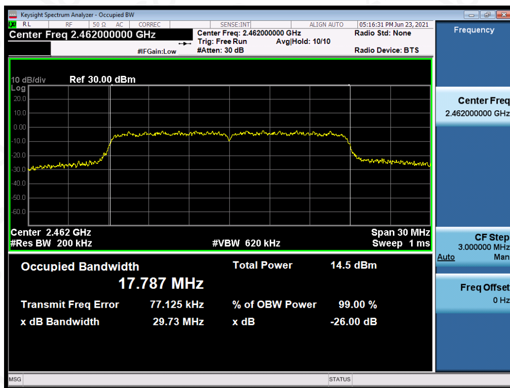
Test_Graph_802.11n20_ANT1_2462_MCS0_OBW
