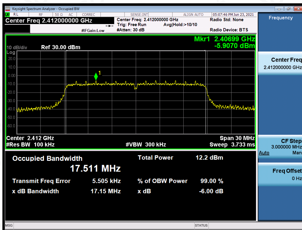
Test_Graph_802.11n20_ANT1_2412_MCS0_DTSBW
