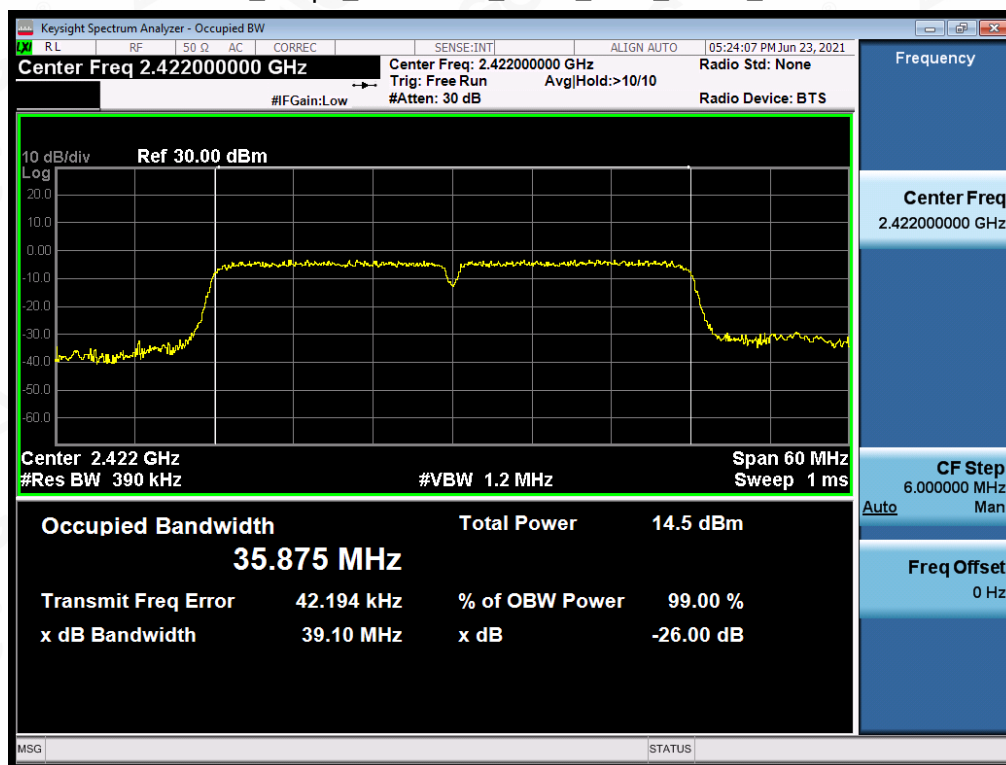
Test_Graph_802.11n40_ANT1_2422_MCS0_OBW
