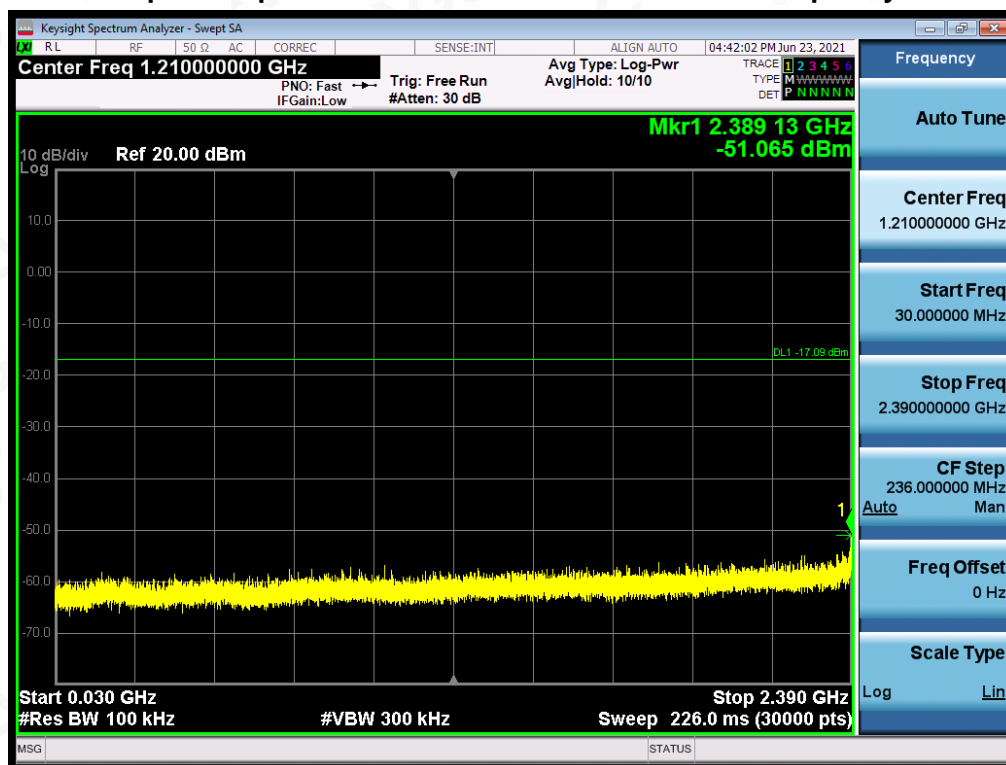
Test_Graph_802.11b_ANT1_2412_1Mbps_Lower Band Emissions
