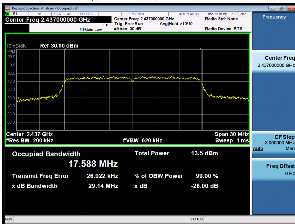
Test_Graph_802.11n20_ANT1_2437_MCS0_OBW
