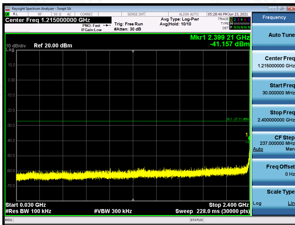
Test_Graph_802.11n40_ANT1_2437_MCS0_Lower Band Emissions
