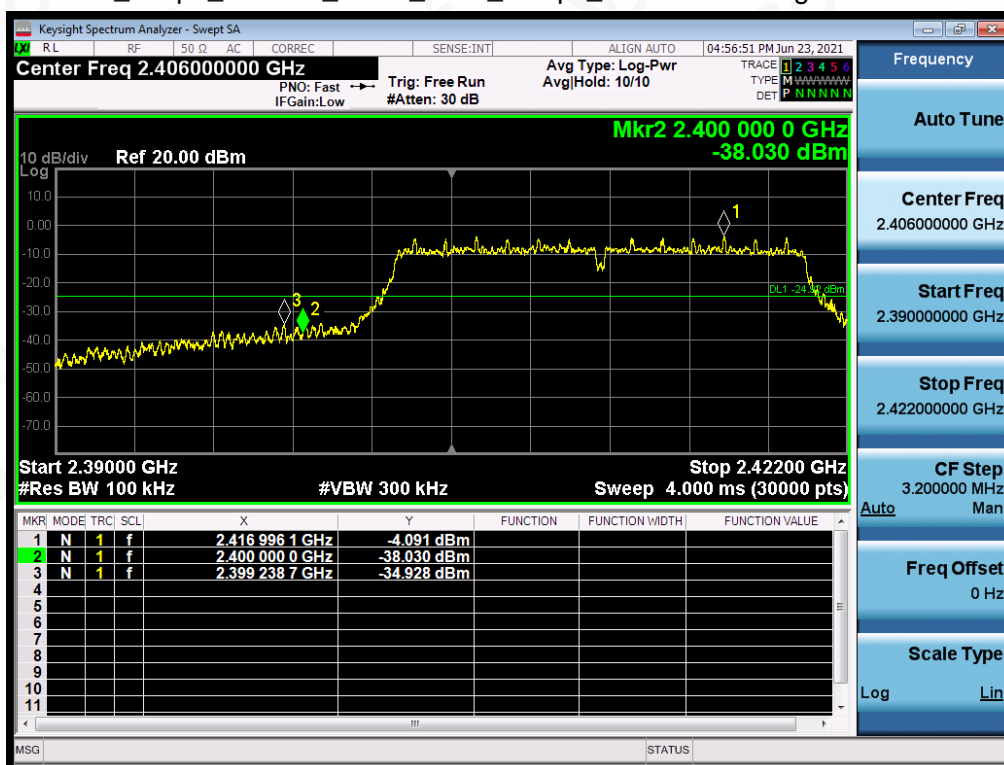
Test_Graph_802.11g_ANT1_2412_6Mbps_Lower Band Edge Emissions
