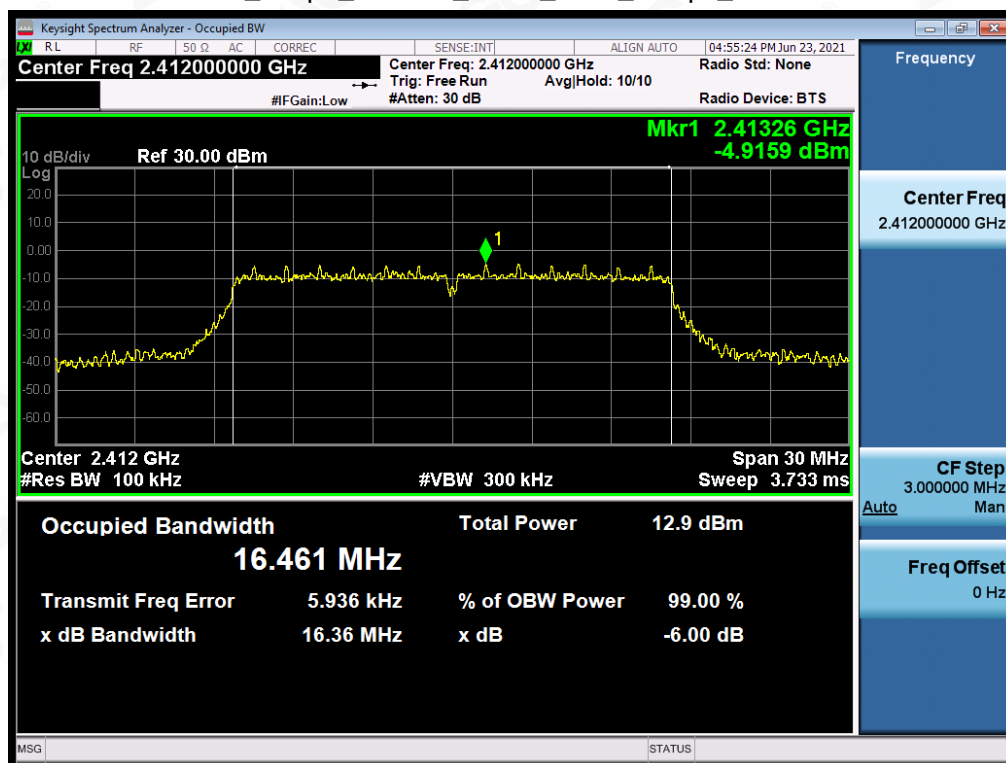
Test_Graph_802.11g_ANT1_2412_6Mbps_DTSBW
