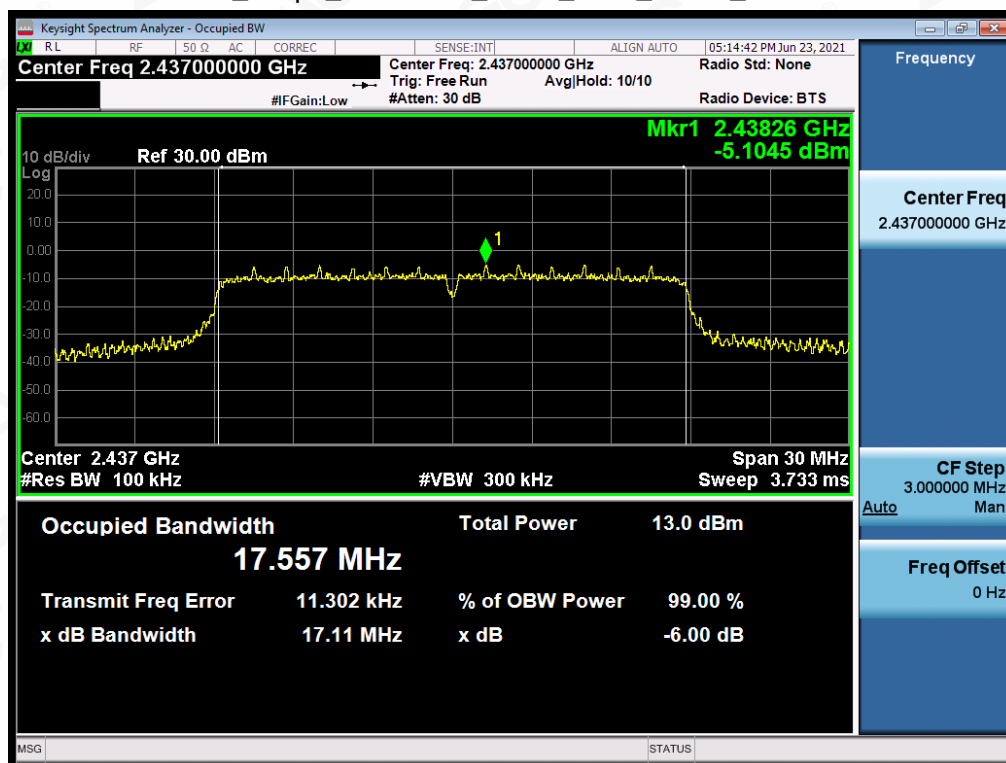
Test_Graph_802.11n20_ANT1_2437_MCS0_DTSBW
