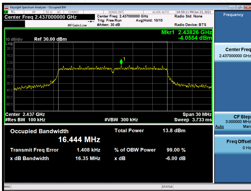
Test_Graph_802.11g_ANT1_2437_6Mbps_DTSBW
