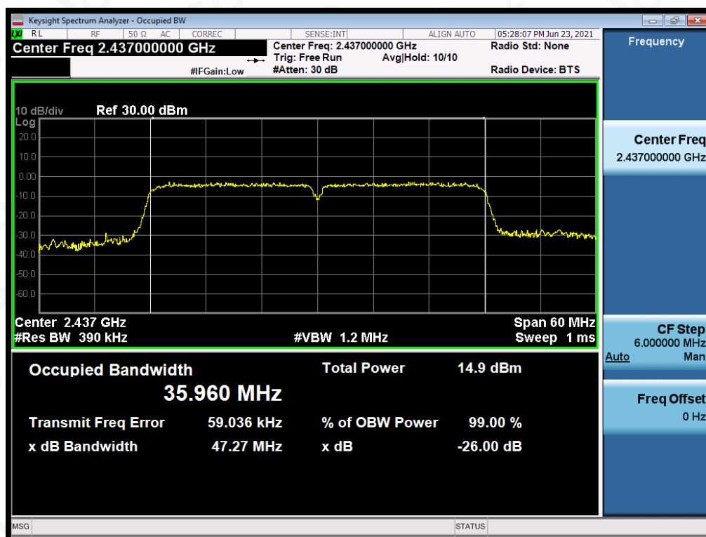
Test_Graph_802.11n40_ANT1_2437_MCS0_OBW
