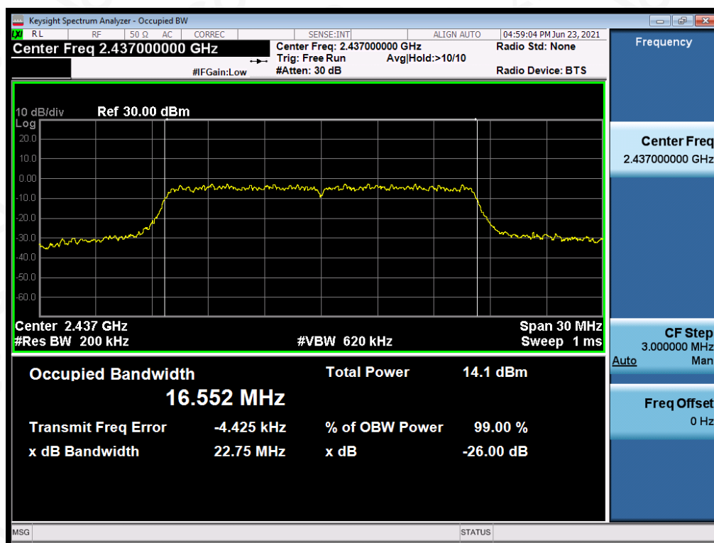
Test_Graph_802.11g_ANT1_2437_6Mbps_OBW
