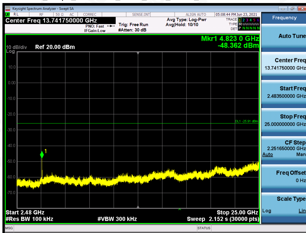
Test_Graph_802.11n20_ANT1_2412_MCS0_Higher Band Emissions
