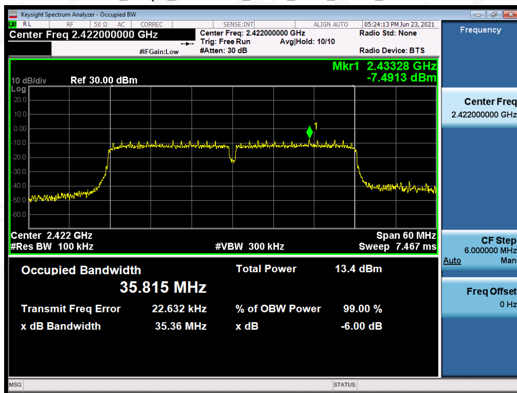
Test_Graph_802.11n40_ANT1_2422_MCS0_DTSBW
