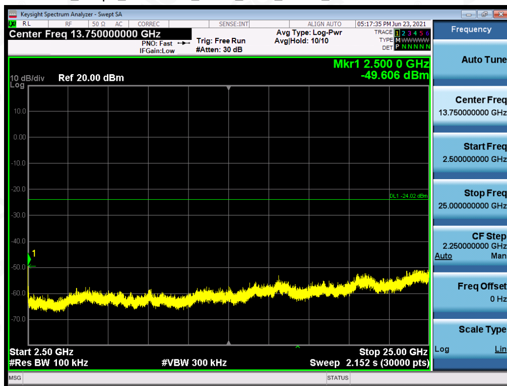
Test_Graph_802.11n20_ANT1_2462_MCS0_Higher Band Emissions
