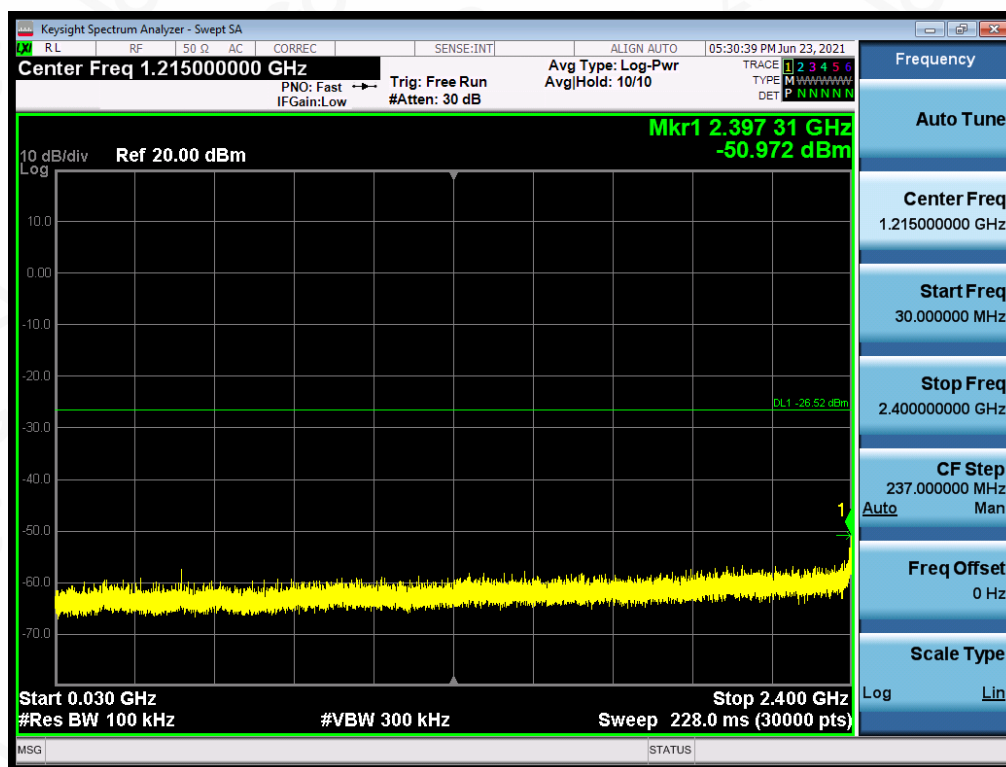
Test_Graph_802.11n40_ANT1_2452_MCS0_Lower Band Emissions
