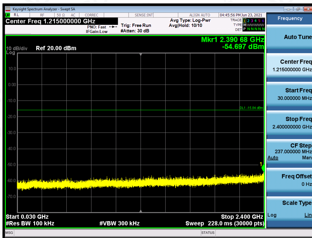
Test_Graph_802.11b_ANT1_2437_1Mbps_Lower Band Emissions
