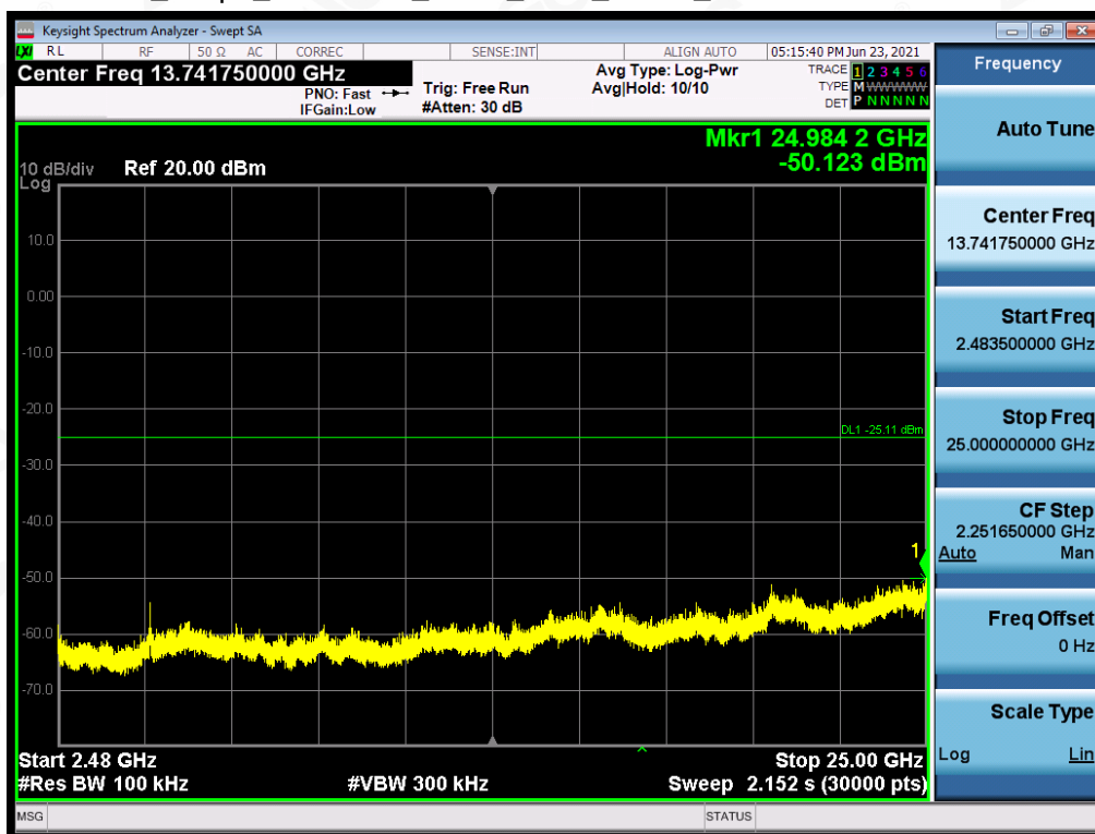
Test_Graph_802.11n20_ANT1_2437_MCS0_Higher Band Emissions
