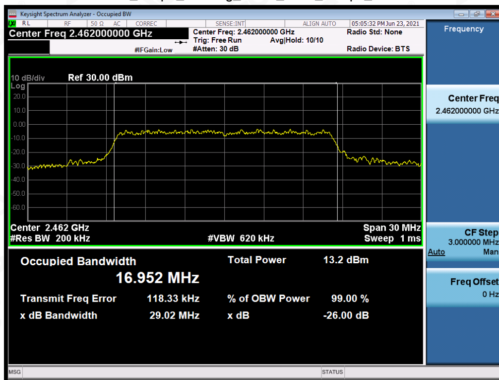
Test_Graph_802.11g_ANT1_2462_6Mbps_OBW
