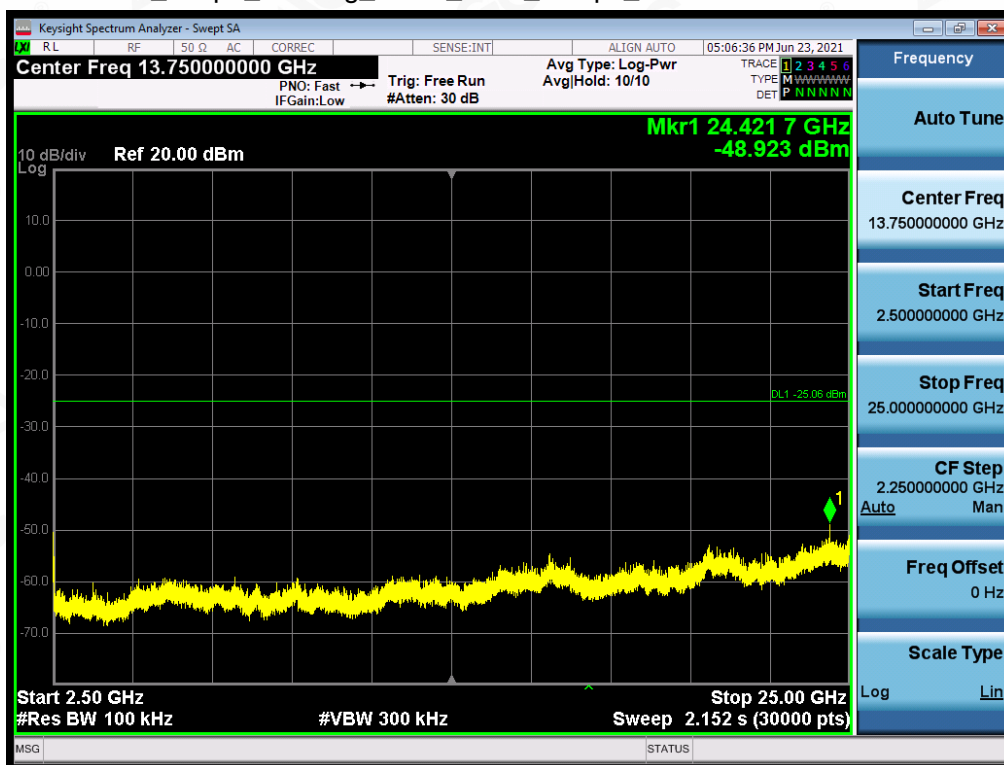
Test_Graph_802.11g_ANT1_2462_6Mbps_Higher Band Emissions
