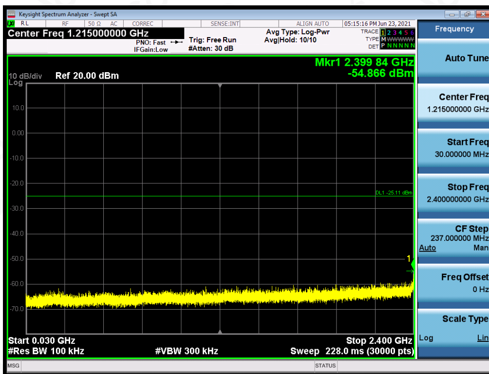
Test_Graph_802.11n20_ANT1_2437_MCS0_Lower Band Emissions
