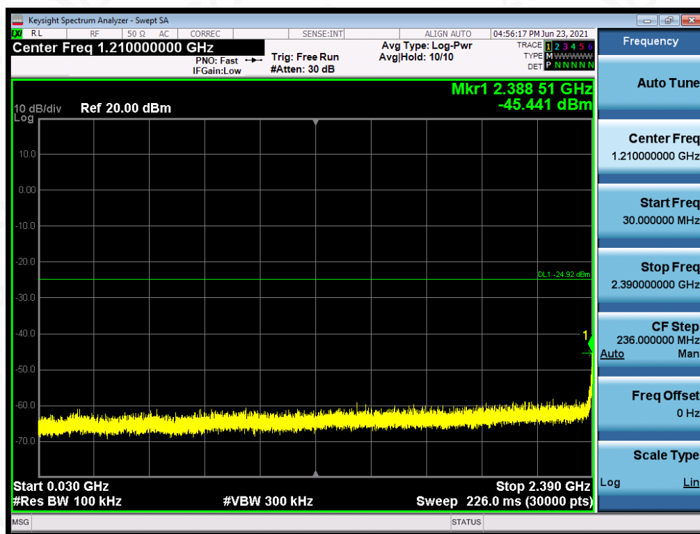
Test_Graph_802.11g_ANT1_2412_6Mbps_Lower Band Emissions
