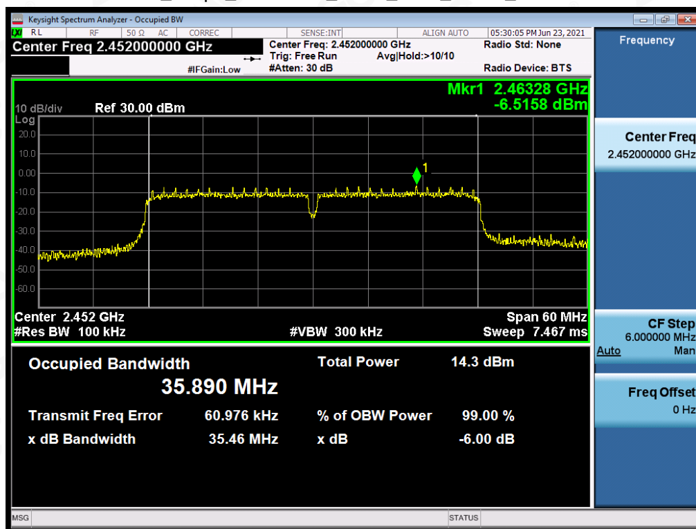
Test_Graph_802.11n40_ANT1_2452_MCS0_DTSBW
