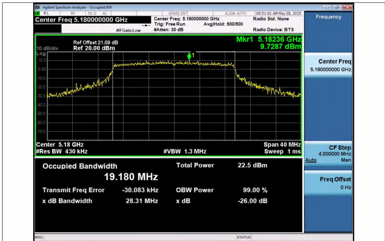
11AX20SISO-Ant1-5180
