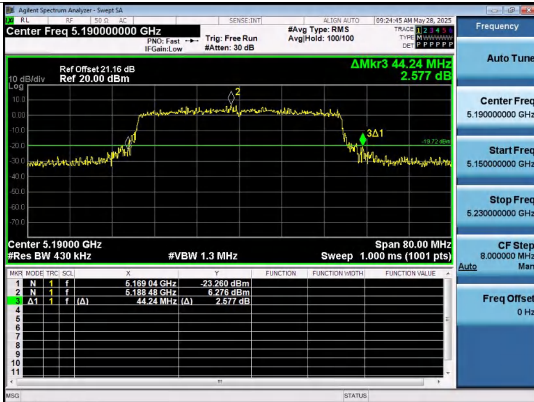
11AX40SISO-Ant1-5190
