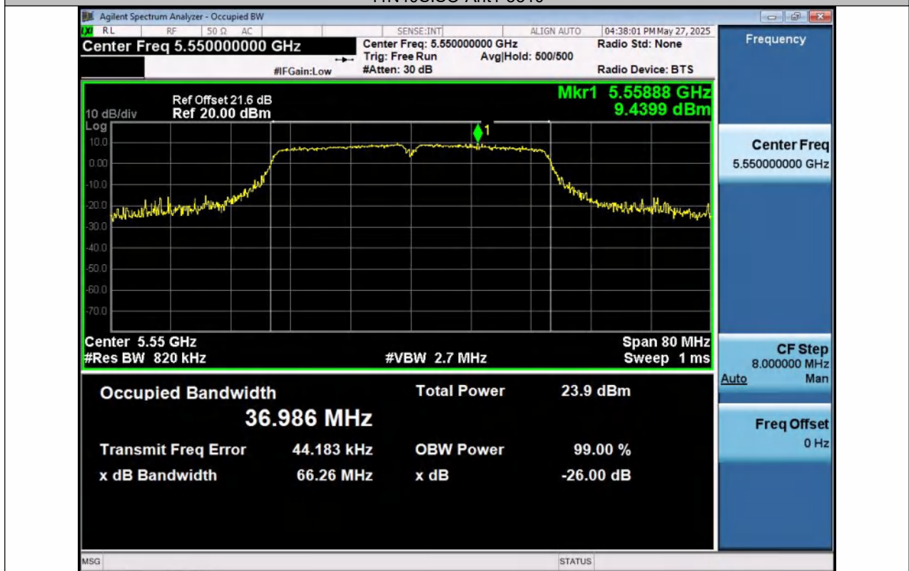
11N40SISO-Ant1-5550
