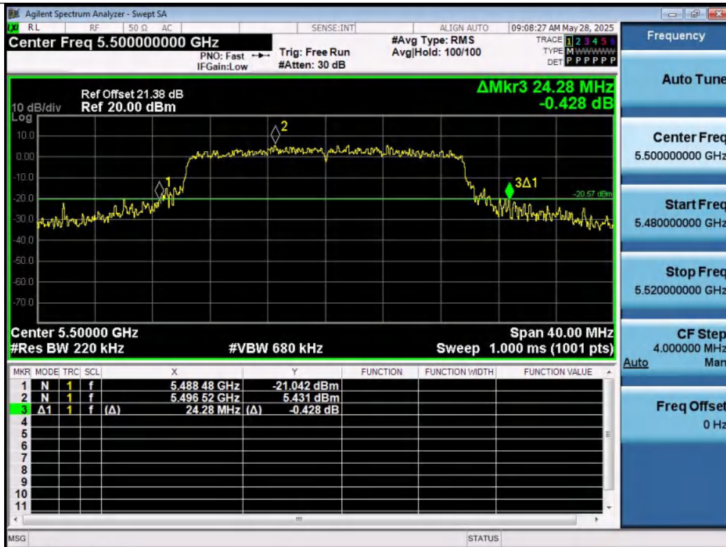
11AX20SISO-Ant1-5500
