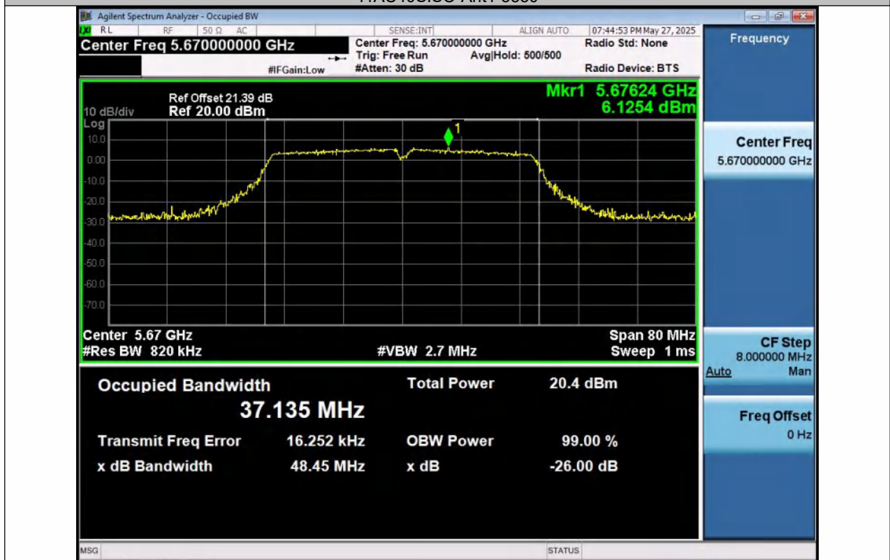
11AC40SISO-Ant1-5670
