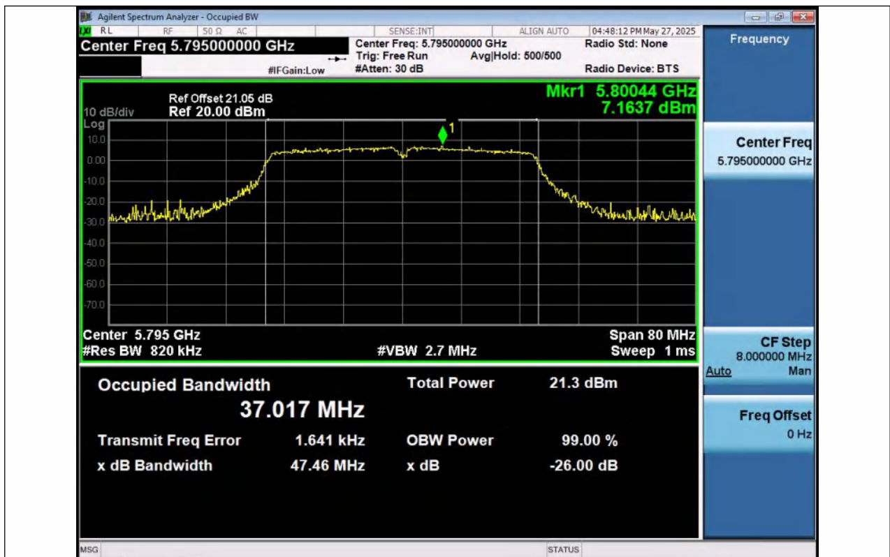
11N40SISO-Ant1-5795
