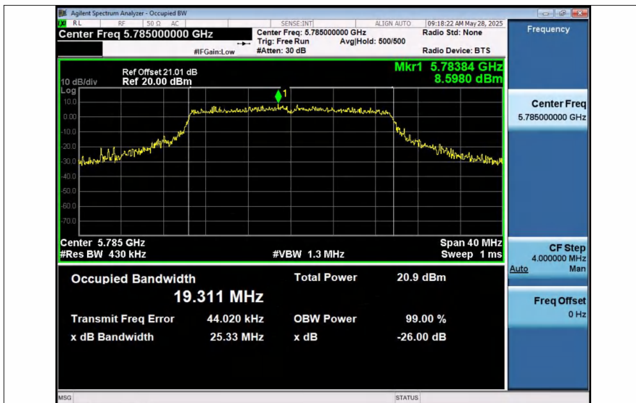
11AX20SISO-Ant1-5785
