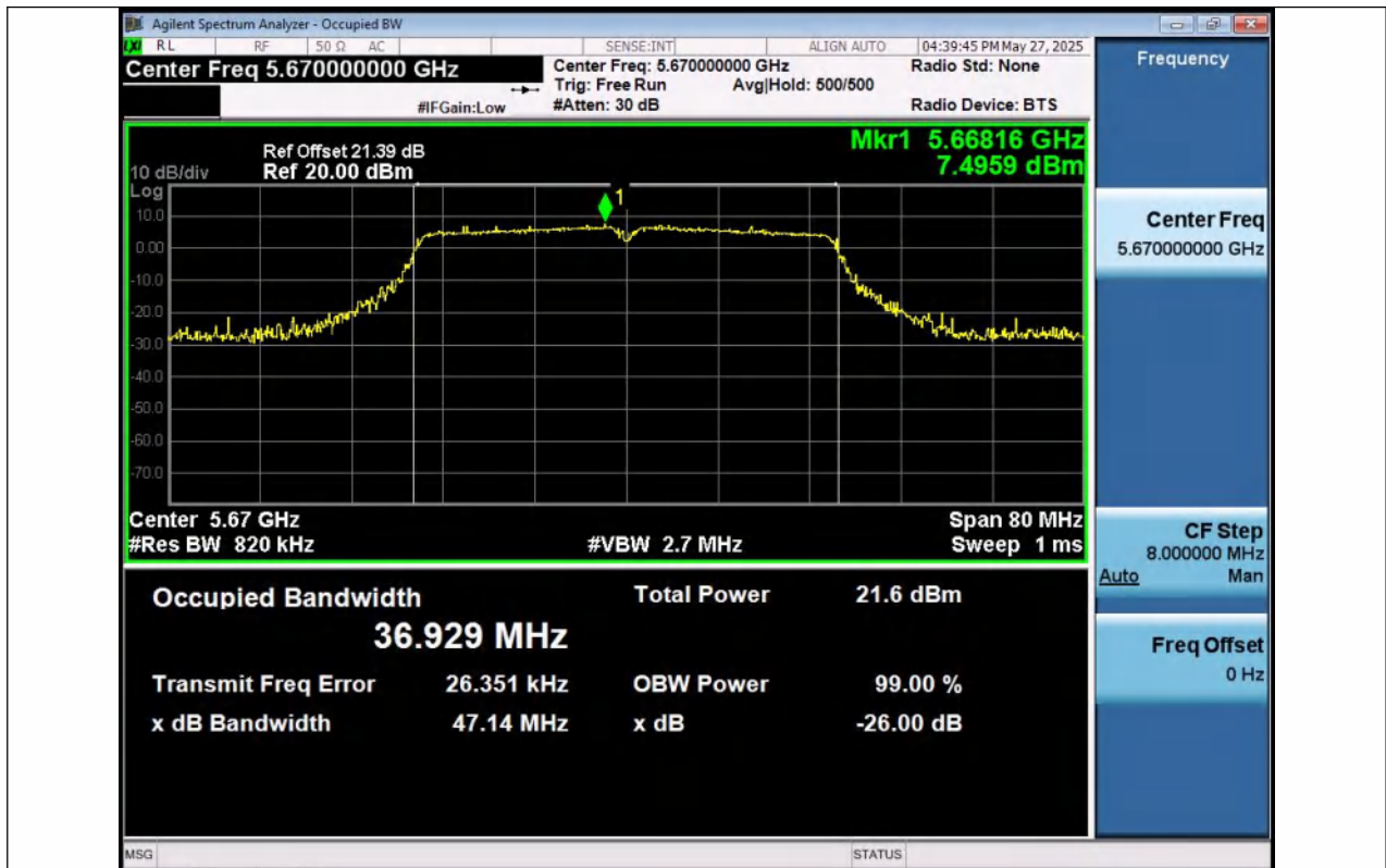
11N40SISO-Ant1-5670
