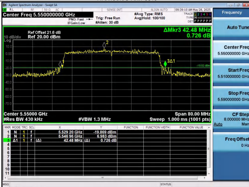
11AX40SISO-Ant1-5550
