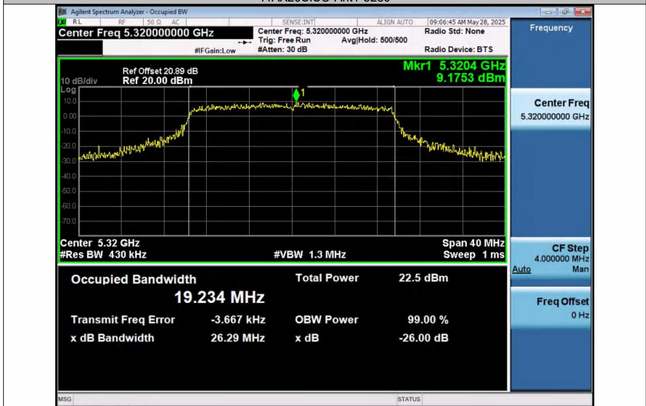
11AX20SISO-Ant1-5320
