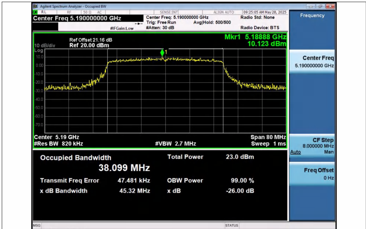
11AX40SISO-Ant1-5190
