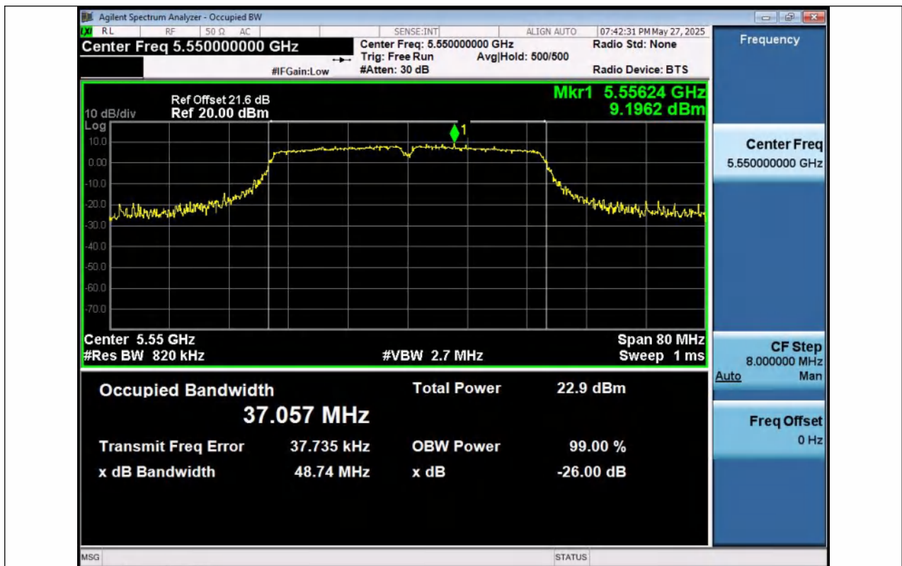
11AC40SISO-Ant1-5550
