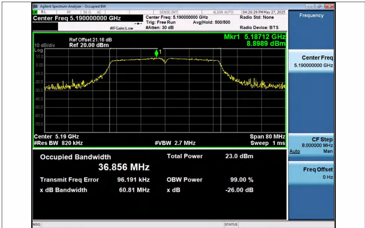
11N40SISO-Ant1-5190
