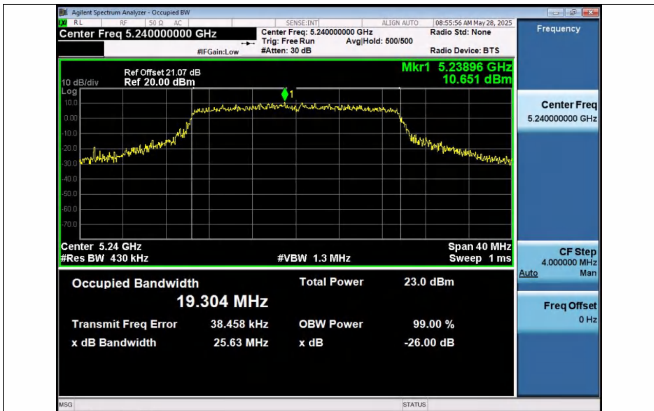
11AX20SISO-Ant1-5240
