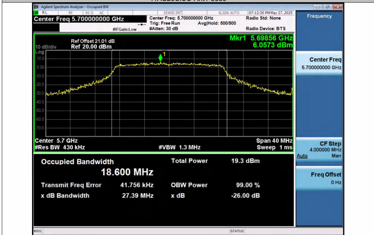
11AC20SISO-Ant1-5700
