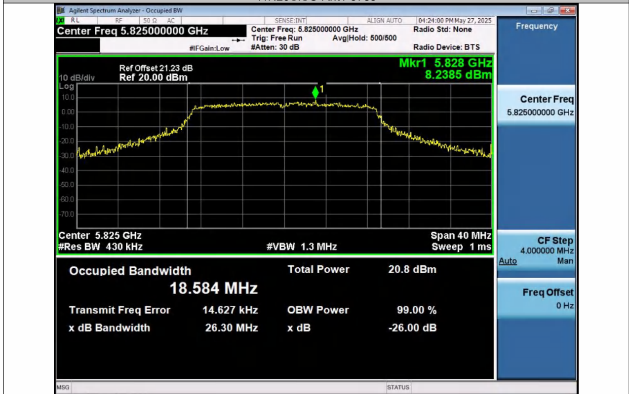
11N20SISO-Ant1-5825
