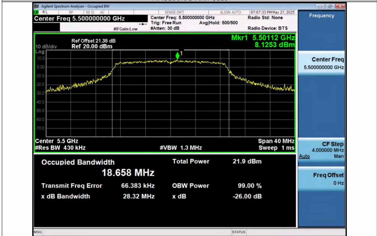
11AC20SISO-Ant1-5500
