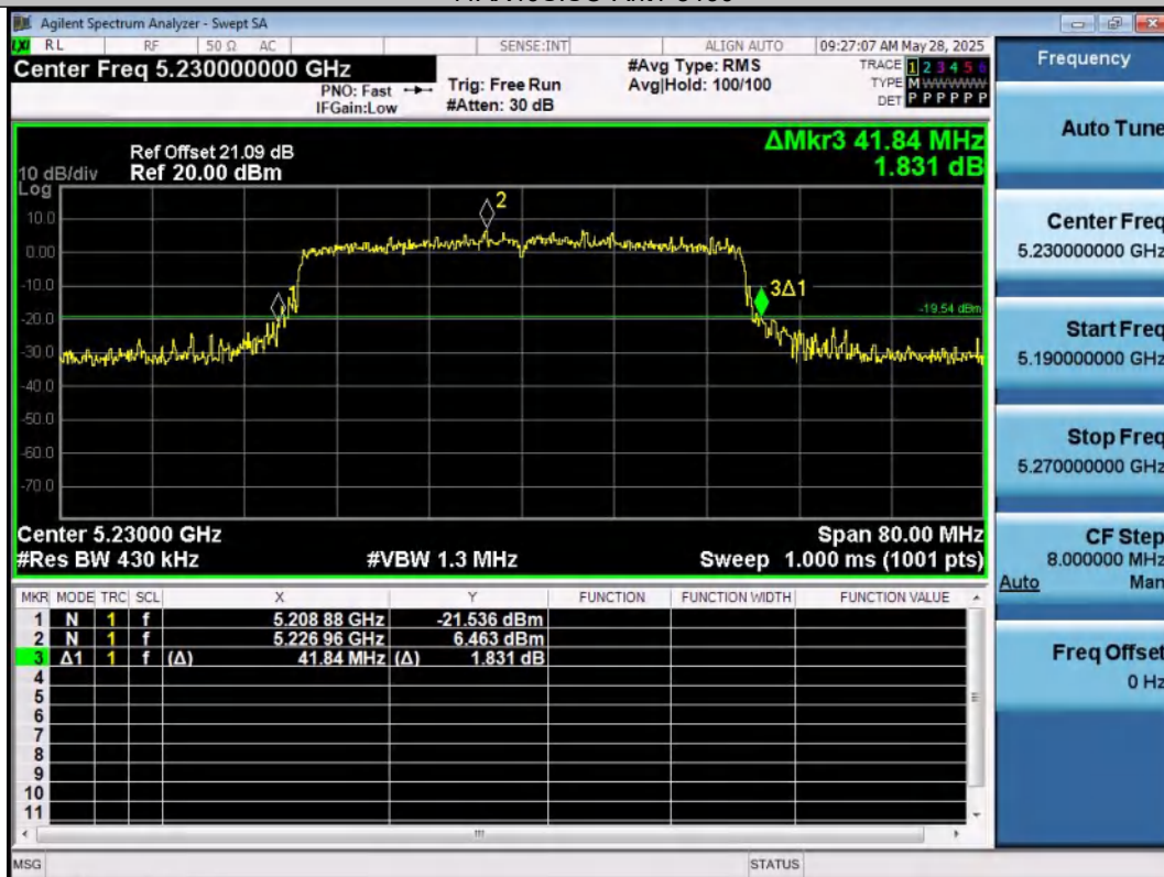
11AX40SISO-Ant1-5230
