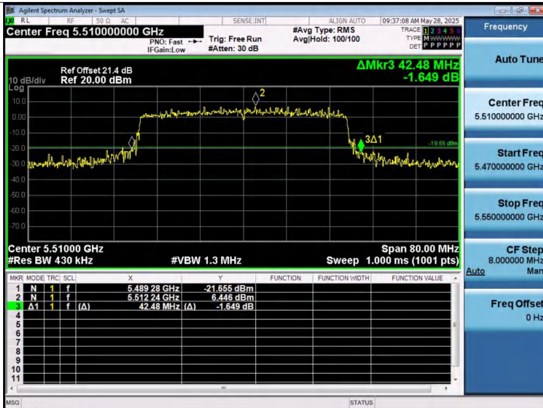
11AX40SISO-Ant1-5510
