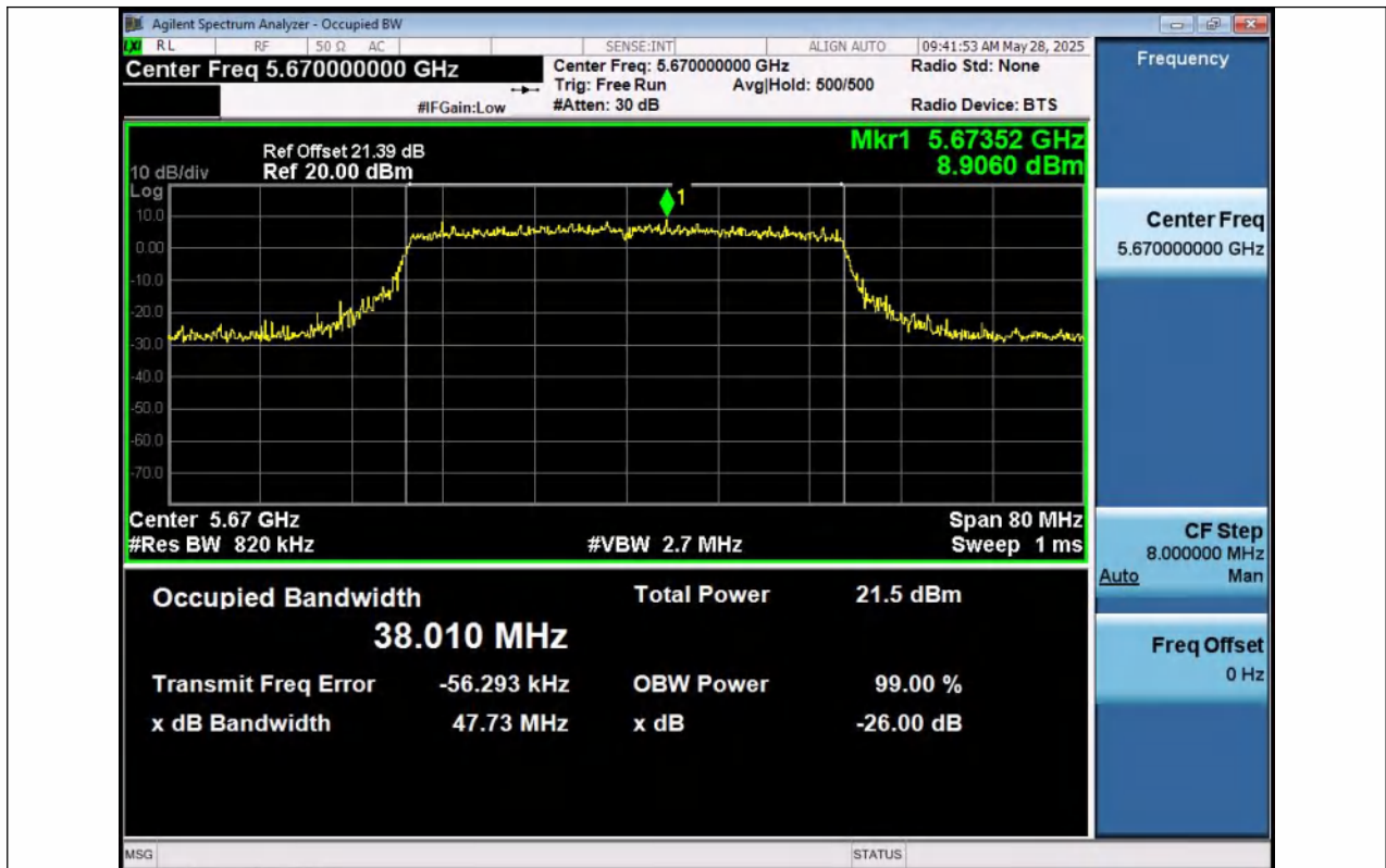
11AX40SISO-Ant1-5670
