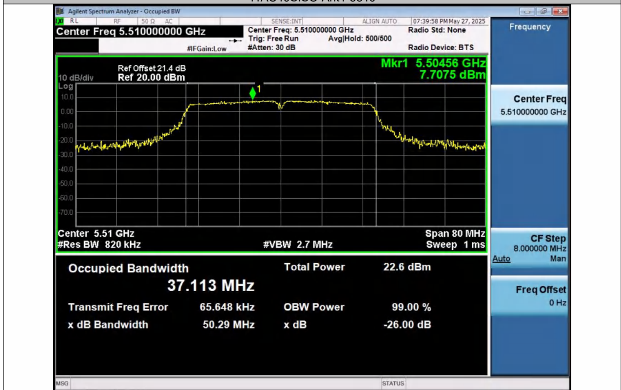
11AC40SISO-Ant1-5510
