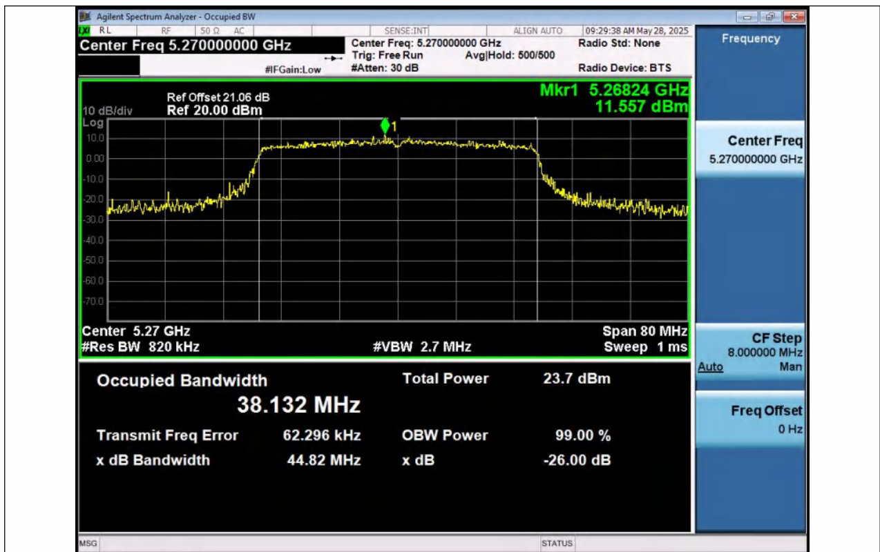
11AX40SISO-Ant1-5270
