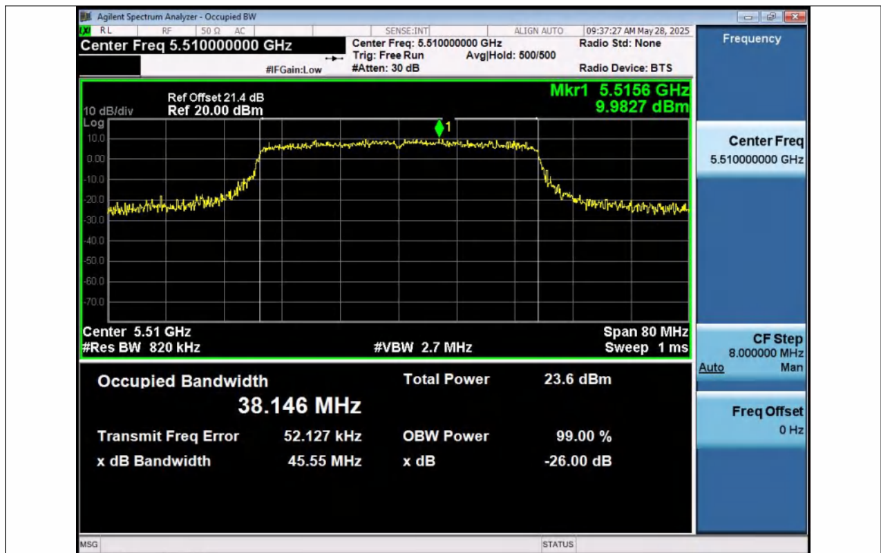
11AX40SISO-Ant1-5510
