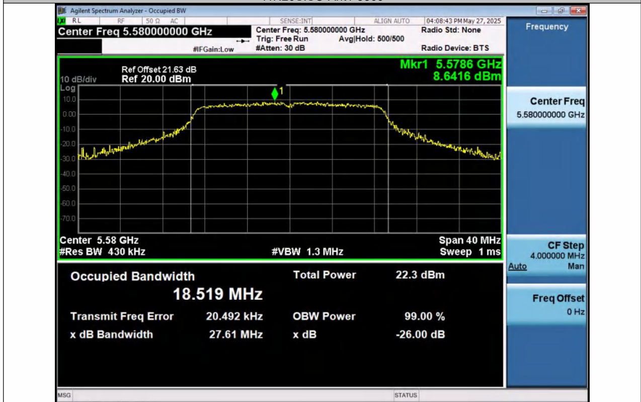
11N20SISO-Ant1-5580
