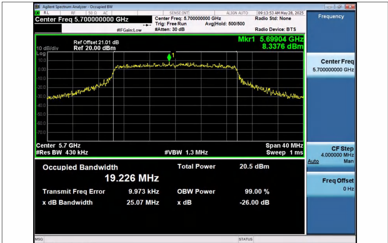
11AX20SISO-Ant1-5700
