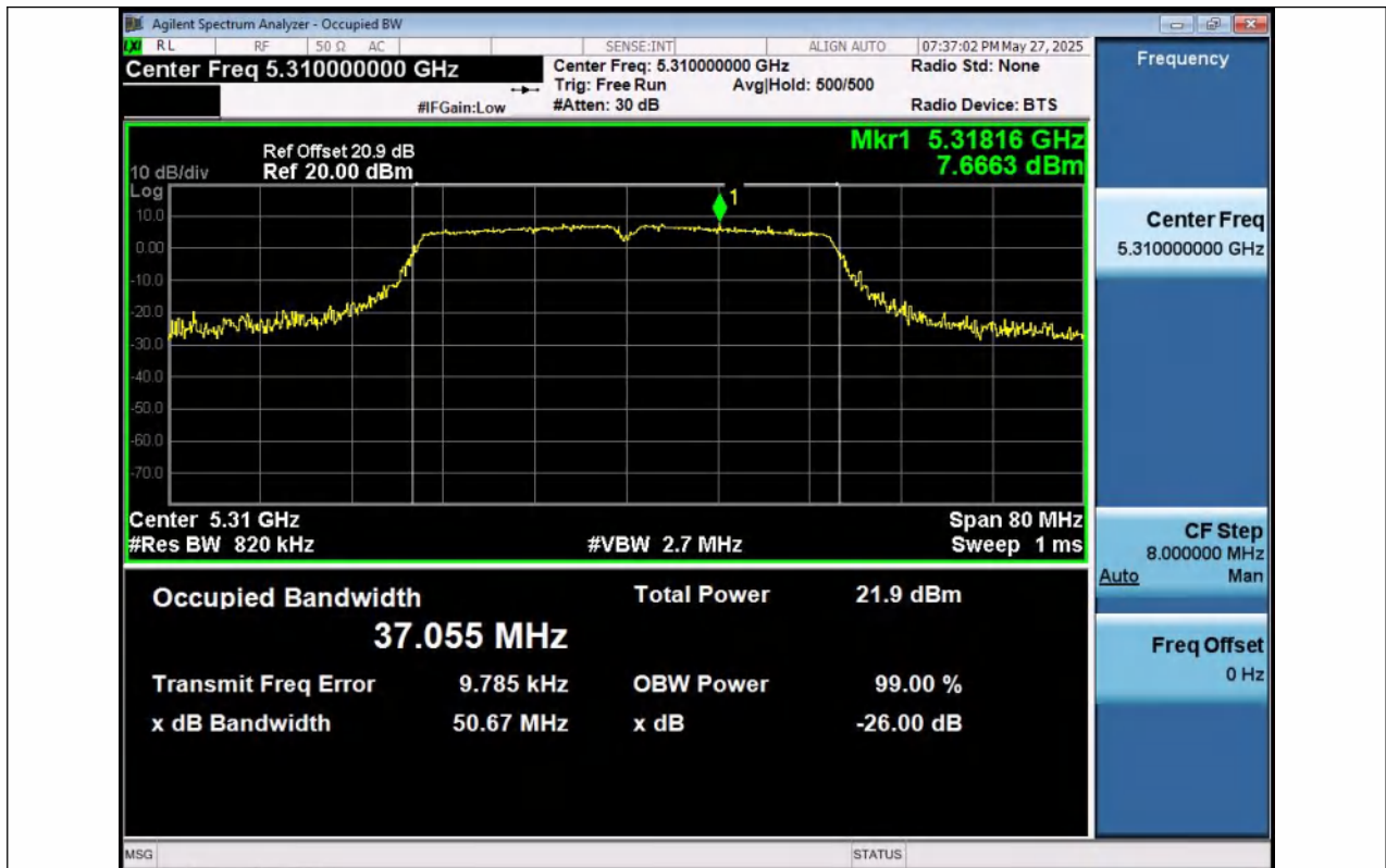
11AC40SISO-Ant1-5310
