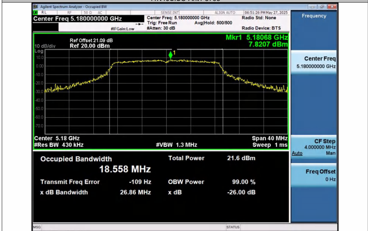
11AC20SISO-Ant1-5180
