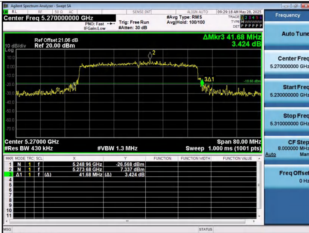
11AX40SISO-Ant1-5270
