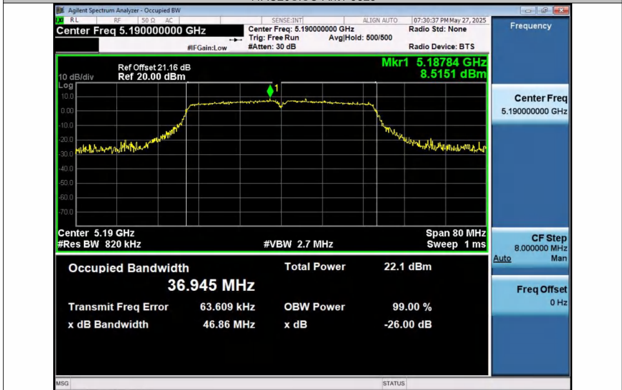
11AC40SISO-Ant1-5190
