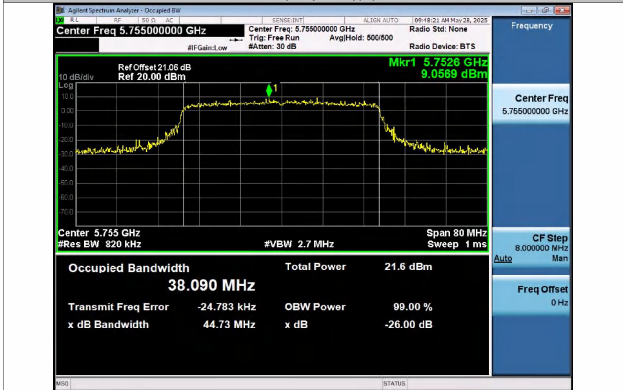
11AX40SISO-Ant1-5755
