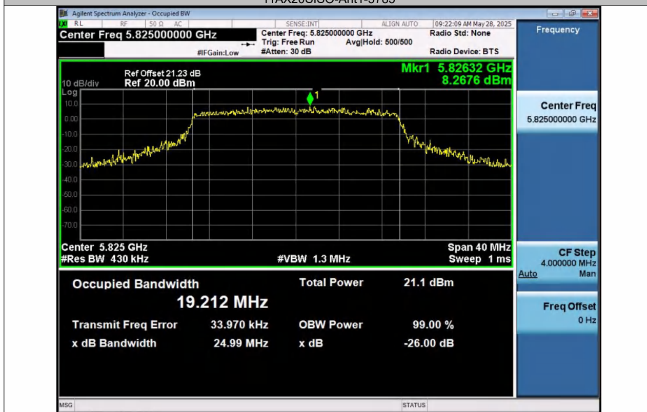
11AX20SISO-Ant1-5825
