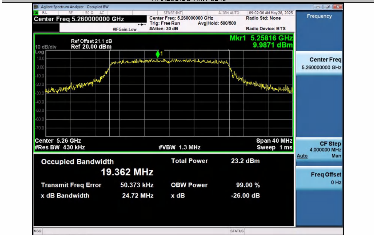
11AX20SISO-Ant1-5260
