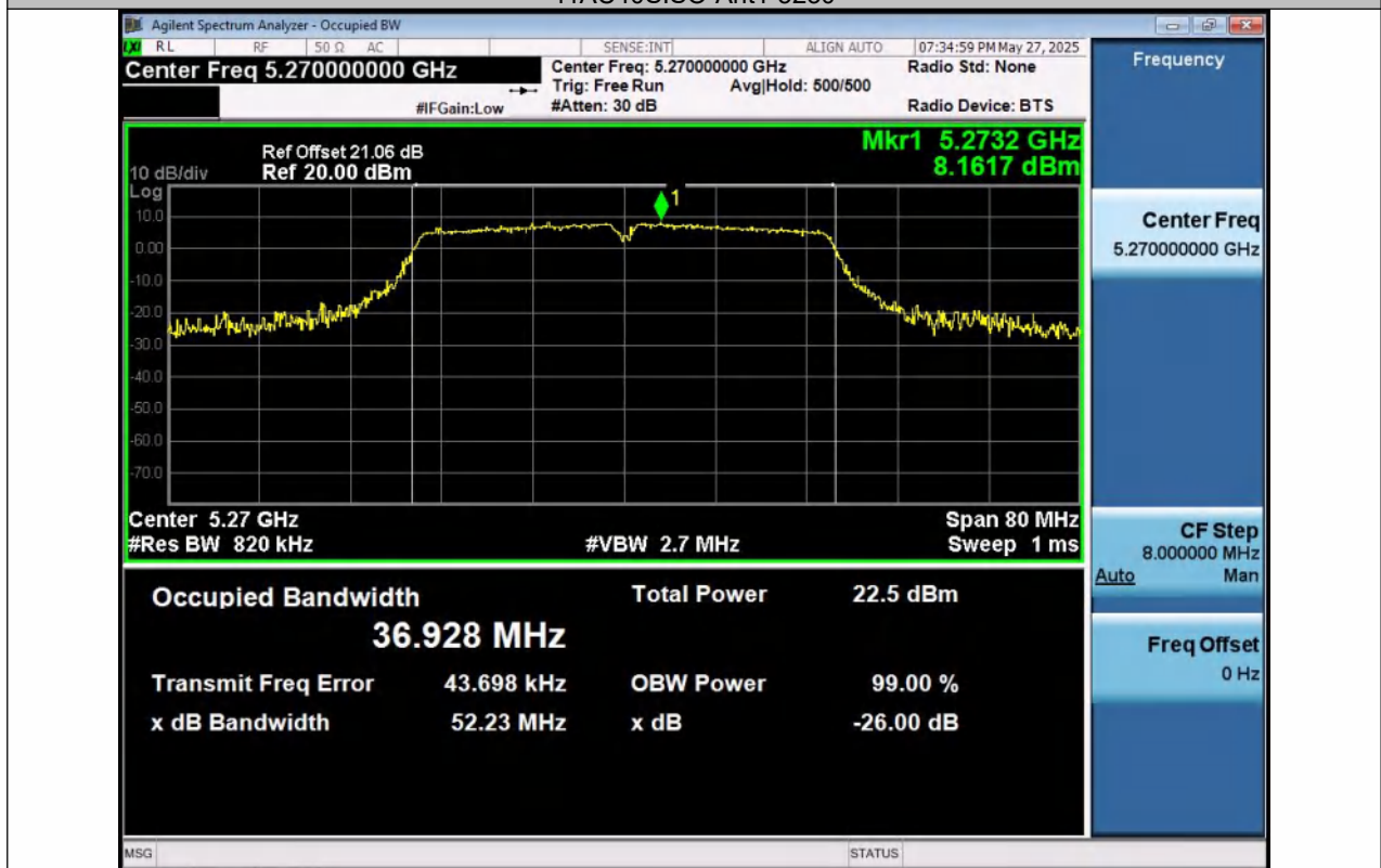
11AC40SISO-Ant1-5270
