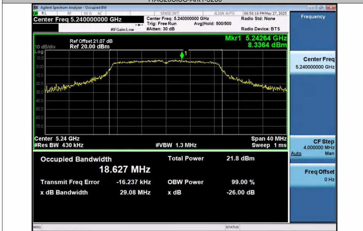
11AC20SISO-Ant1-5240
