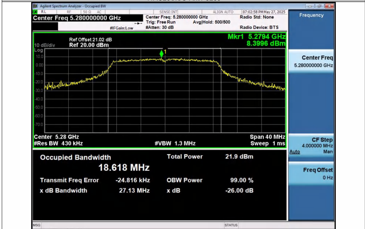
11AC20SISO-Ant1-5280
