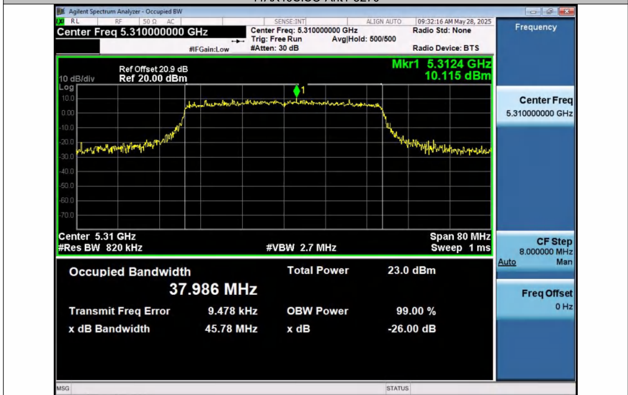
11AX40SISO-Ant1-5310
