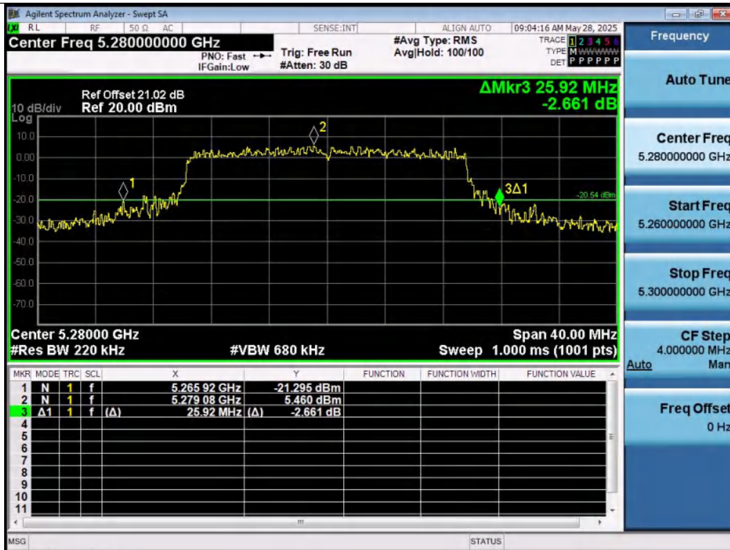
11AX20SISO-Ant1-5280
