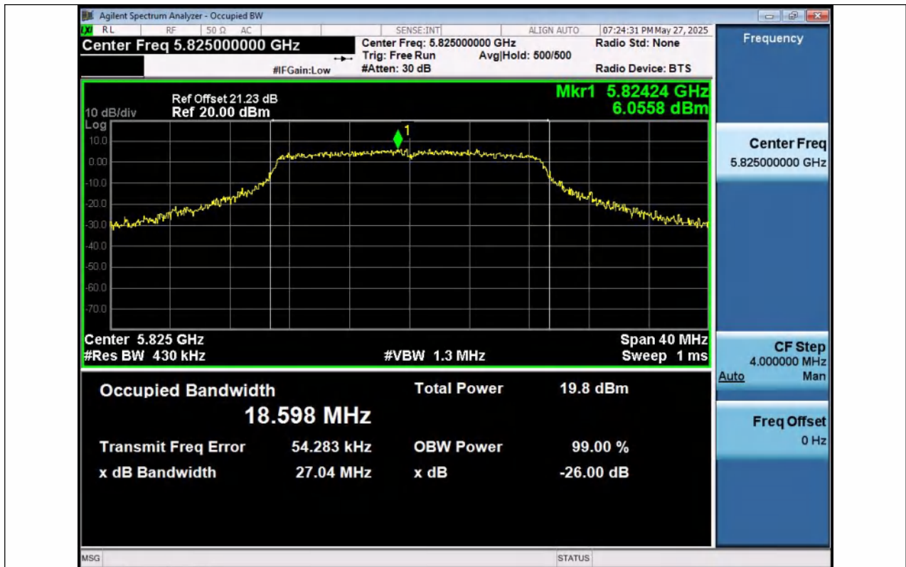
11AC20SISO-Ant1-5825
