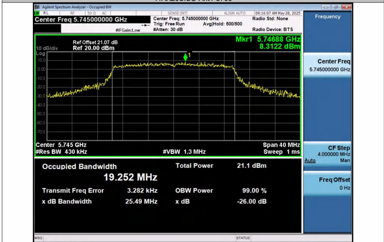
11AX20SISO-Ant1-5745
