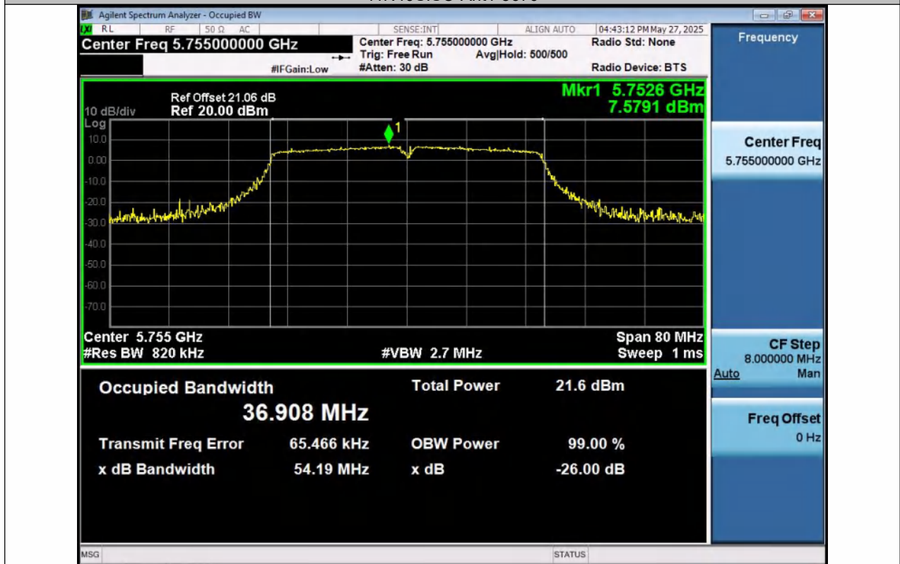
11N40SISO-Ant1-5755
