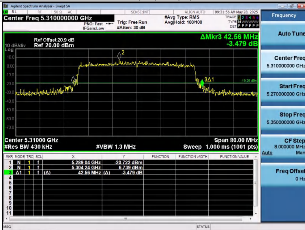
11AX40SISO-Ant1-5310
