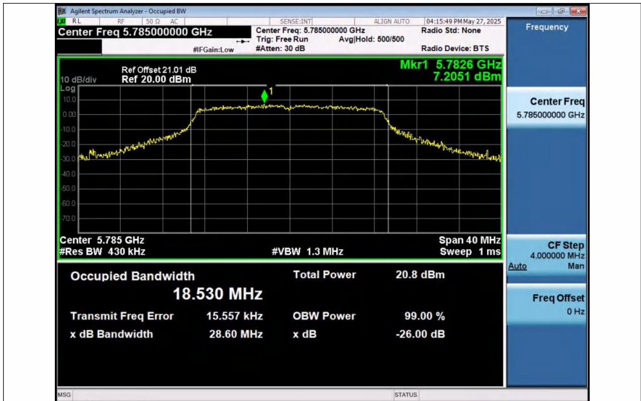
11N20SISO-Ant1-5785
