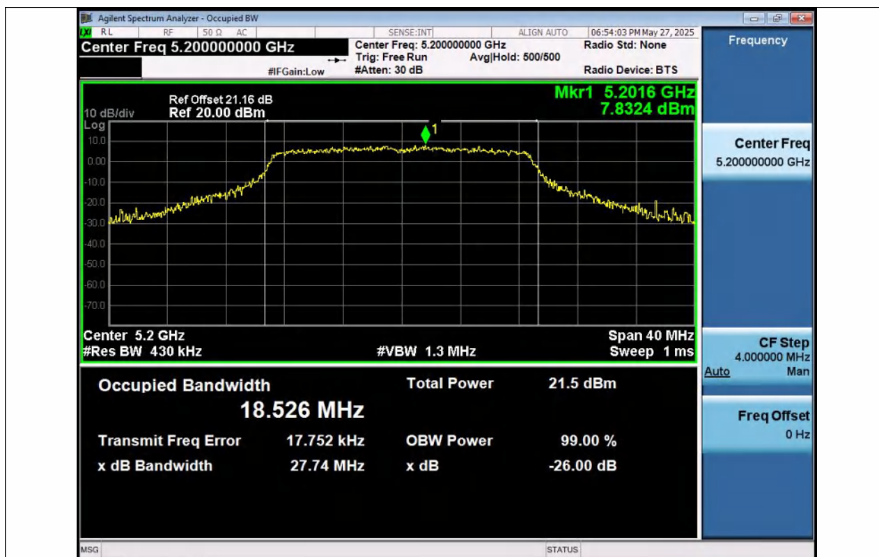
11AC20SISO-Ant1-5200
