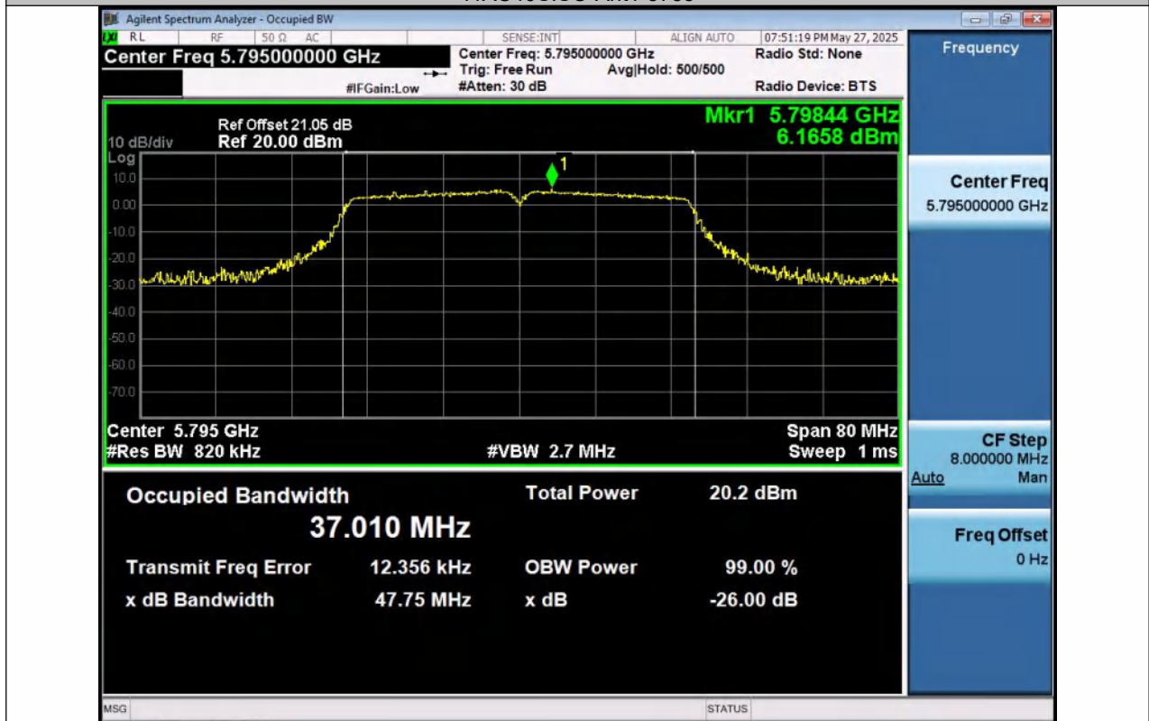
11AC40SISO-Ant1-5795
