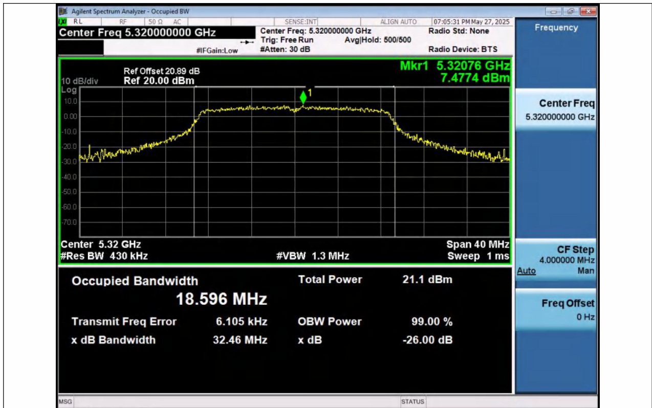
11AC20SISO-Ant1-5320
