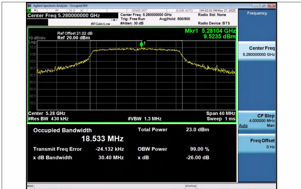
11N20SISO-Ant1-5280
