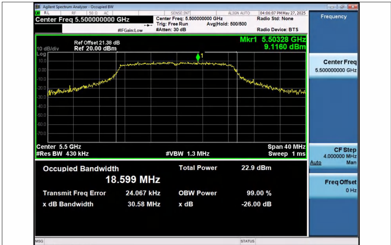
11N20SISO-Ant1-5500
