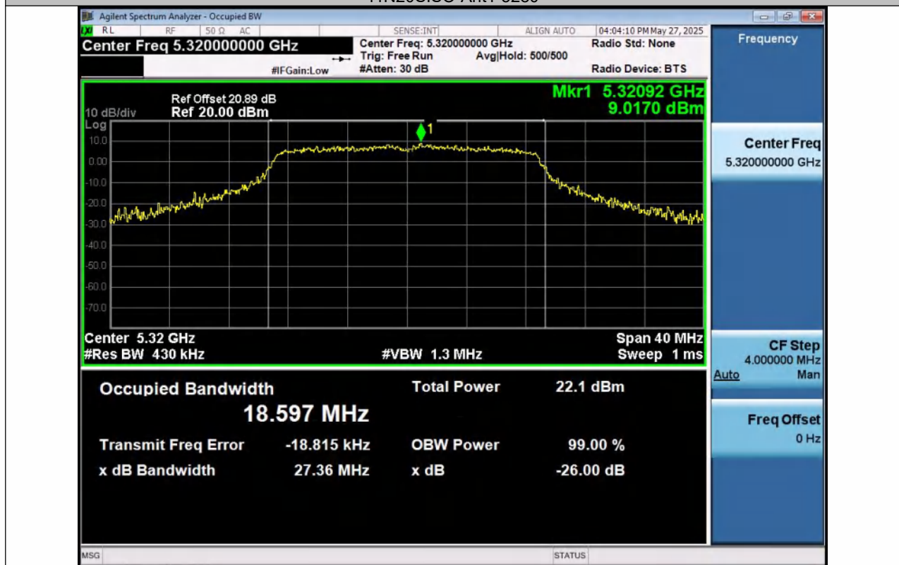
11N20SISO-Ant1-5320
