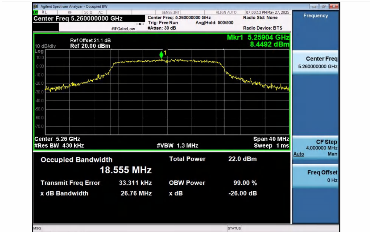
11AC20SISO-Ant1-5260
