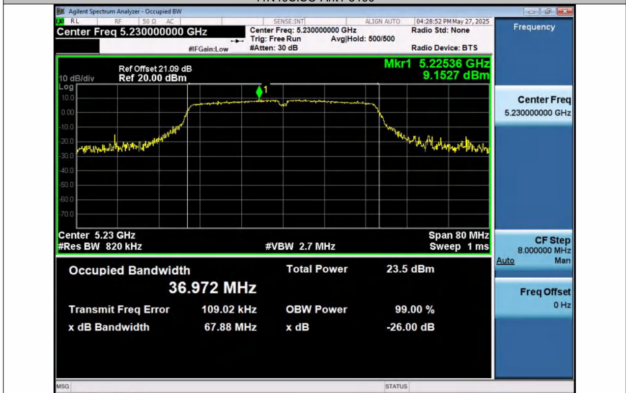
11N40SISO-Ant1-5230
