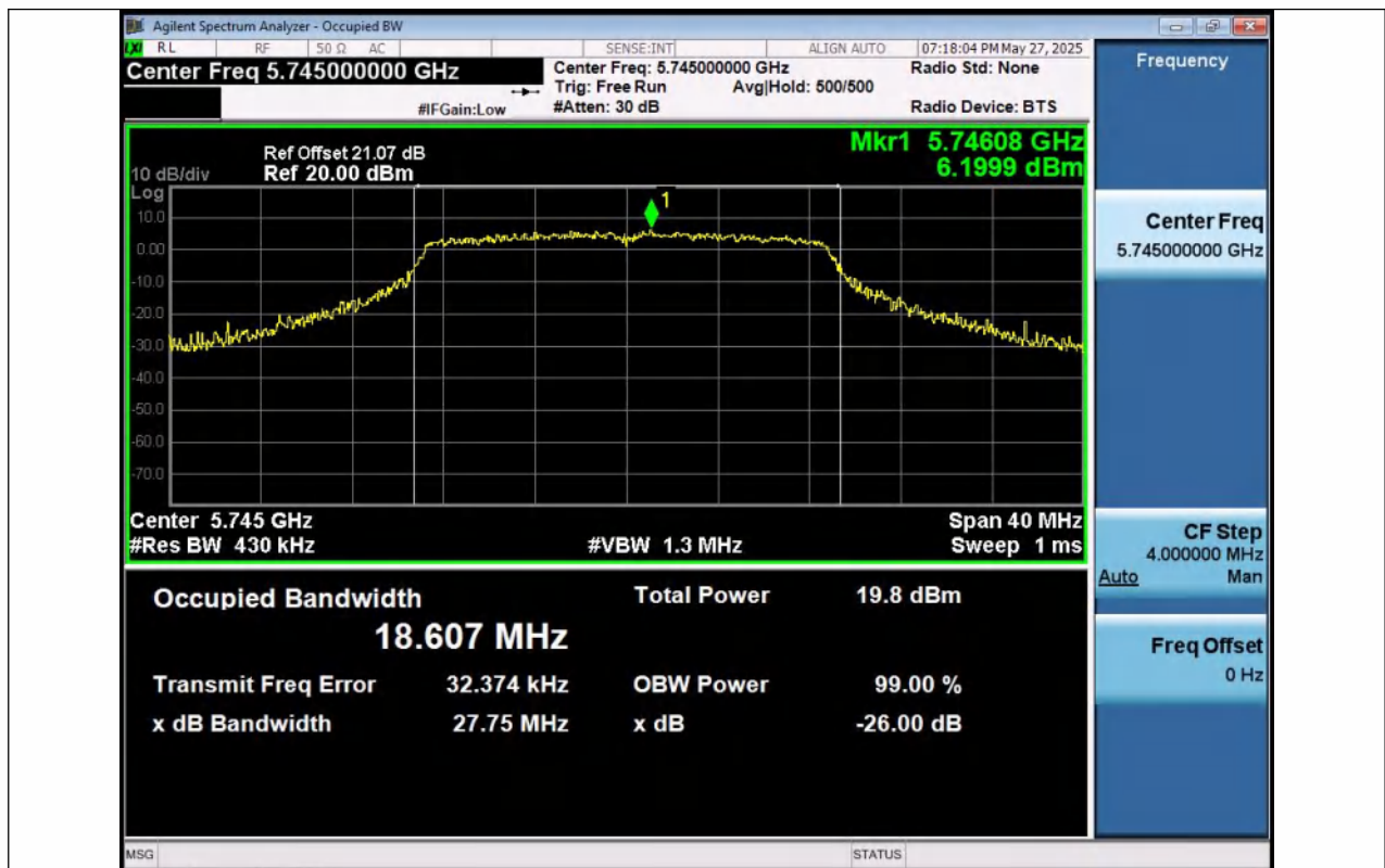
11AC20SISO-Ant1-5745
