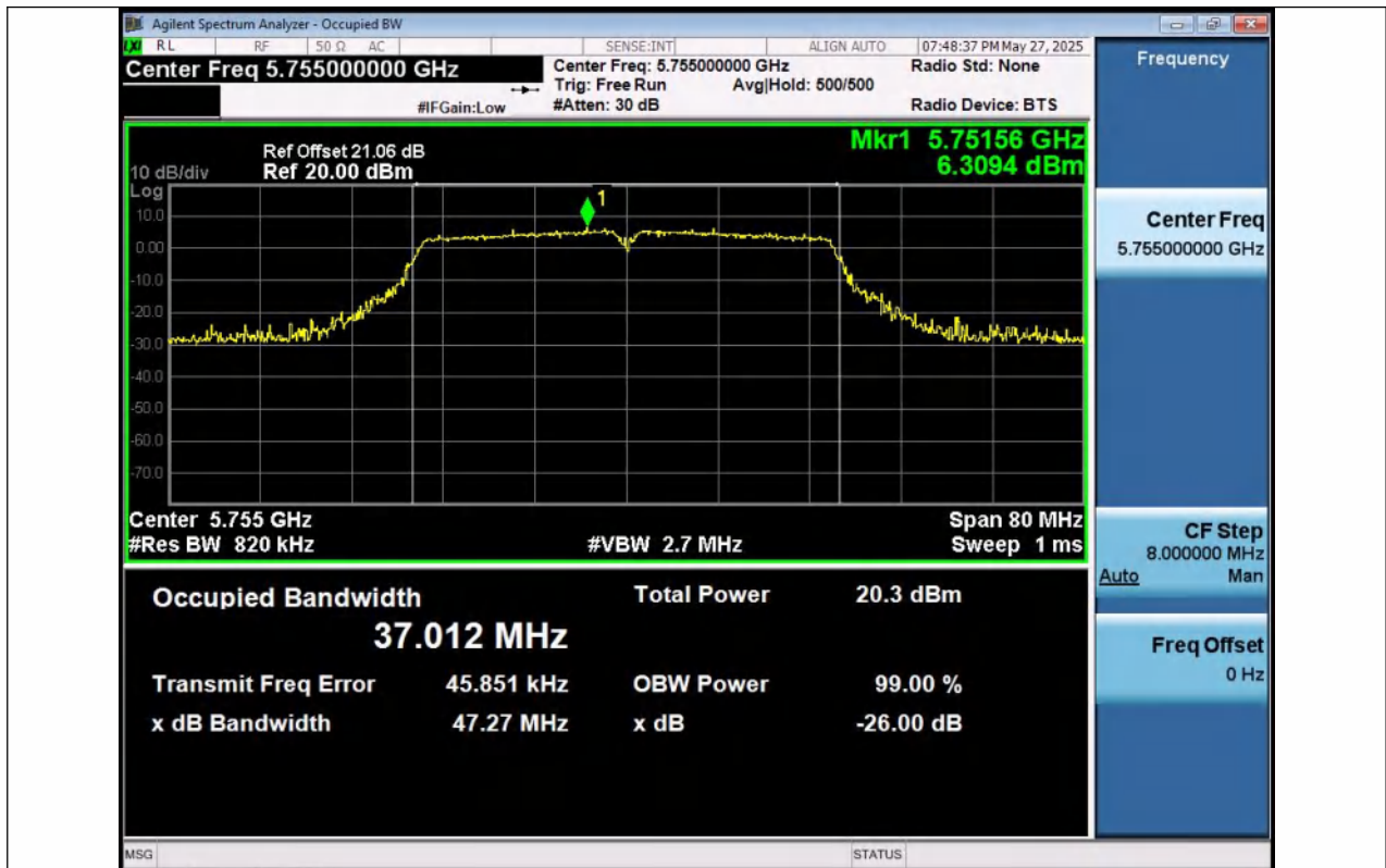
11AC40SISO-Ant1-5755
