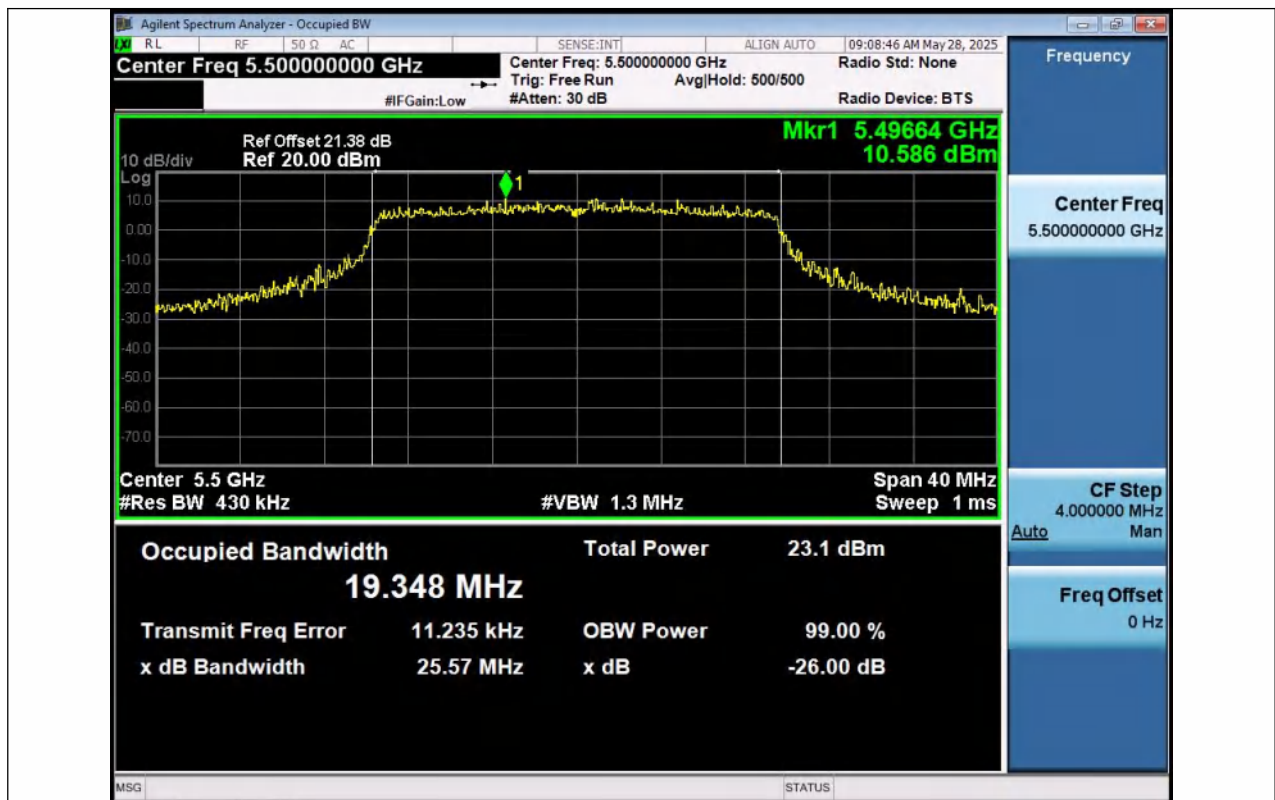
11AX20SISO-Ant1-5500
