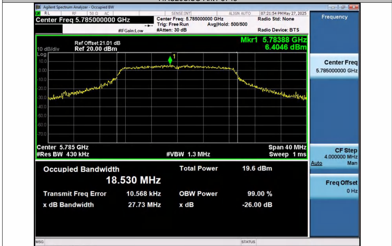
11AC20SISO-Ant1-5785
