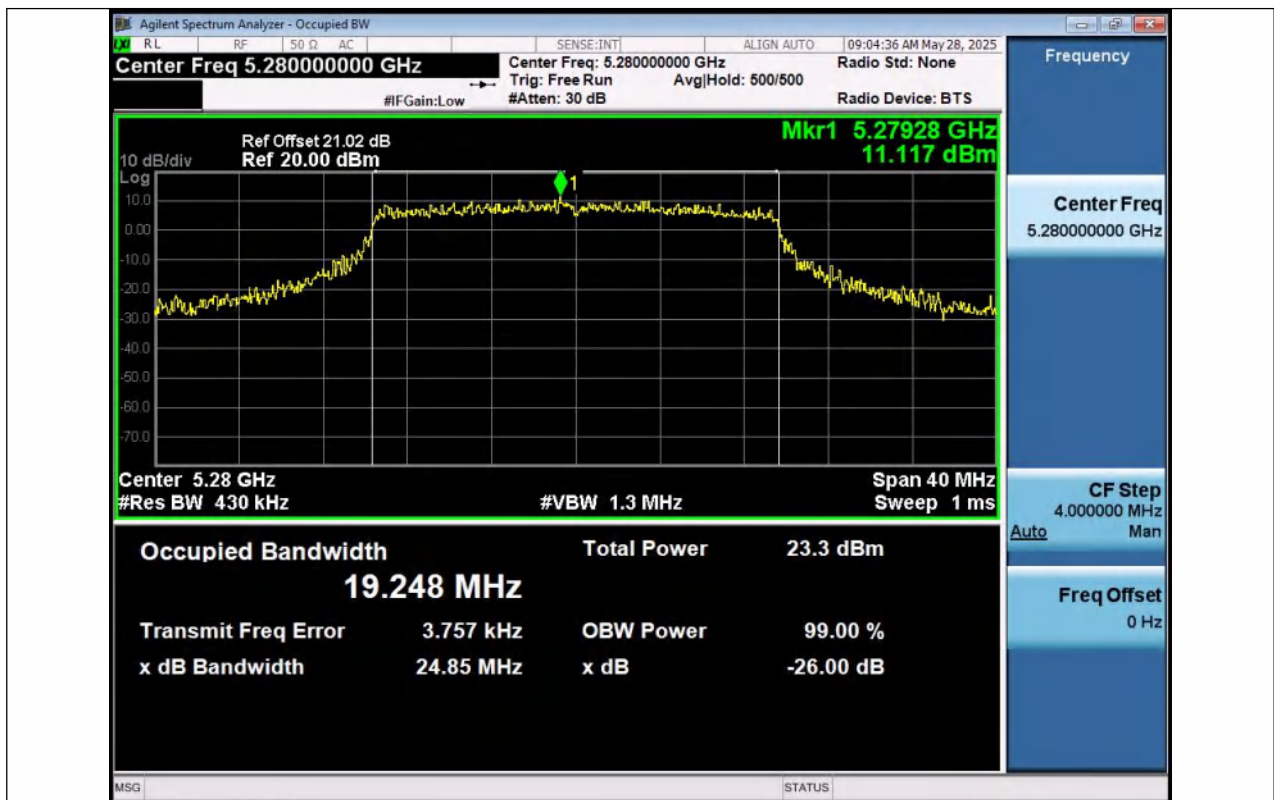
11AX20SISO-Ant1-5280
