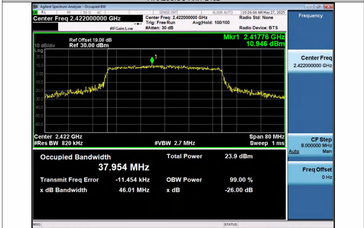
11AX40SISO-Ant1-2422
