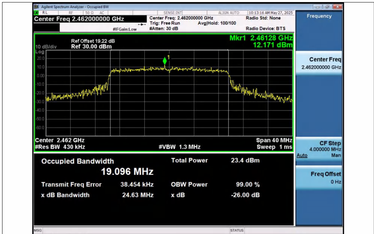
11AX20SISO-Ant1-2462
