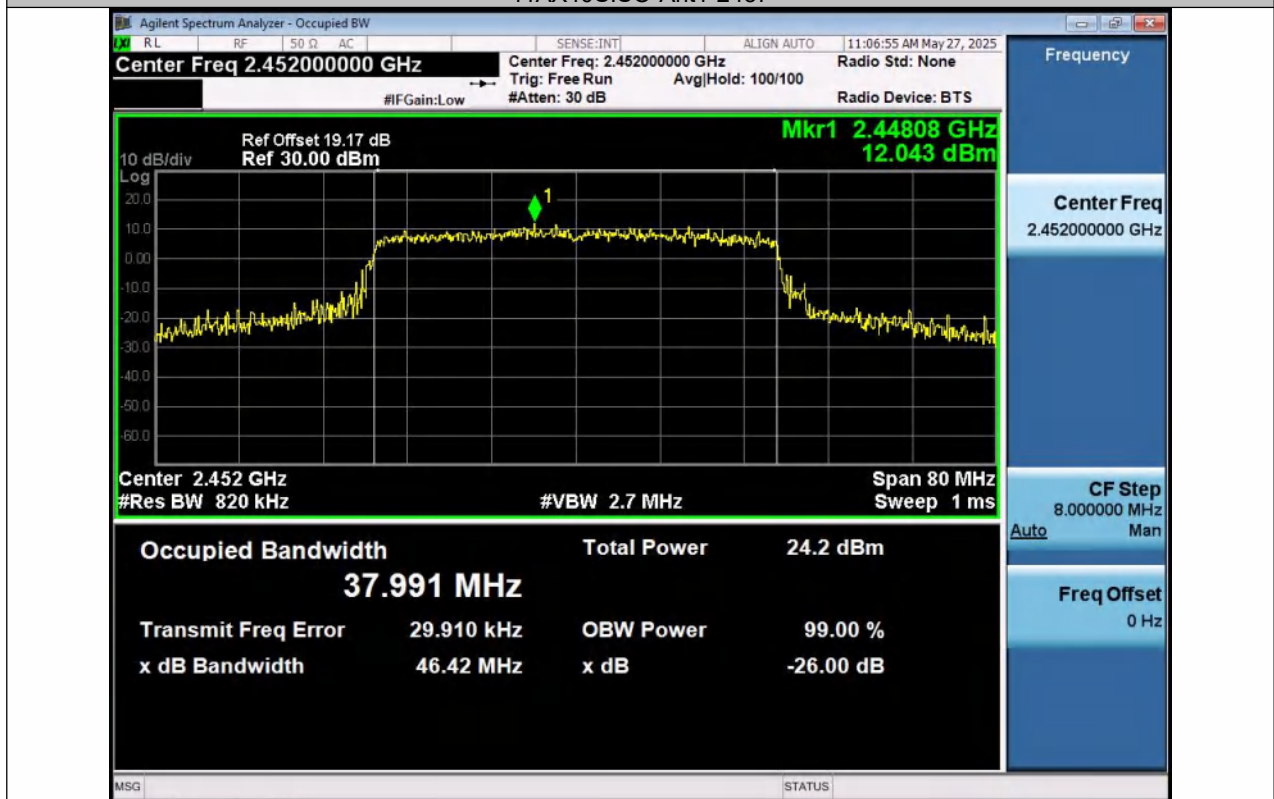
11AX40SISO-Ant1-2452
