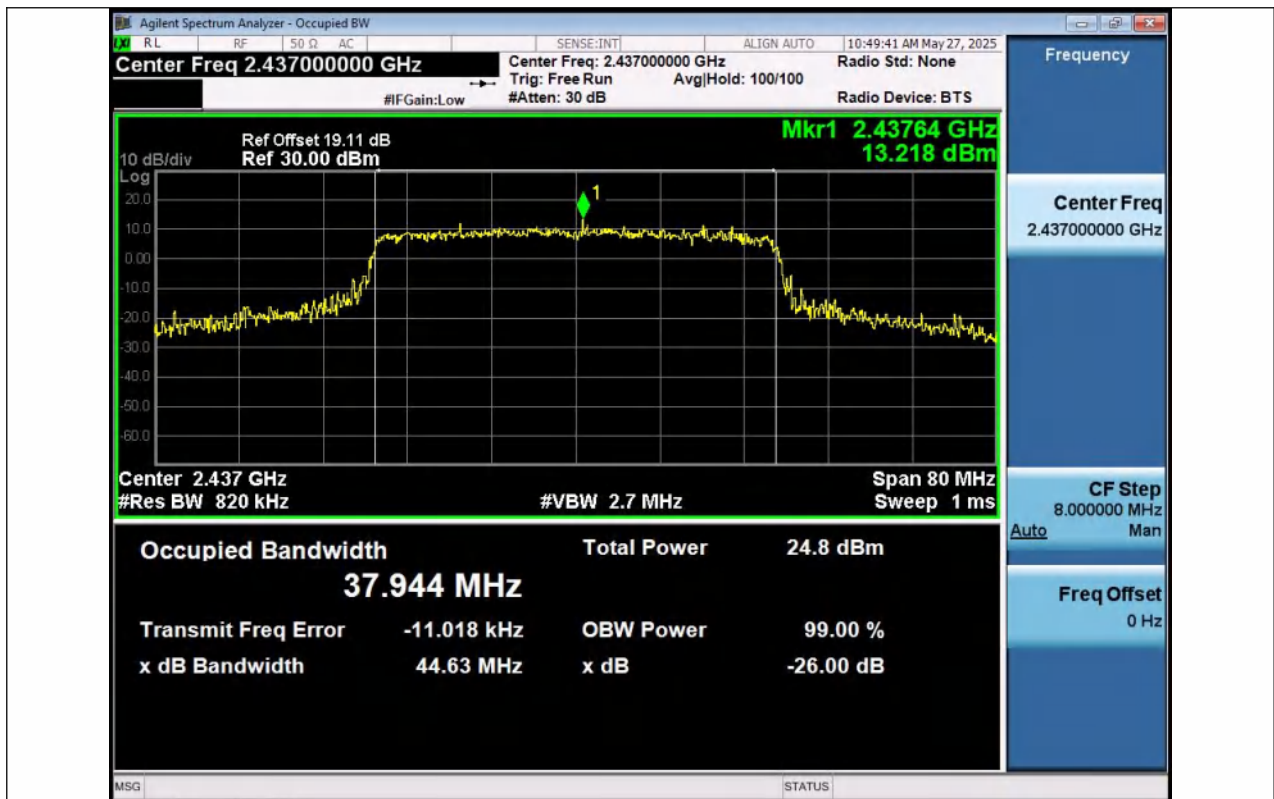
11AX40SISO-Ant1-2437
