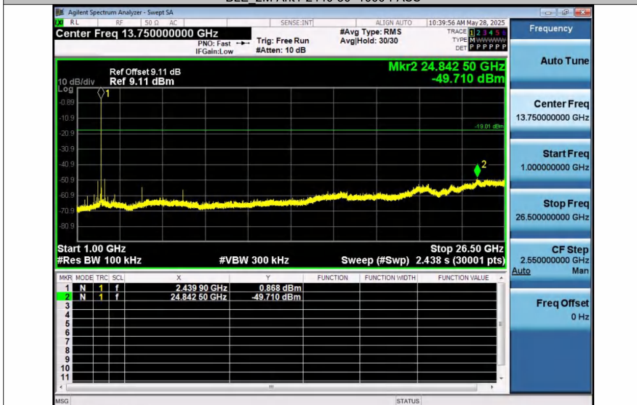
BLE_2M-Ant1-2440-1000~26500-PASS
