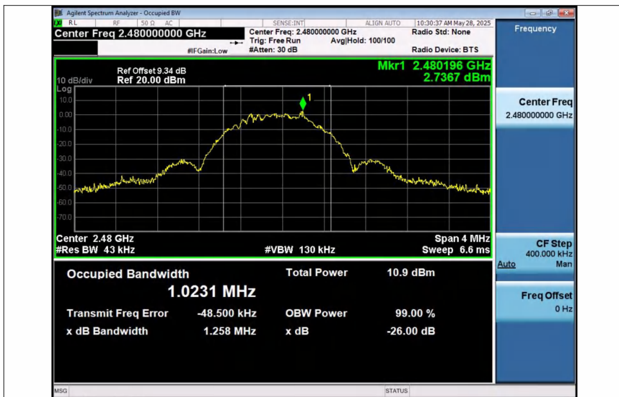
BLE_1M-Ant1-2480
