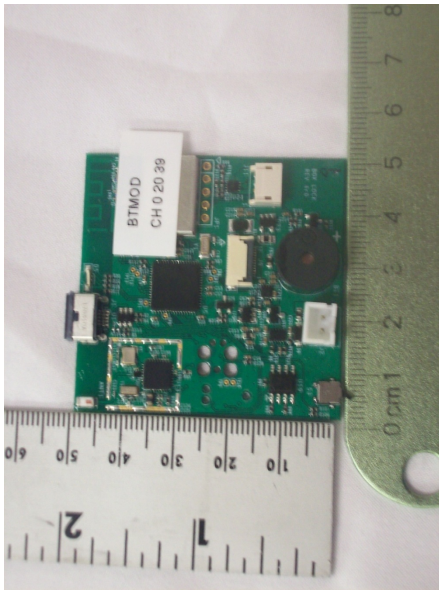
Figure 8. PCB with WiFi Module (no shield) and BT Module (with Shield)
