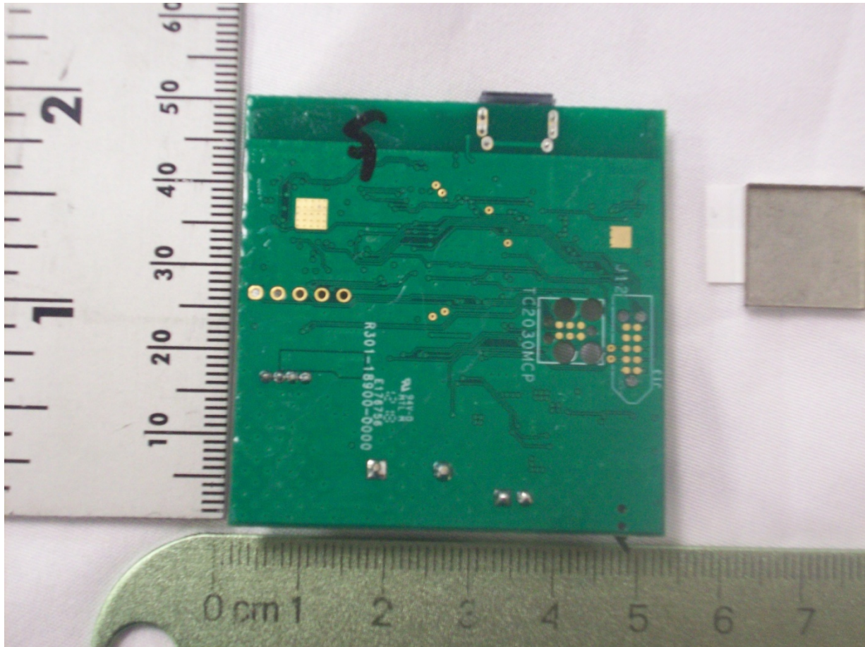
Figure 10. PCB, Back
