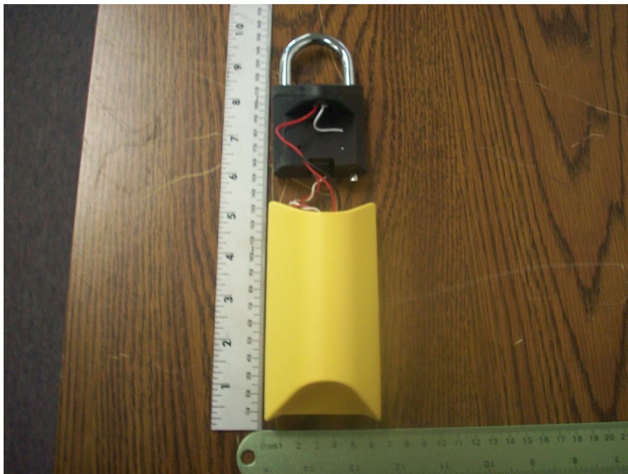
Figure 6. Locking Mechanism (Bar Code Scanner) Removed
