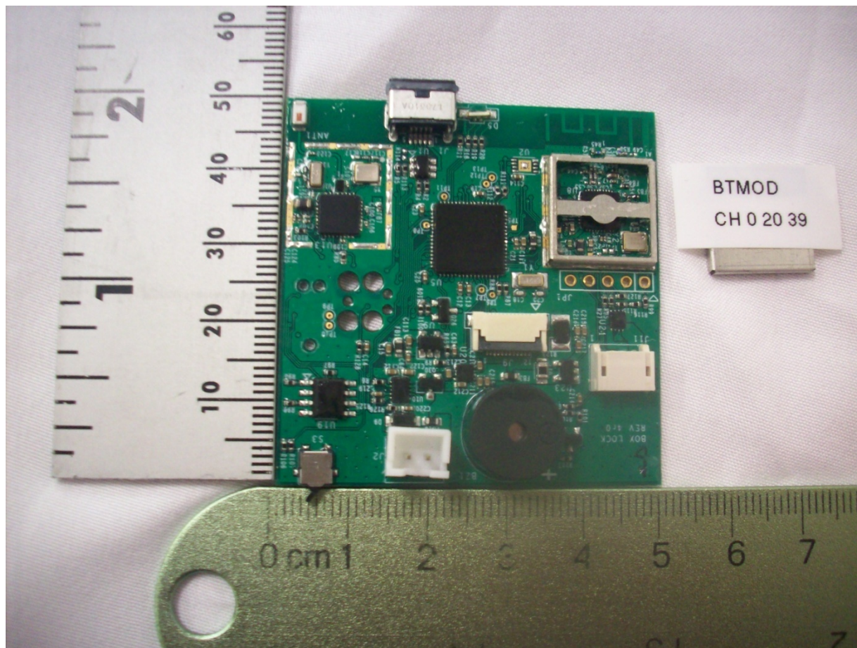
Figure 9. PCB with WiFi Module (no shield) and BT Module, Top of Shield Removed
