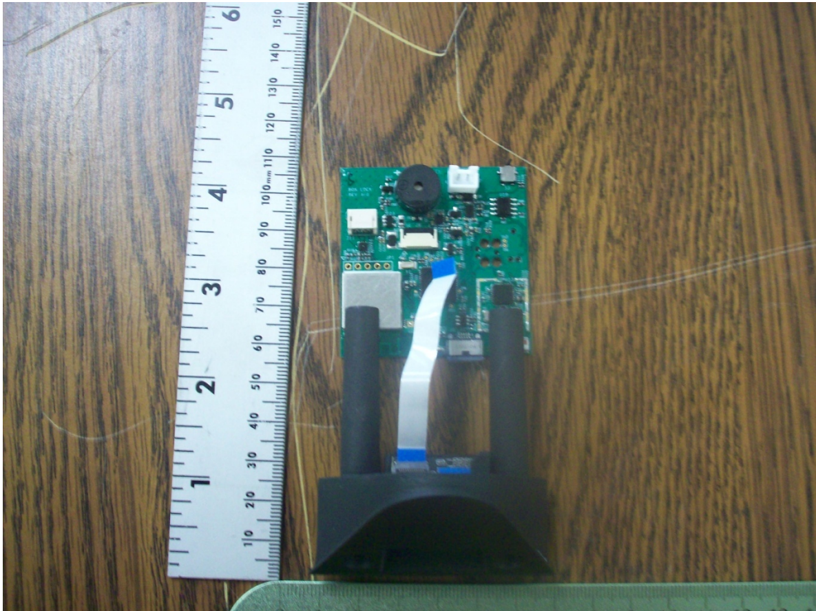
Figure 4. Bottom Piece Removed, with PCB Attached
