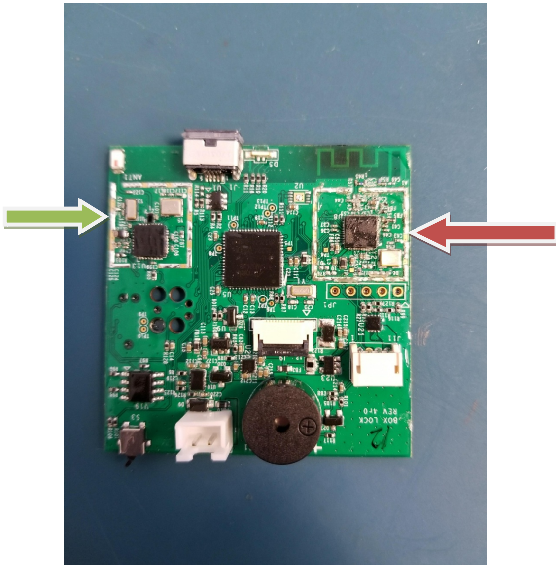
Figure 9. Main PCB with WiFi Module (green arrow) and BT Module (red arrow), Shield Removed
