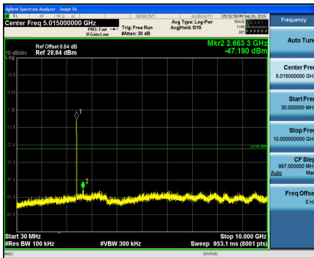
30MHz-10GHz
