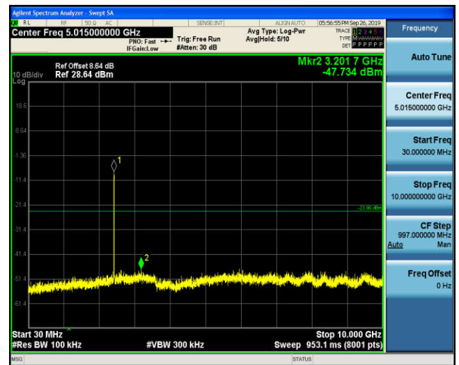
30MHz-10GHz
