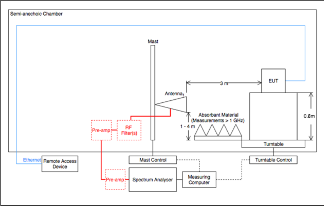
Figure 1 - Example Test Setup
