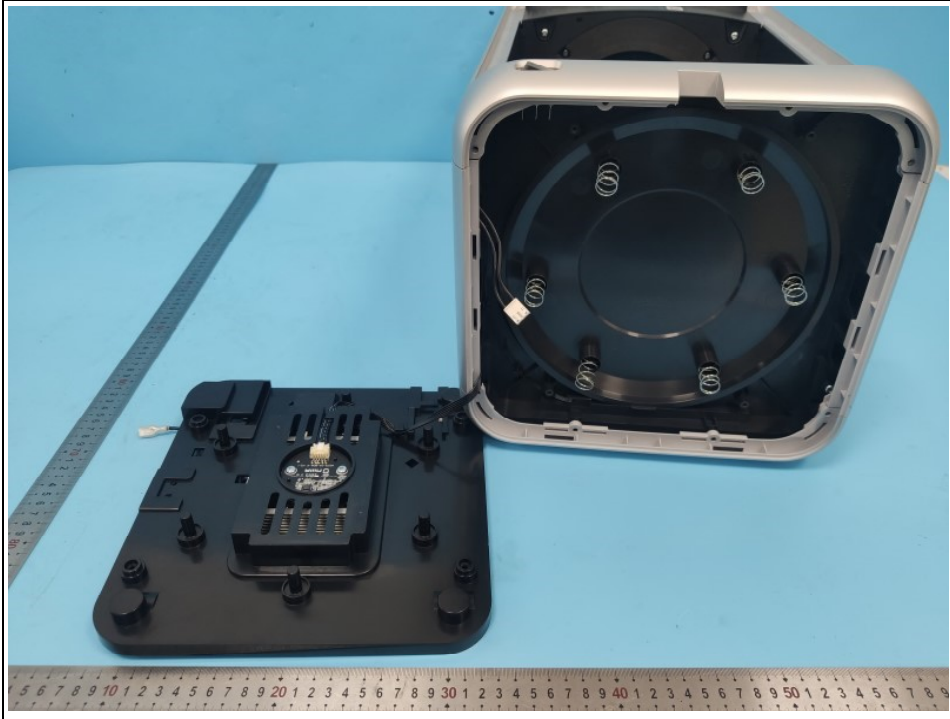
Fig.20 Disassembly view
