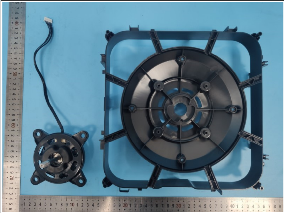
Fig. 47 Disassembly view
