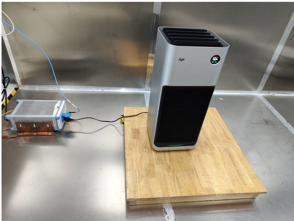
Photograph 4: Set-up photo for Conducted Emissions on AC Mains
