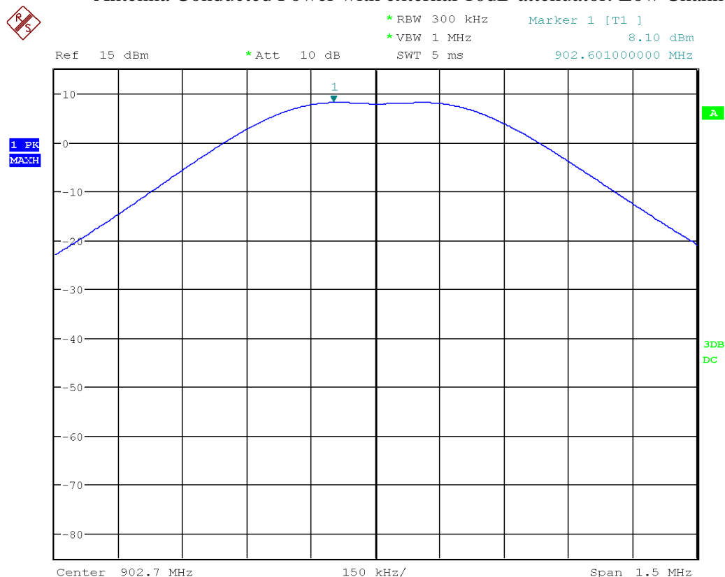
Antenna Conducted Power with external 10dB attenuator: Low Channel
