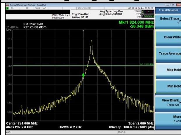
Band 26_15KHz_1#0_BPSK_Low
