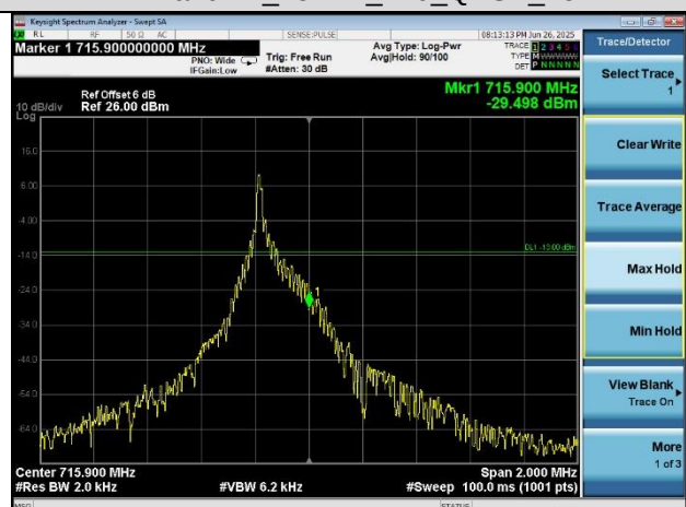
Band 12_15KHz_1#0_QPSK_Low
