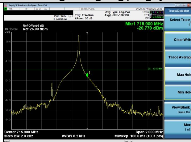
Band 17_15KHz_1#0_QPSK_Low
