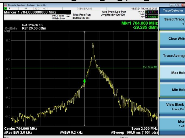
Band 17_15KHz_1#0_QPSK_Low
