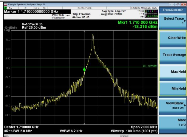
Band 4_15KHz_1#0_QPSK_Low
