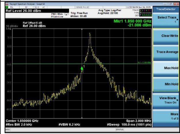
Band 2_15KHz_1#0_BPSK_Low
