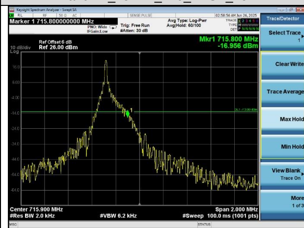
Band 12_15KHz_1#0_BPSK_Low
