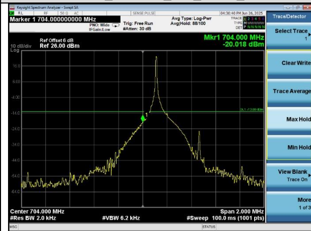
Band 17_3.75KHz_1#47_BPSK_High
