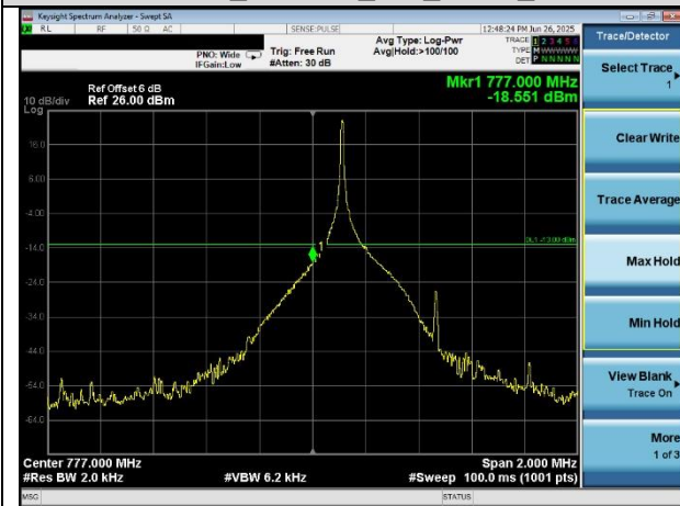
Band 13_3.75KHz_1#47_BPSK_High
