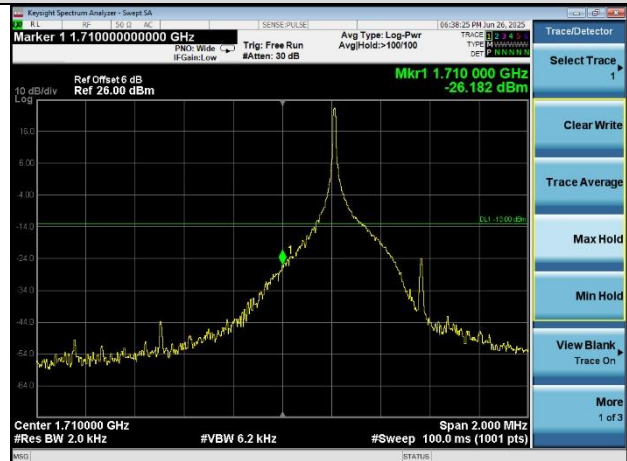
Band 66_3.75KHz_1#47_QPSK_High
