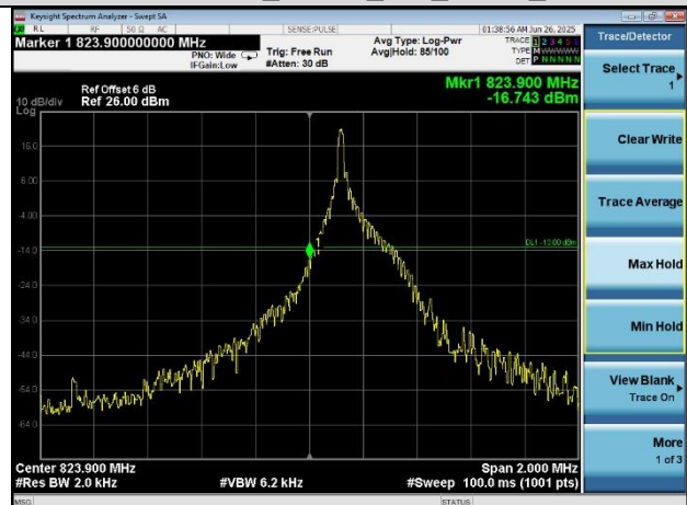
Band 5_15KHz_1#0_QPSK_Low
