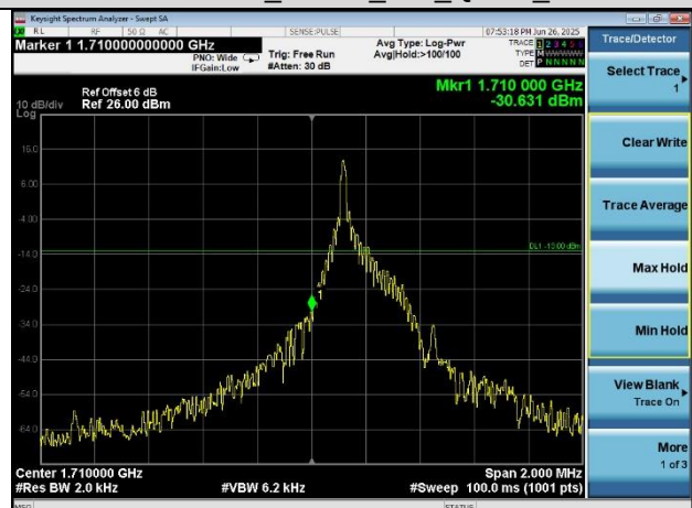
Band 66_15KHz_1#0_QPSK_Low
