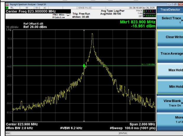
Band 5_15KHz_1#0_BPSK_Low
