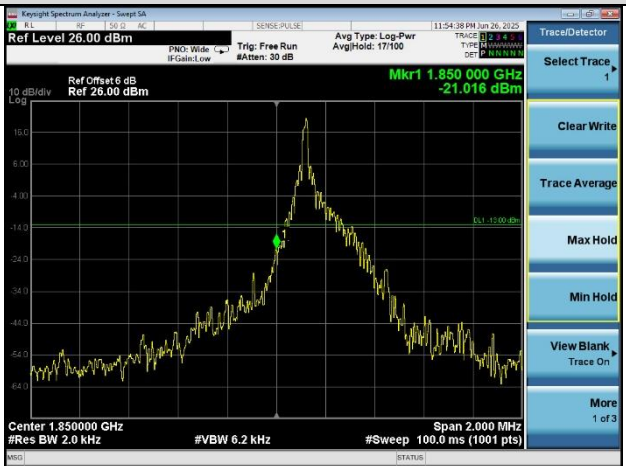
Band 2_15KHz_1#0_QPSK_Low
