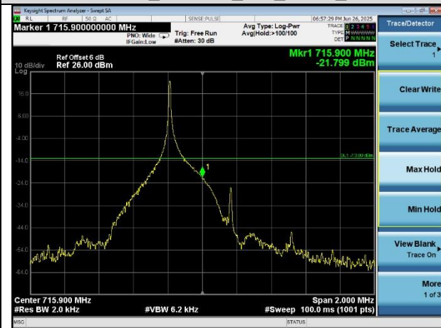
Band 12_3.75KHz_1#47_BPSK_High
