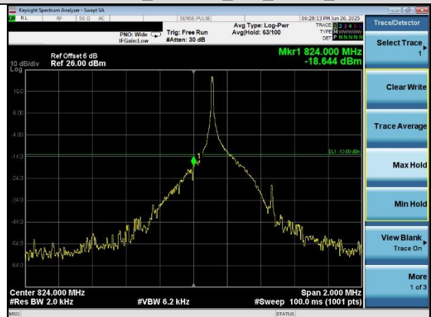
Band 26_3.75KHz_1#47_QPSK_High
