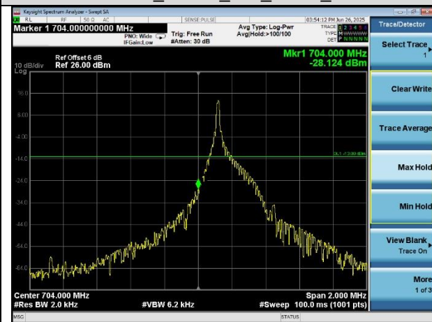
Band 17_15KHz_1#0_BPSK_Low
