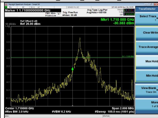
Band 66_15KHz_1#0_BPSK_Low
