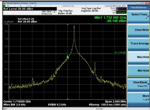
Band 4_3.75KHz_1#47_QPSK_High
