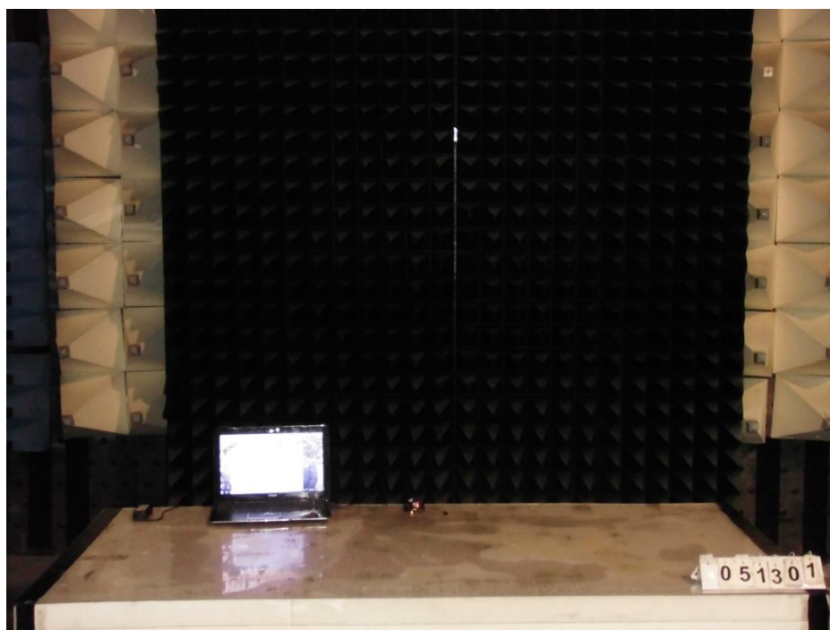
03.Radiation Measurement 30MHz to 1GHz (Front)
