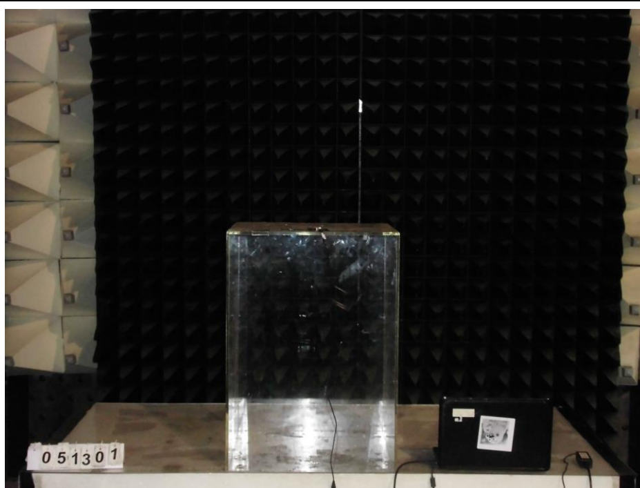
06. Radiation Measurement Above 1GHz (Rear)
