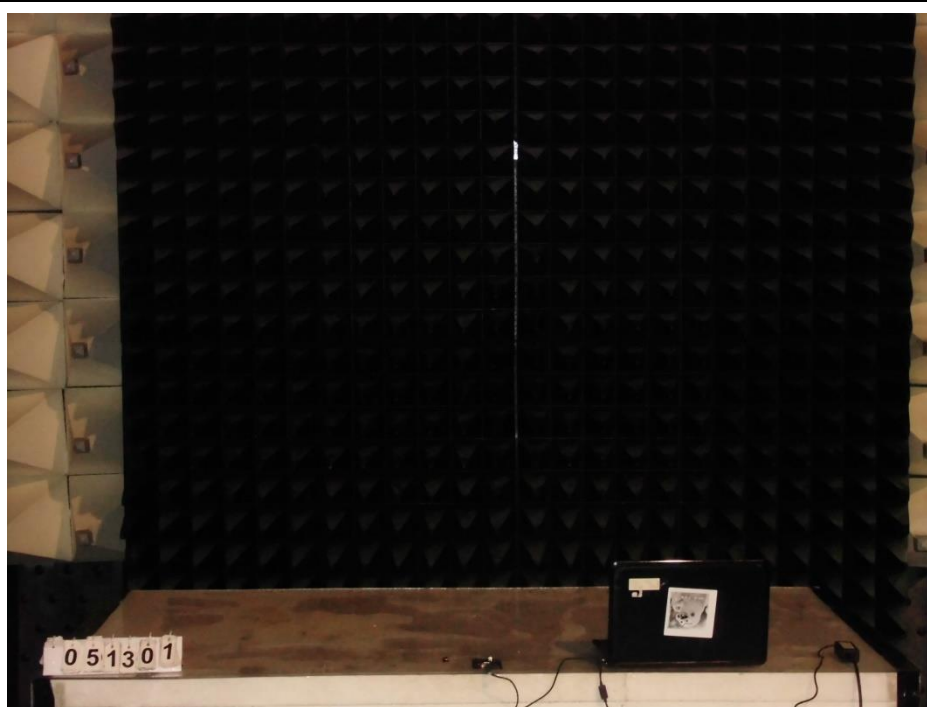
04.Radiation Measurement 30MHz to 1GHz (Rear)
