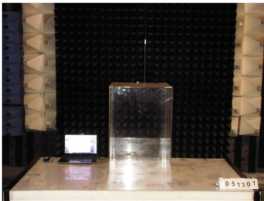
05. Radiation Measurement Above 1GHz (Front)
