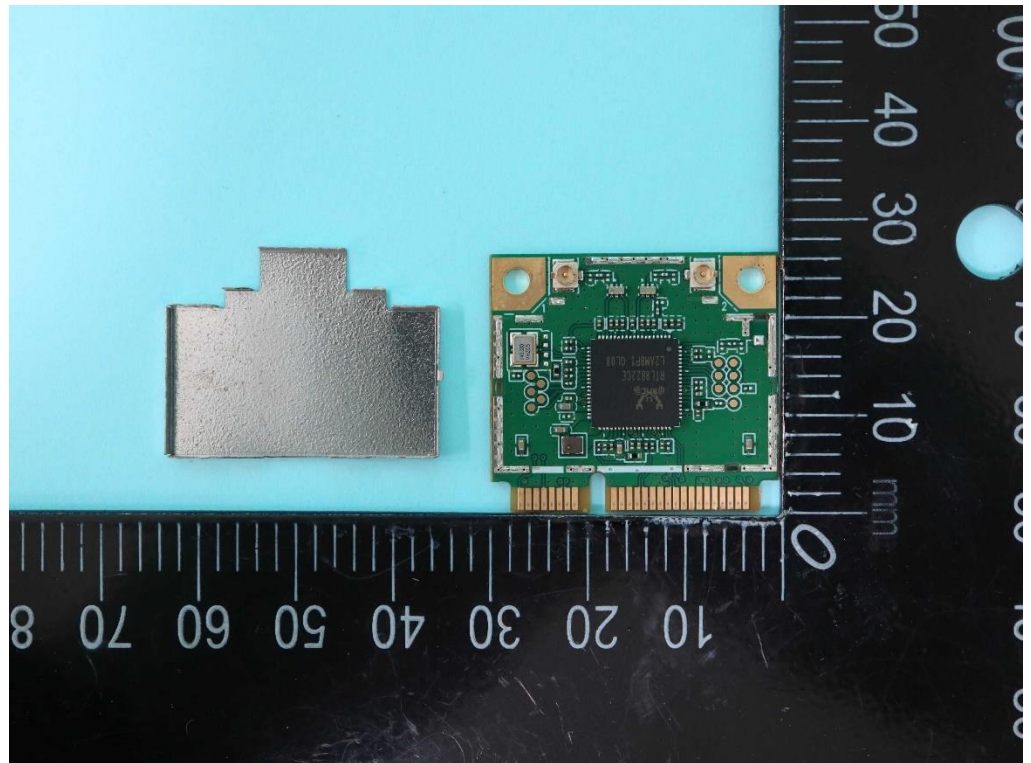
MCR822CE-P With MHF1 connector (One Generations Connector)
