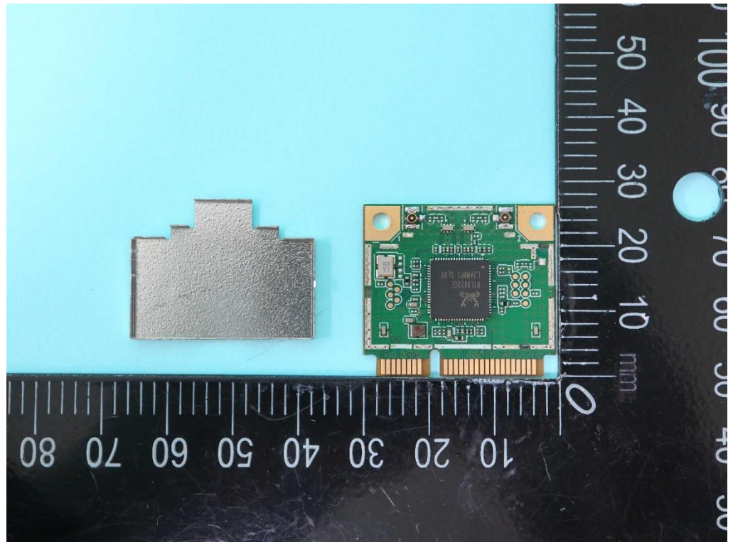
MCR822CE-P4 With MHF4 connector (Four Generations Connector)
