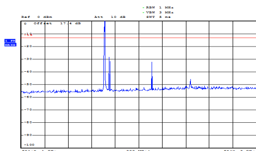
LTE Band 4 1.4MHz CH-Low 1GHz~3GHz
