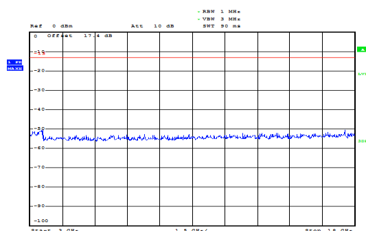
LTE Band 4 1.4MHz CH-Middle 3GHz~18GHz
