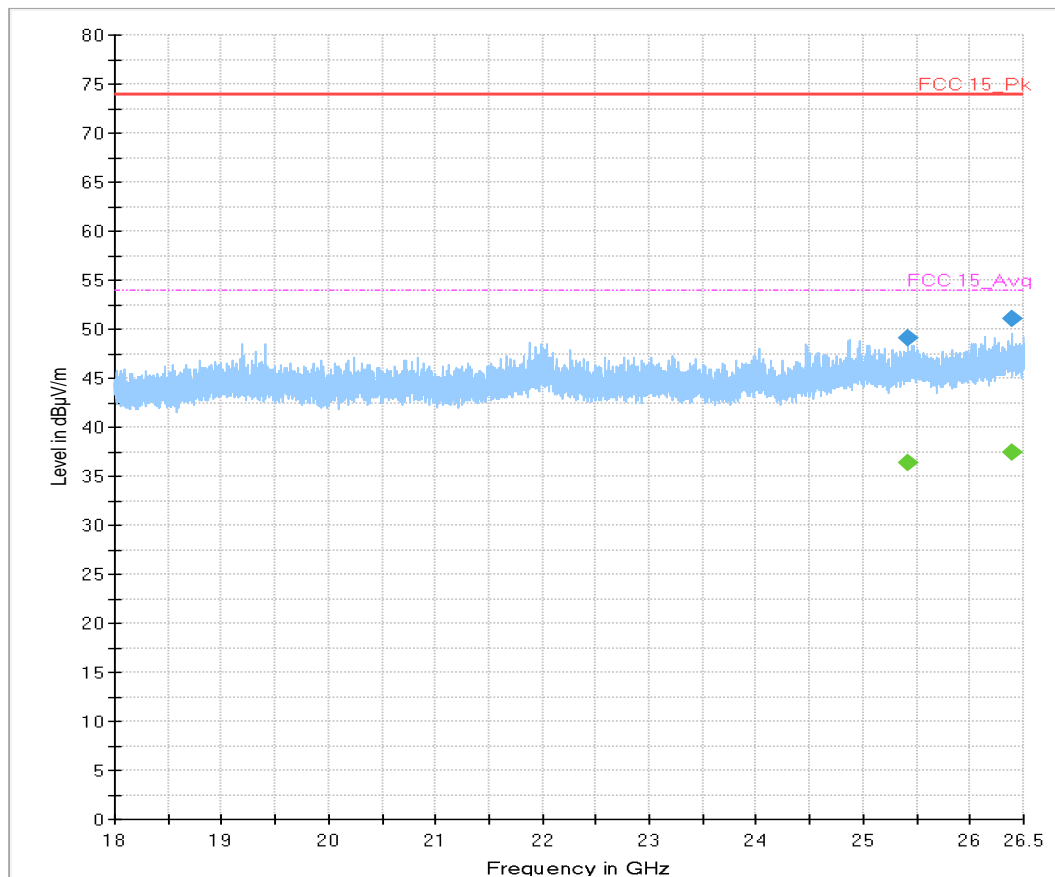
Plot 42. 18-26.5GHz, 1Mbps, 2440MHz
