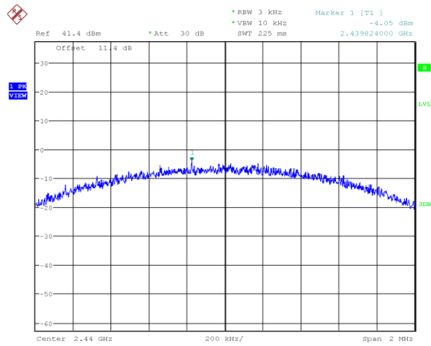
Plot 17. 2Mbps, 2440MHz PSD
