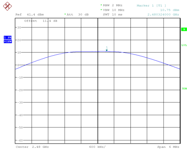
Plot 6. Maximum Conducted Power, 2Mbps 2480MHz
