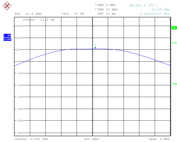
Plot 4. Maximum Conducted Power, 2Mbps 2402MHz
