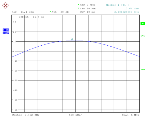
Plot 1. Maximum Conducted Power, 1Mbps 2402MHz
