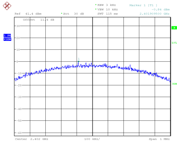
Plot 13. 1Mbps, 2402MHz PSD
