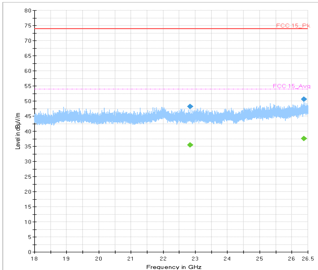
Plot 43. 18-26.5GHz, 1Mbps, 2480MHz
