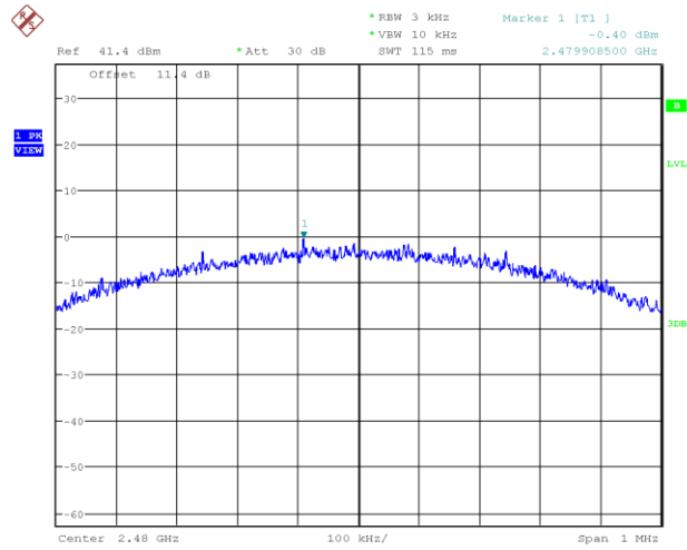
Plot 15. 1Mbps, 2480MHz PSD
