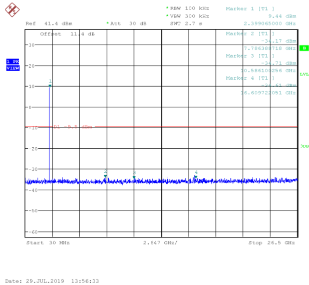
Plot 25. 1Mbps, 2402MHz 30MHz-26.5GHz Spurious
