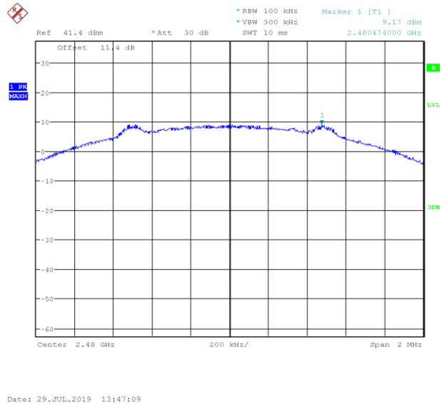
Plot 24. Non-Restricted Reference Measurement, 2Mbps 2480MHz
