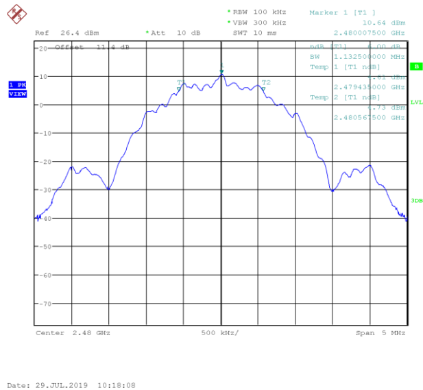
Plot 12. 2Mbps, 2480MHz, 6dB Bandwidth
