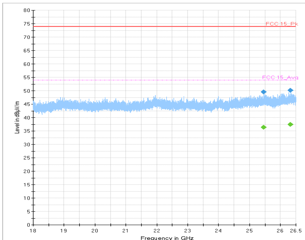
Plot 41. 18-26.5GHz, 1Mbps, 2402MHz
