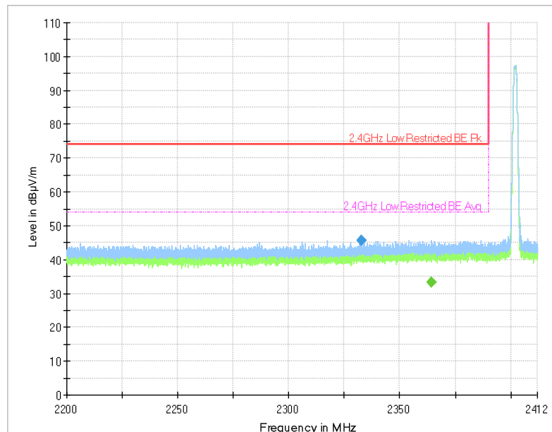
Plot 31. 1Mbps, 2402MHz, Lower Band Edge, Restricted
