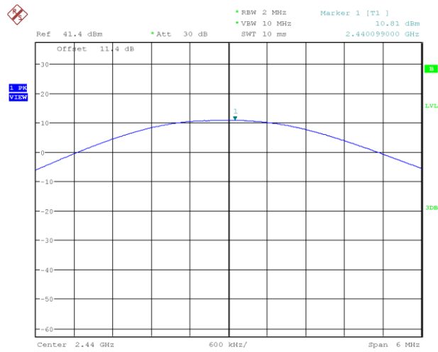
Plot 2. Maximum Conducted Power, 1Mbps 2440MHz
