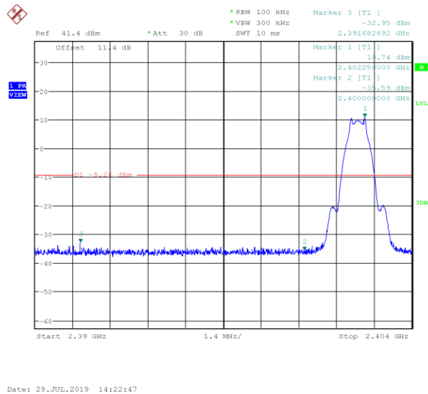
Plot 19. 1Mbps, 2402MHz Lower Band Edge
