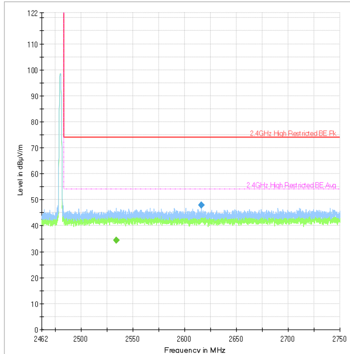
Plot 33. 1Mbps, 2480MHz, Upper Band Edge, Restricted
