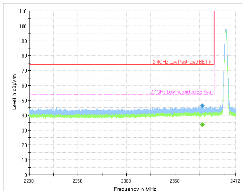
Plot 32. 2Mbps, 2402MHz, Lower Band Edge, Restricted
