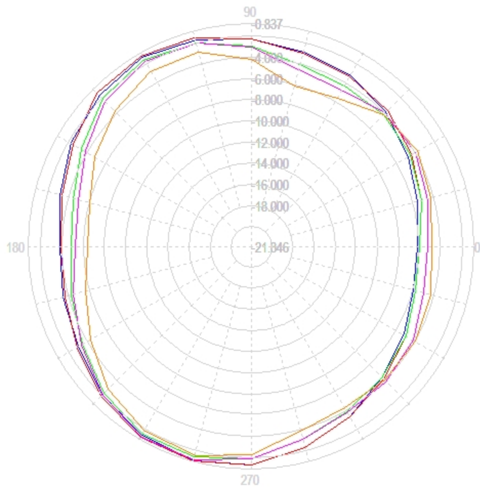
- H Plane Polar/Line Chart -
