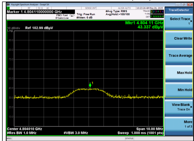
Low channel 2 nd harmonic (Peak)
