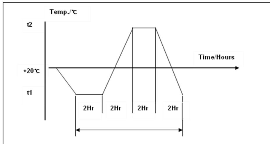
Figure 3.2.1 Temperature Cycling
