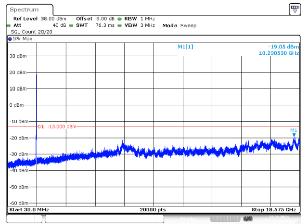
15MHz_Low_QPSK_75@0
