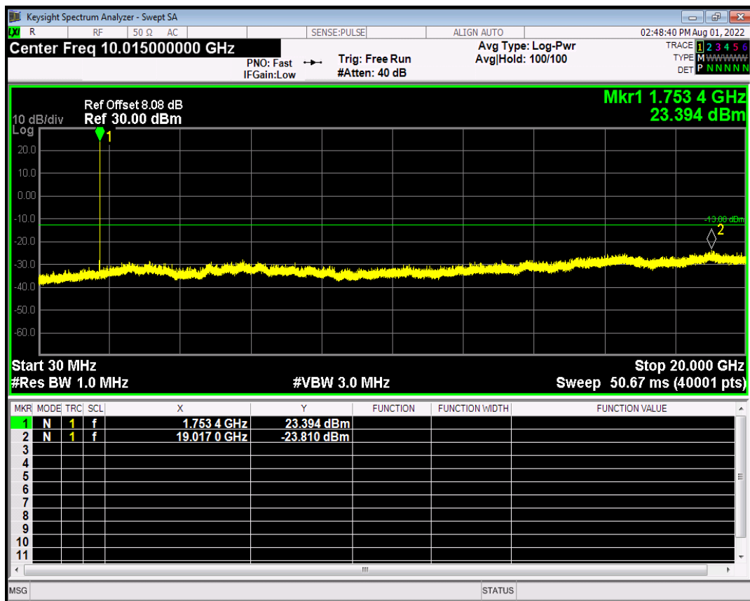
HSDPA Band4 Subtest2 Channel=1513
