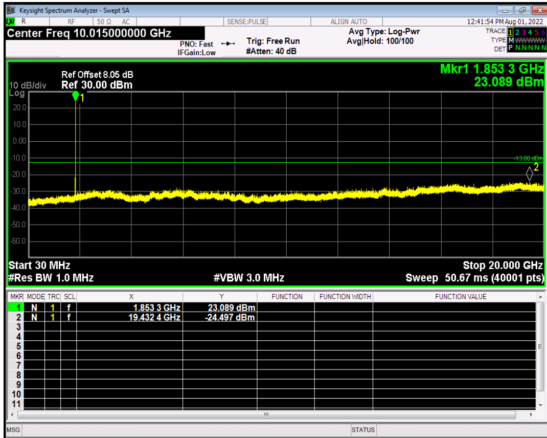
HSDPA Band2 Subtest2 Channel=9262
