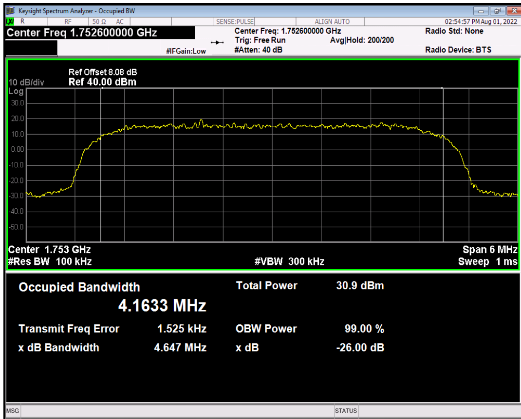
HSUPA Band4 Subtest3 Channel=1513
