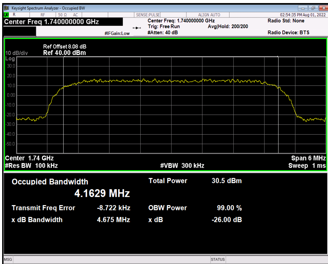
HSUPA Band4 Subtest2 Channel=1450
