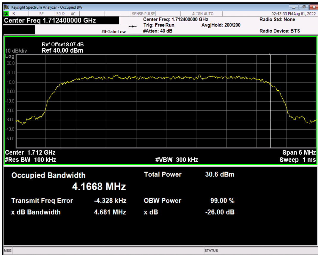
HSDPA Band4 Subtest2 Channel=1312
