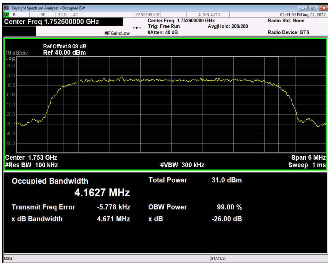
HSDPA Band4 Subtest2 Channel=1513
