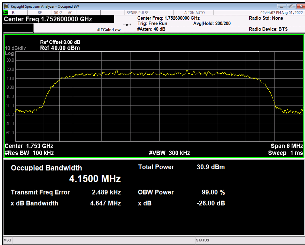
HSDPA Band4 Subtest3 Channel=1513
