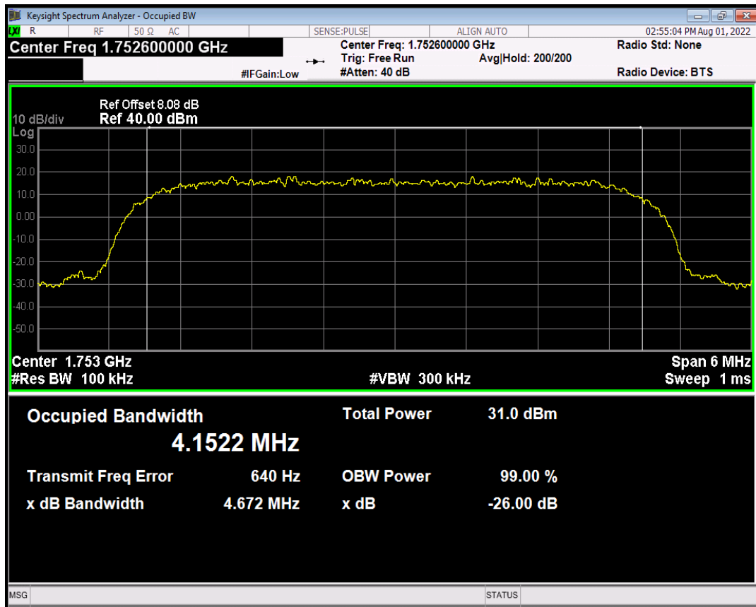
HSUPA Band4 Subtest5 Channel=1513
