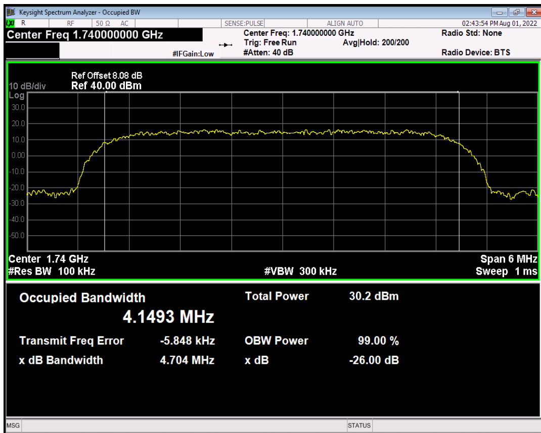
HSDPA Band4 Subtest4 Channel=1450
