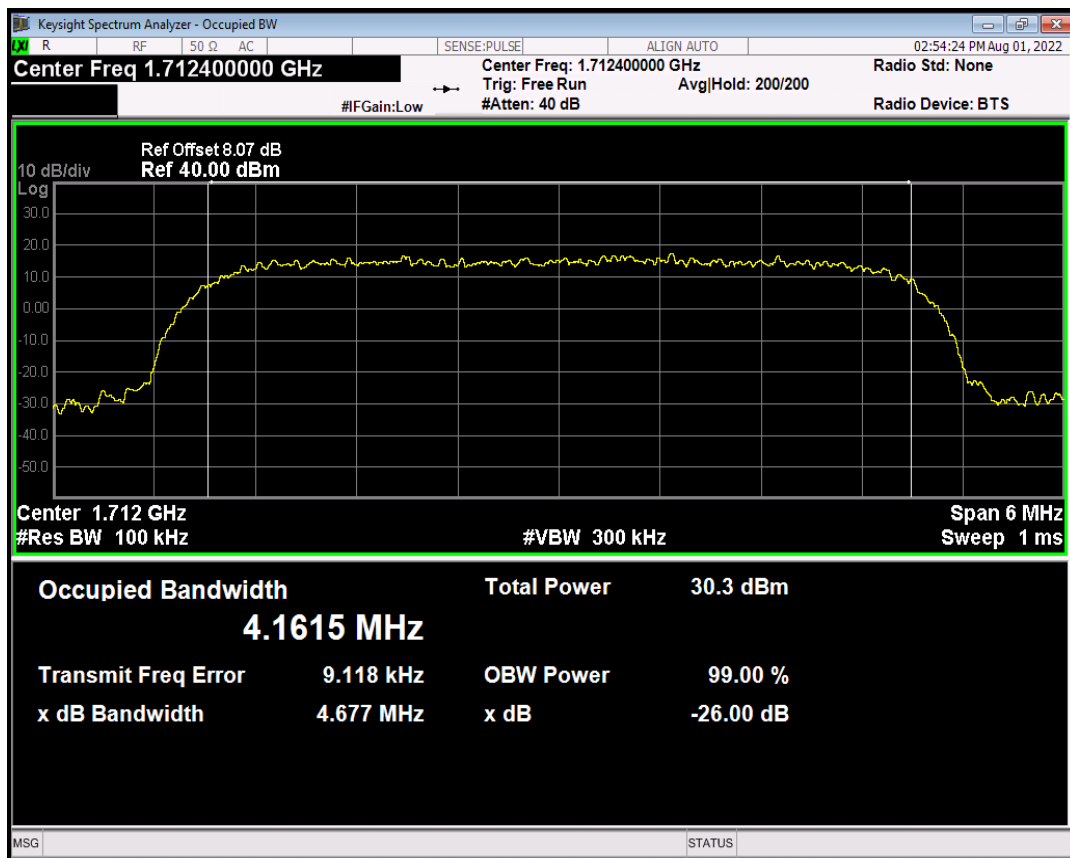
HSUPA Band4 Subtest4 Channel=1312
