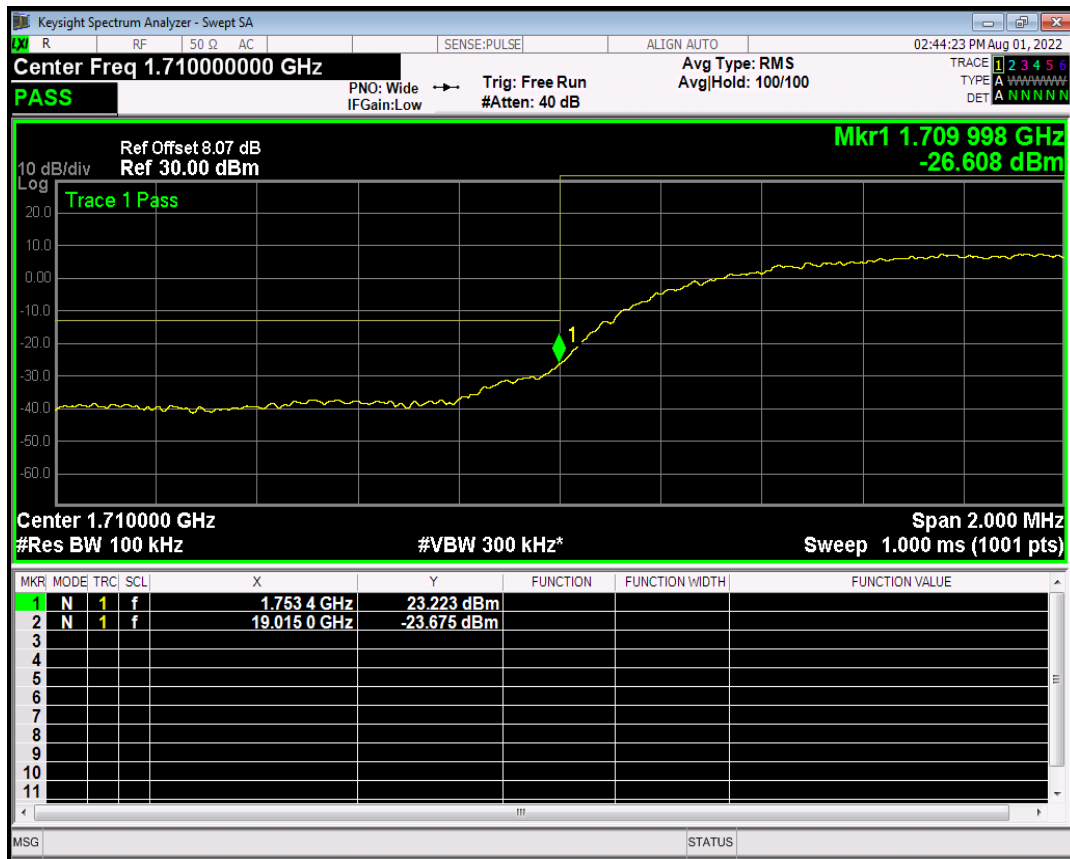
HSDPA Band4 Subtest3 Channel=1312
