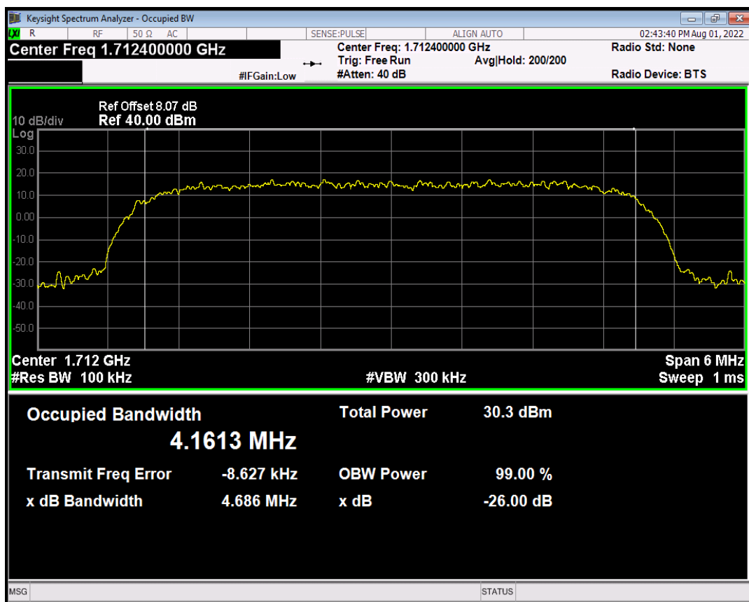
HSDPA Band4 Subtest4 Channel=1312
