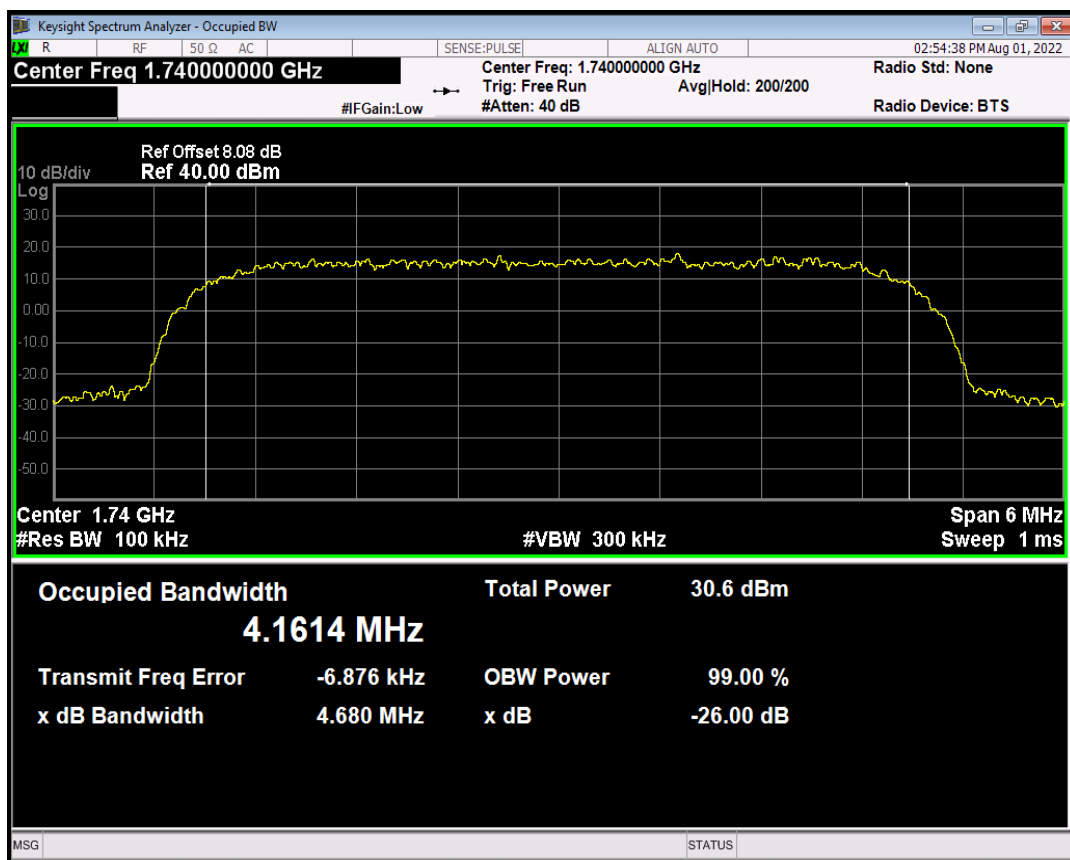
HSUPA Band4 Subtest3 Channel=1450
