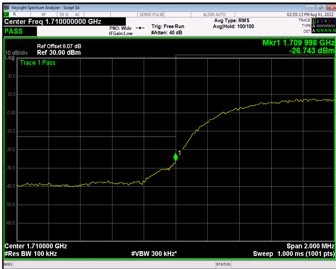
HSUPA Band4 Subtest2 Channel=1312
