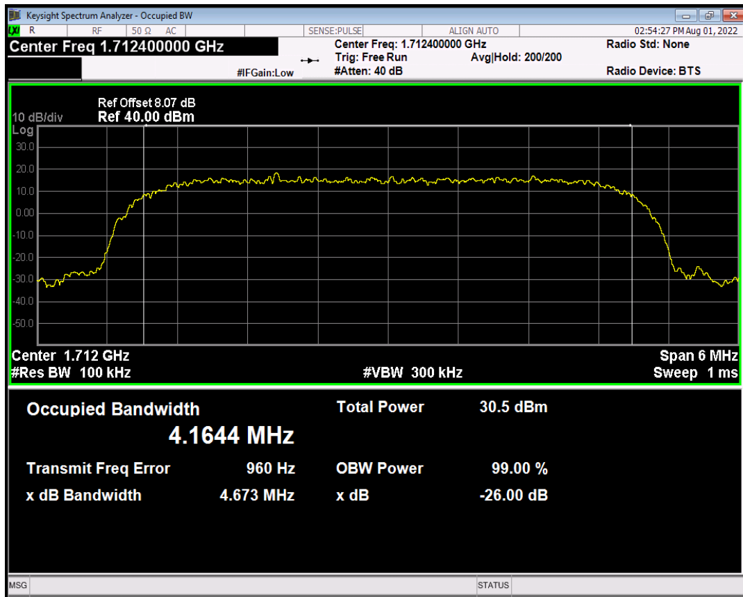
HSUPA Band4 Subtest5 Channel=1312
