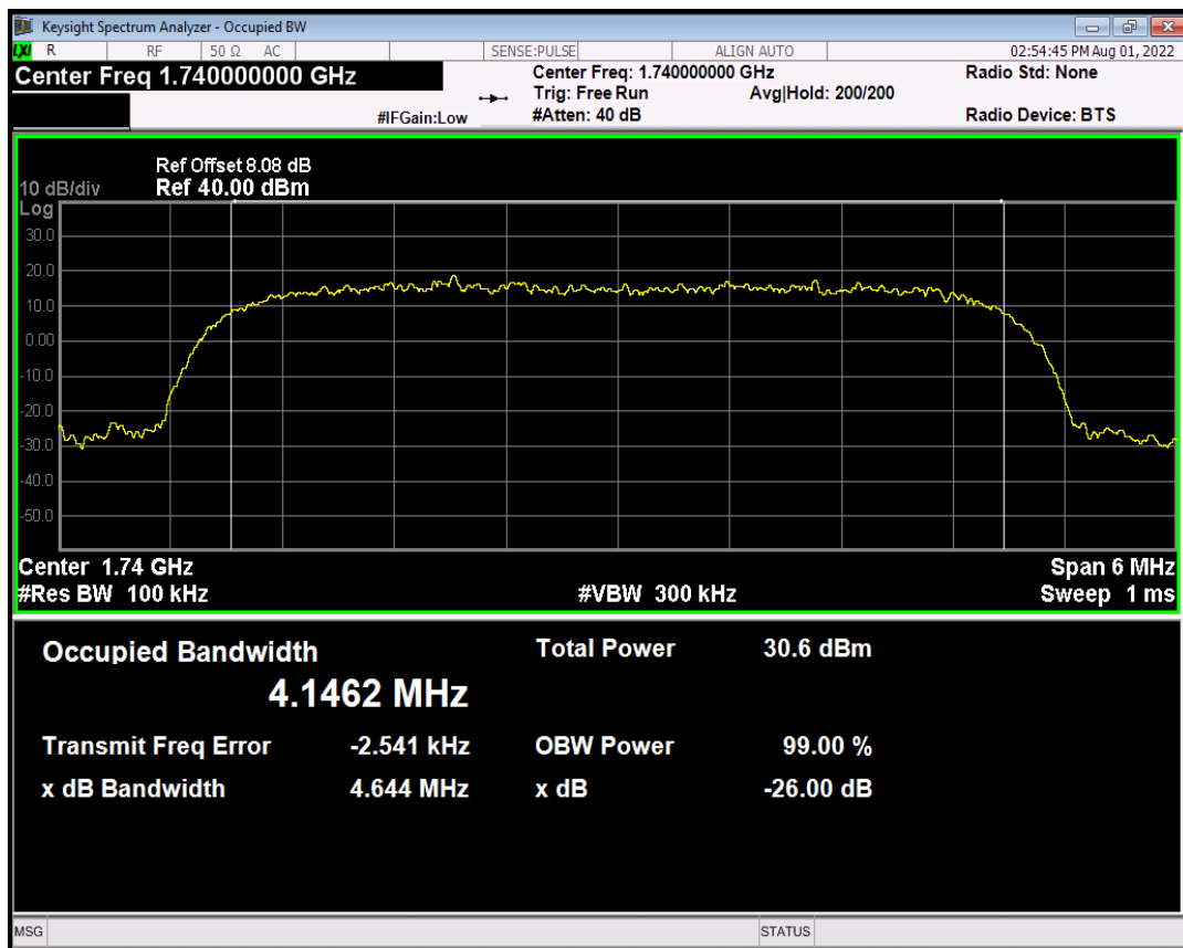
HSUPA Band4 Subtest5 Channel=1450
