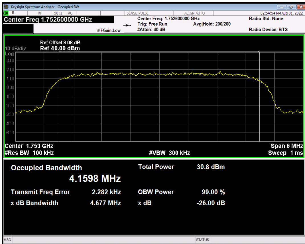
HSUPA Band4 Subtest2 Channel=1513
