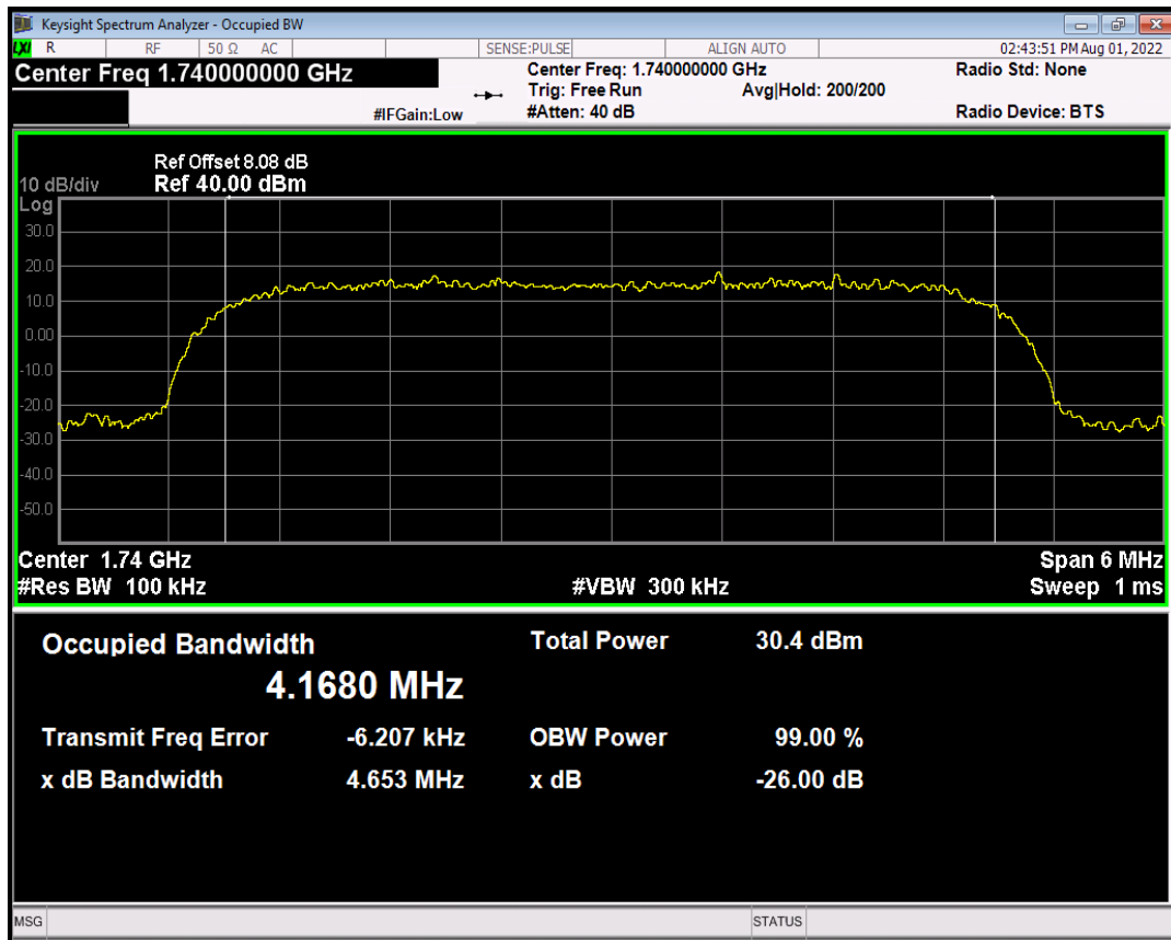
HSDPA Band4 Subtest3 Channel=1450
