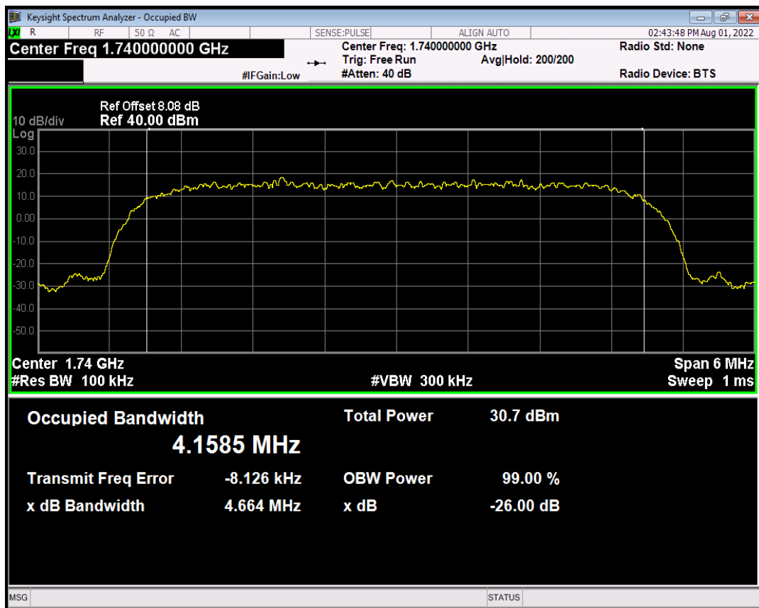
HSDPA Band4 Subtest2 Channel=1450
