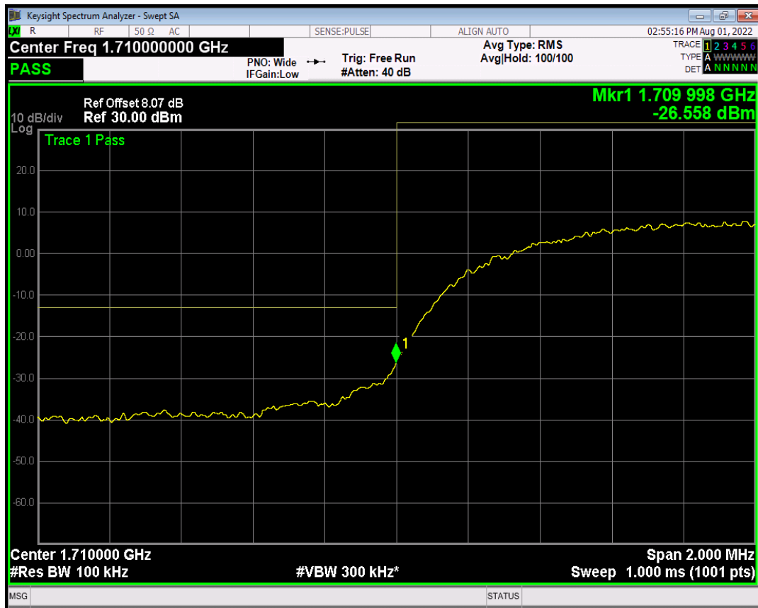
HSUPA Band4 Subtest3 Channel=1312
