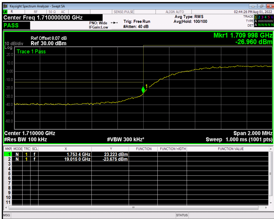
HSDPA Band4 Subtest4 Channel=1312
