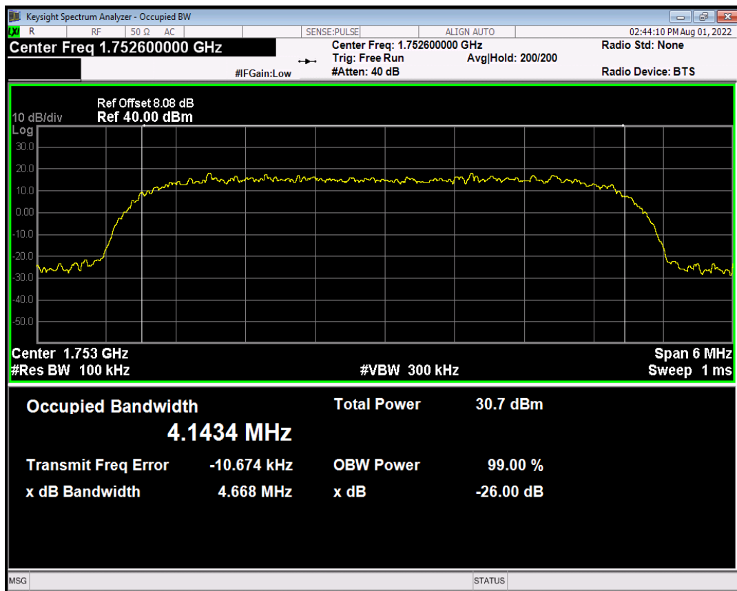
HSDPA Band4 Subtest4 Channel=1513
