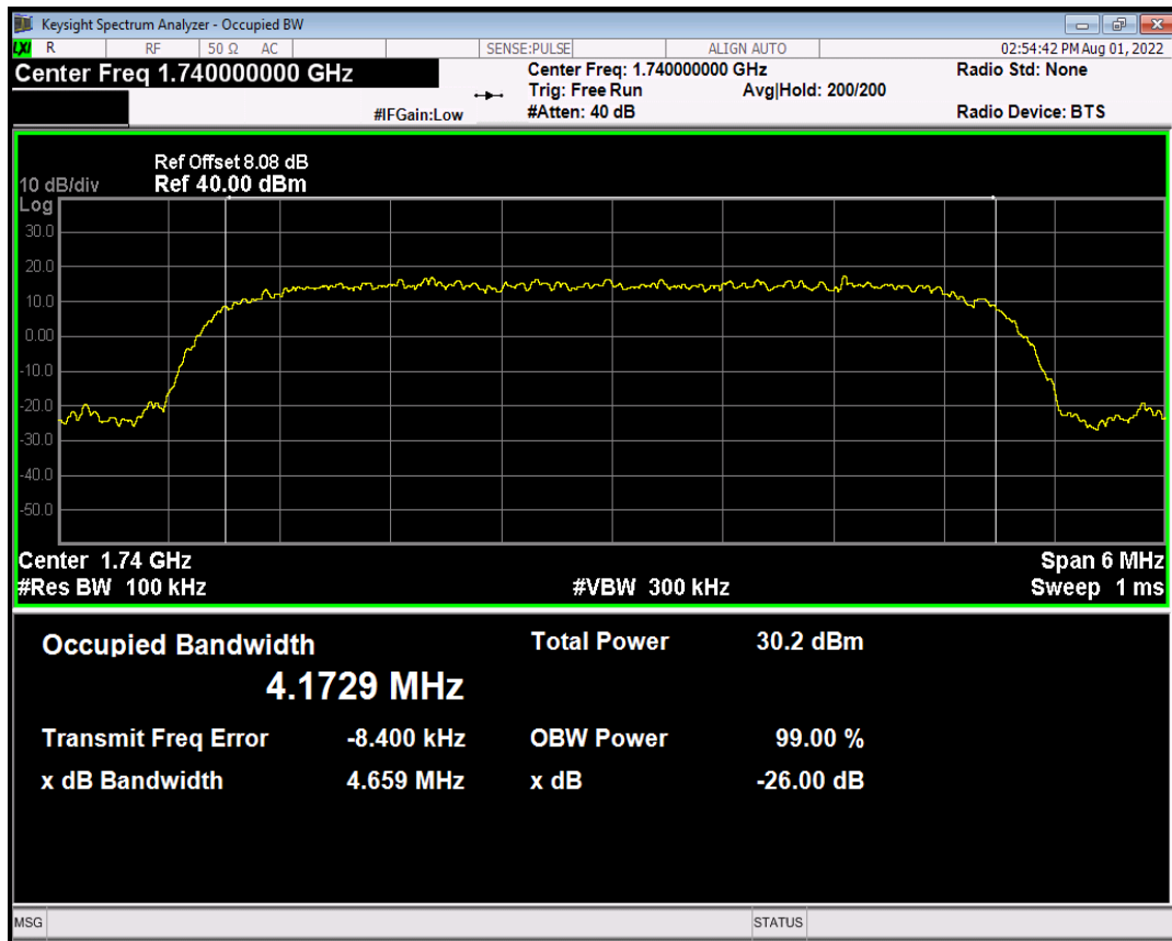
HSUPA Band4 Subtest4 Channel=1450
