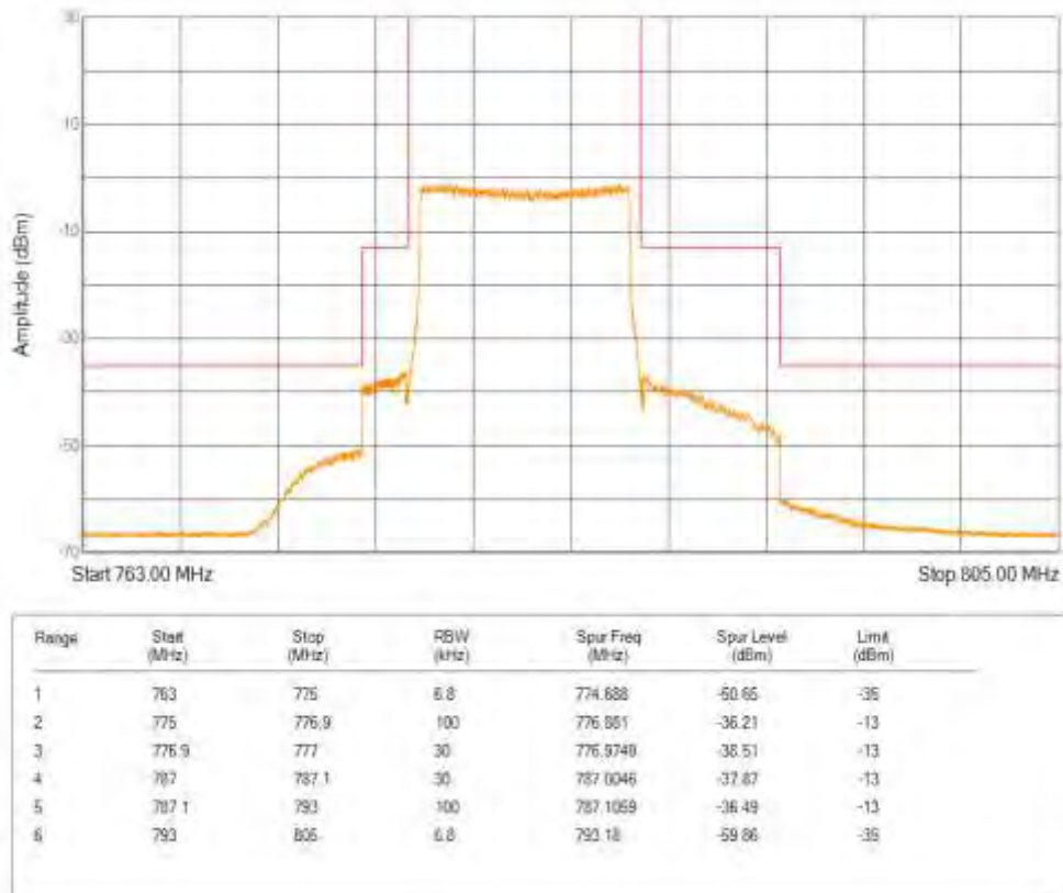
Band13 16QAM BW=5MHz Channel=23205 RB Size=25 Position=#0
