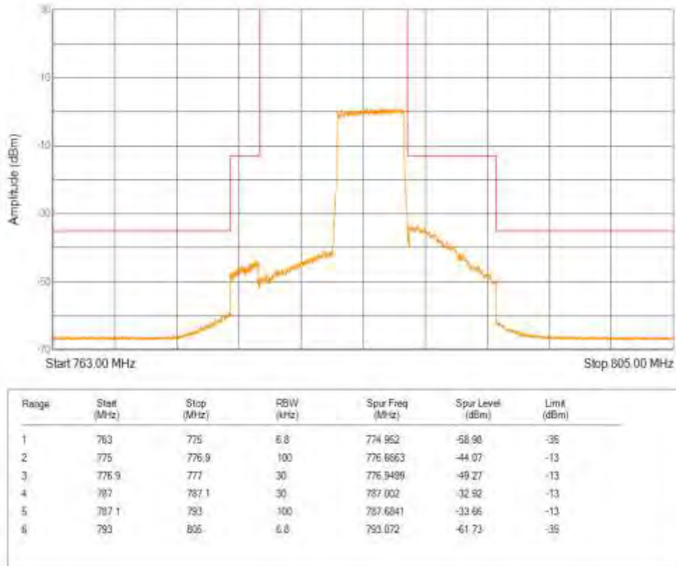
Band13 QPSK BW=10MHz Channel=23230 RB Size=50 Position=#0
