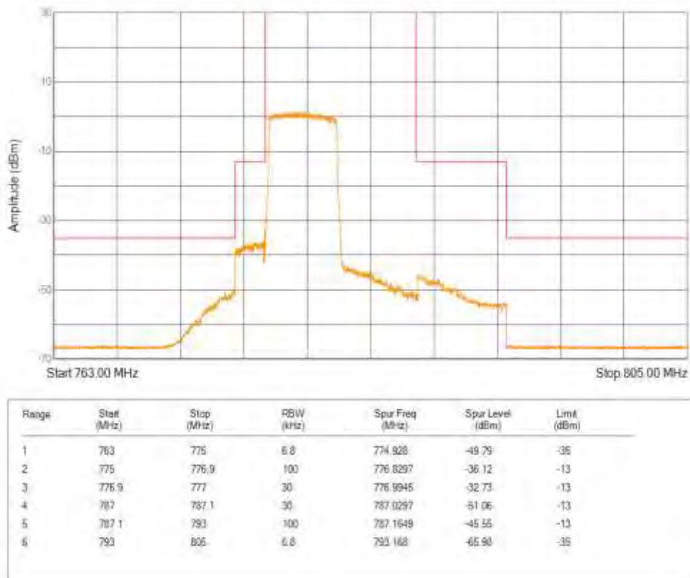
Band13 16QAM BW=5MHz Channel=23255 RB Size=25 Position=#0
