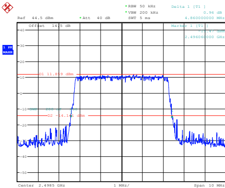
26dB Bandwidth
