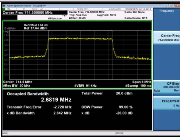
HCH_QPSK_15RB#0
