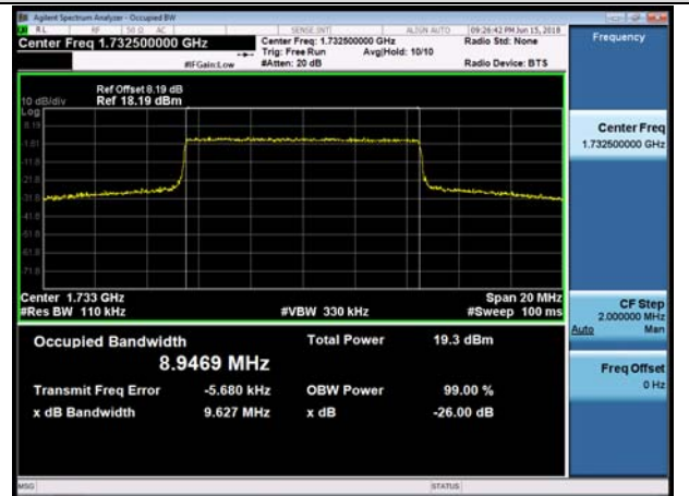
MCH_16QAM_50RB#0
