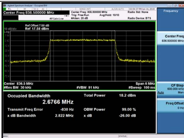
MCH_QPSK_15RB#0
