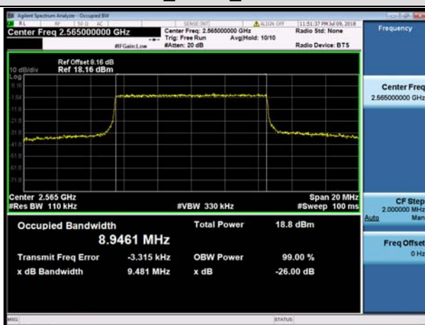
HCH_QPSK_50RB#0
