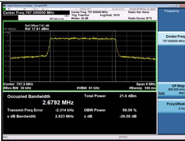
MCH_16QAM_15RB#0
