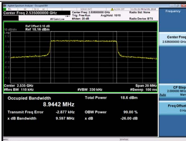
MCH_QPSK_50RB#0
