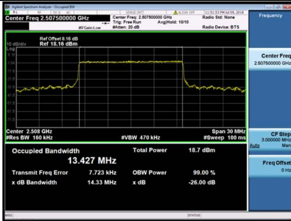
LCH_QPSK_75RB#0
