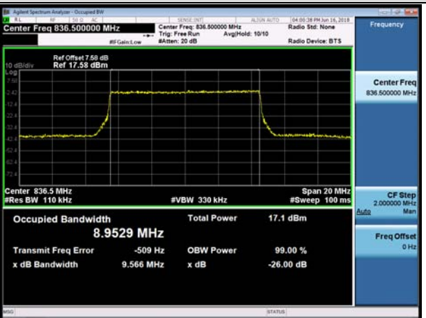
MCH_QPSK_50RB#0
