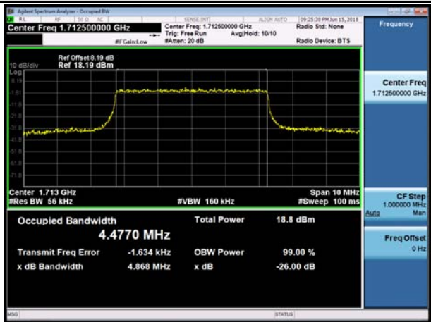
LCH_QPSK_25RB#0
