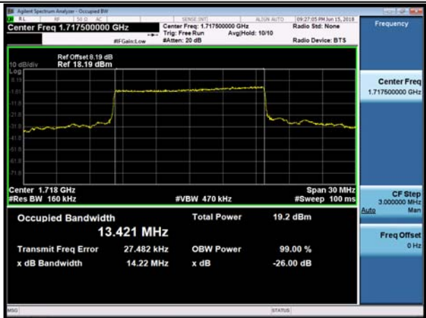
LCH_QPSK_75RB#0
