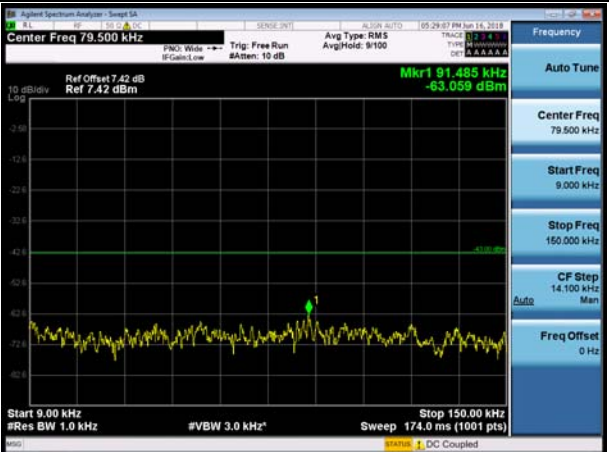
10MHz_LCH_QPSK_1RB#0
