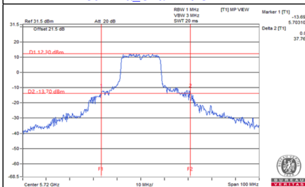
802.11ac (VHT40)_Chain 0 / CH142
