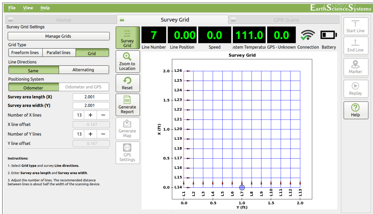
Figure 6: Survey Grid tab with open dock. Blue dot indicates current sensor position.
