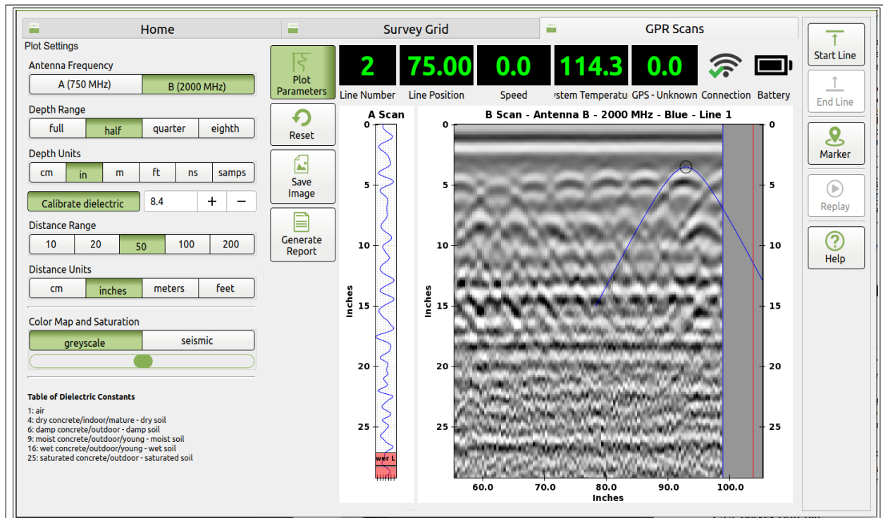
Figure 5: Plot settings dock. After clicking Calibrate dielectric , touch the top of a hyperbola. Then touch \pm or \pm until blue hyperbola matches the reflected radar arrivals on the screen.
